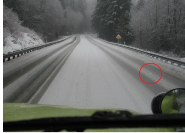
Figure 2-42 Laser path guidance system illustration and actual laser projection on the road from a winter operations vehicle (Laserline, 2018)
