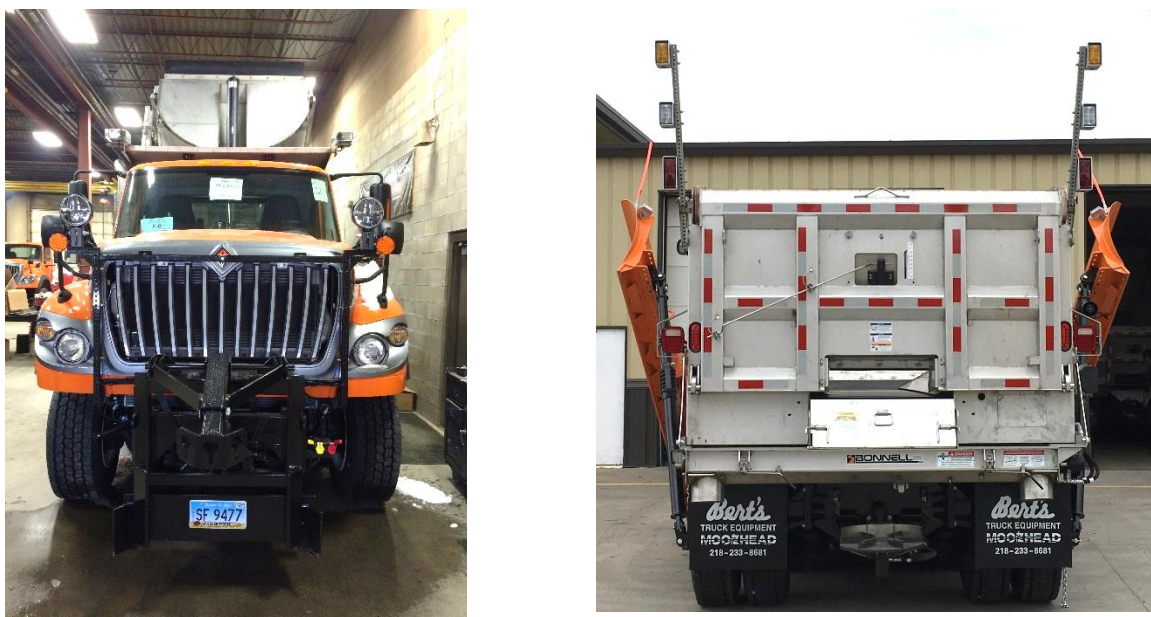
Figure 3-11 Front (left) and back (right) views of winter operations vehicles of North Dakota
