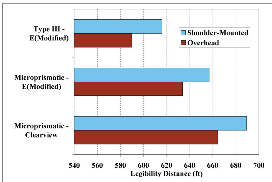
Figure 3. Legibility Results
