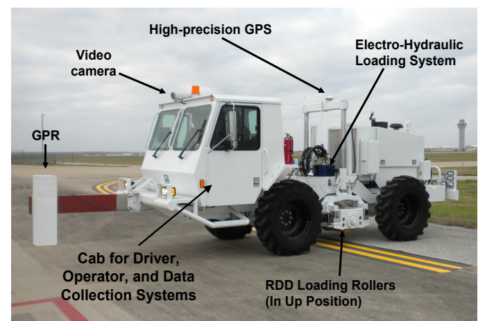
Figure 1. Photograph of the Total Pavement Acceptance Device Preparing to Evaluate a Jointed Concrete Pavement at the TxDOT Flight Services Facility.
