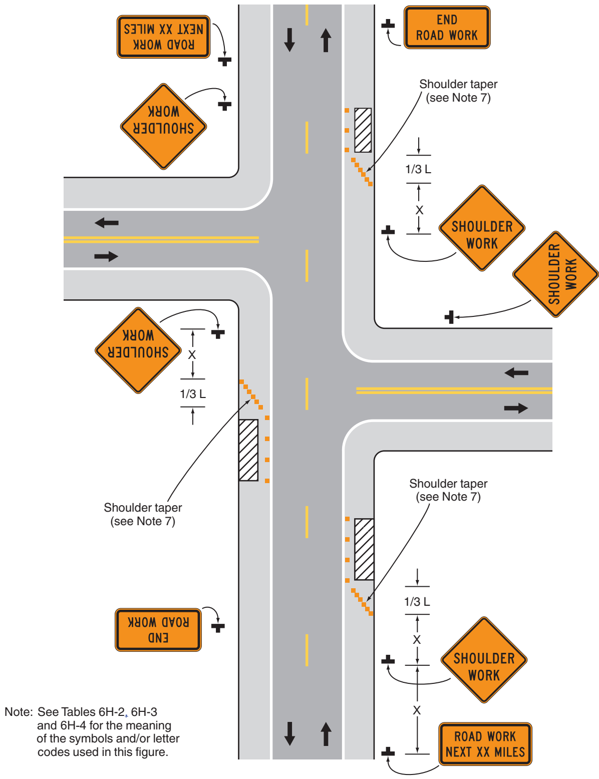
Typical Application 3
