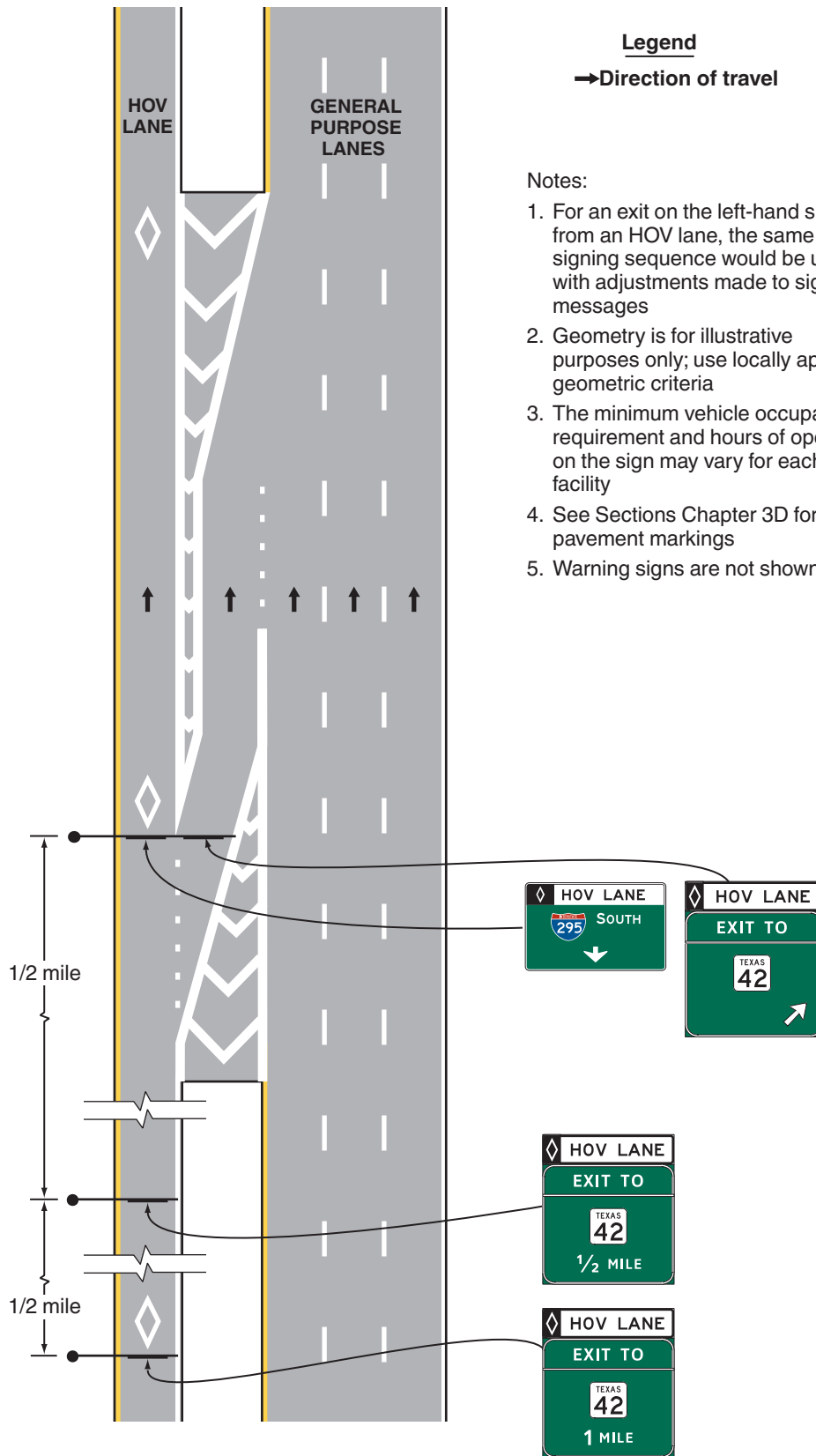
Figure 2G-12. Examples of Signs for an Intermediate Egress from a Barrier- or Buffer-Separated HOV Lane
