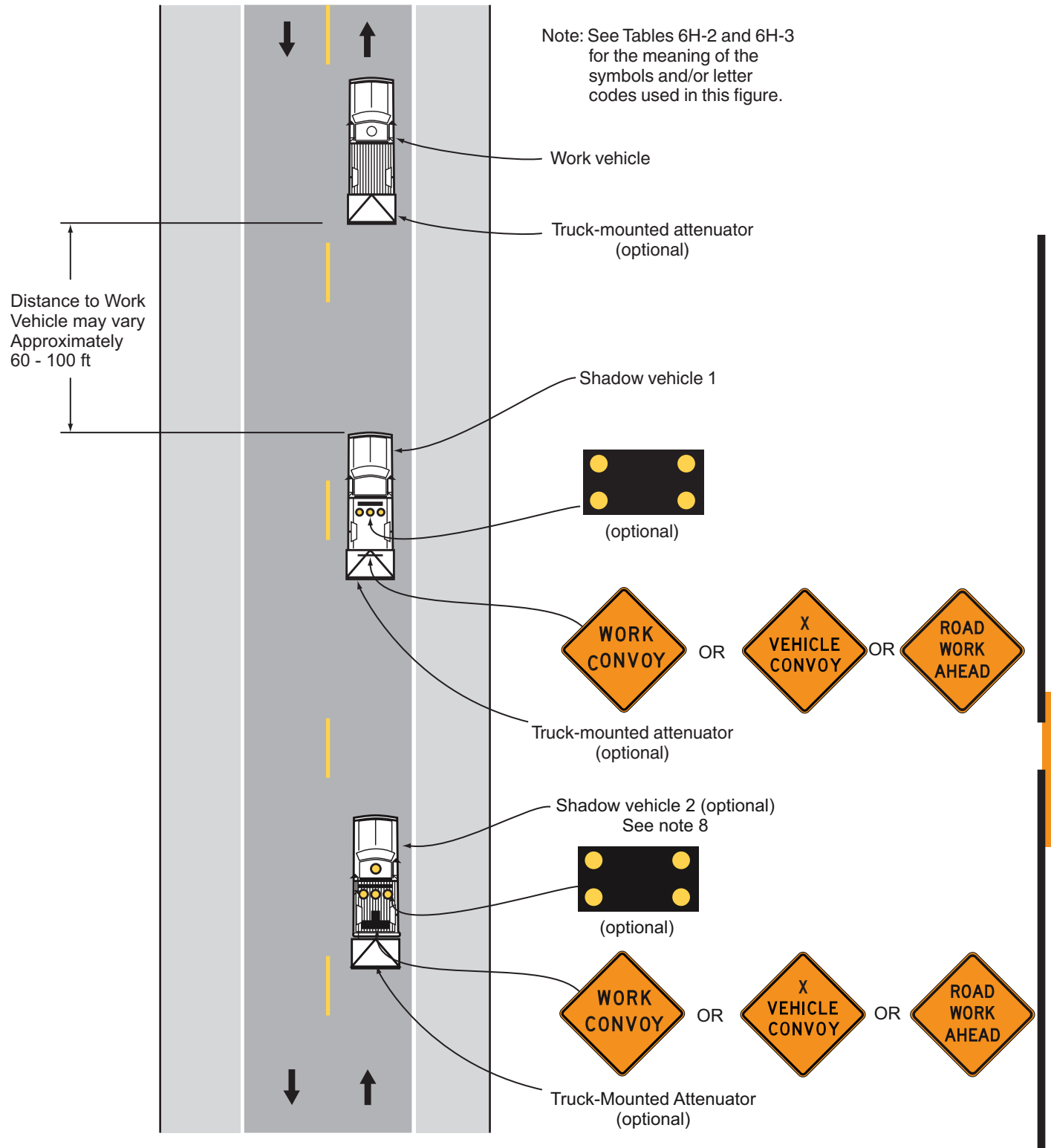
Typical Application 17
