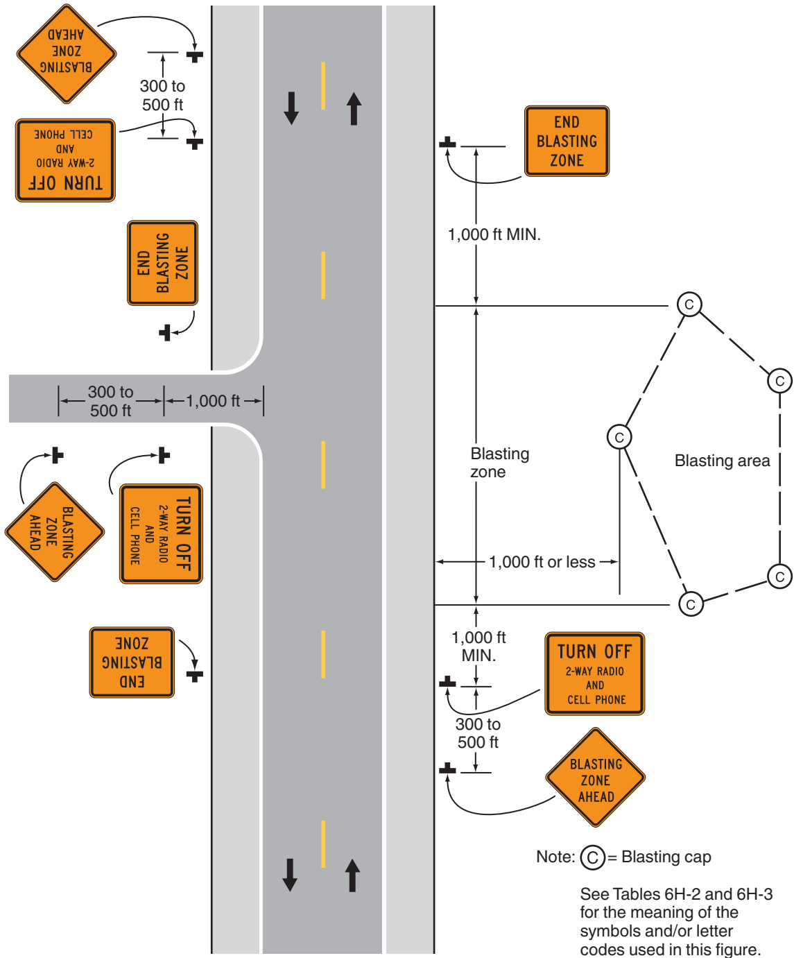
Typical Application 2
