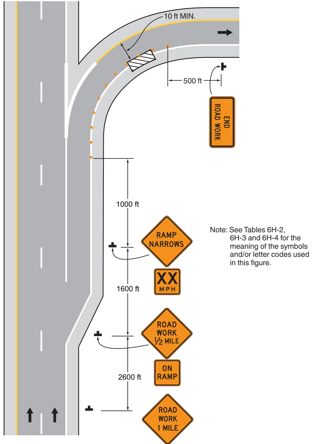
Typical Application 43
