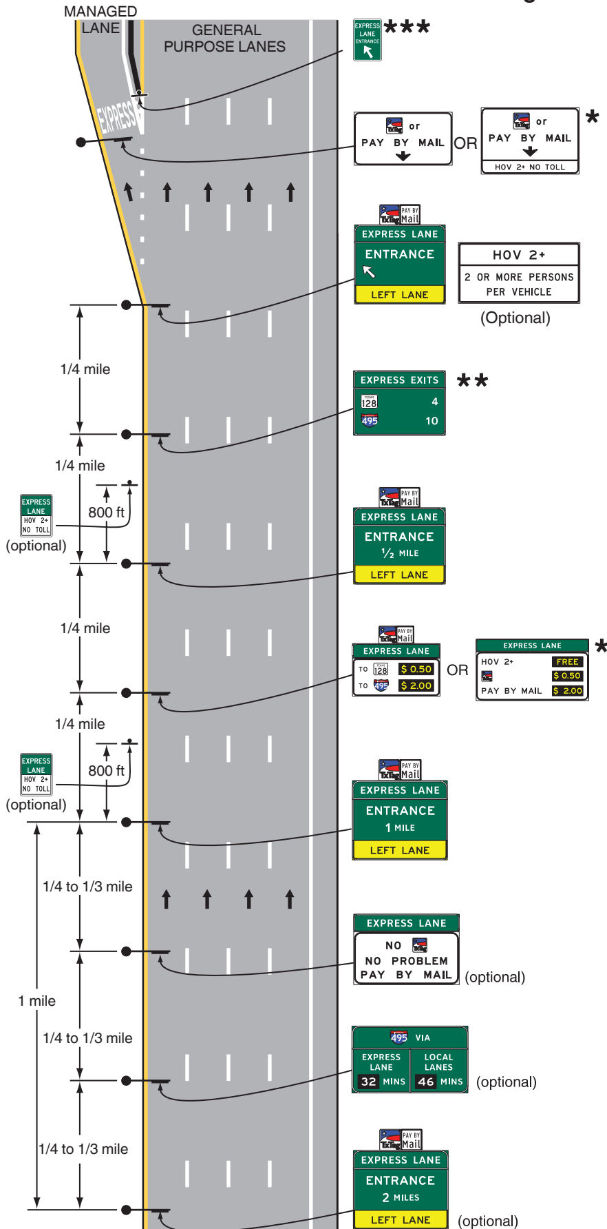
Figure 2G-21T. Example of Signing for the Entrance to an Access-Restricted Priced Managed Lane (Express Lane)
