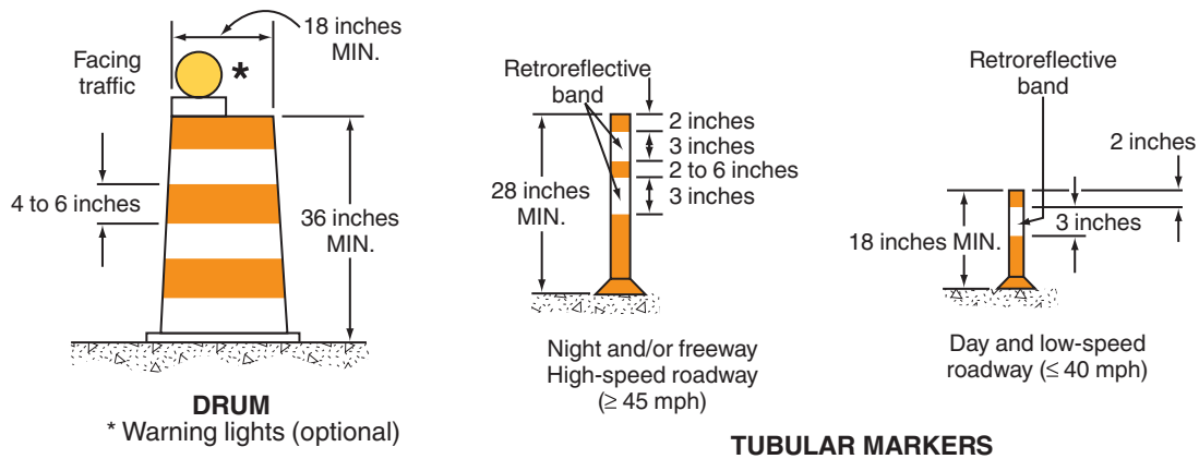
Figure 6F-7. Channelizing Devices (Sheet 1 of 2)
