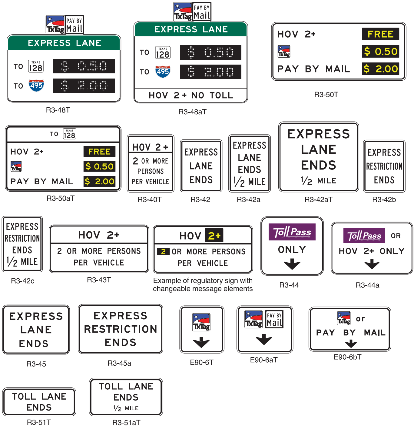
Figure 2G-17. Regulatory Signs for Managed Lanes
