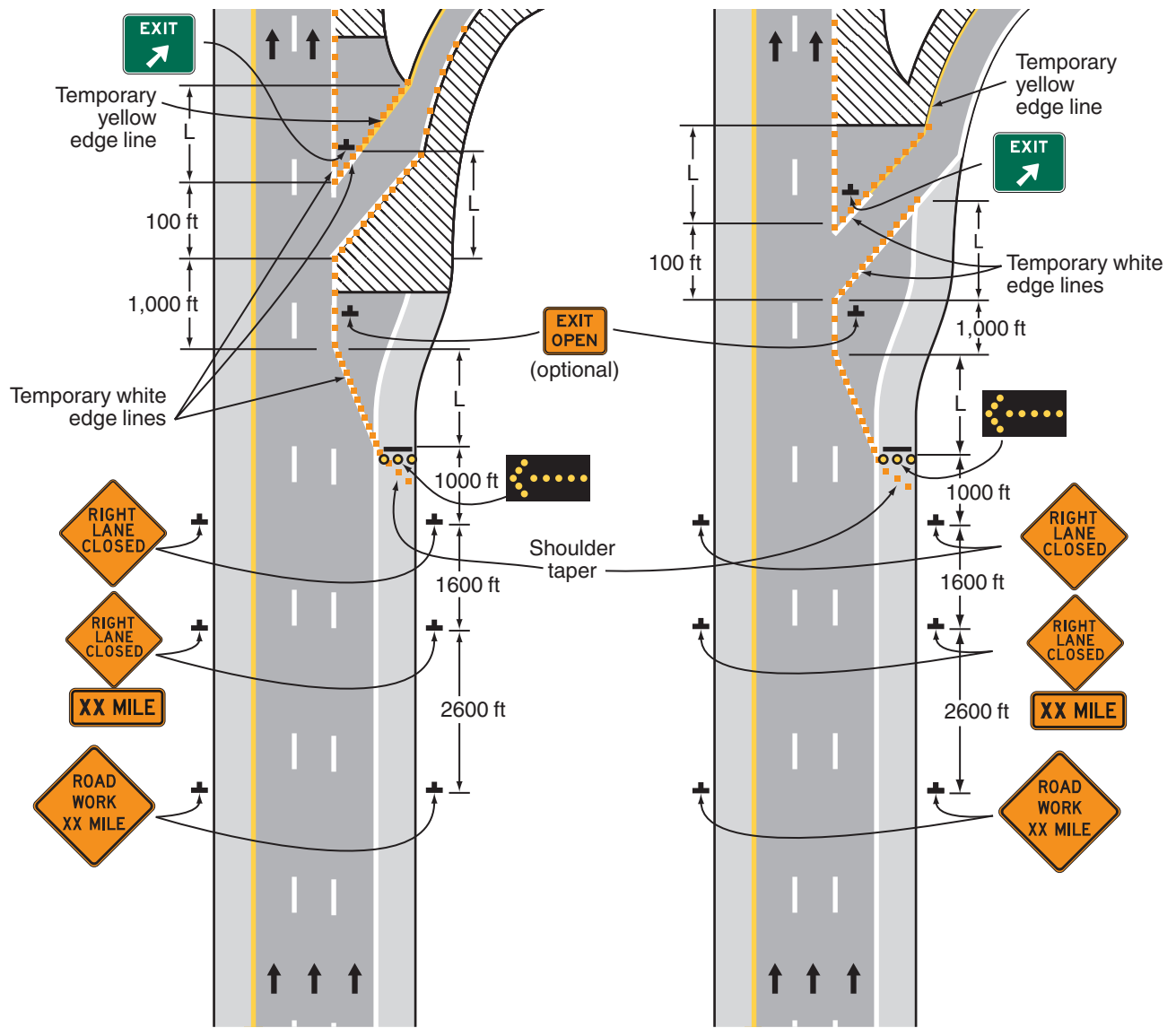
Typical Application 42
