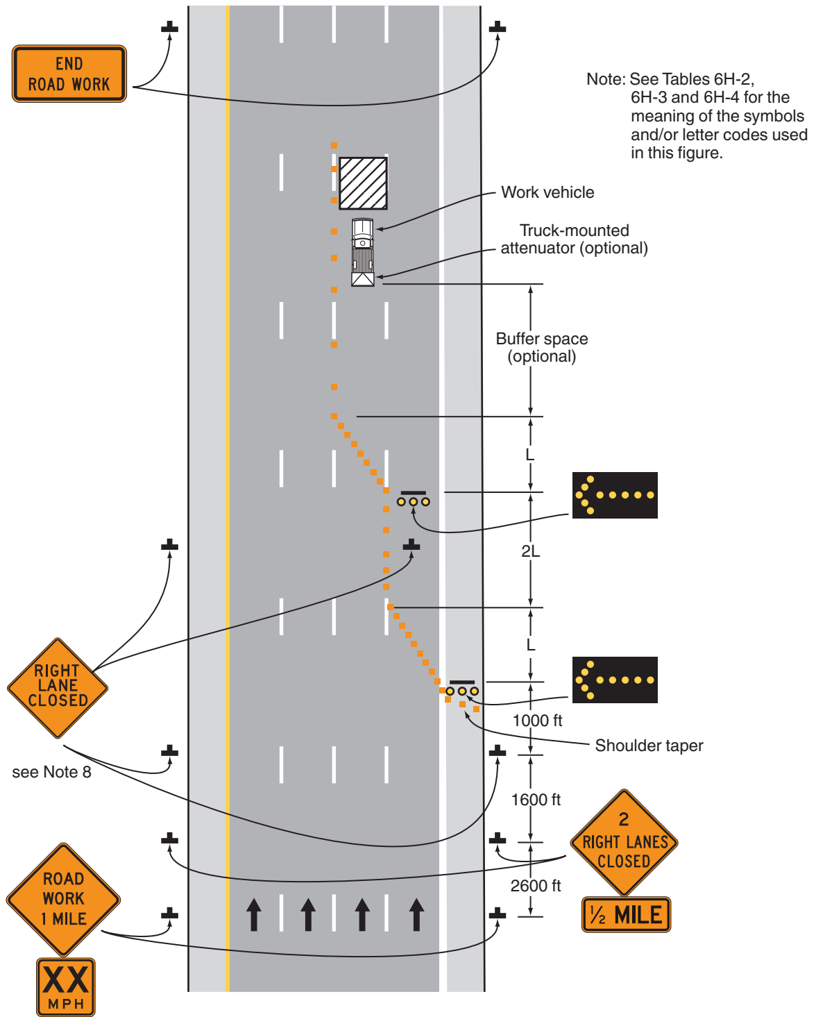
Typical Application 37
