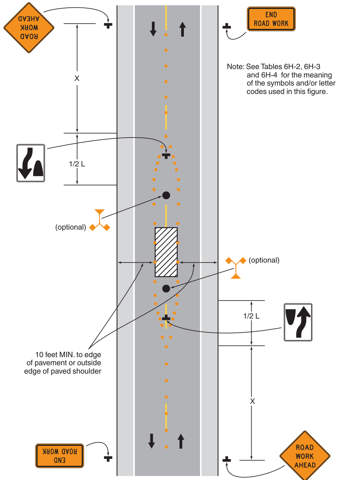
Typical Application 15
