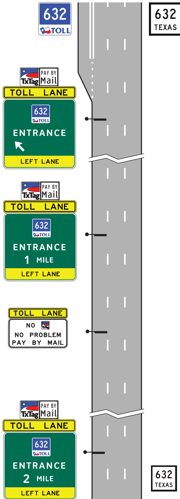
Figure 2F-7TB. Non -Toll Roadway with Left Lane Entrance to Toll Lane
