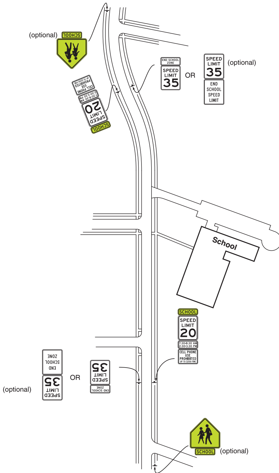
Figure 7B-3. Example of Signing for a Cell Phone Use Prohibited with a School Speed Limit
