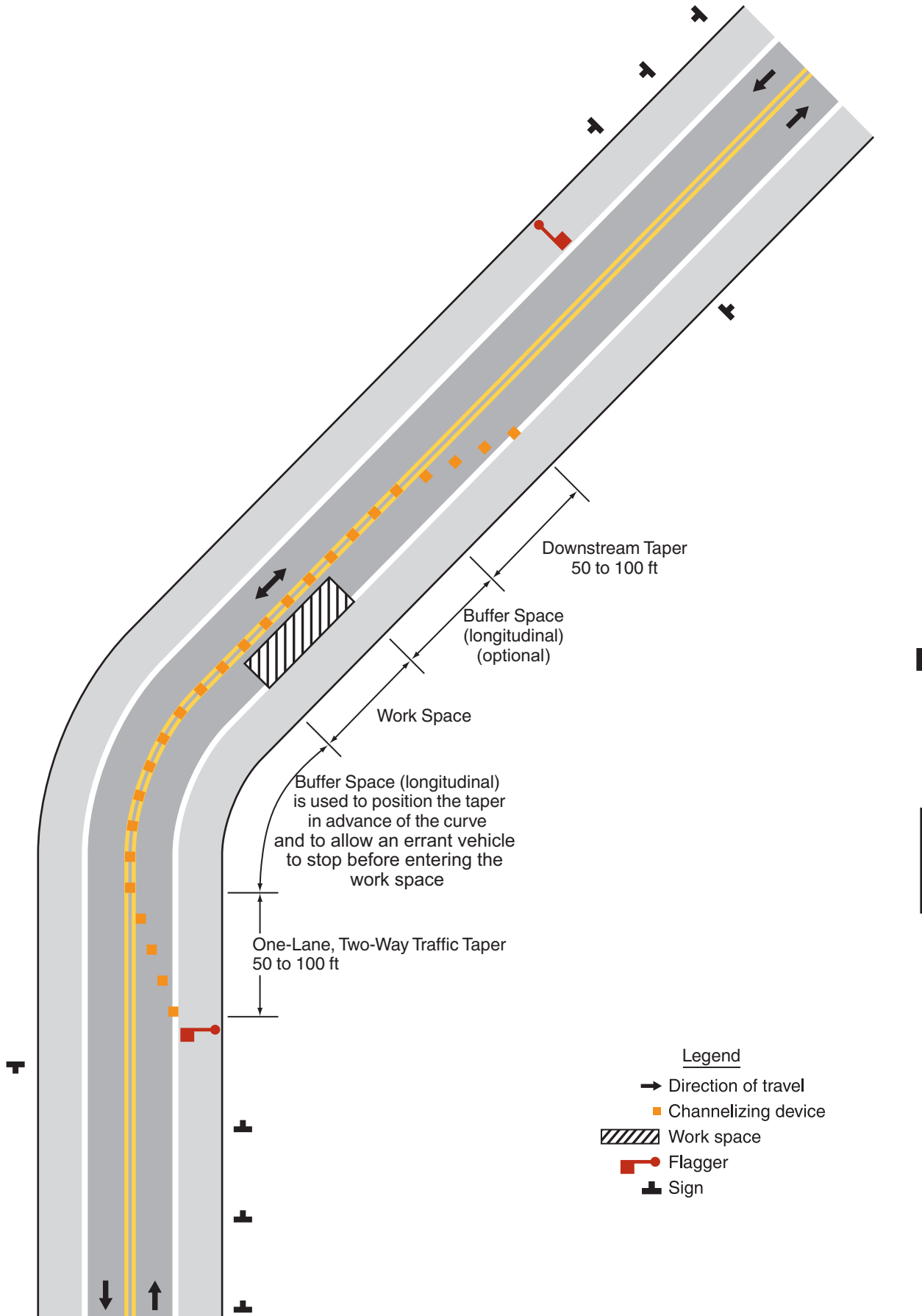
Figure 6C-3. Example of a One-Lane, Two-Way Traffic Taper
