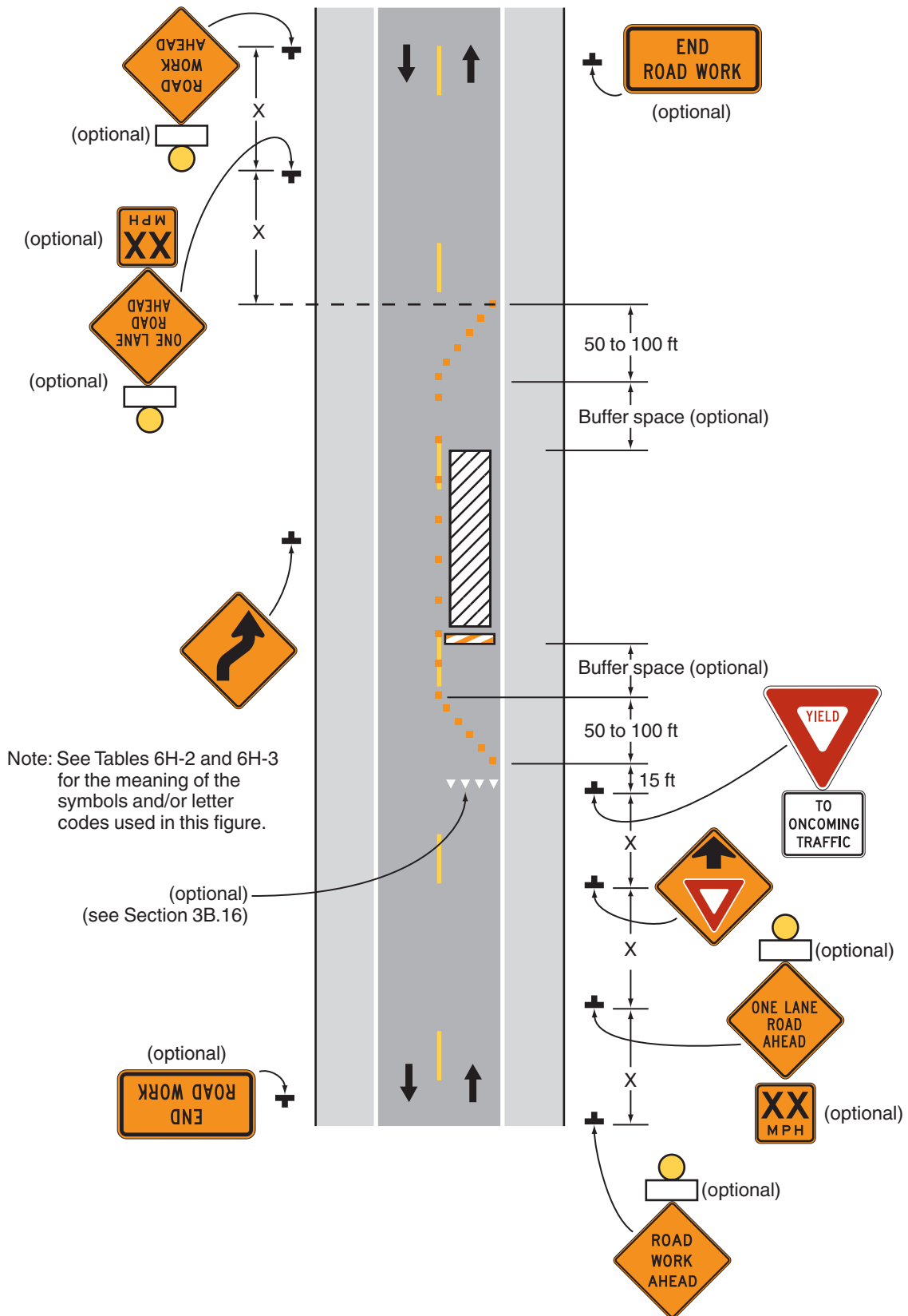
Typical Application 11
