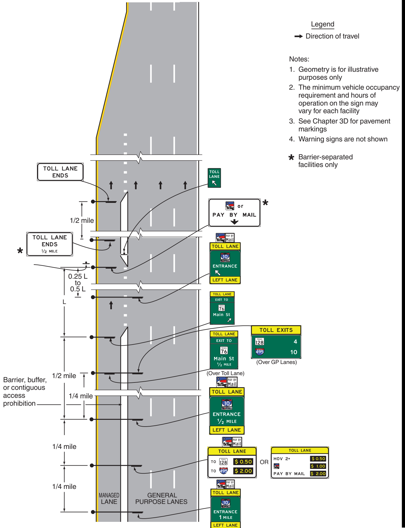
Figure 2G-24TA. Example of Signing for the Intermediate Entry to, Egress from, and End of Access-Restricted Priced Toll Lanes
