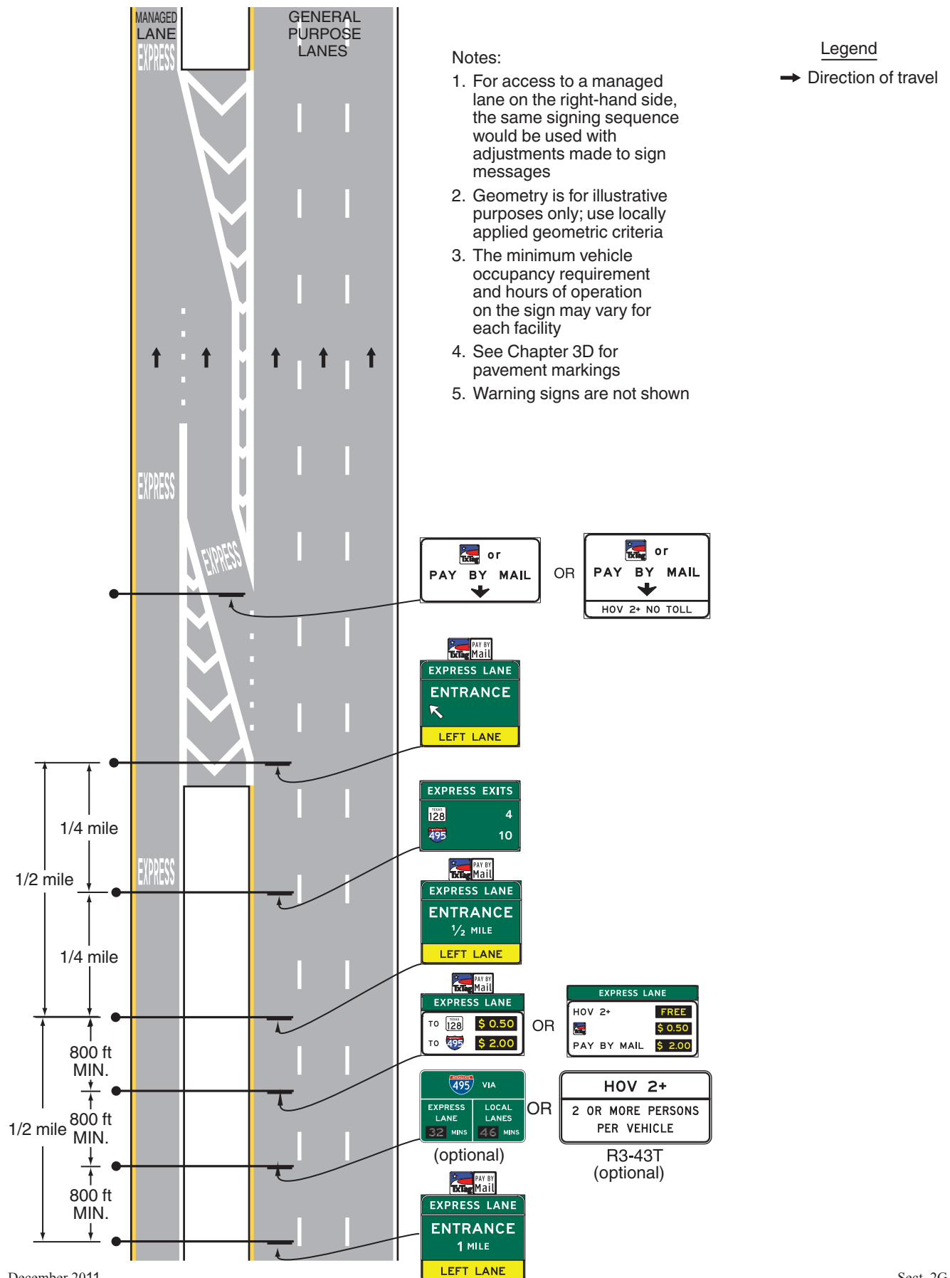
Figure 2G-23T. Example of Signing for an Intermediate Entry to a Barrier- or Buffer-Separated Priced Managed Lane
