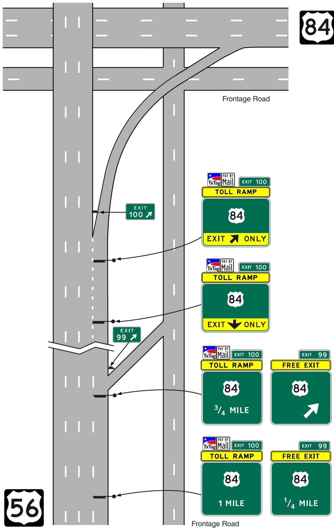
Figure 2F-6TB. Examples of Guide Signs from the Main Lanes to a Toll Ramp
