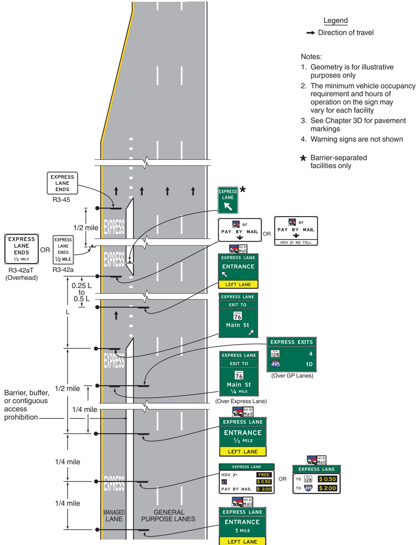
Figure 2G-24T. Example of Signing for the Intermediate Entry, Egress from, and End of Access-Restricted Priced Express Lanes
