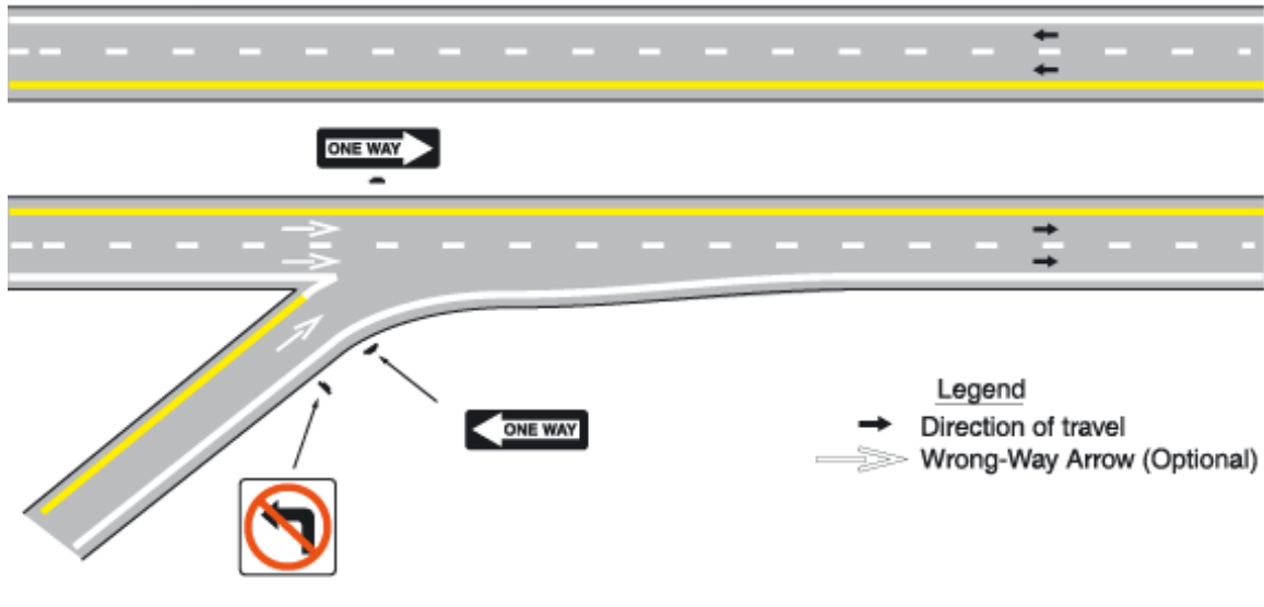
Figure 2E-32. Typical Regulatory Signing and Pavement Markings at Entrance Ramp Terminal Where Design Does Not Clearly Indicate the Direction of Flow
