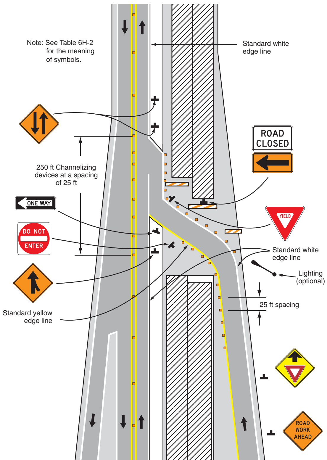
Typical Application 40
