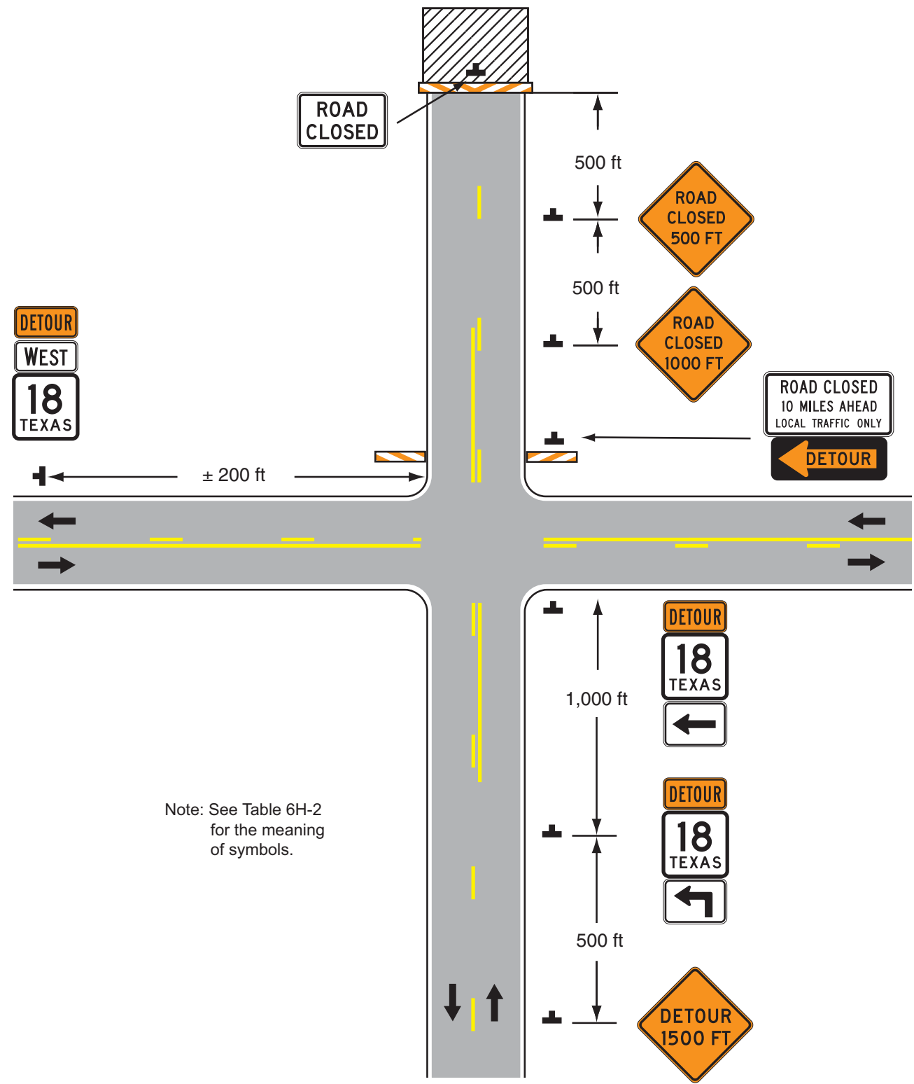
Typical Application 8
