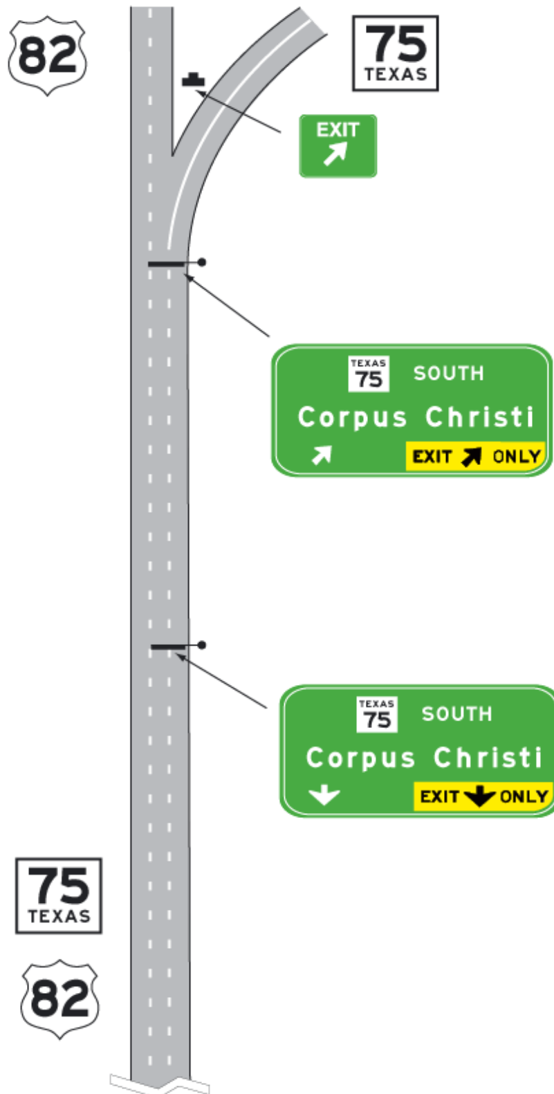
Figure 2E-9b. Two Lane EXIT ONLY Panels with an Option Lane for Two Lanes Dropped at an Interchange
