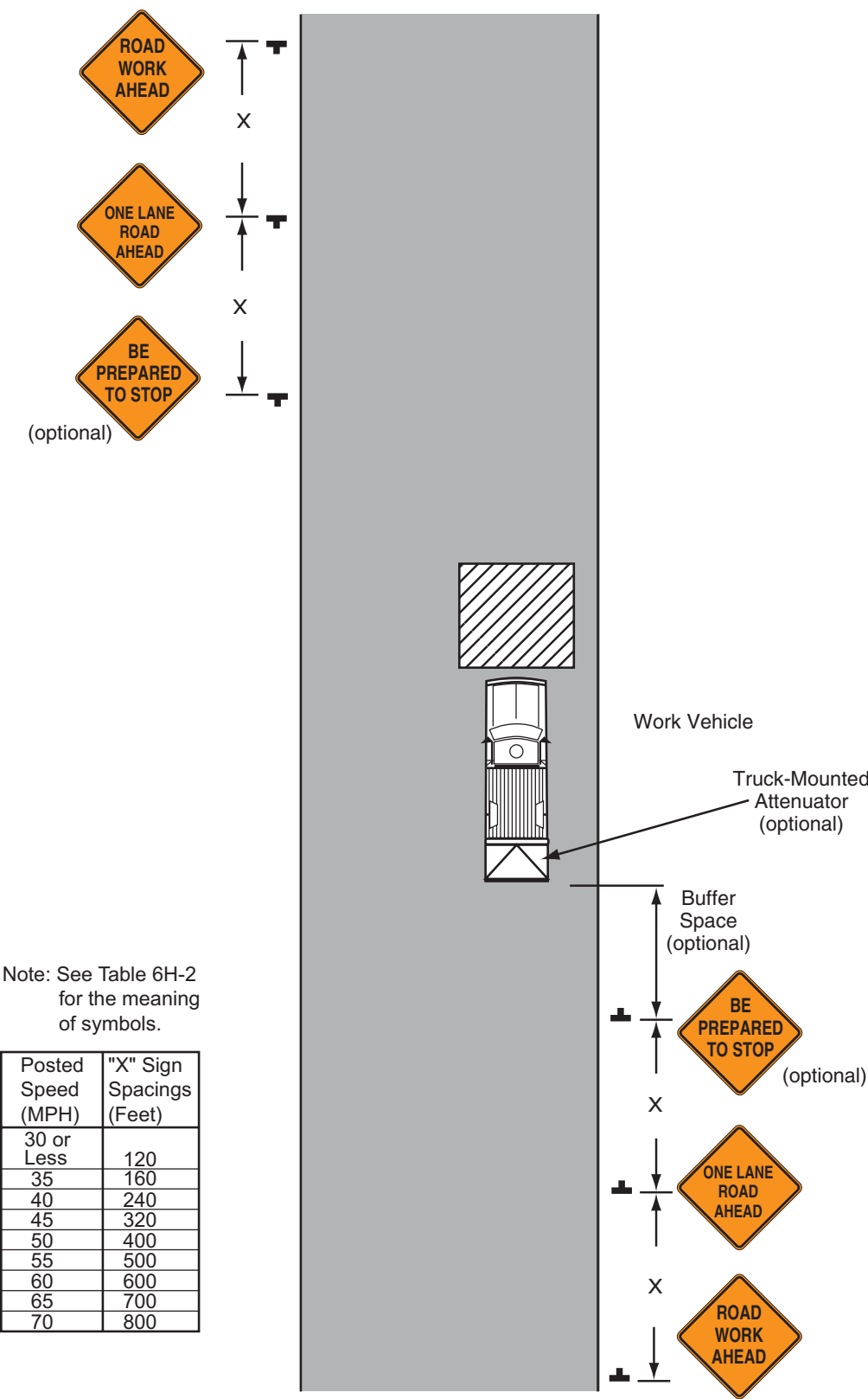
Typical Application 2
