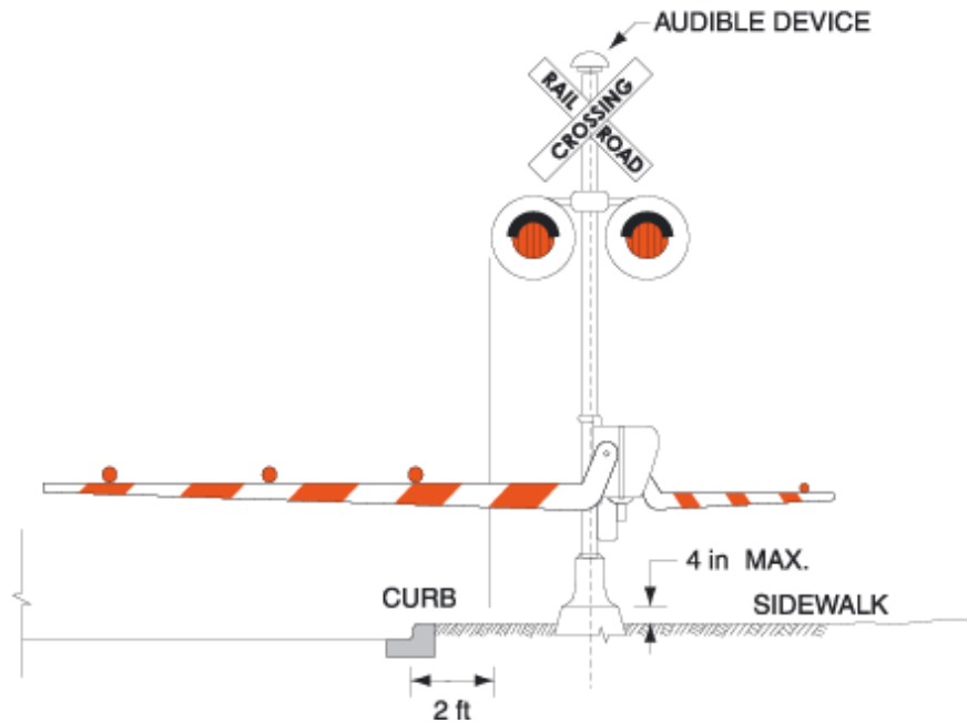
Figure 10D-4. Typical Pedestrian Gate Placement with Pedestrian Gate Arm
