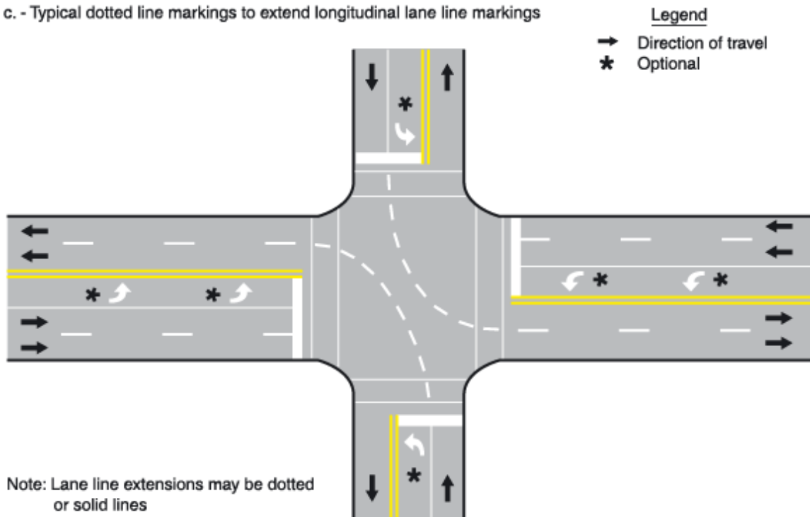
Figure 3B-11. Typical Pavement Marking Applications (Sheet 2 of 2)
