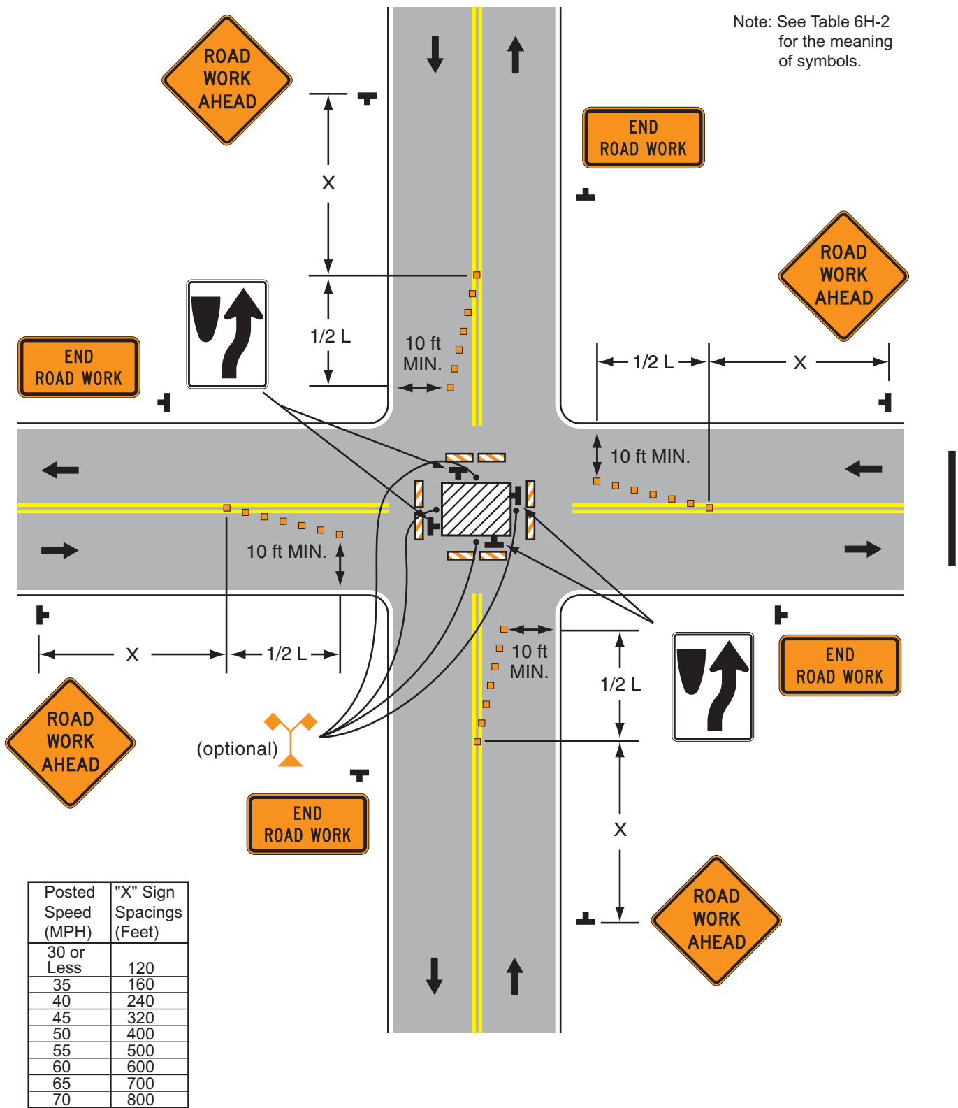
Typical Application 26
