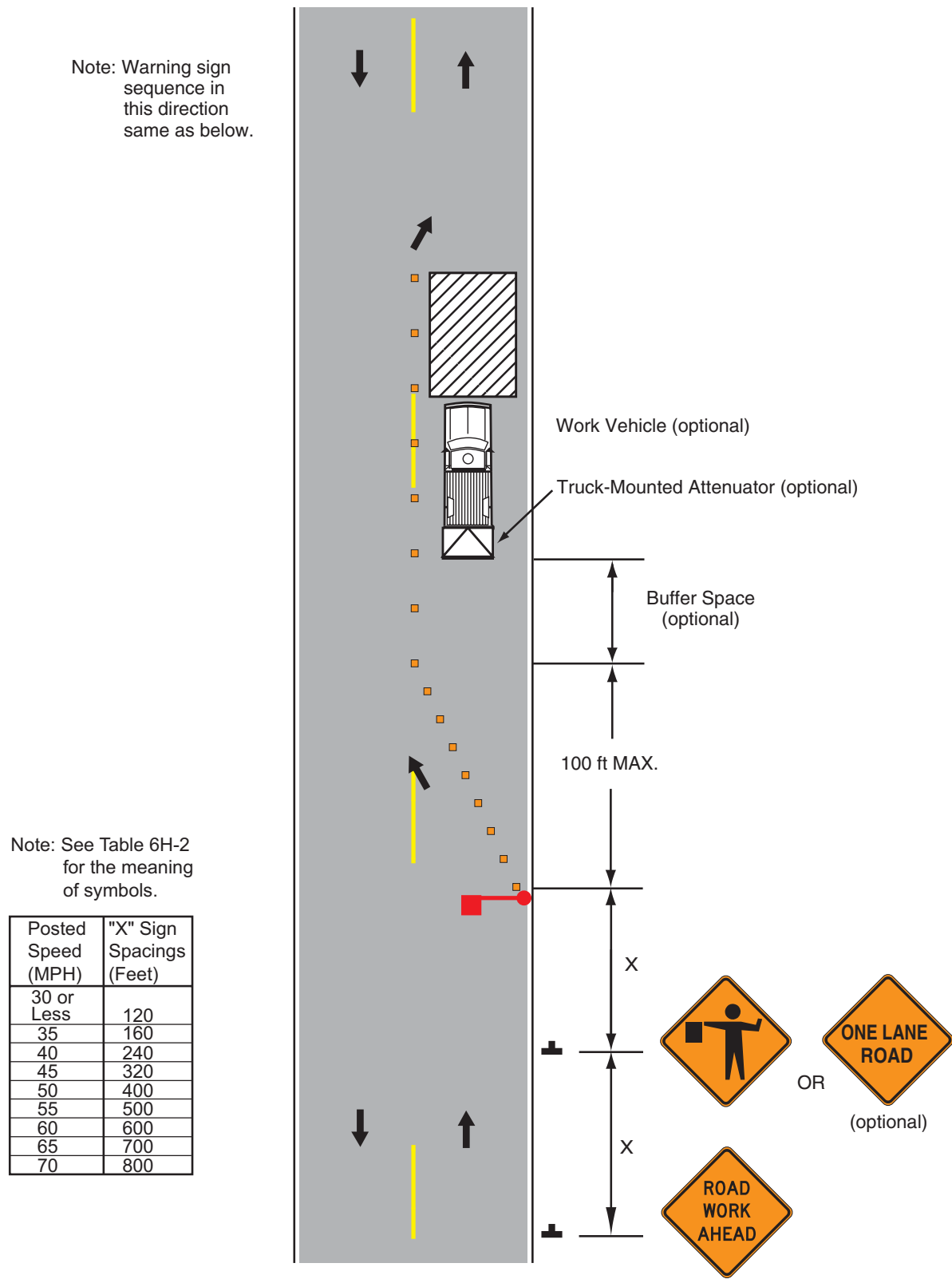
Typical Application 18
