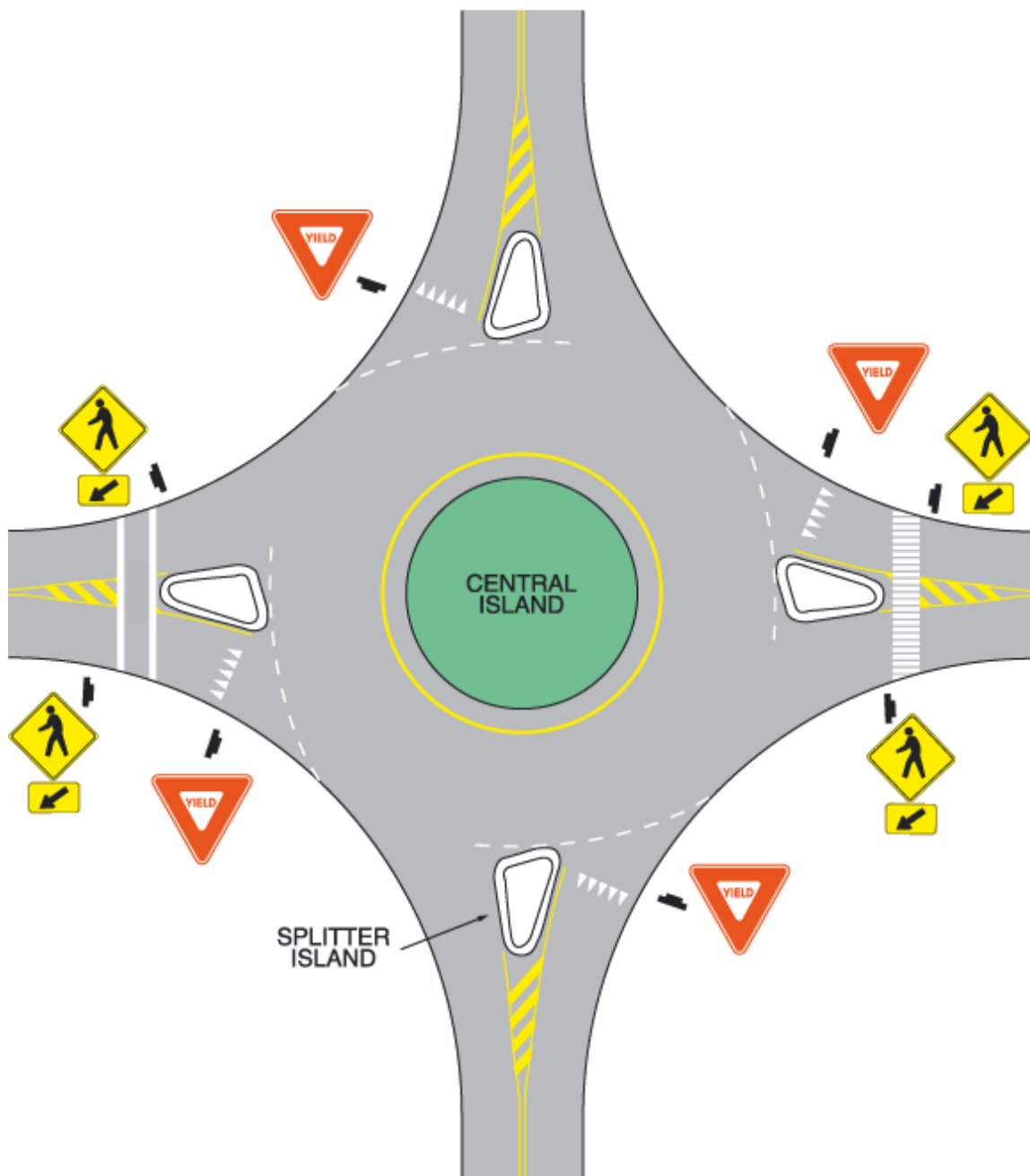
Figure 3B-26. Typical Markings for Roundabouts with One Lane
