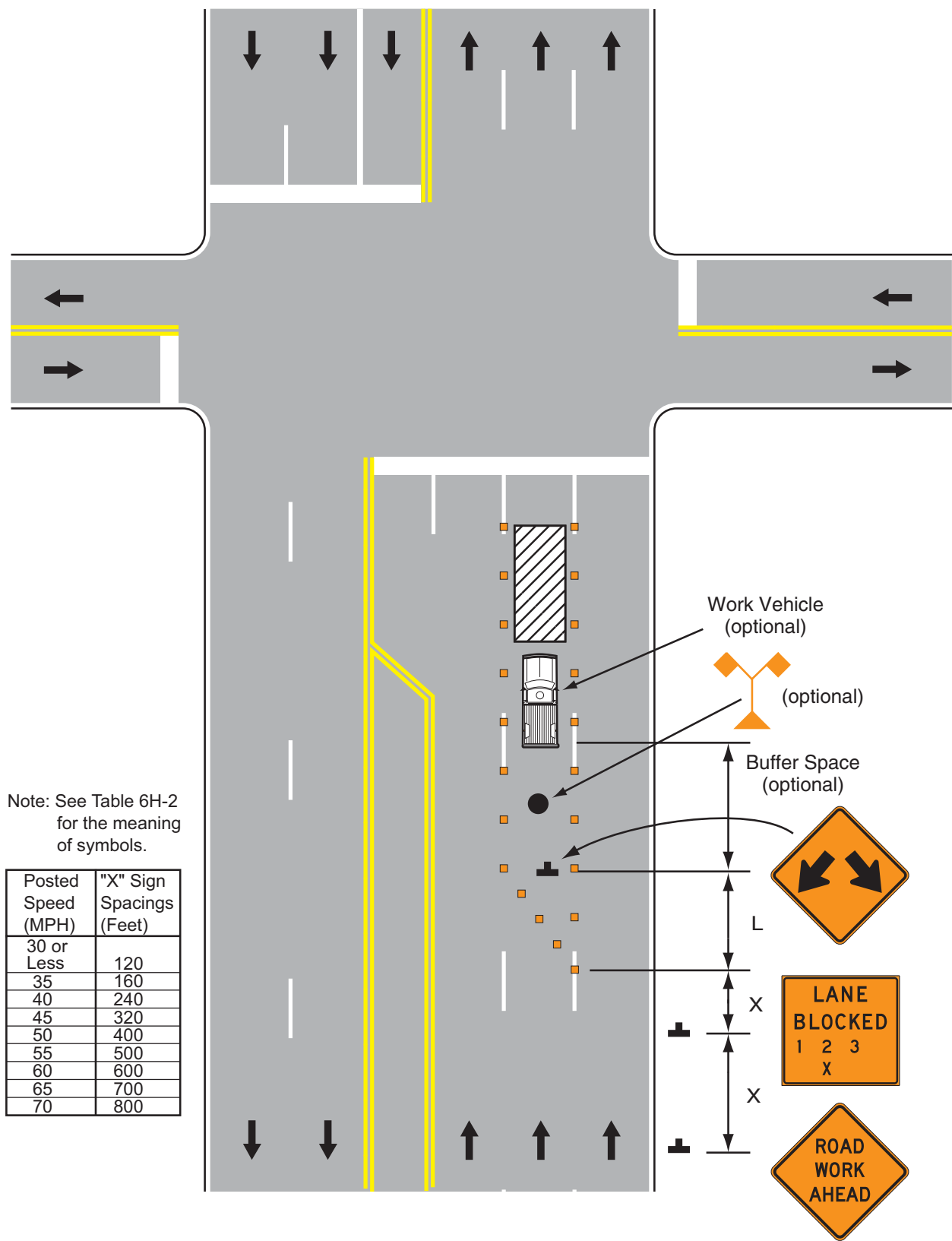
Typical Application 21
