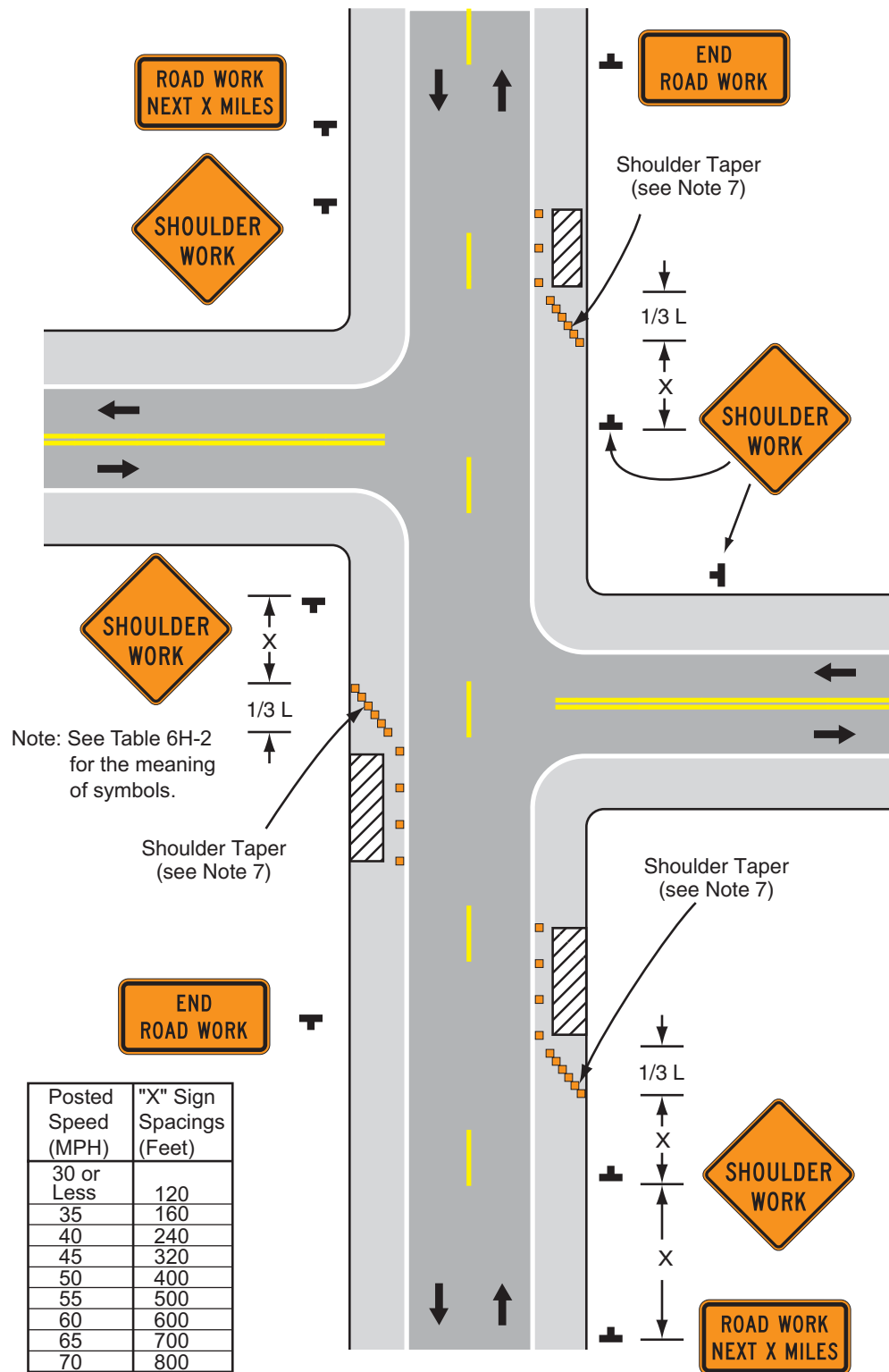
Typical Application 3
