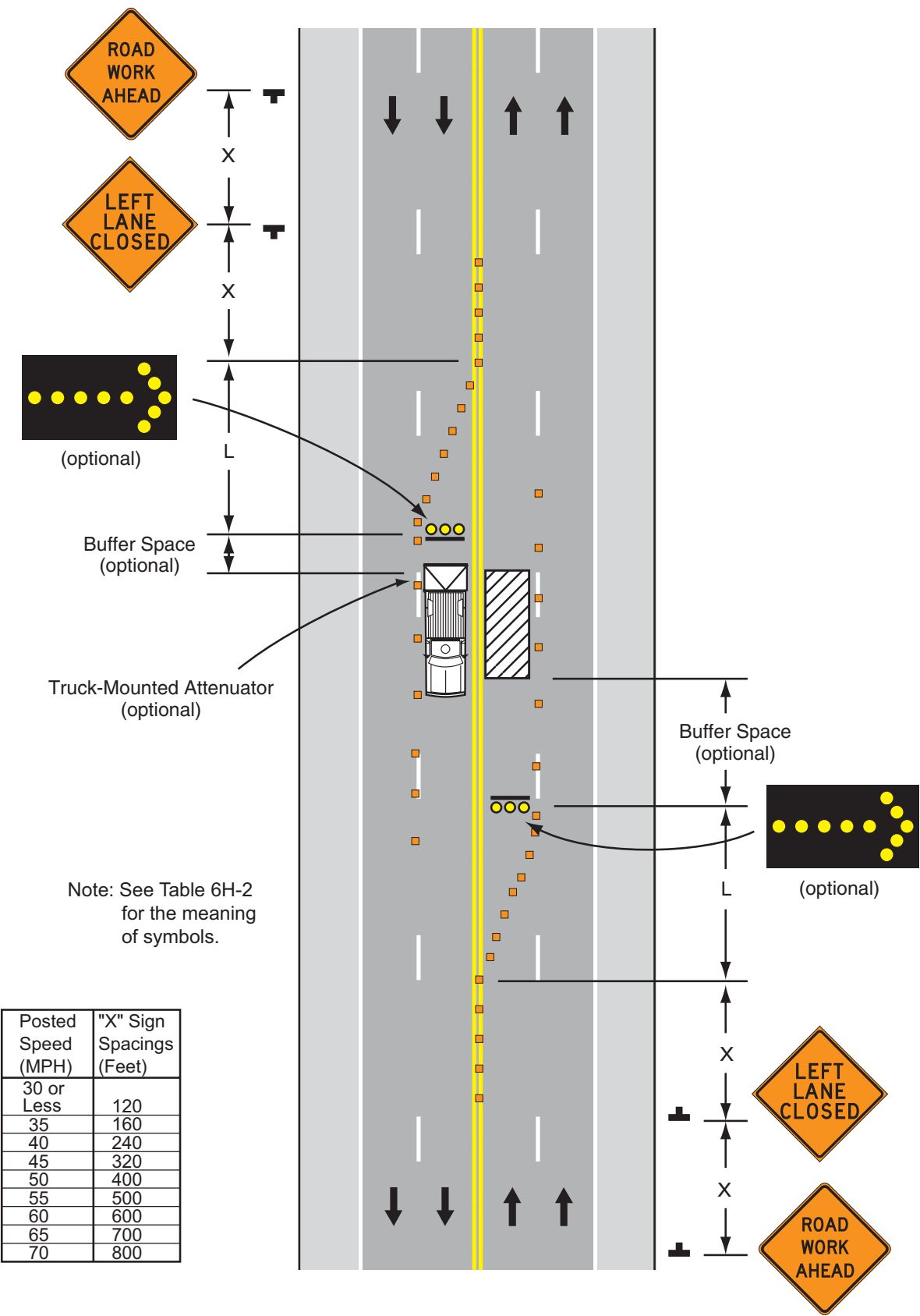
Typical Application 30
