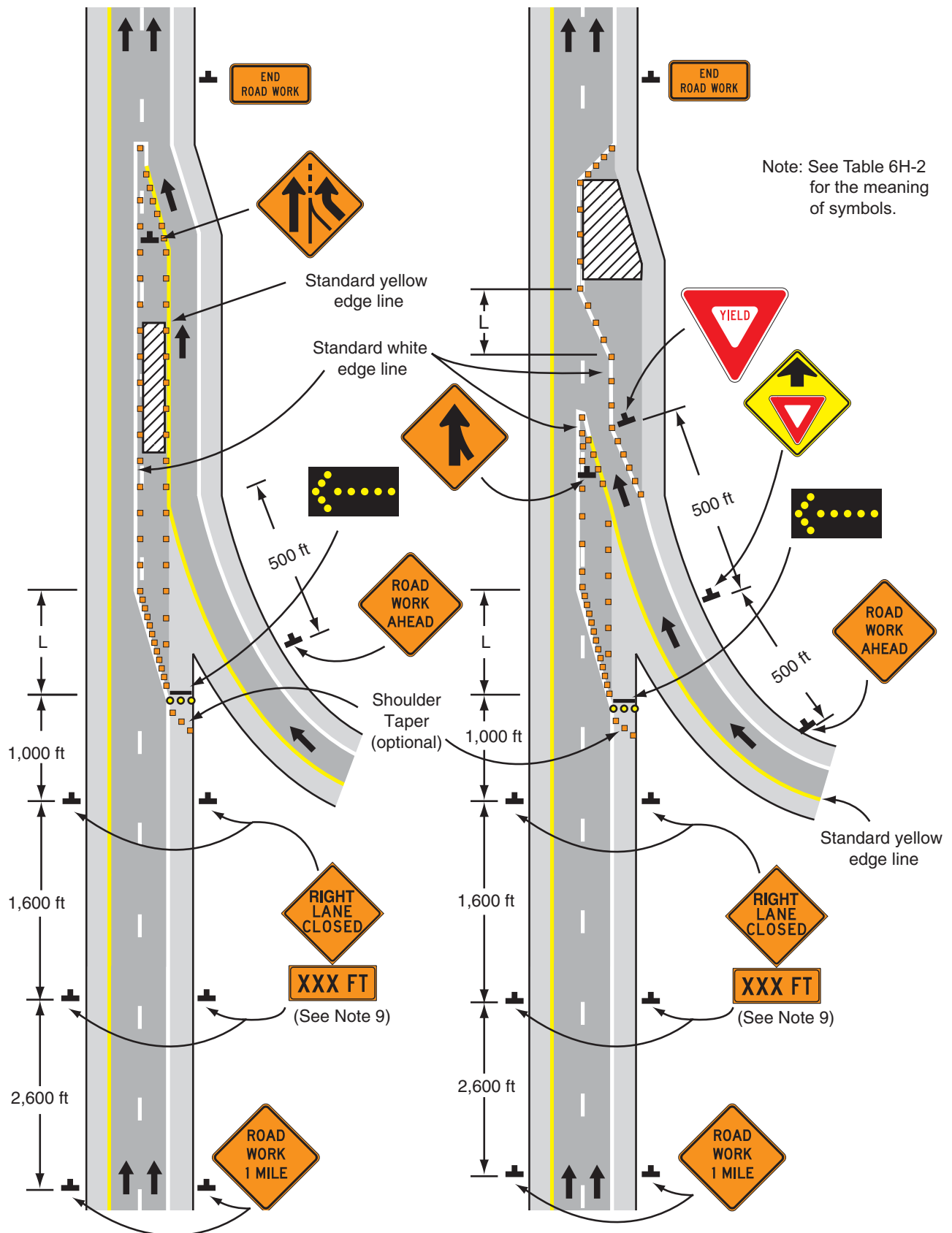
Figure 6H-44. Work in Vicinity of Entrance Ramp (TA-44)
