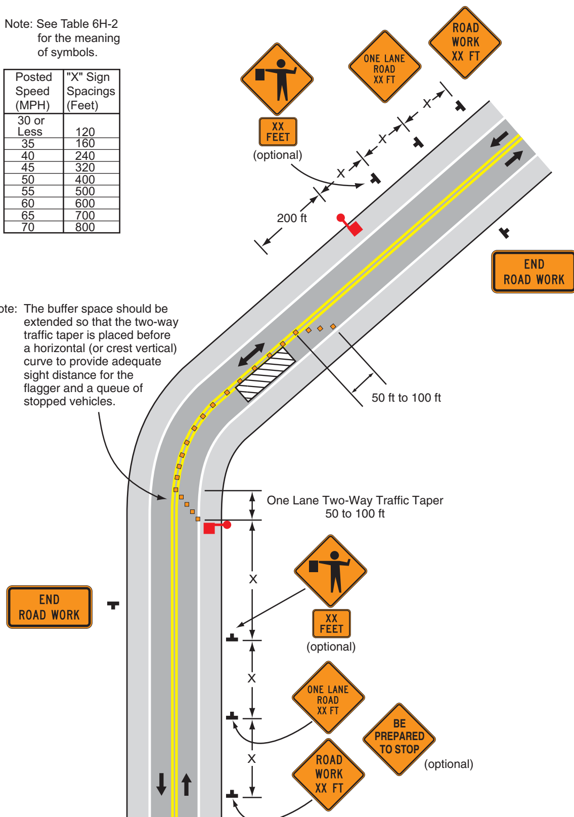
Typical Application 10
