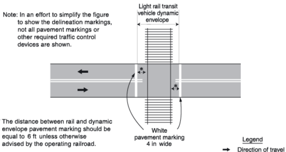
Figure 10C-2. Typical Light Rail Transit Vehicle Dynamic Envelope Delineation Pavement Markings
