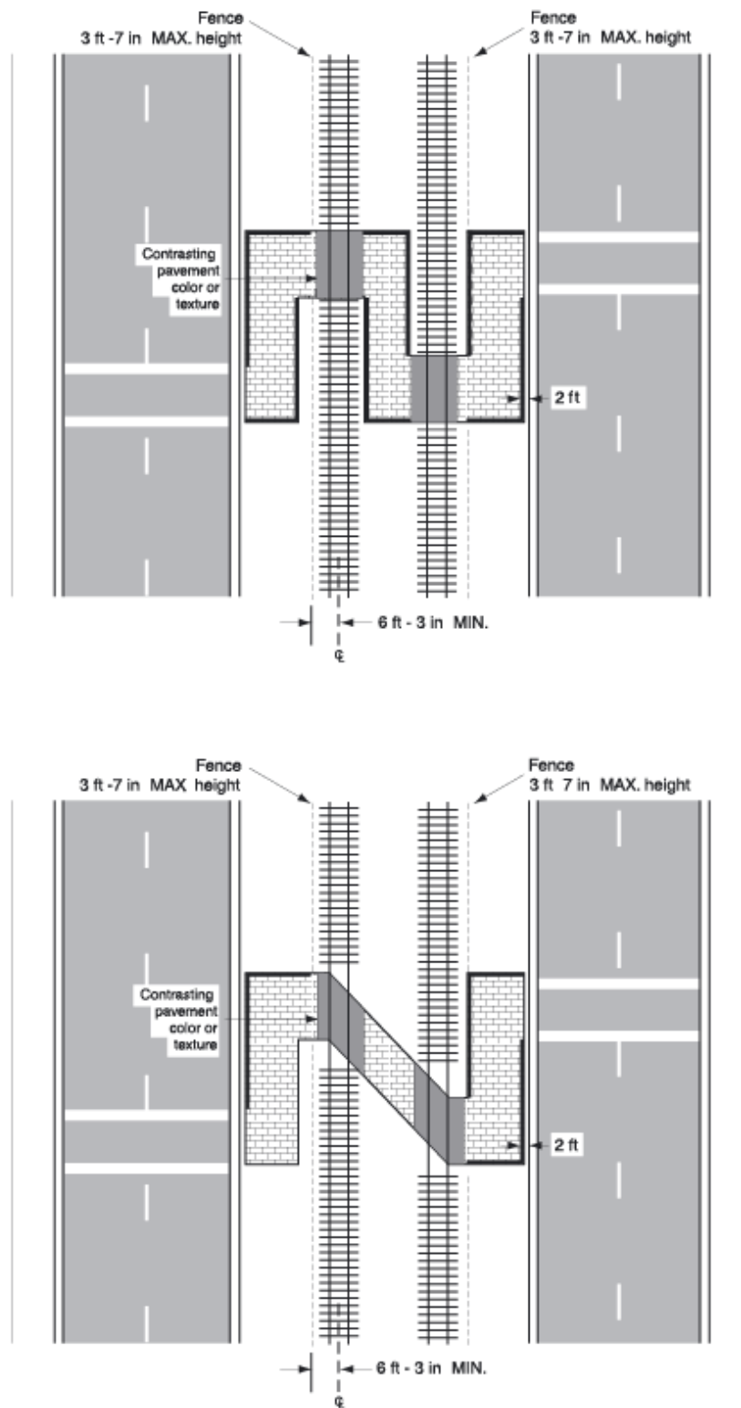
Figure 10D-8. Typical Examples of Pedestrian Barrier Installation at an Offset Nonintersection Light Rail Transit Crossing
