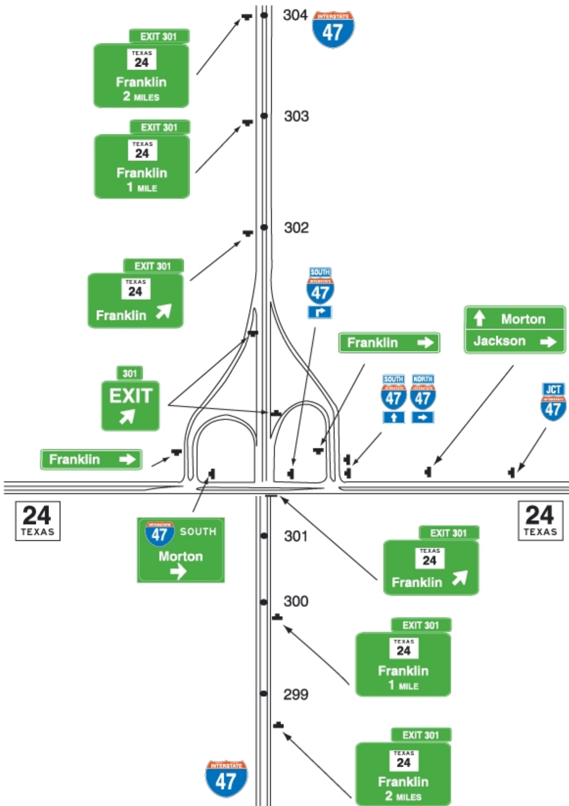
Figure 2E-27. Typical Partial Cloverleaf Interchange Guide Signs
