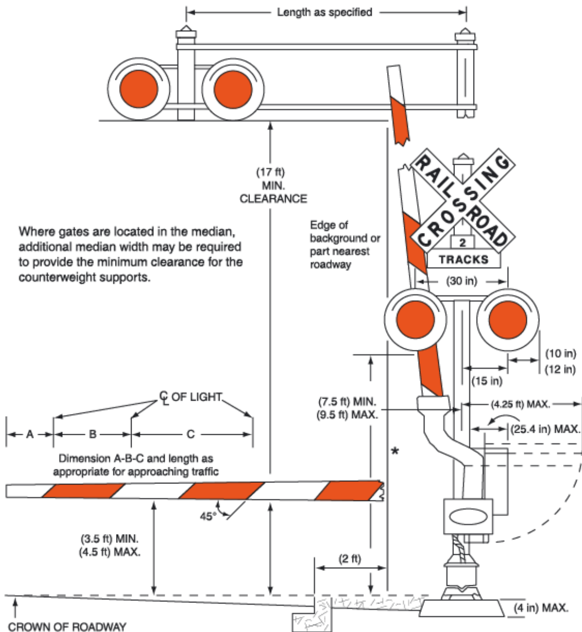
Figure 8D-1. Composite Drawing of Active Traffic Control Devices for Highway-Rail Grade Crossings Showing Clearances
