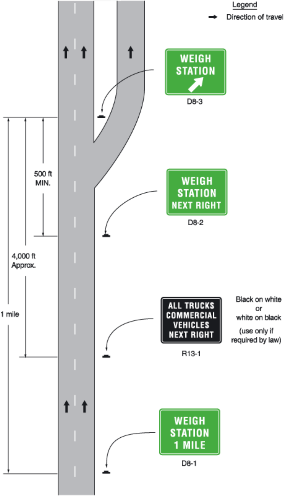
Figure 2D-3. Typical Weigh Station Signing
