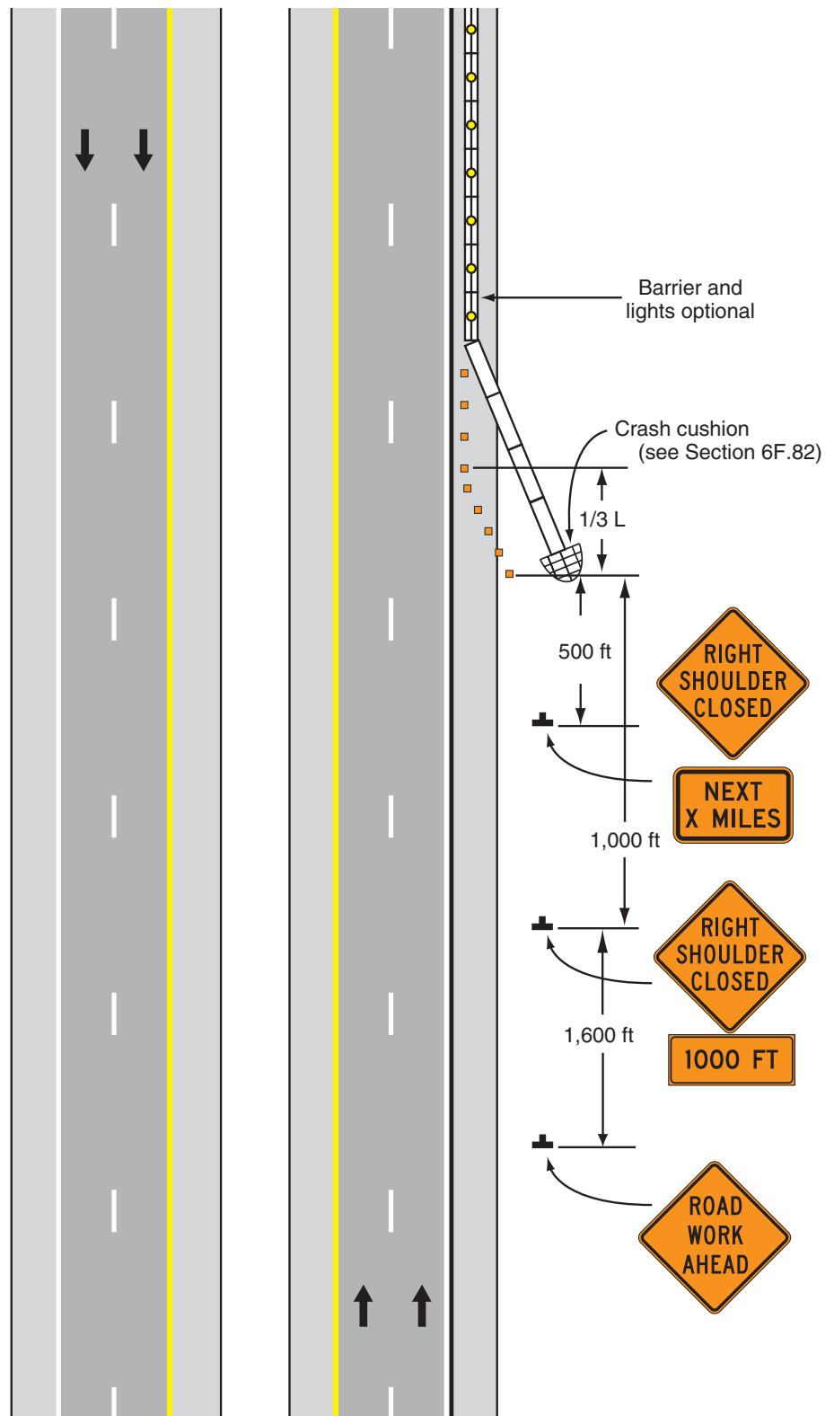
Typical Application 5
