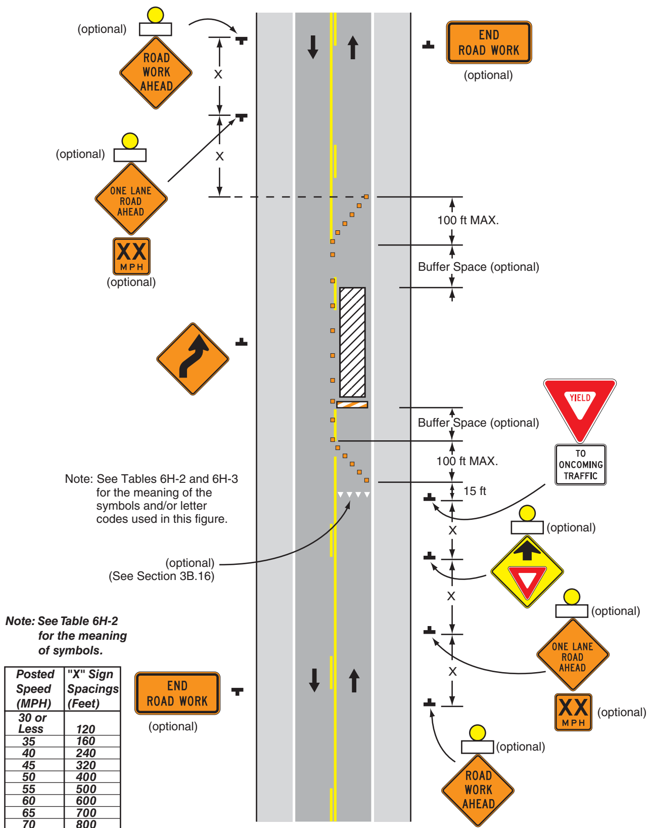
Typical Application 11
