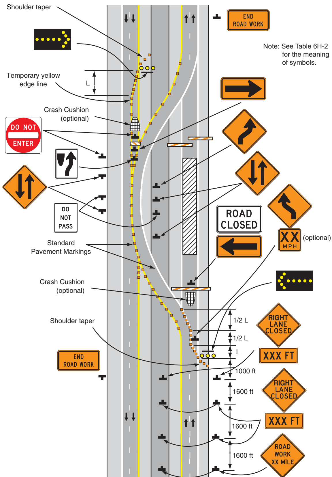
Typical Application 39
