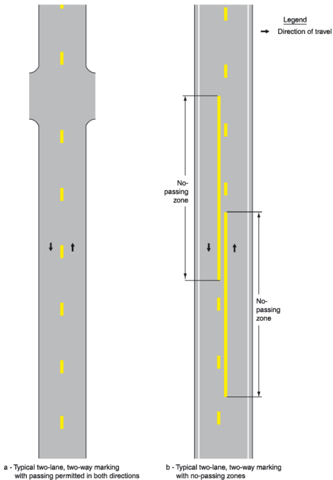
Figure 3B-1. Typical Two-Lane, Two-Way Marking Applications
