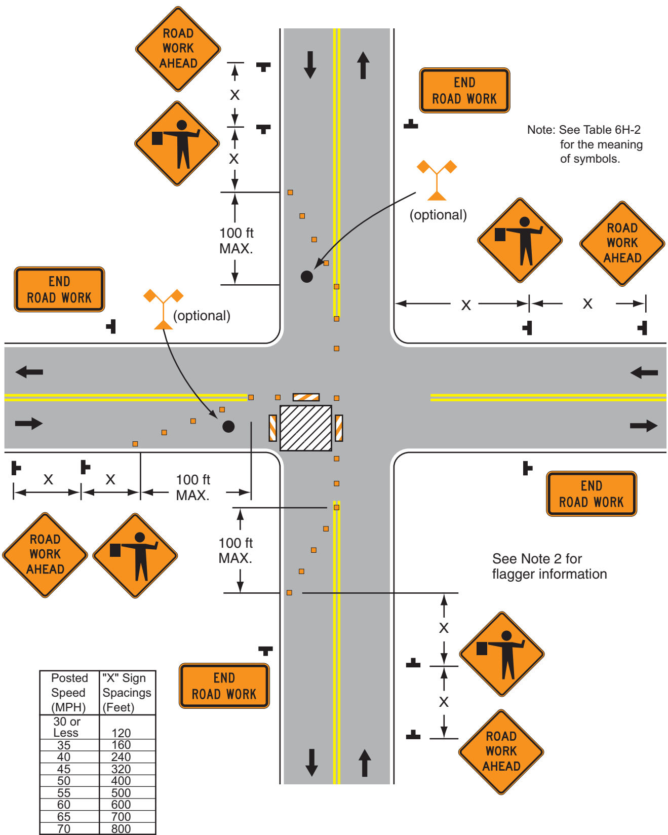
Typical Application 27
