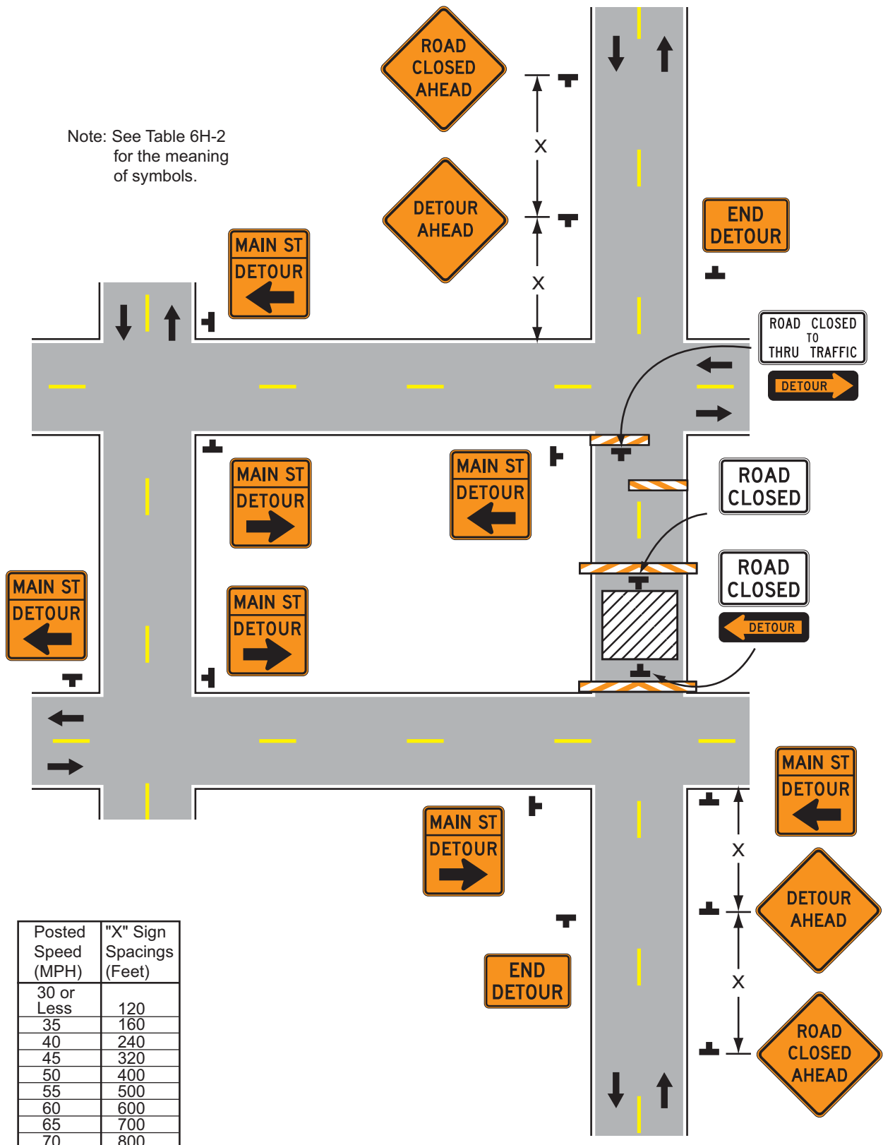
Typical Application 20
