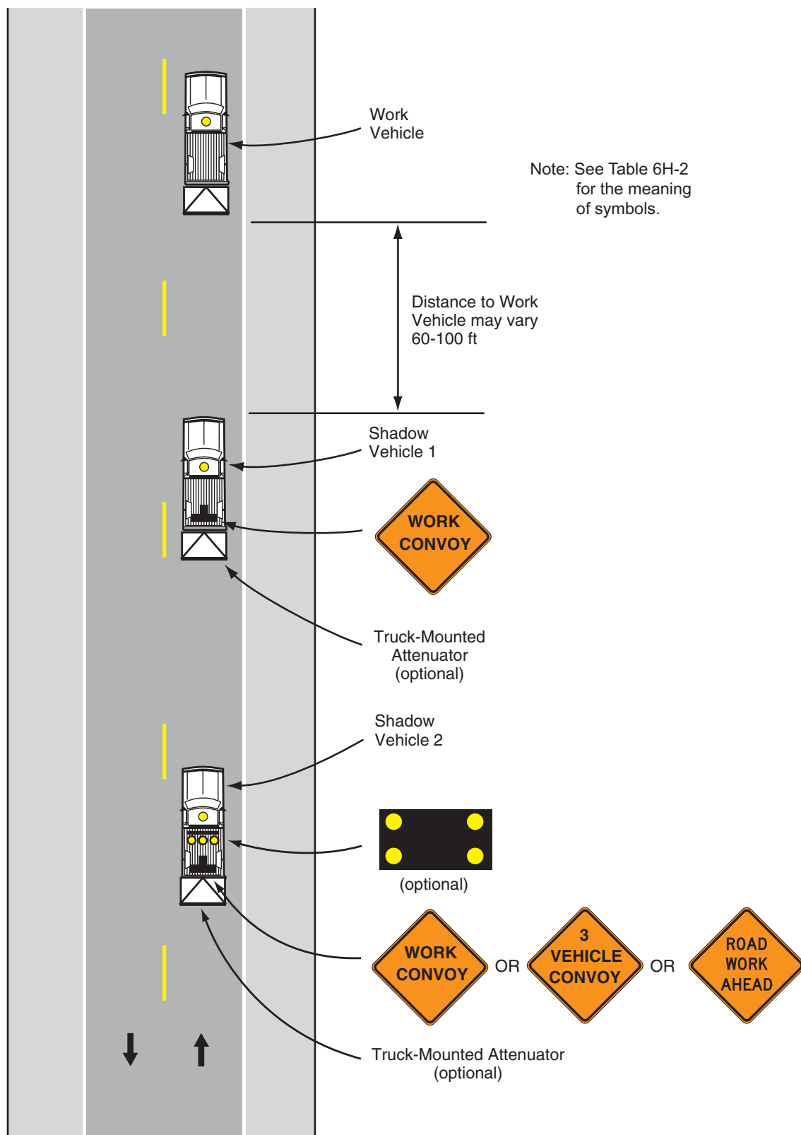
Typical Application 17
