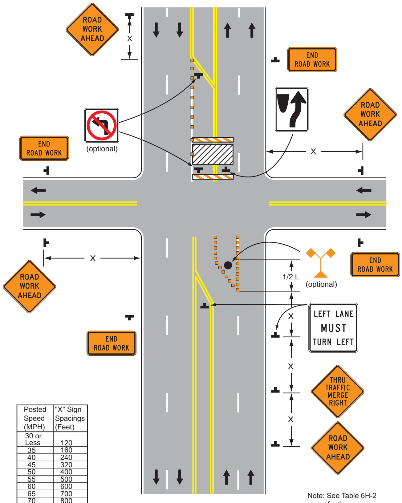
Typical Application 25
