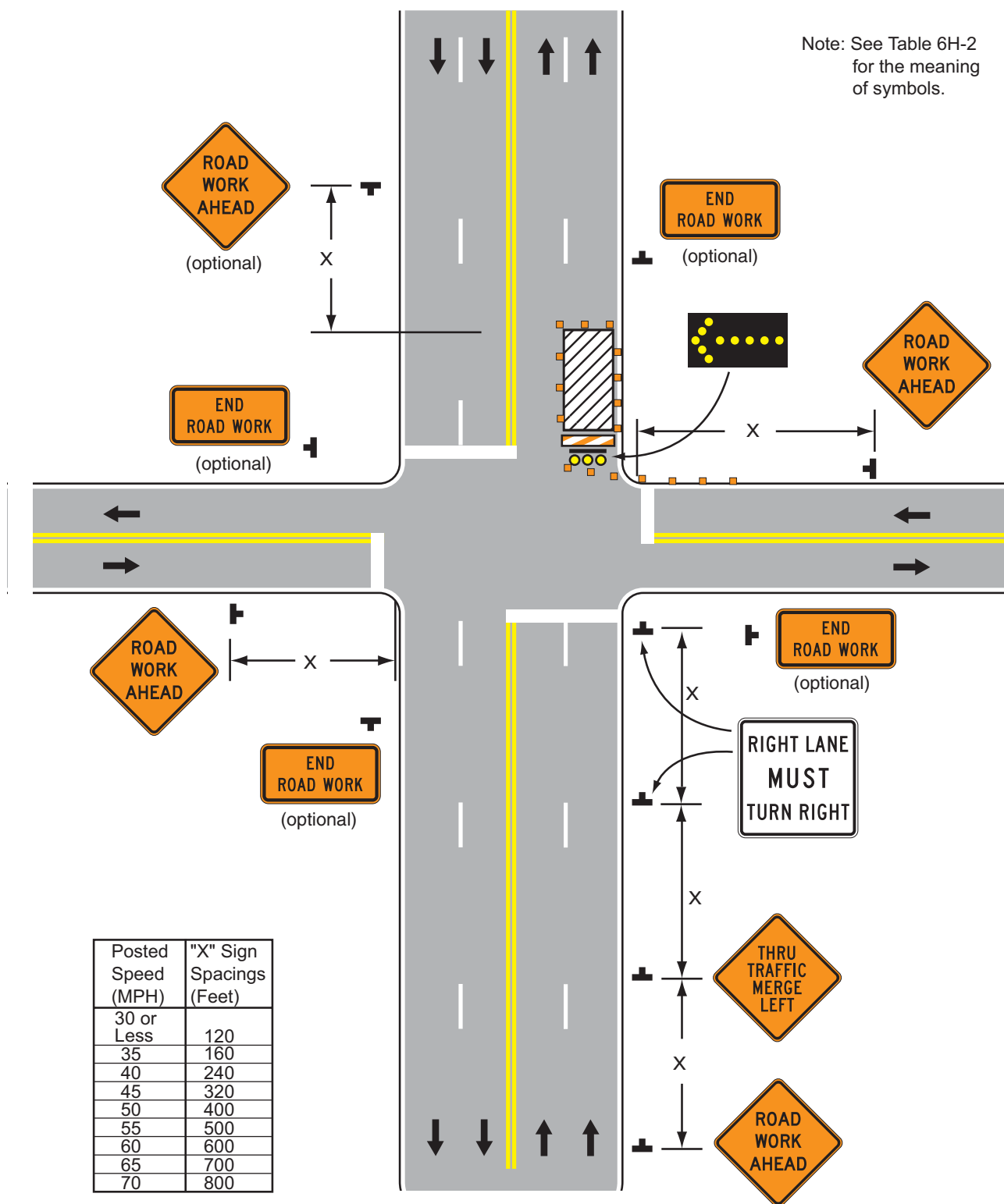
Typical Application 22
