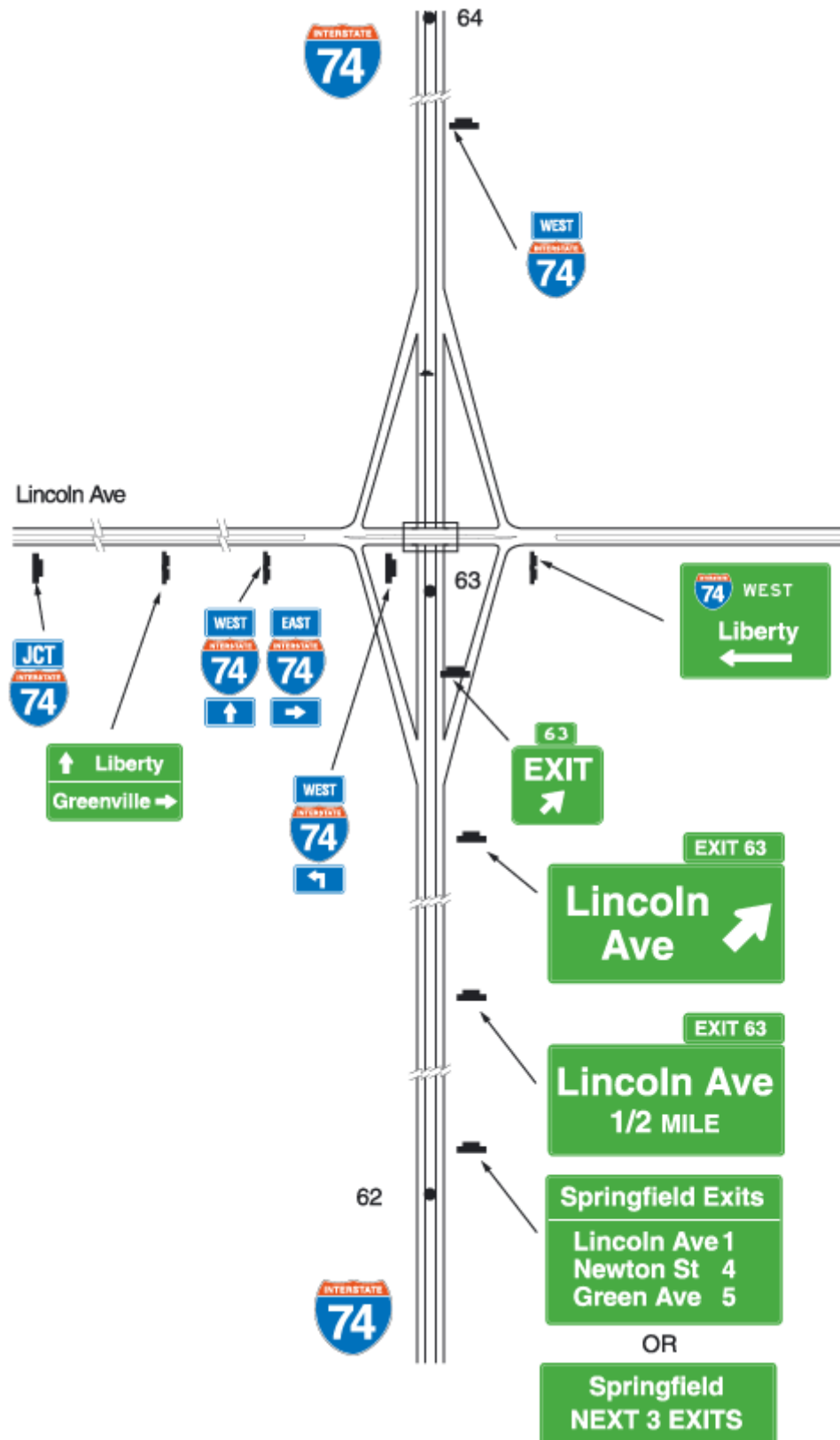
Figure 2E-29. Typical Urban Diamond Interchange Guide Signs
