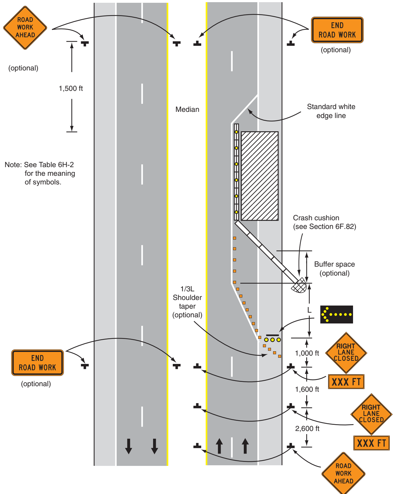
Typical Application 34
