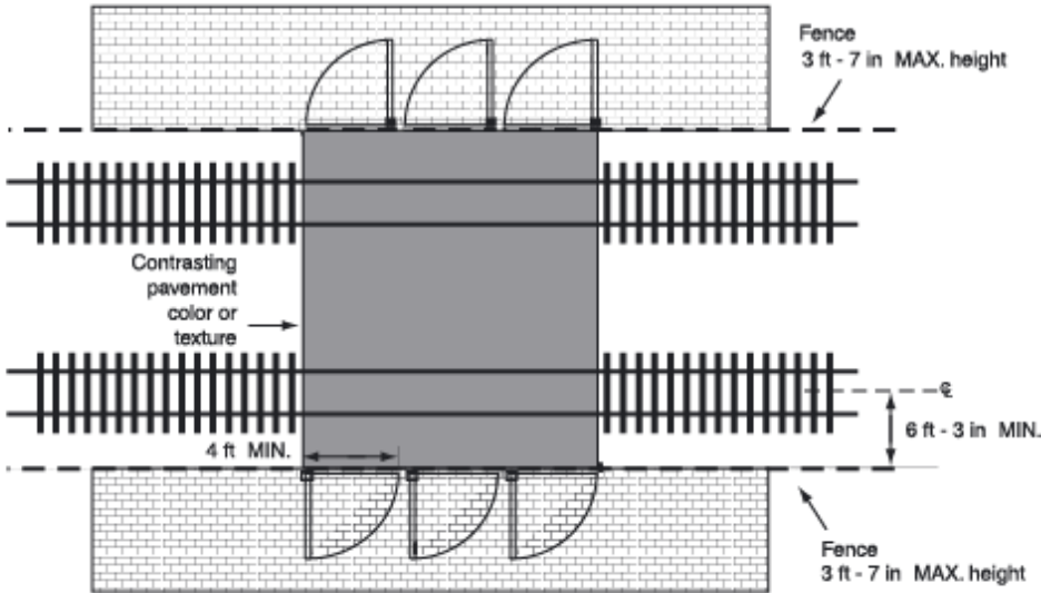
Figure 10D-6. Typical Swing Gates
