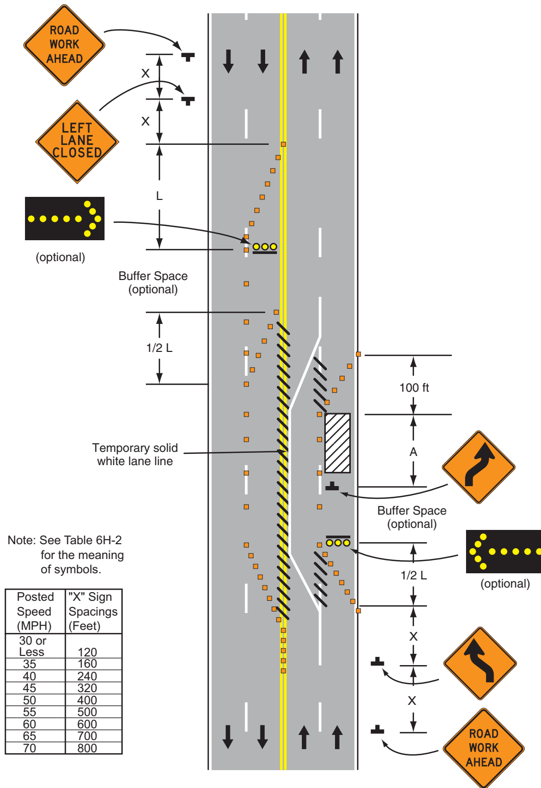
Typical Application 31
