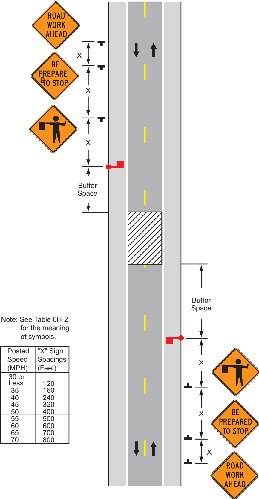
Typical Application 13
