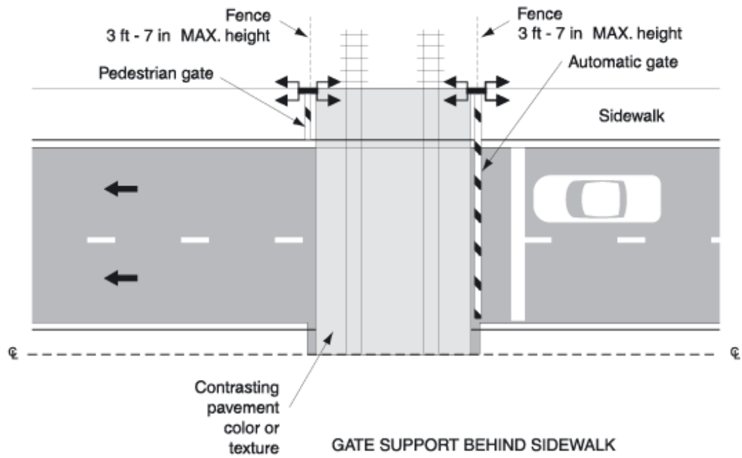
Figure 10D-5. Typical Placement of Pedestrian Traffic Gates
