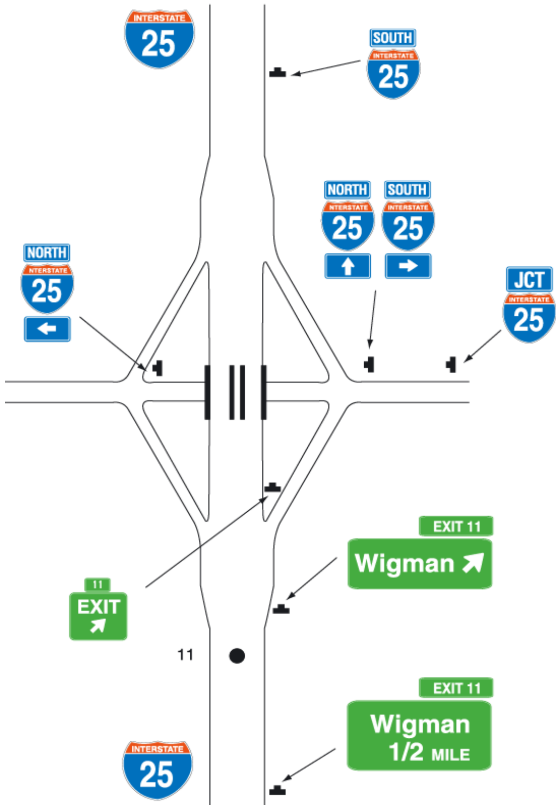
Figure 2E-30. Typical Minor Interchange Guide Signs
