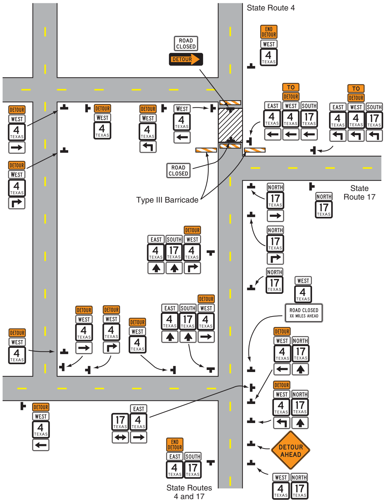
Figure 6H-9. Overlapping Routes with Detour (TA-9)
