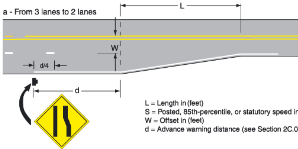
Figure 3B-12. Typical Lane Reduction Transition Markings
