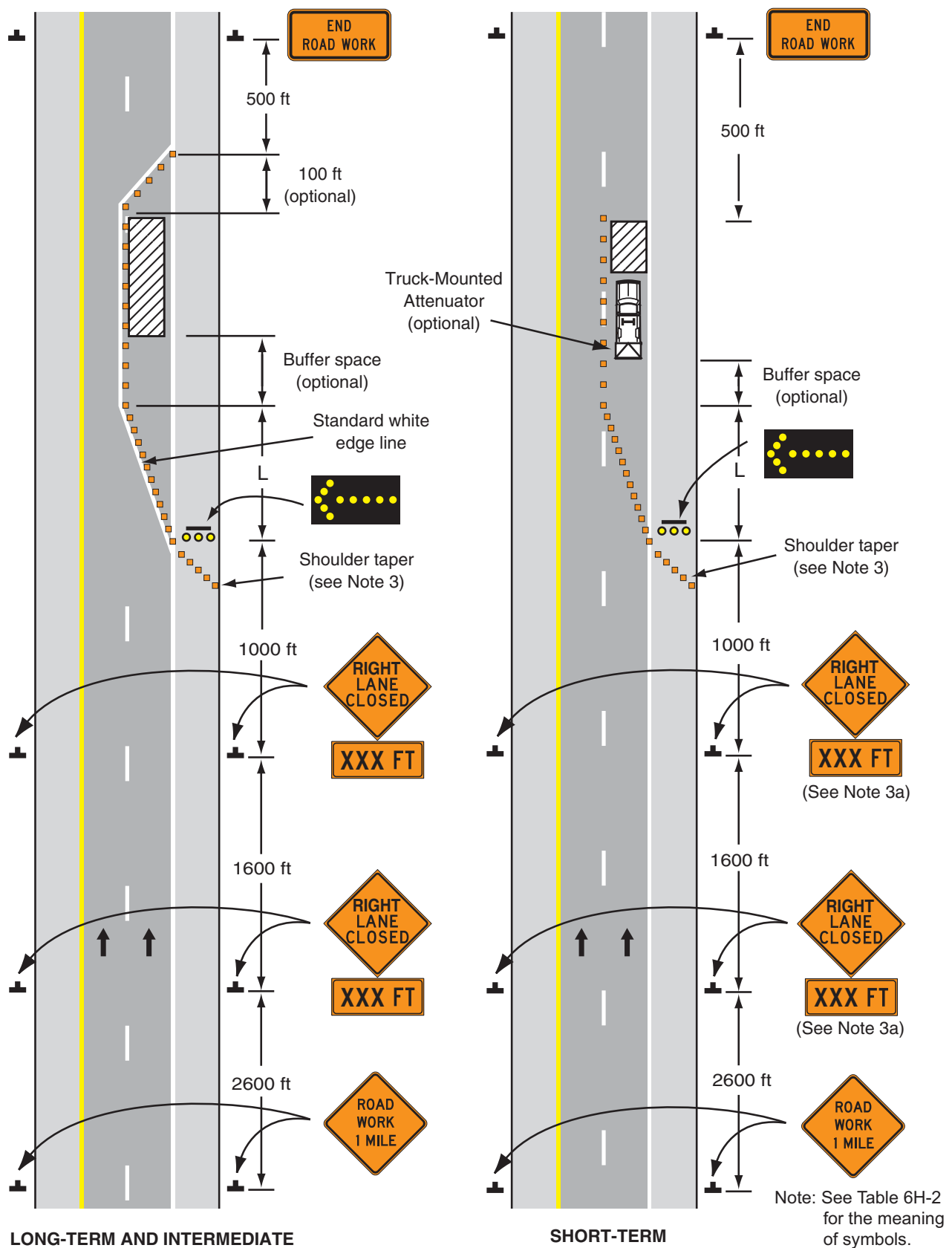
Typical Application 33
