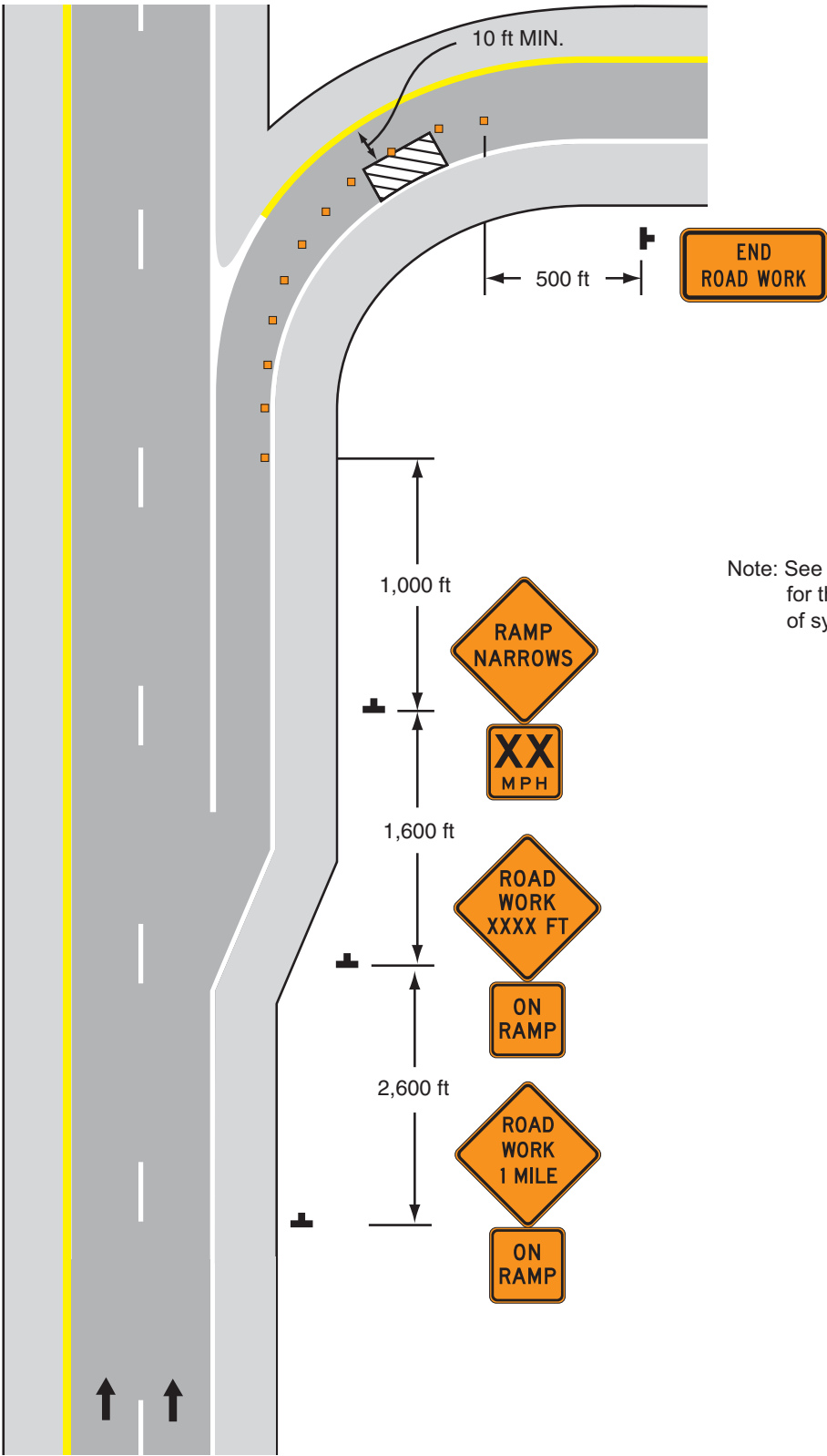
Typical Application 43
