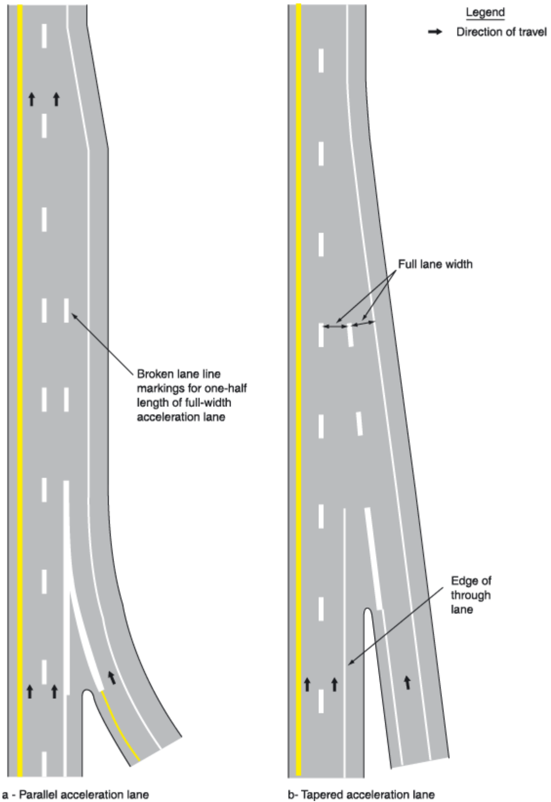
Figure 3B-9. Typical Entrance Ramp Markings
