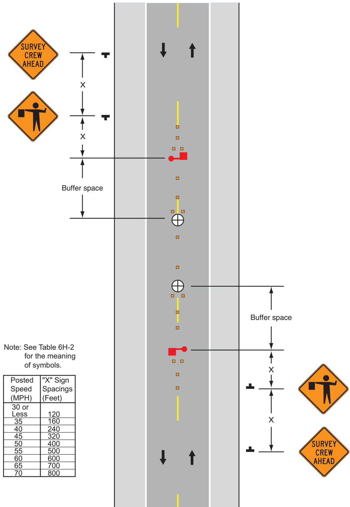
Typical Application 16
