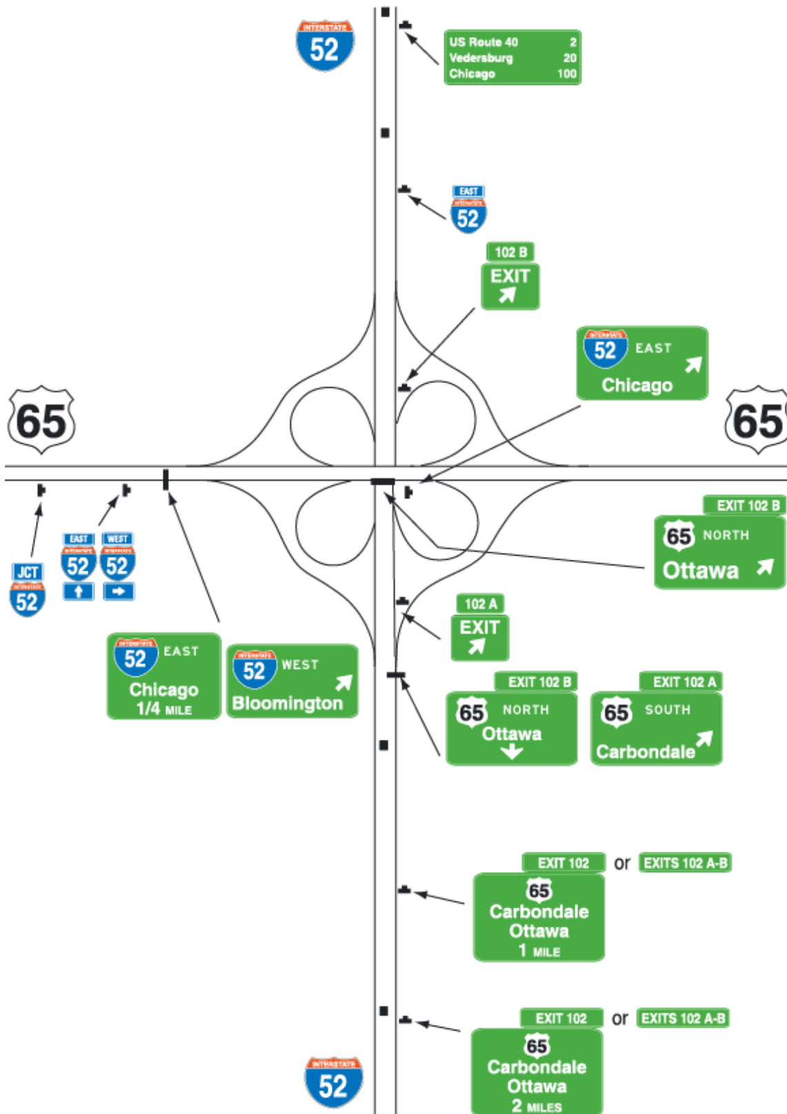
Figure 2E-26. Typical Guide Signs for Full Cloverleaf Interchange
