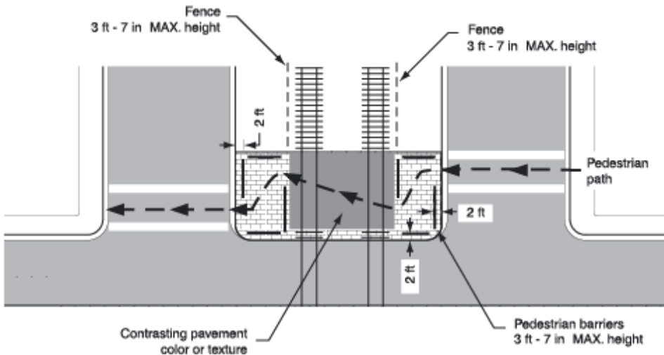
Figure 10D-7. Typical Pedestrian Barriers at an Offset Highway-Light Rail Transit Crossing
