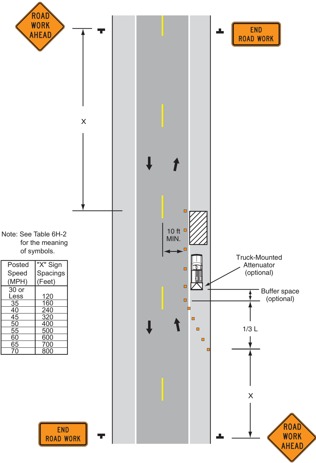
Typical Application 6
