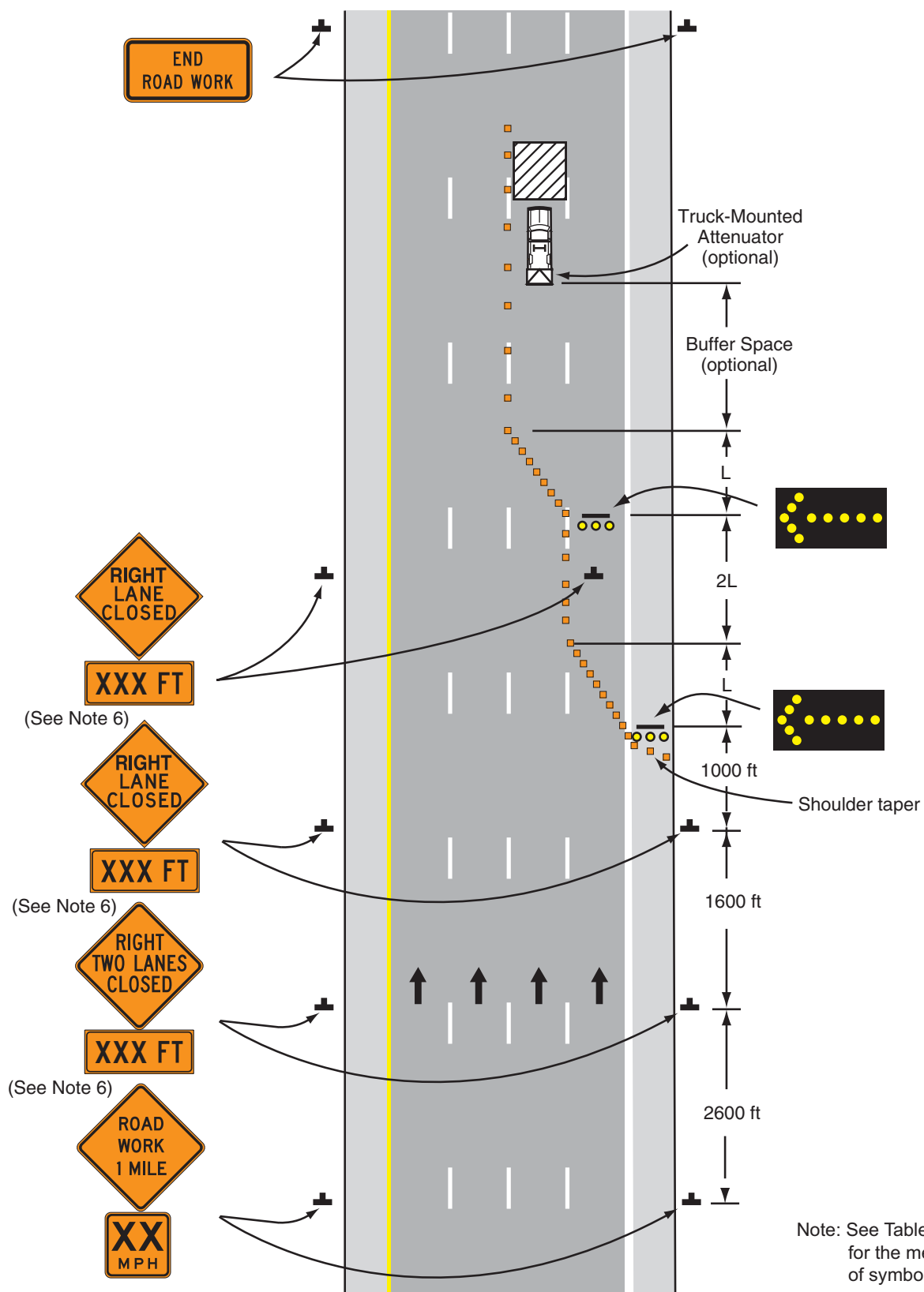
Typical Application 37
