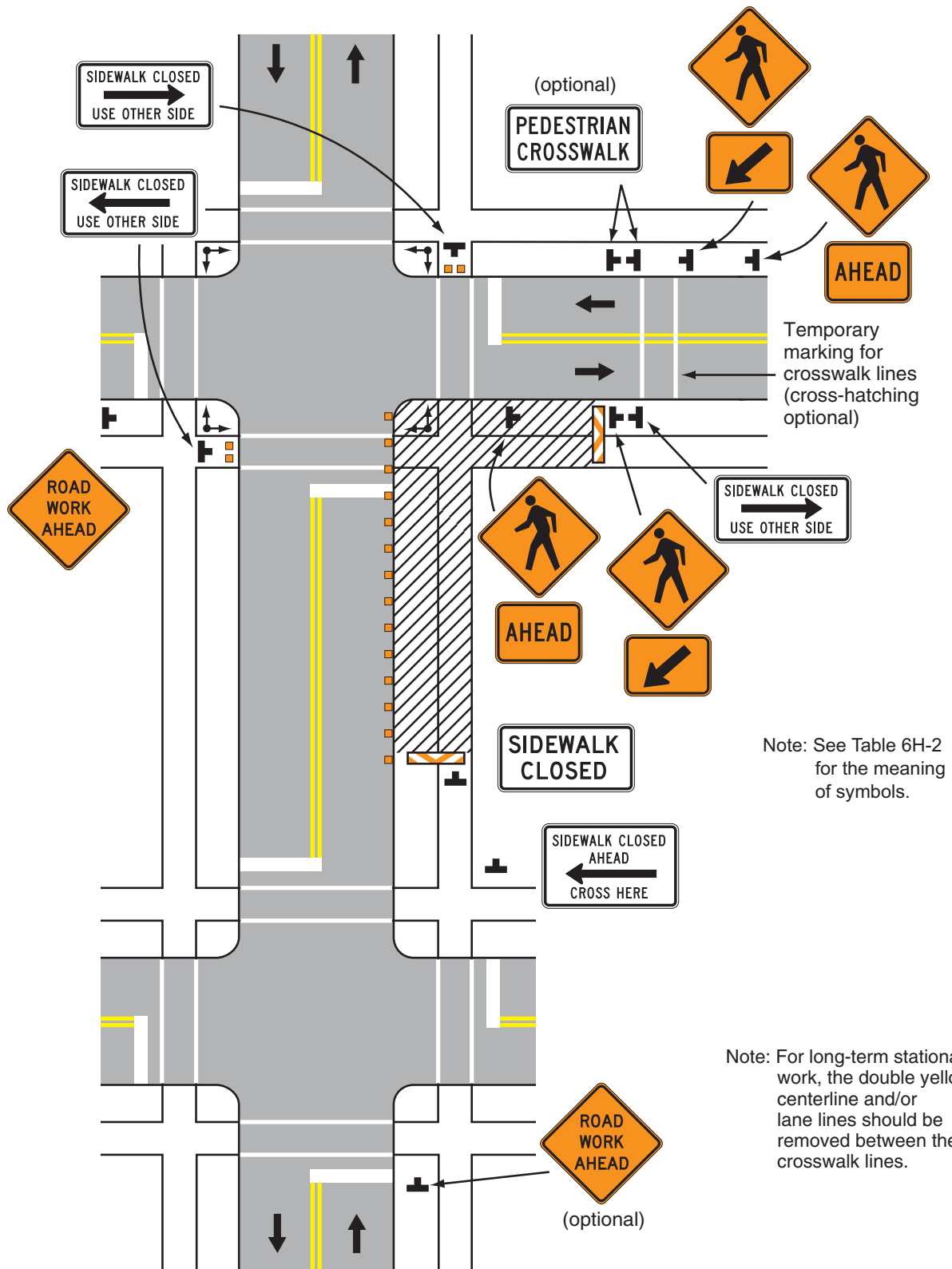
Figure 6H-29. Crosswalk Closures and Pedestrian Detours (TA-29)
