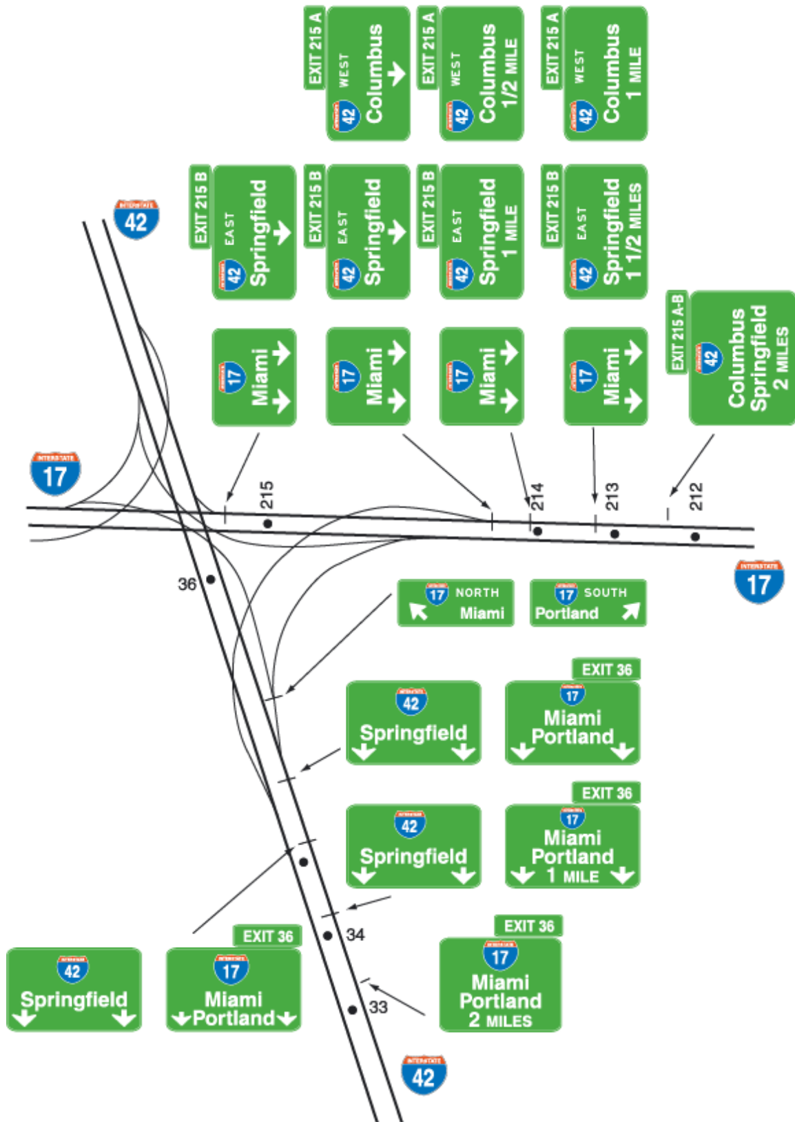
Figure 2E-25. Typical Freeway-to-Freeway Interchange Guide Signs
