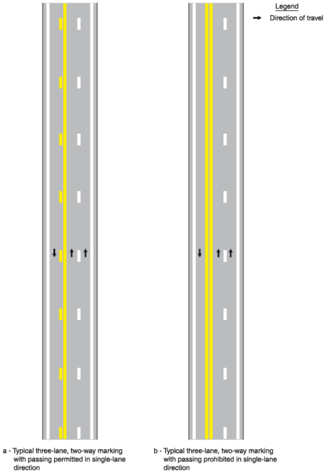
Figure 3B-3. Typical Three-Lane, Two-Way Marking Applications
