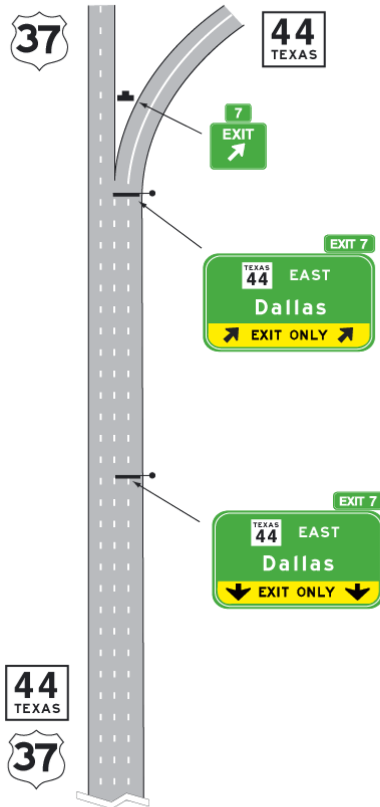
Figure 2E-9a. Two Lane EXIT ONLY Panels for Two Lanes Dropped at an Interchange
