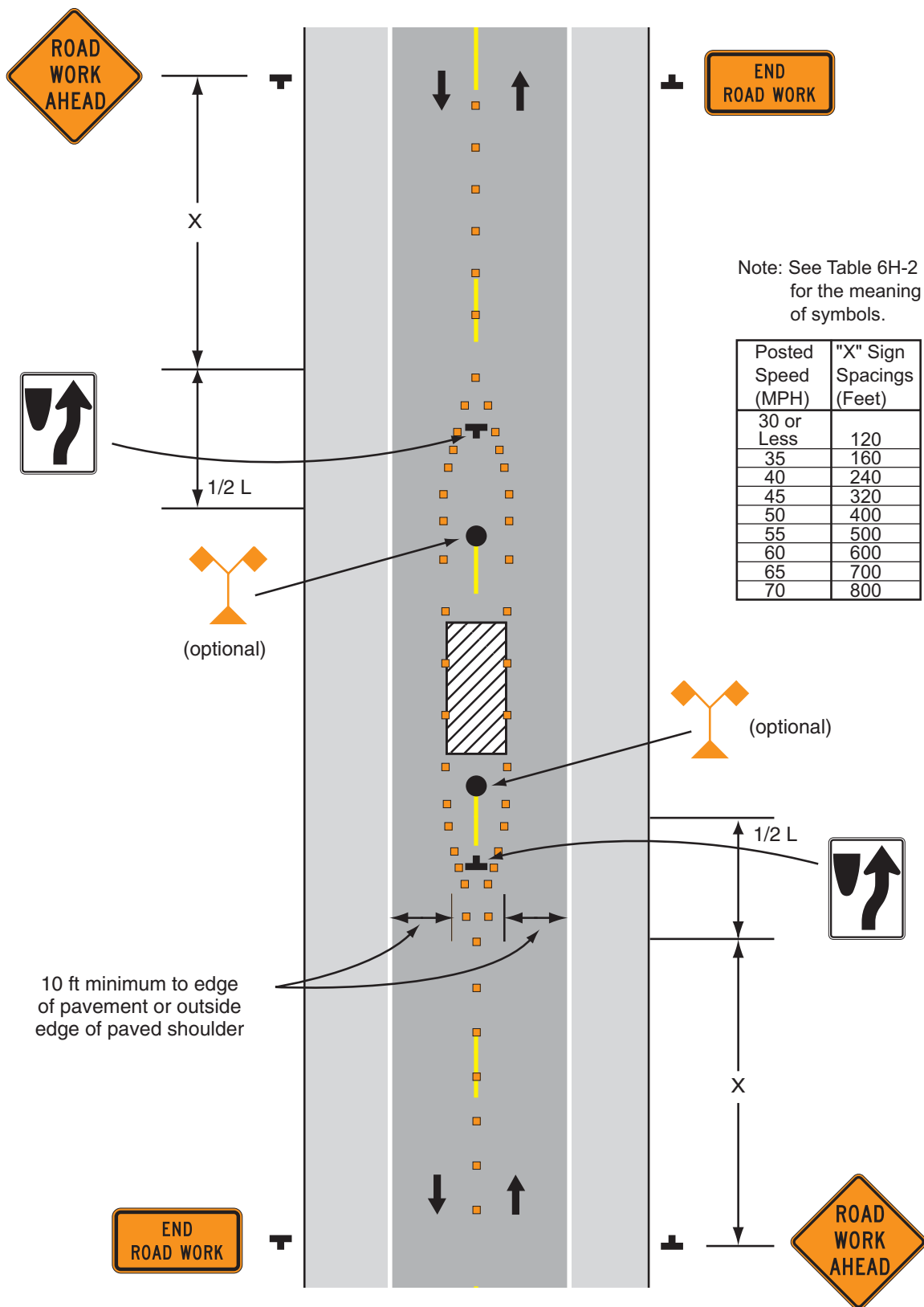
Typical Application 15
