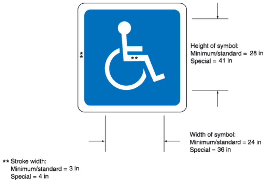
Figure 3B-18. International Symbol of Accessibility Parking Space Marking with Blue Background and White Border Options
