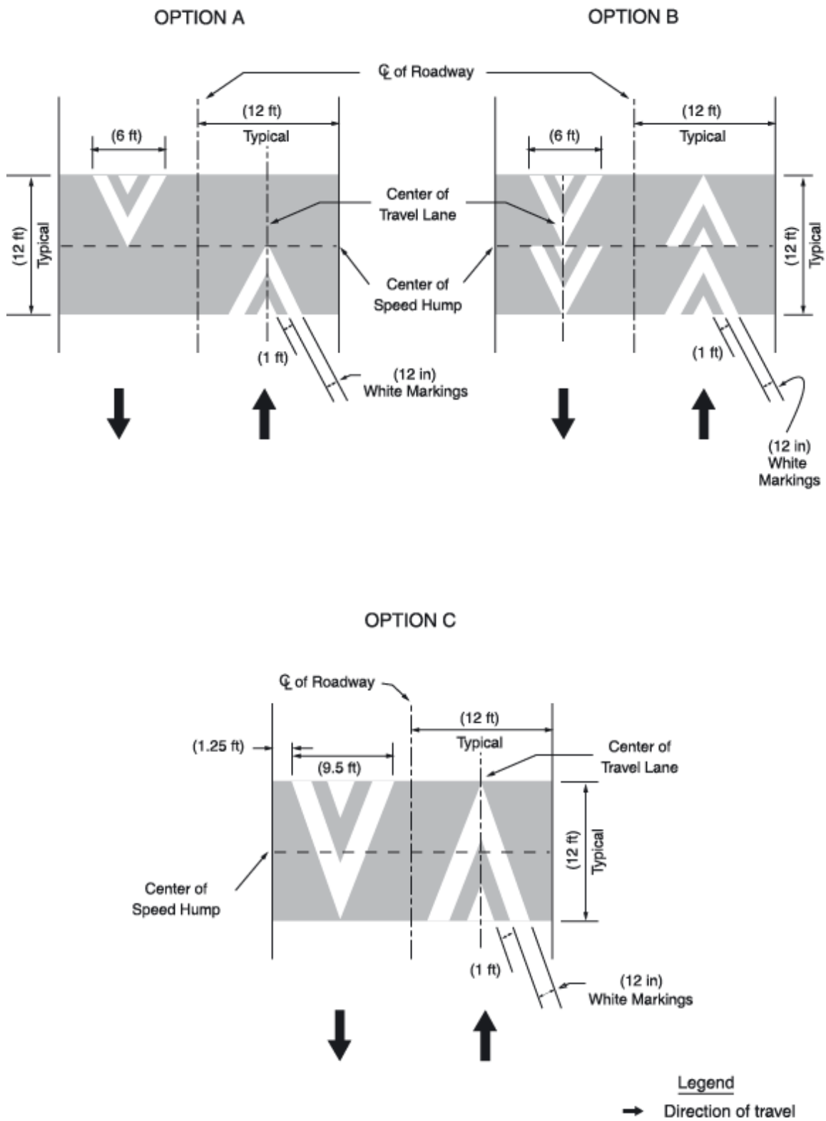
Figure 3B-28. Typical Pavement Markings for Speed Humps
