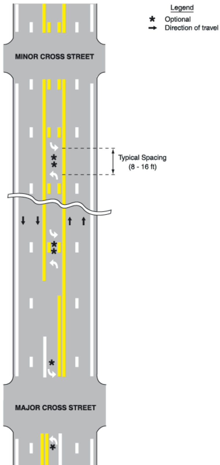
Figure 3B-7. Typical Two-Way Left-Turn Lane Marking Applications
