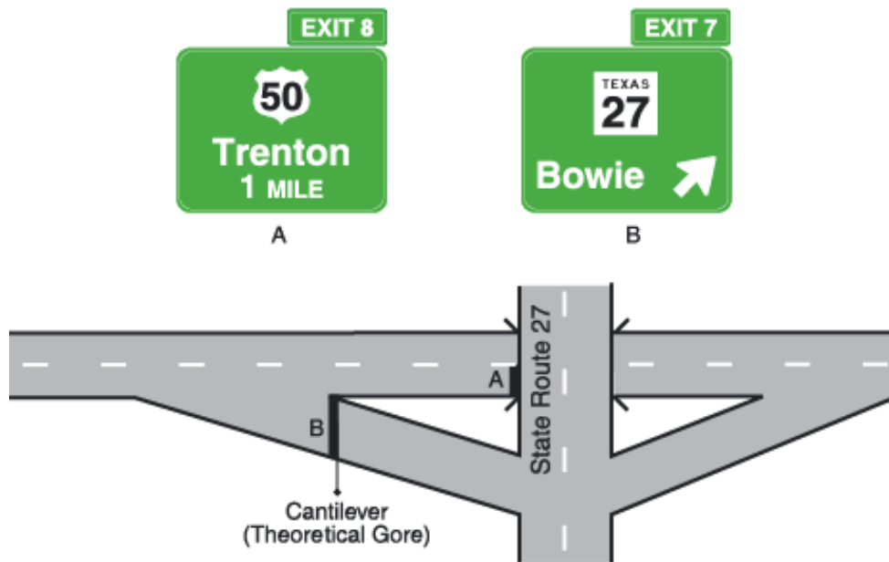
Figure 2E-1. Example of Guide Sign Spreading
