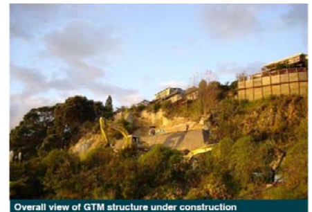
Overall view of GTM structure under construction
