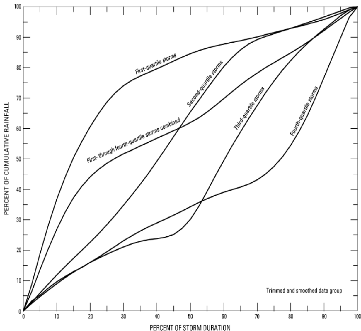
Dimensionless hyetograph curves for 50th percentile for a storm duration of 0-72 hours and a rainfall total of 1 inch or more.
