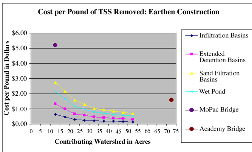
Figure 2. Earthen construction
