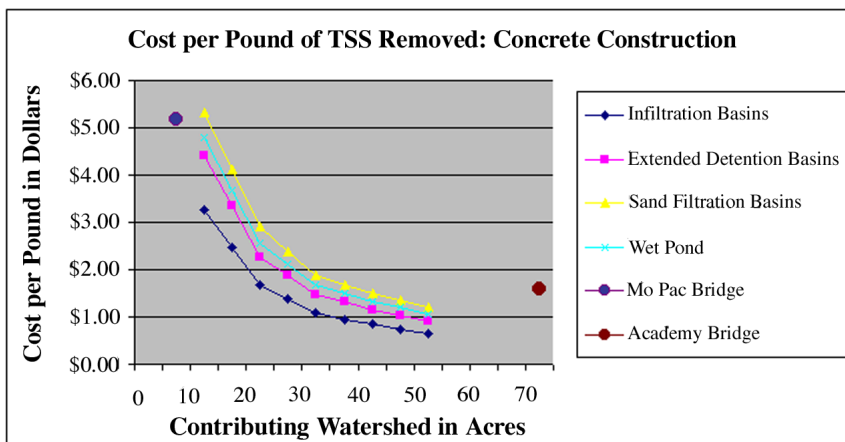
Figure 3. Concrete construction
