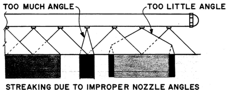
Figure 7-18. Effect of Incorrect Nozzle Angle.
