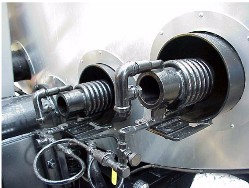
Figure 7-7. Burner Configuration at Rear of Tank.
