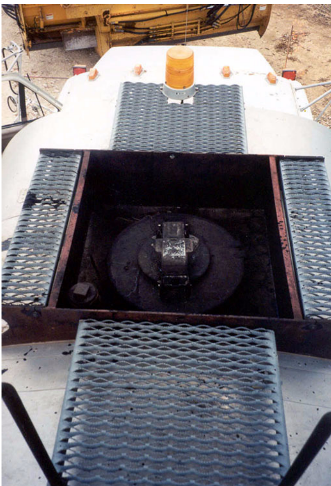
Figure 7-6. Manhole Cover on Top of Distributor Tank.
