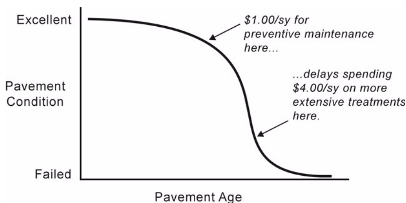
Figure 2-1. The Concept of Preventive Maintenance. (After Applied Pavement Technology, Inc., 1999)
