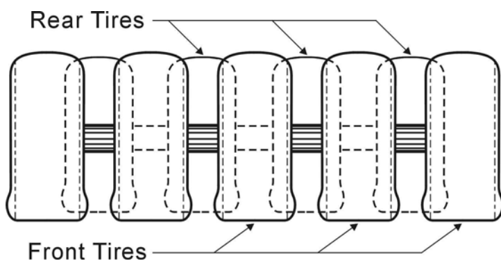
Figure 7-46. Wheel Configuration on Pneumatic Rollers.
