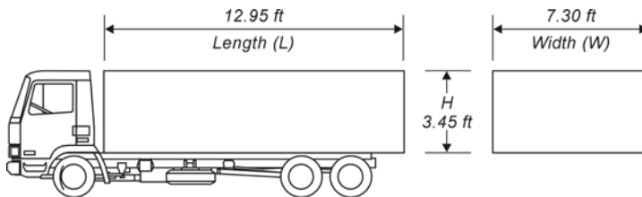
Figure 7-42. Volume of Truck Bed
