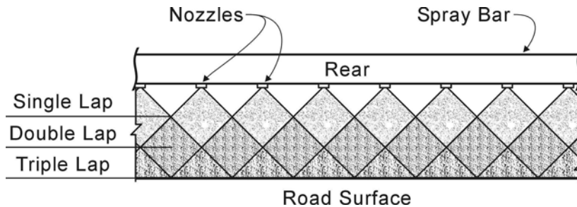
Figure 7-19. Various Asphalt Spray Patterns.
