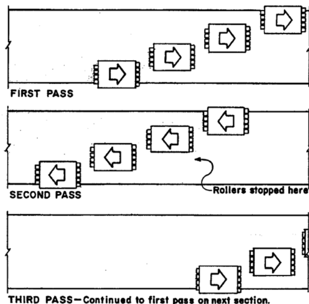
Figure 8-8. Illustration of Echelon Rolling Pattern.
