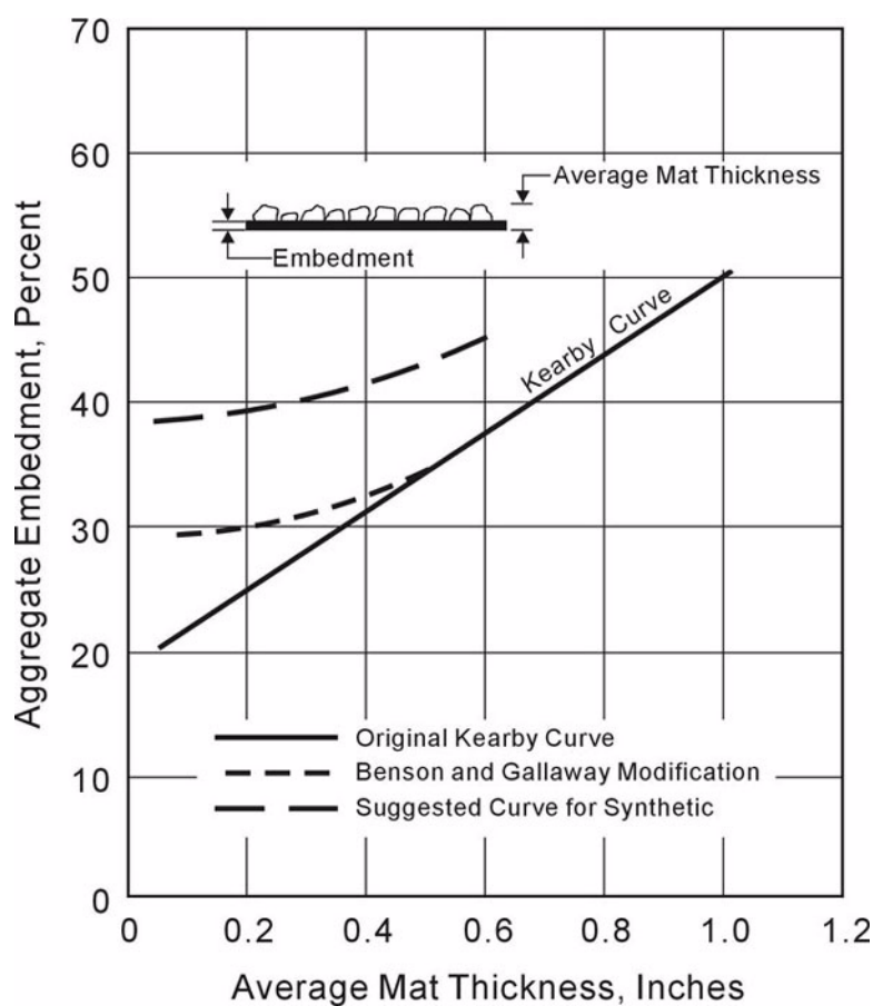
Figure 4-1. Relation of Percent Embedment to Mat Thickness for Determining Quantity of Asphalt. (After Epps et al., 1981)
