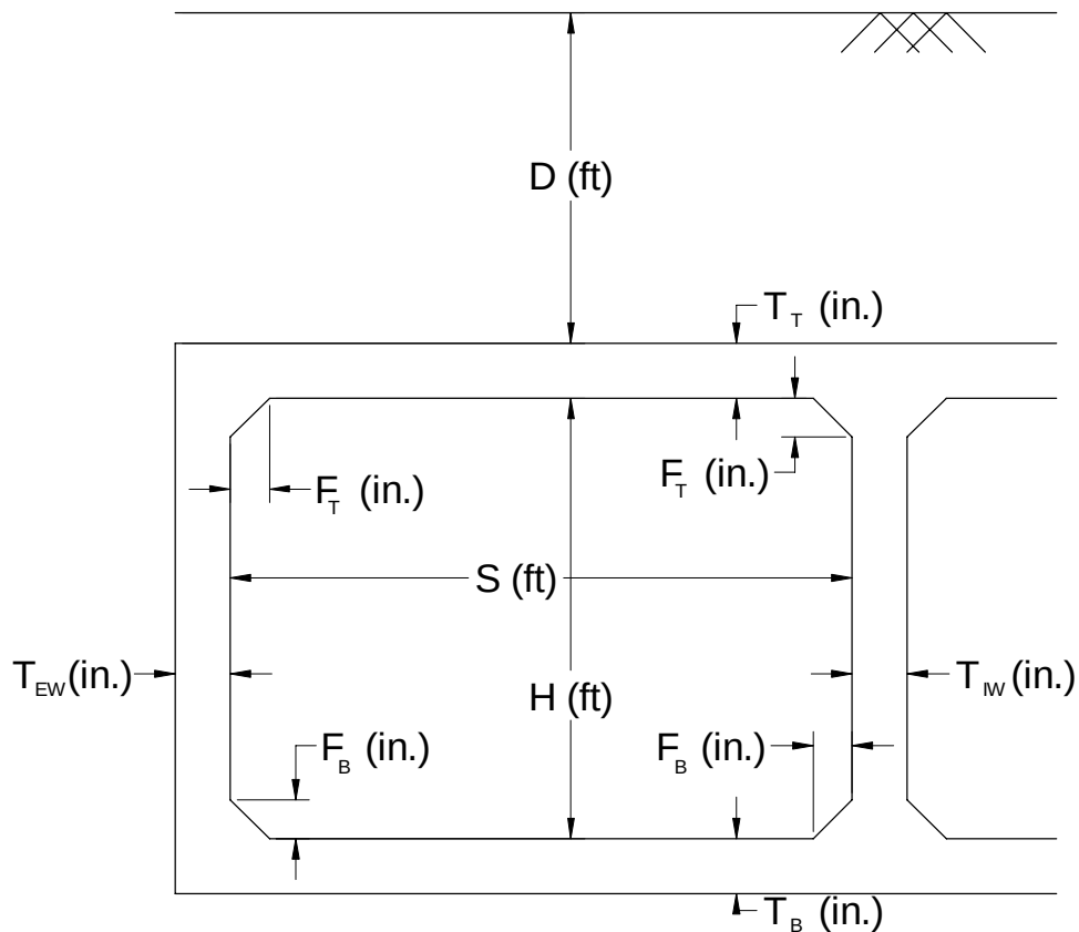
FIGURE IV.1. CULVERT DIMENSIONS.
