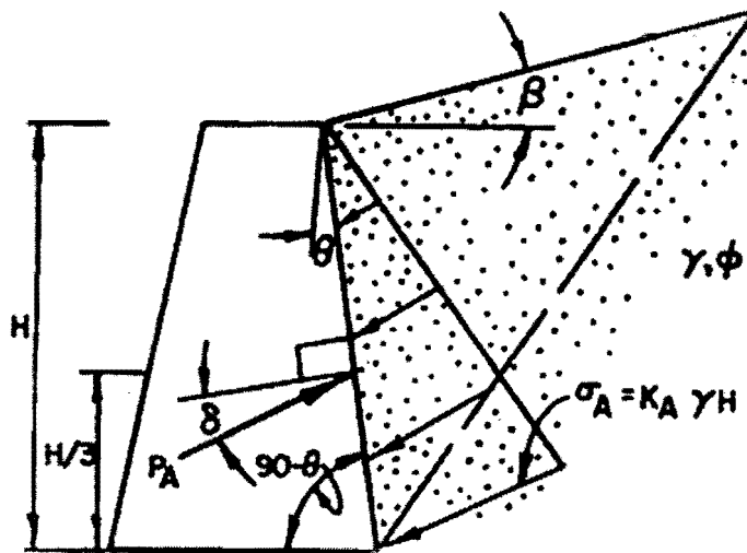
Figure 3.7: Coulomb's Active Earth Pressure (22)
