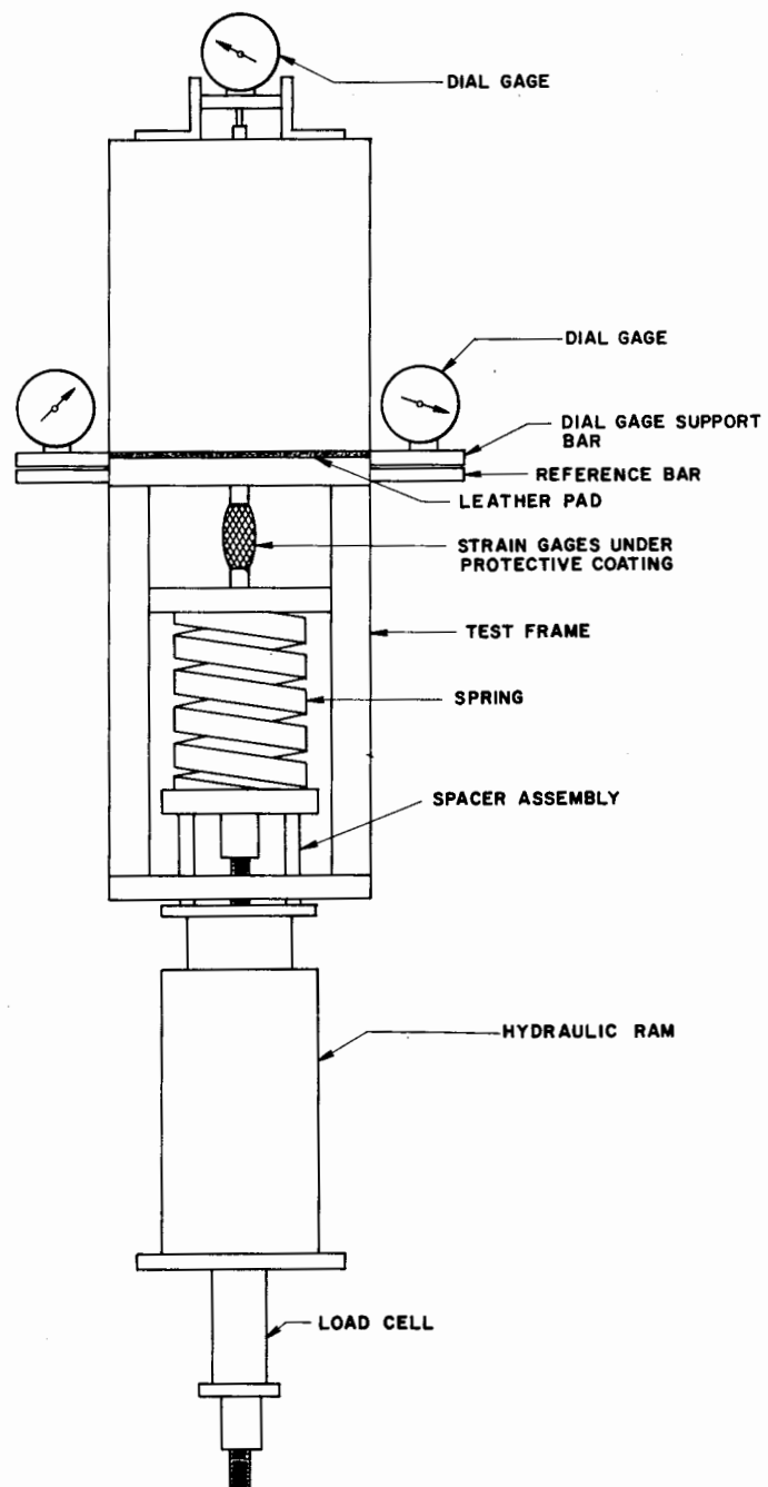
Specimen Loading Assembly
