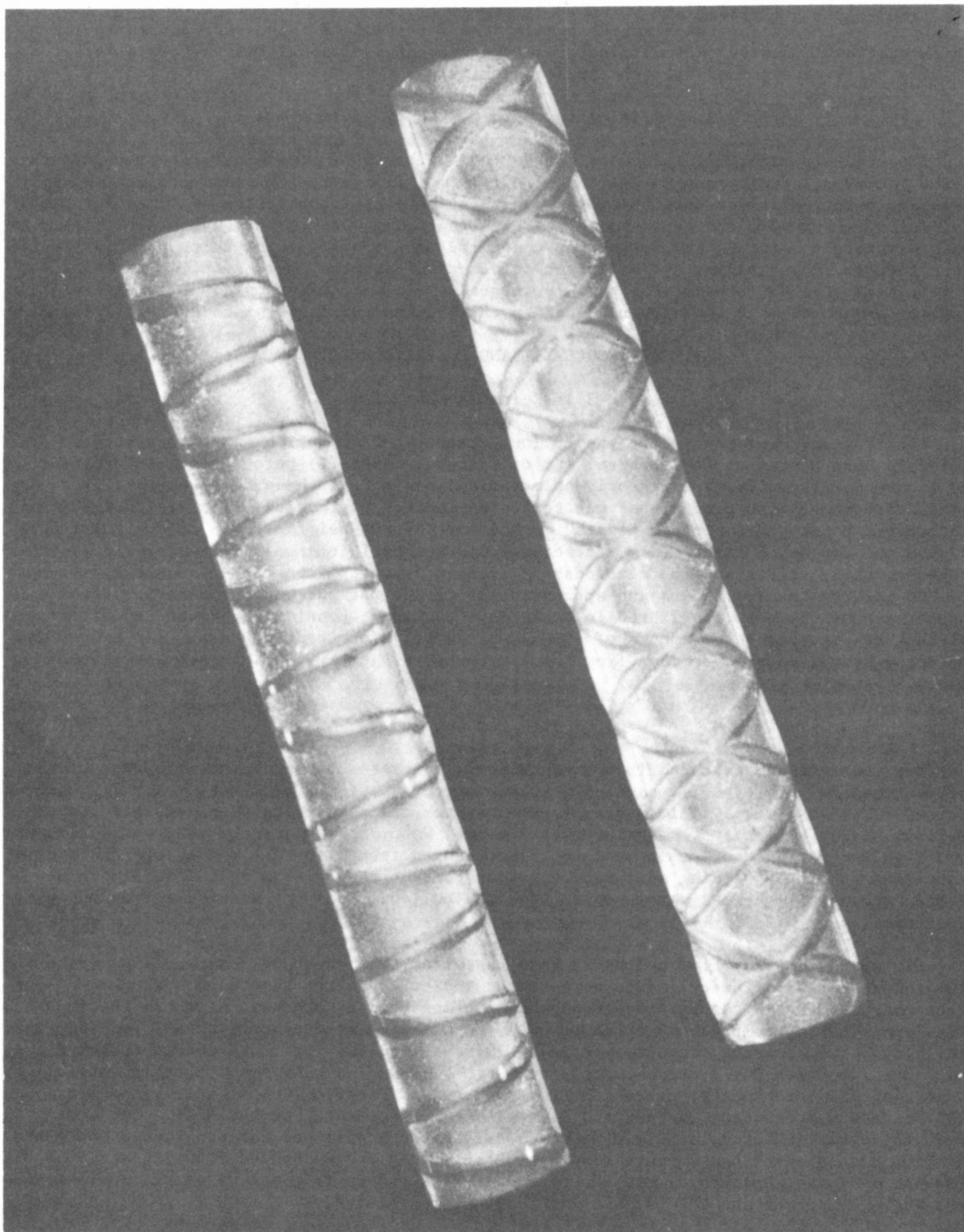
FIGURE 1. View of No. 6D (upper bar) and No. 6B (lower bar) reinforcing bars. D denotes diamond shaped deformation pattern and B indicates barrel pattern.
