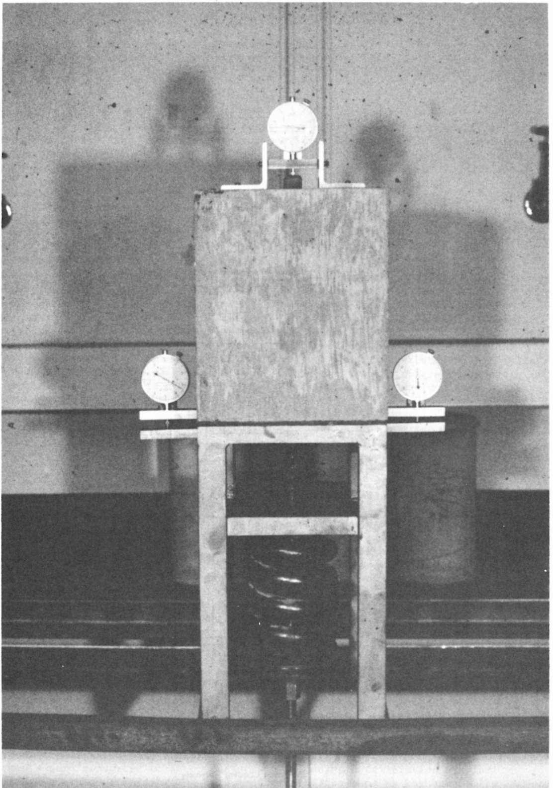
FIGURE 18. Creep specimen loaded to a tensile stress level of 30,000 psi (in the steel reinforcing bar).
