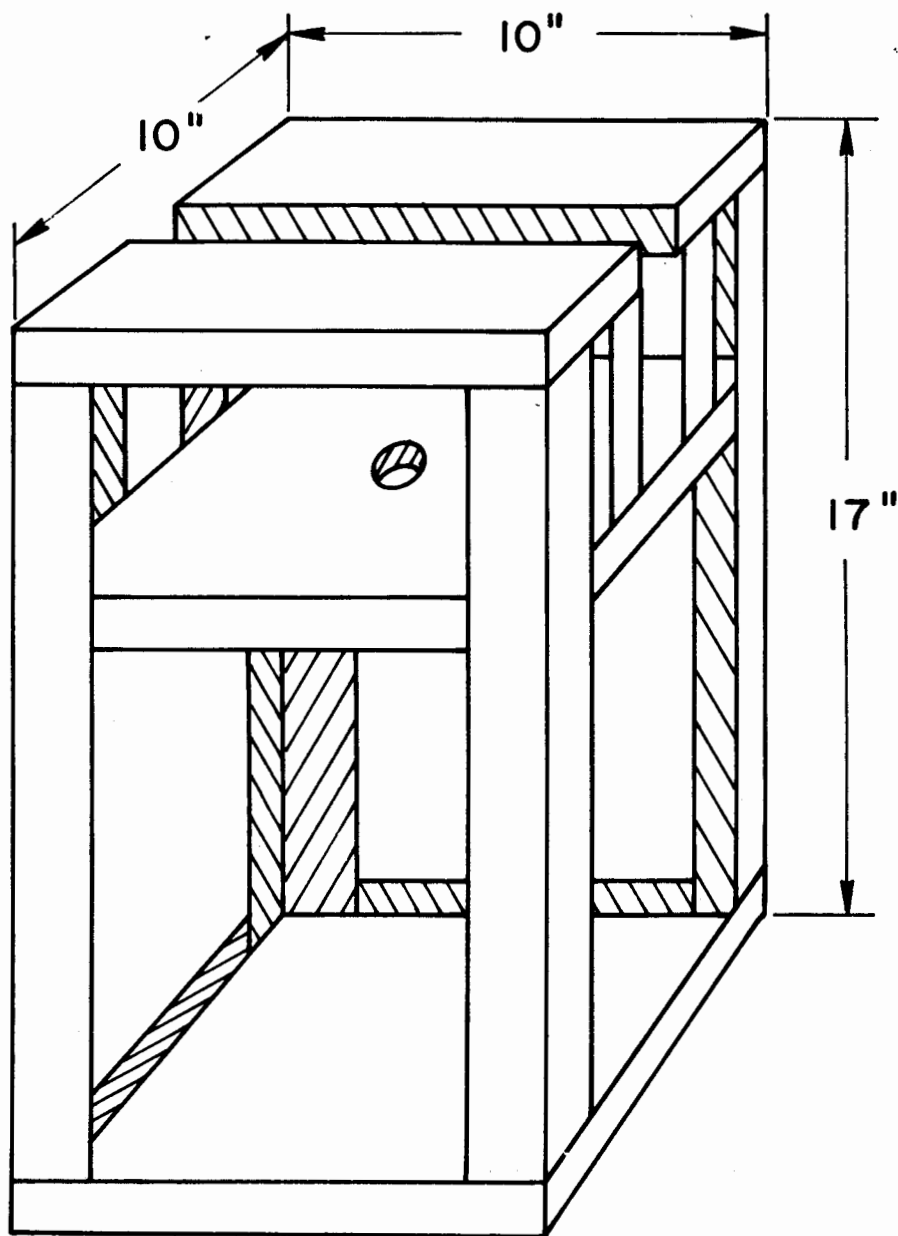
Test Frame
