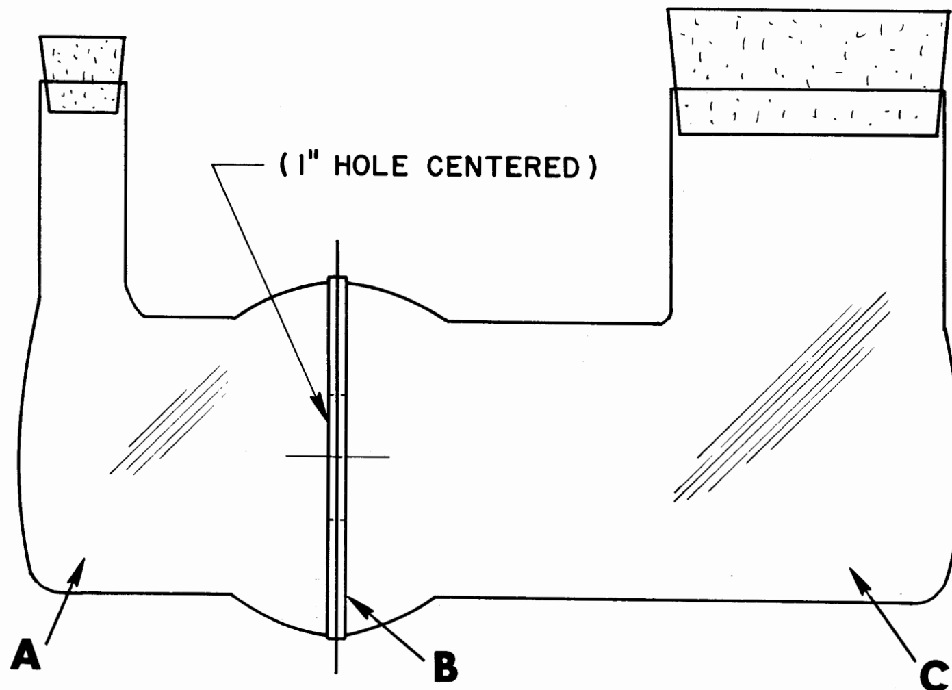
FIGURE 4. Permeability Cell
