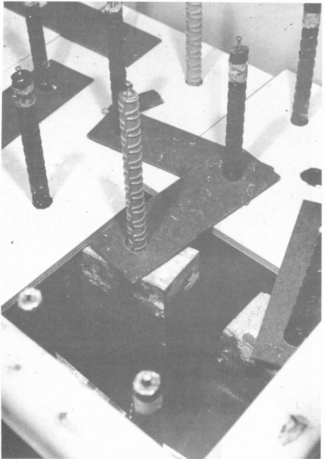
FIGURE 13. Corrosion-test specimens immersed in 3.5 percent solution of NaCl.
