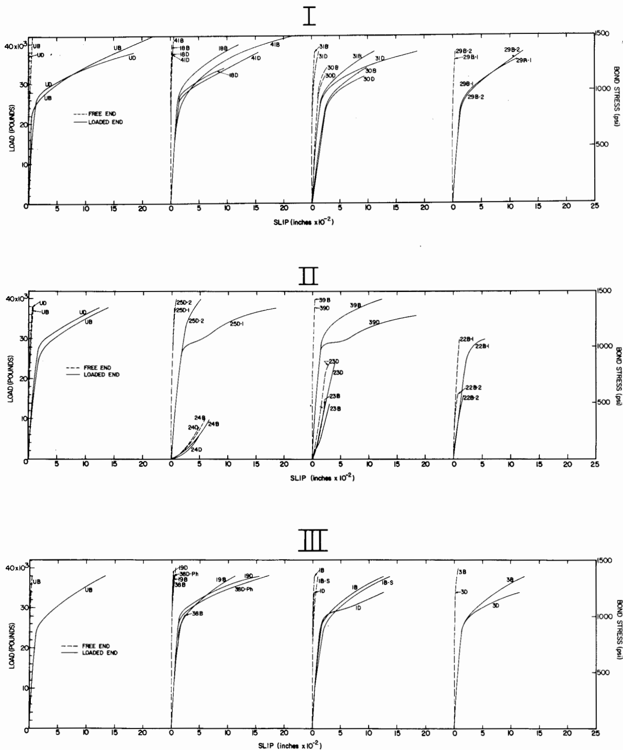
FIGURE 16. Applied load to reinforcing bar in pullout specimens versus free-end and loaded-end slip. Roman numbers indicate concrete batch number, while Arabic numbers identify the coating materials (table 1).
