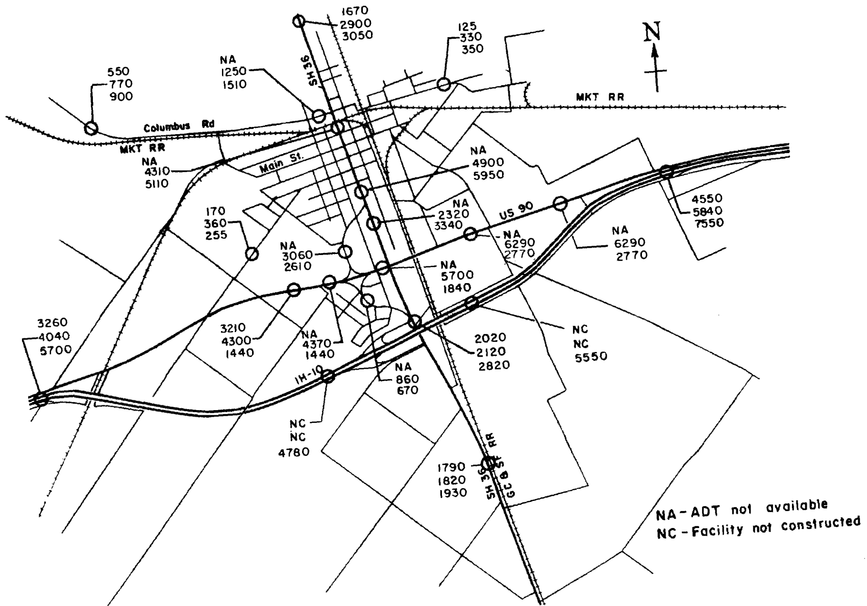
FIGURE 6.1.: TRAFFIC VOLUMES, SEALY ADT 1956, 1965, 1967
