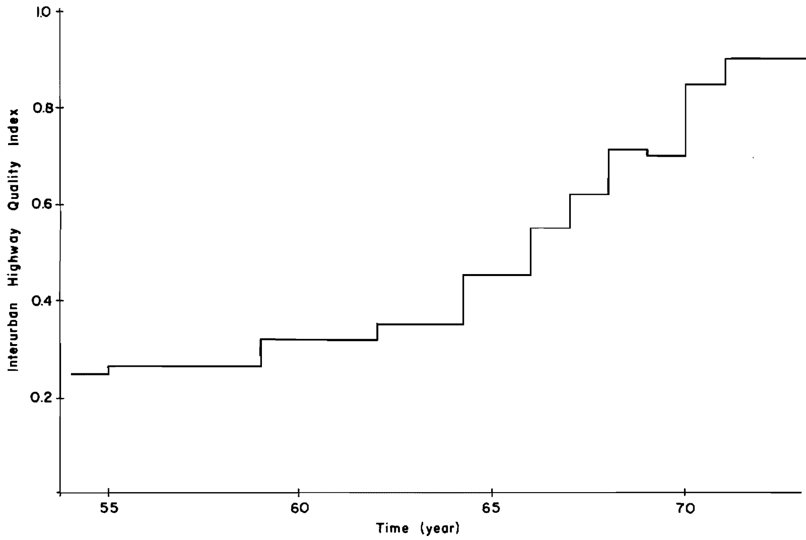
FIGURE A6.4: INTERURBAN HIGHWAY ROUTE QUALITY INDEX, US 90/IH 10 SAN ANTONIO - HOUSTON
