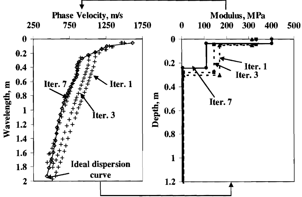
Figure 2.3 - Graphical Illustration of SASW Inversion Process
