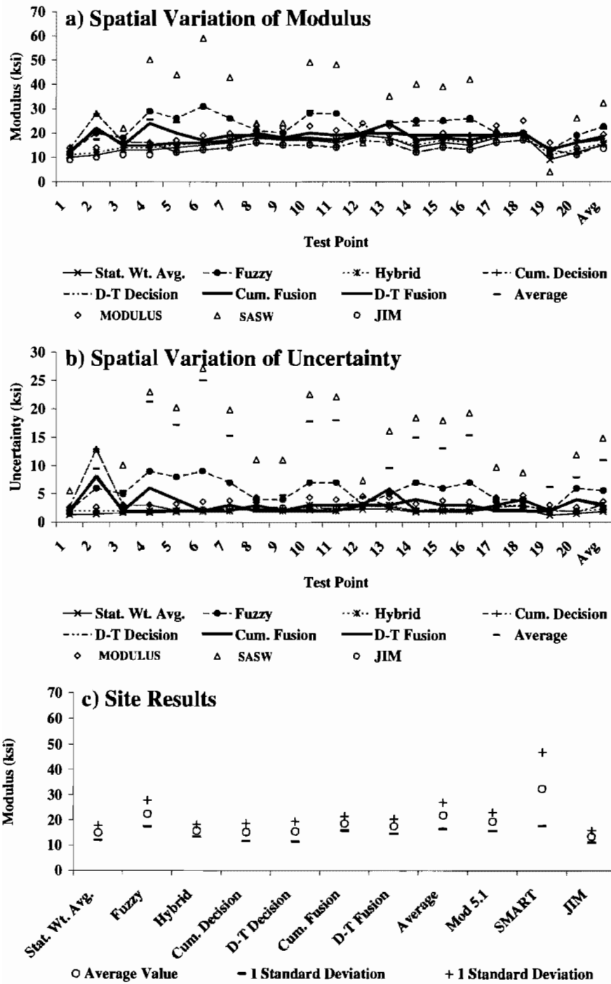
Figure 8.9 - Summary of Results for Subgrade Modulus Using TTI Site Data
