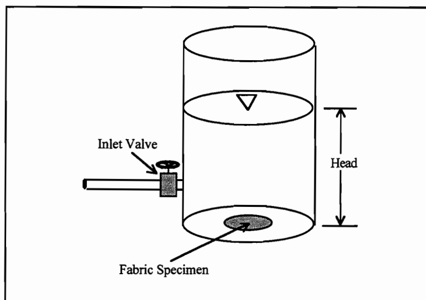
Figure 5.8 Modified Soil Permeameter
