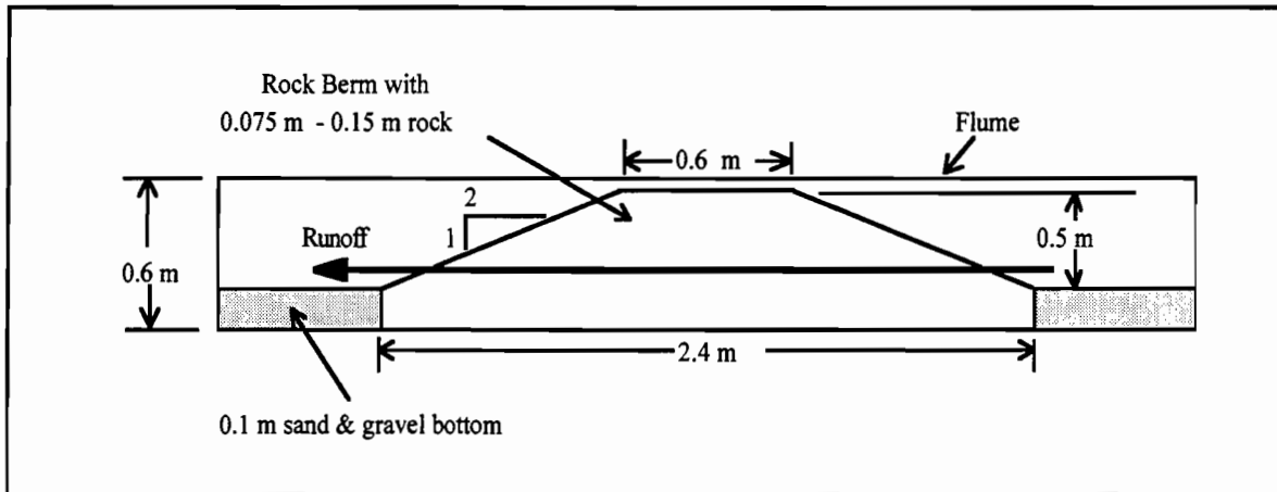
Figure 5.3 Section of Flume and Rock Berm Cross-Section
