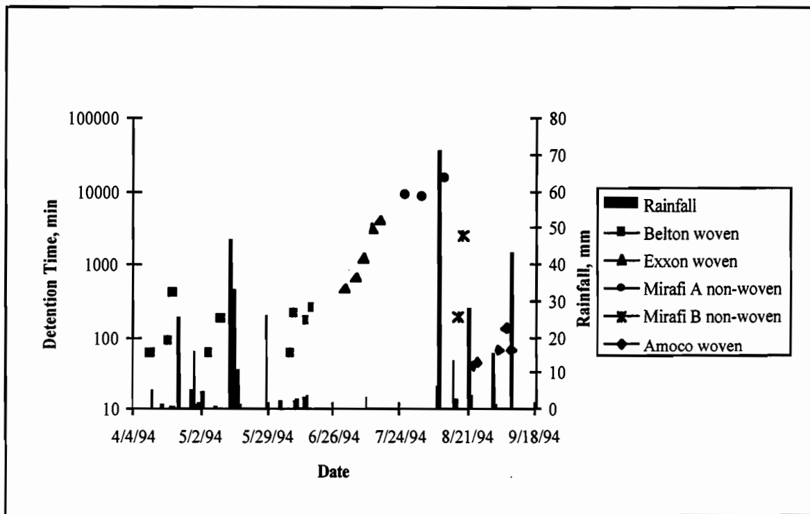
Figure 5.7 Detention Times as a Function of Testing Schedule
