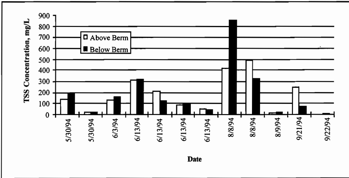
Figure 4.2 TSS Concentration of Samples Above and Below Rock Berm
