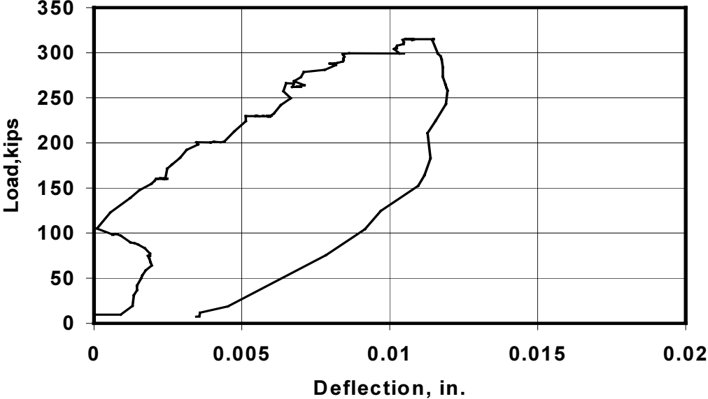
BG3N - North Bearing Pad (East Web)
