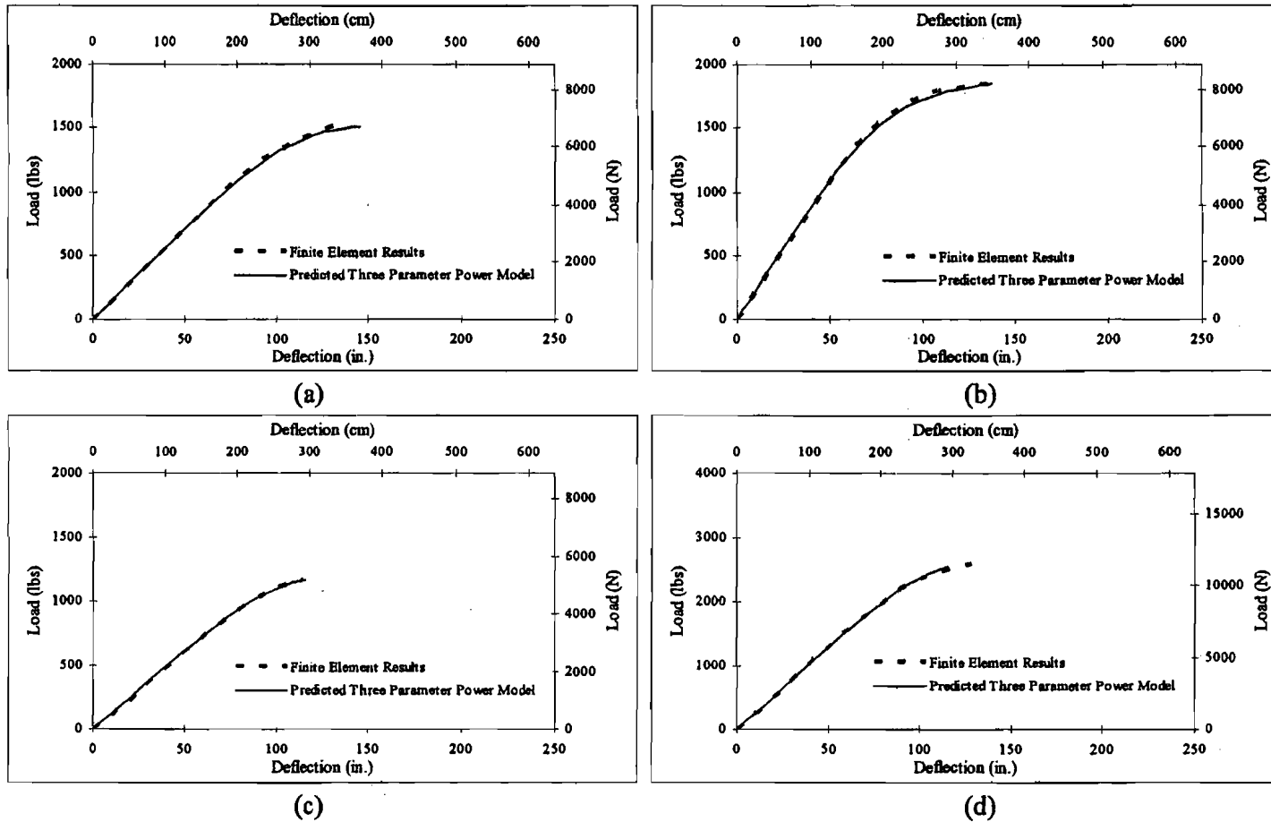
Figure C-6 Comparison of FEM model and predicted equation model for FRP poles: (a) F35-1-0.275-0.275-1.125-12-6.5-2.75-16-15-50-3.5; (b) F35-1-0.3-0.3-1.25-12-7-2.5-16.2-15.7-56-5; (c) F35-1-0.35-0.35-1-10-5-2.5-13.5-12.5-41-4.5; (d) F35-1.25-0.325-0.325-1.5-13-8-3-17.5-16-90-4
