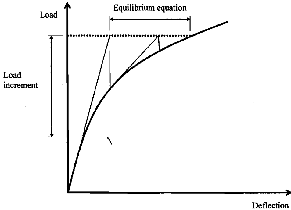
Figure 3.7 Newton-Raphson scheme
