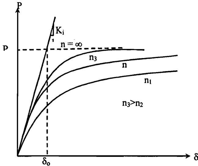
Figure 4.2 Three-parameter power model
