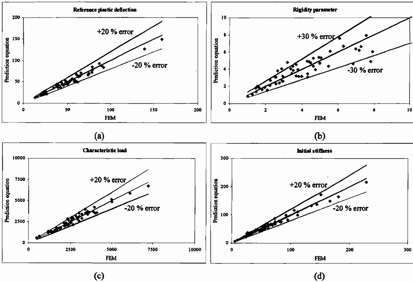
Figure D-1 Error band analysis for steel poles: (a) Reference plastic deflection; (b) Rigidity parameter; (c) Proposed characteristic load; (d) Initial stiffness
