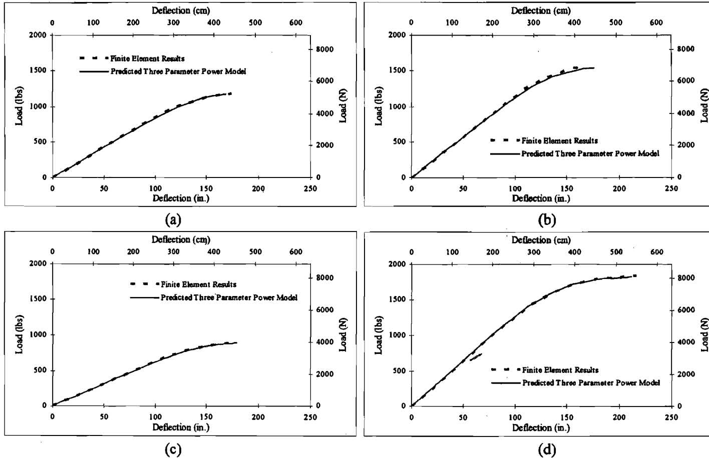
Figure C-8 Comparison of FEM model and predicted equation model for FRP poles: (a) F40-1-0.275-0.3-1.125-11-5.5-2.75-14.5-13-50-4; (b) F40-1-0.3-0.325-1.25-12.5-6-3-16.5-15-60-3.5; (c) F40-1-0.325-0.325-1-9-4.5-2.25-12-10.5-45-5; (d) F40-1-0.35-0.325-1.5-12-6.5-3.25-16.5-15-95-4
