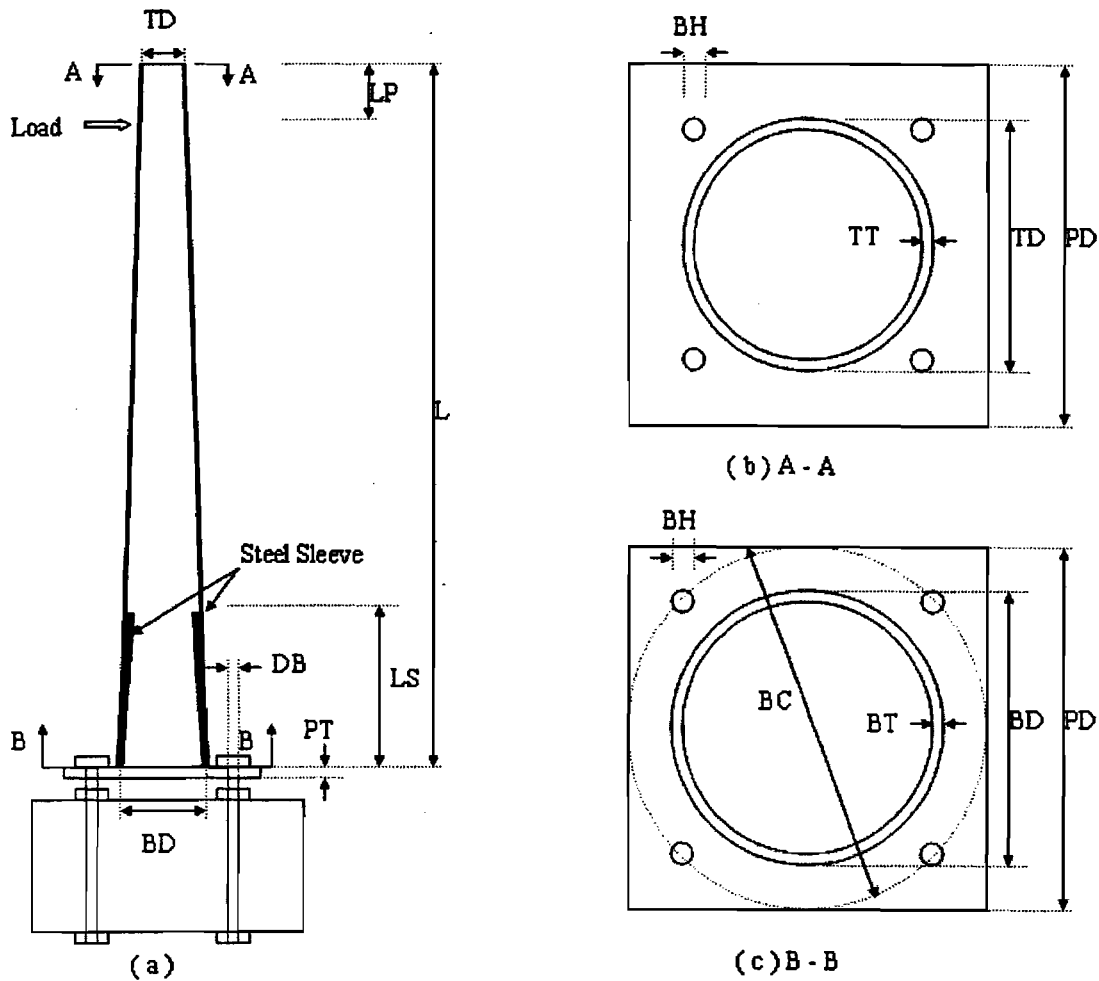
Figure 2.2 Typical dimensions of FRP poles tested: (a) Front view; (b) Section A-A; (c) Section B-B
