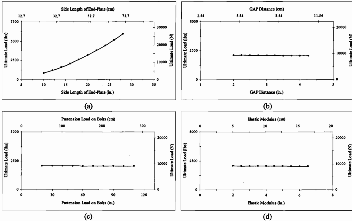
Figure F-3 Sensitivity plots of ultimate load vs. PD, GAP, E_p , and E for FRP poles: (a) Ultimate load vs. side length of end-plate; (b) Ultimate load vs. GAP distance; (c) Ultimate load vs. pretension load on bolts; (d) Ultimate load vs. elastic modulus
