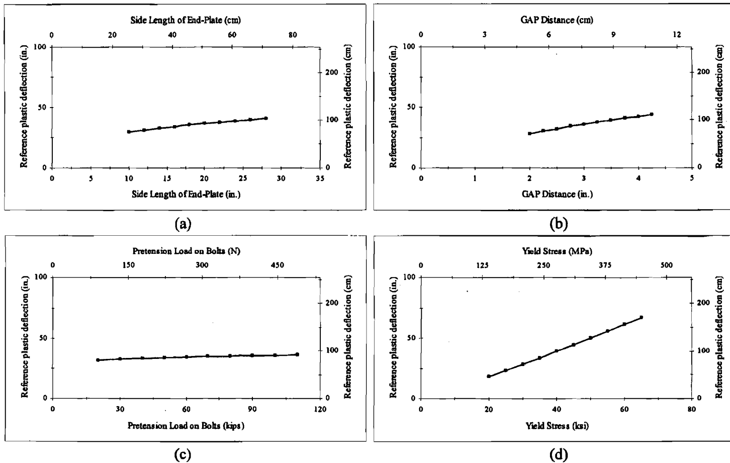
Figure E-6 Sensitivity plots of reference plastic deflection vs. PD, GAP, F_p , and F_y for steel poles: (a) \delta_0 vs. side length of end-plate; (b) \delta_0 vs. GAP distance; (c) \delta_0 vs. pretension load on bolts; (d) \delta_0 vs. yield stress
