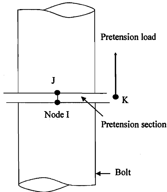
Figure 3.4 Pre-tensioning section
