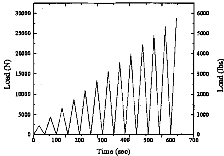
Figure 2.7 Loading history
