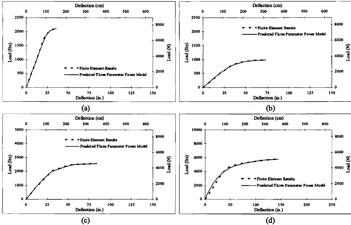
Figure B-4 Comparison of FEM model and predicted equation model for steel poles: (a) S30-1-0.15-0.15-1.25-11-6-3.25-40-15.5-15-50; (b) S30-1.25-0.15-0.15-1-7-4-2.75-45-10.5-10-40; (c) S35-1-0.2-0.2-1.25-11-7-3-40-15.5-17-70; (d) S35-1-0.3-0.3-1.75-12-6-3.75-50-18-17-100
