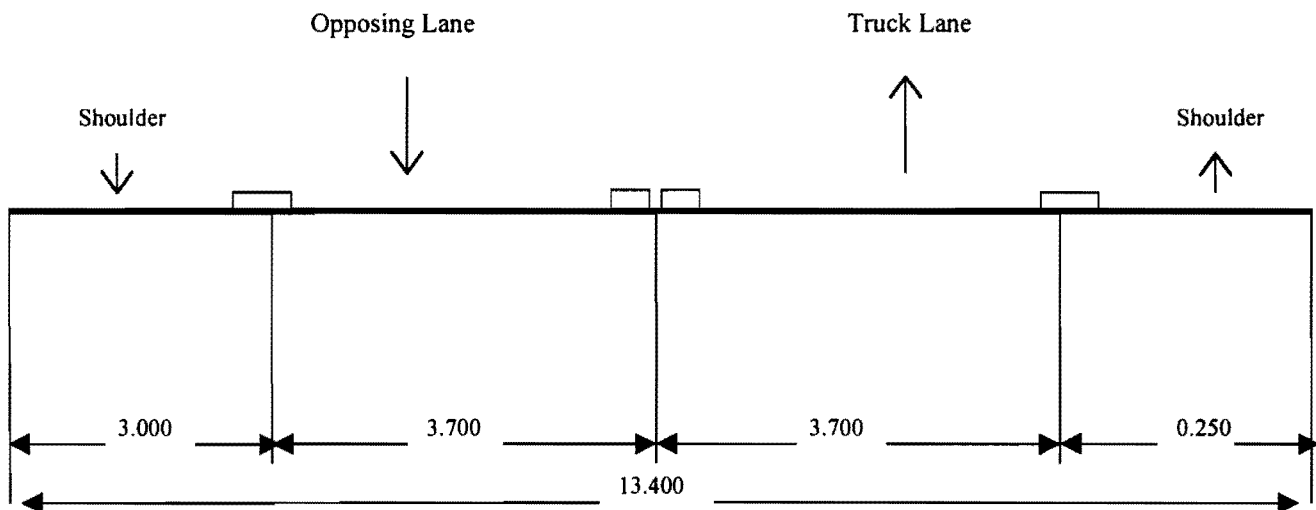
Figure 2-1: Current Two-Lane Rural Highway Cross-section
