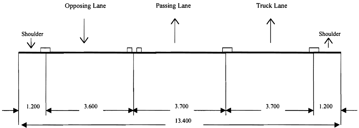
Figure 2-2: Three Lane Highway Cross Section in Canada
