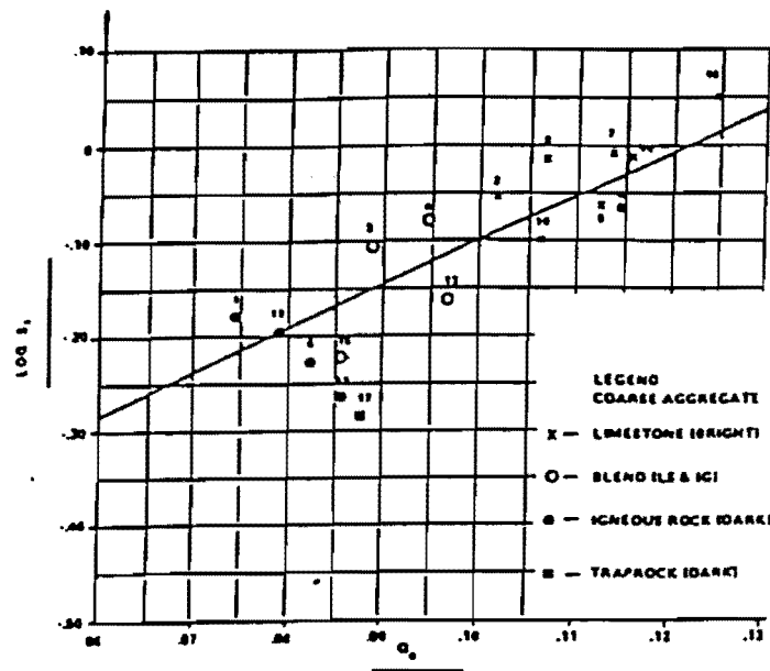
Figure 3.27. Specularity plot of ( \log S1 vs. Q_0 ) samples from Highway 40 test section, Ontario (Jung et al., 1984)
