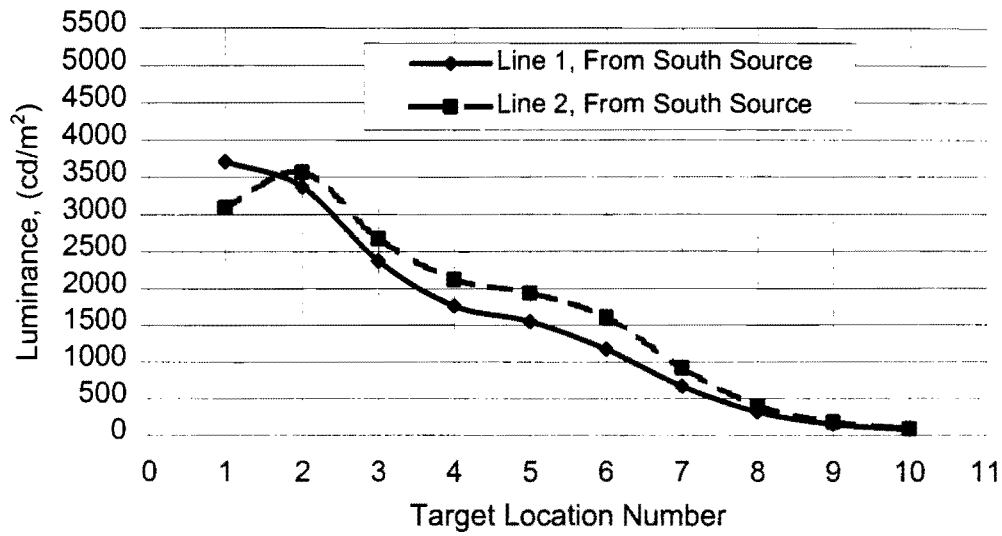
Figure 6.2 Luminance distribution, in the south source direction, between the installation at 26 cm height above the roadway surface on the lines 1 and 2.
