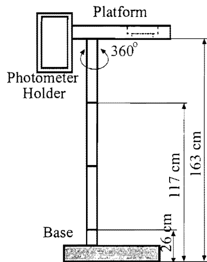
Figure 5.6 Luminance-illuminance-photometer stand.
