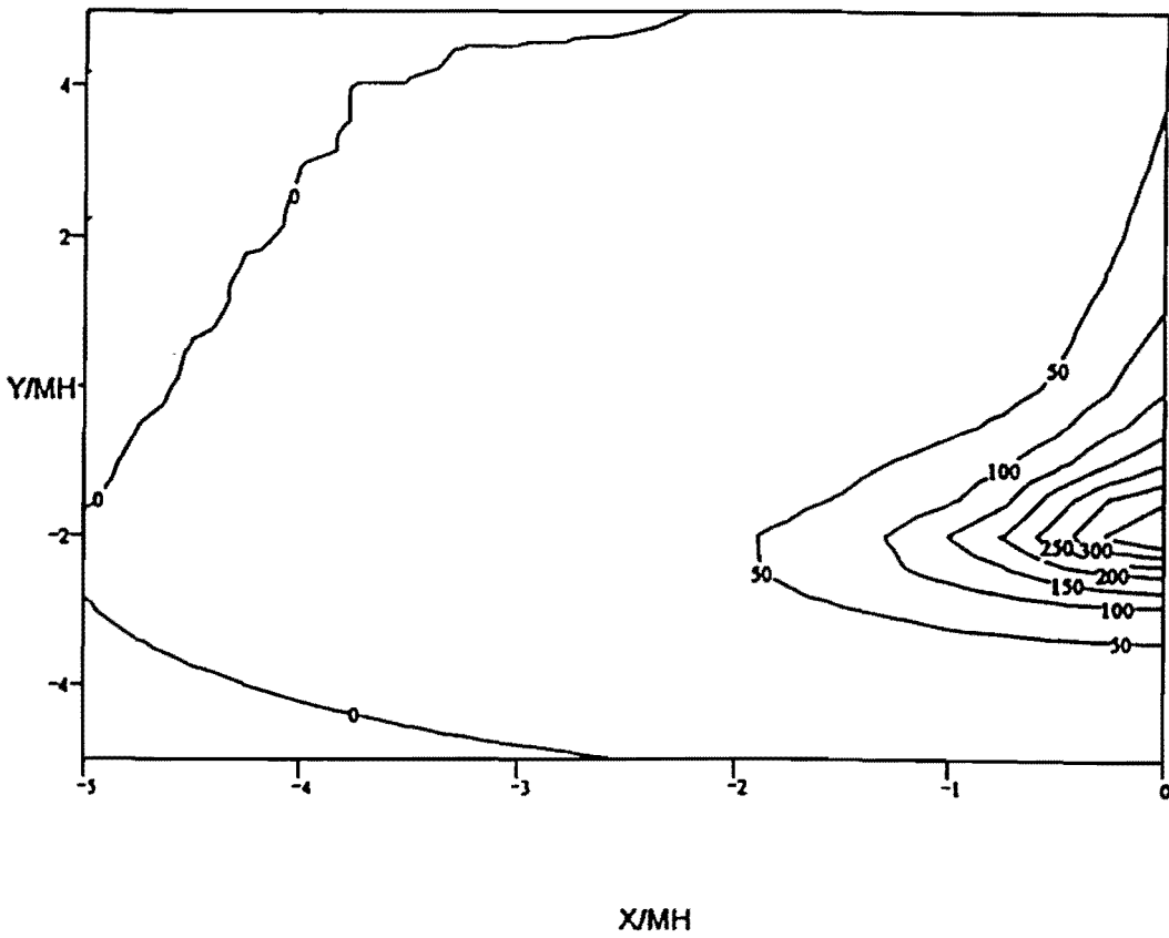
Figure 3.10. R-table and contour diagram of the r-values for standard R1 class
