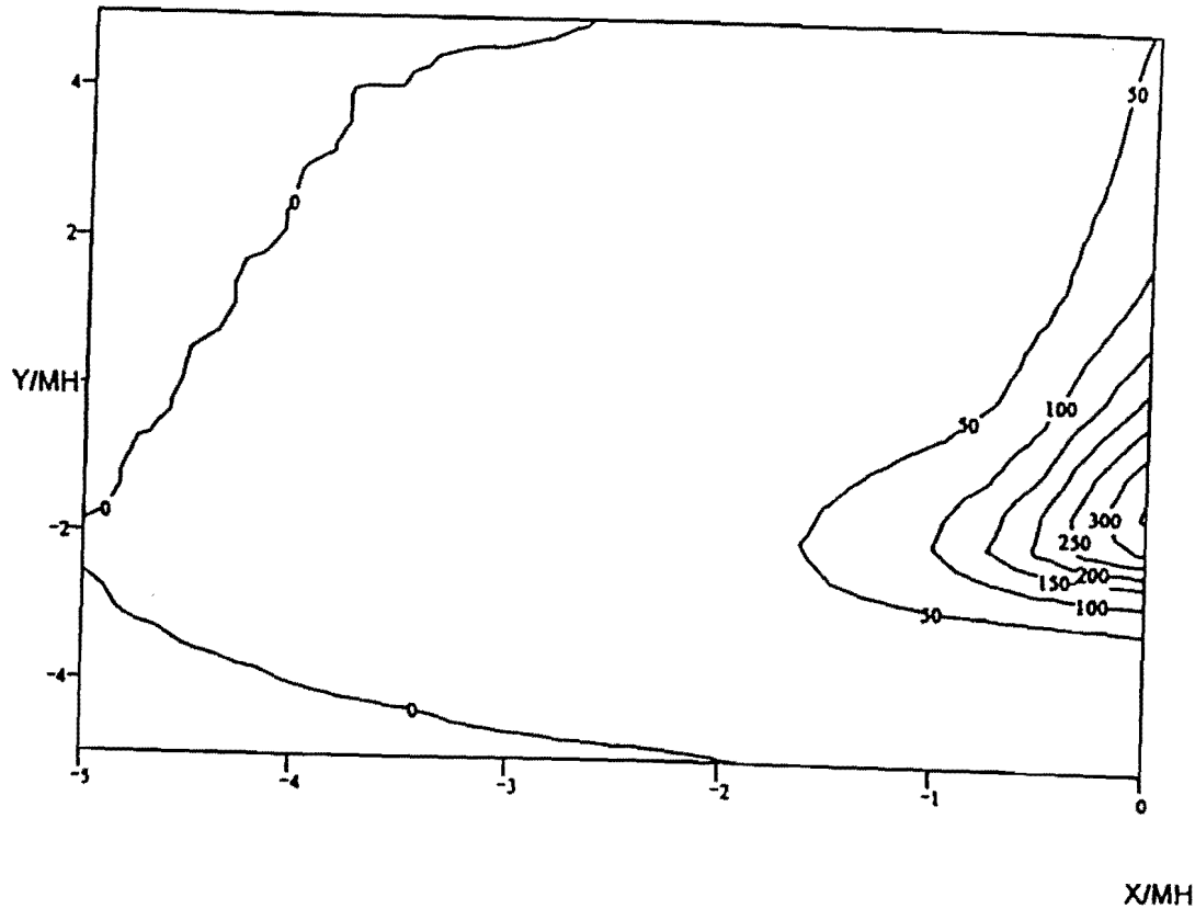
Figure 3.11. R-table and contour diagram of the r-values for standard R2 class
