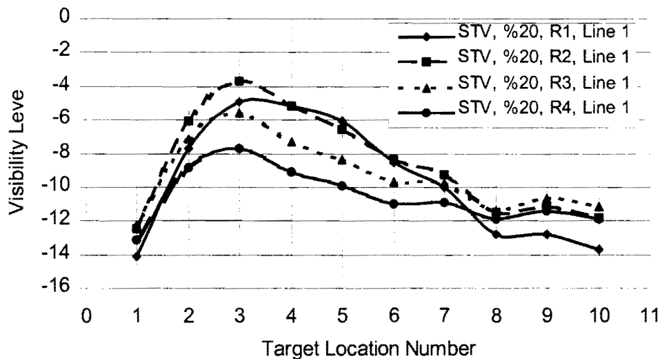
Figure 7.22 Visibility level distribution for four different pavements on the line 1 between the installations.
