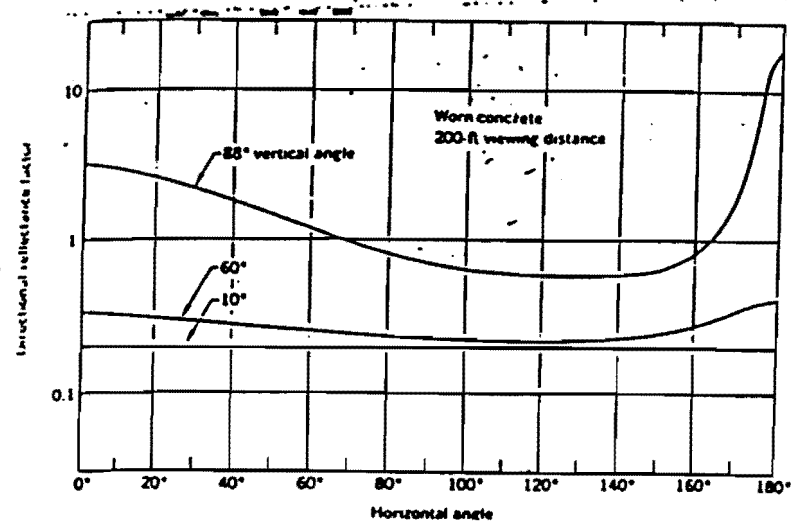
Figure 3.21. Directional reflectance factors for (a) asphalt and (b) Portland cement pavement surface (King and Finch, 1968)
