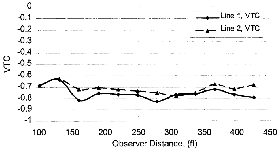
Figure 8.29 Dynamic contrast distribution for ninth target location on lines 1 and 2.
