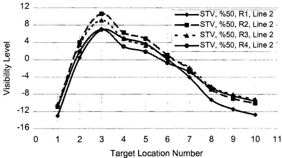
Figure 7.25 Visibility level distribution for four different pavements on the line 2 between the installations.
