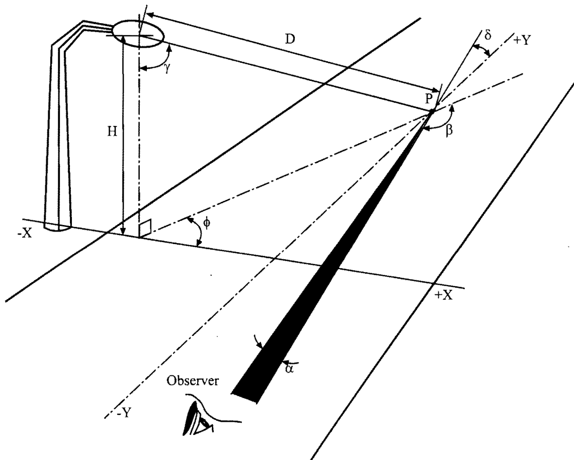
Figure 7.8 Single luminaire.
