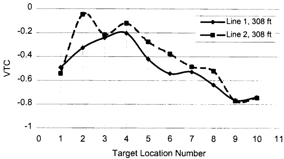
Figure 8.39 VTC distribution for constant distance 308 ft on lines 1 and 2.
