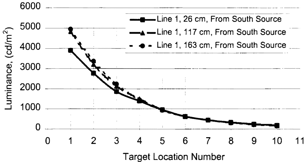
Figure 6.28 Luminance distribution, from south source, at 26 cm, 117 cm and 163 cm height above the roadway surface on line 1.
