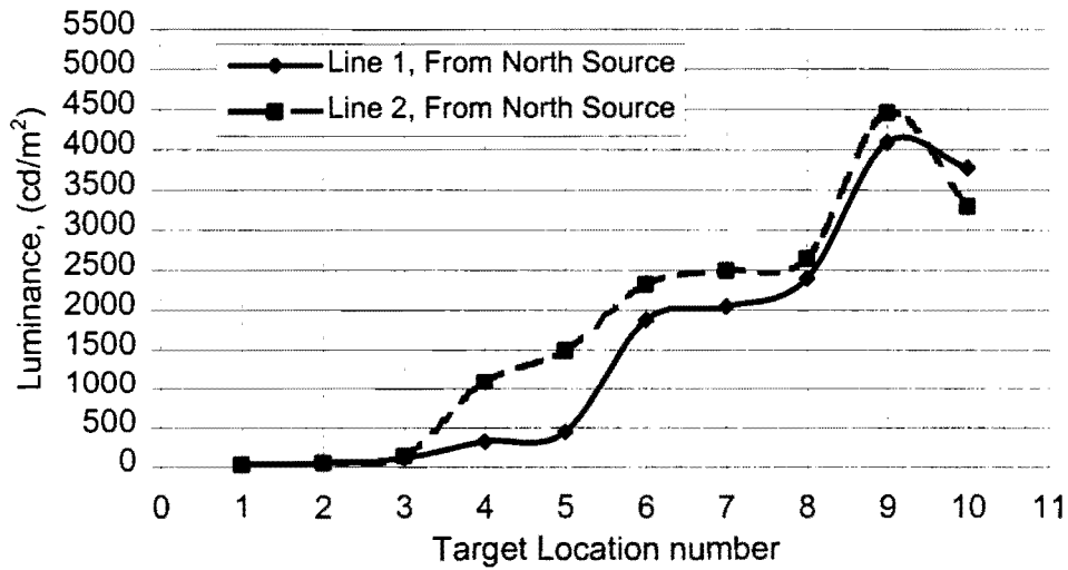
Figure 6.3 Luminance distribution, in the north source direction, between the installation at 26 cm height above the roadway surface on the lines 1 and 2.
