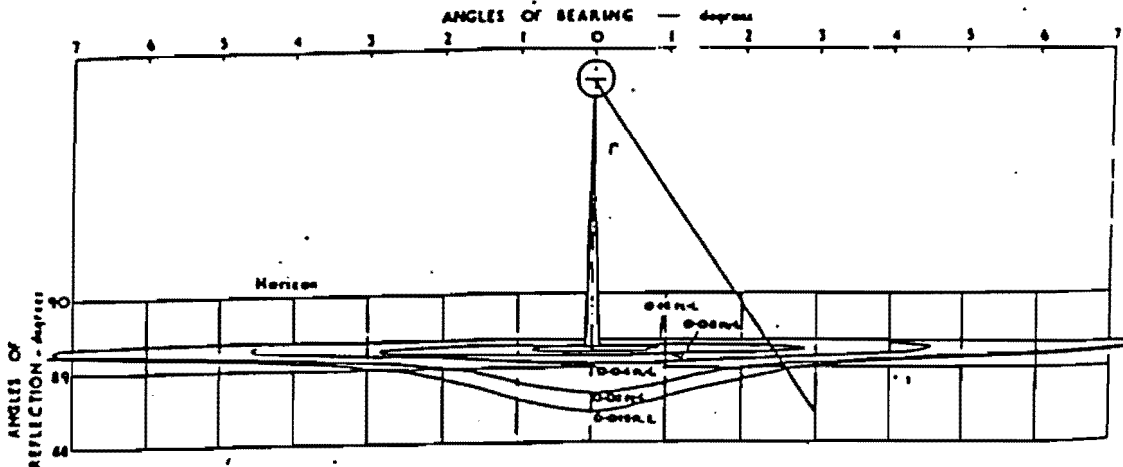
Figure 3.24. Standard iso luminance contours in perspective for bituminous sand carpet under standard conditions (Christie, 1954)
