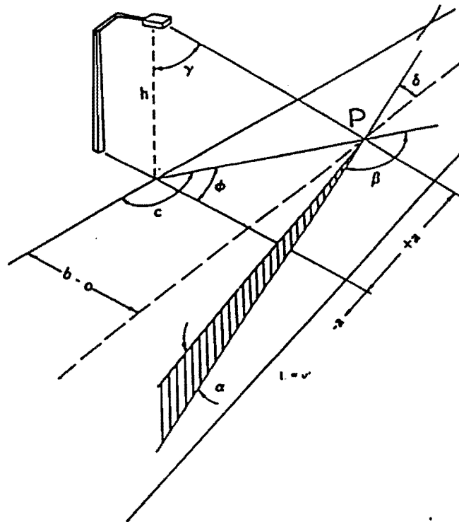
Figure 3.2. Angular relationships for calculating luminance for a single luminaire
