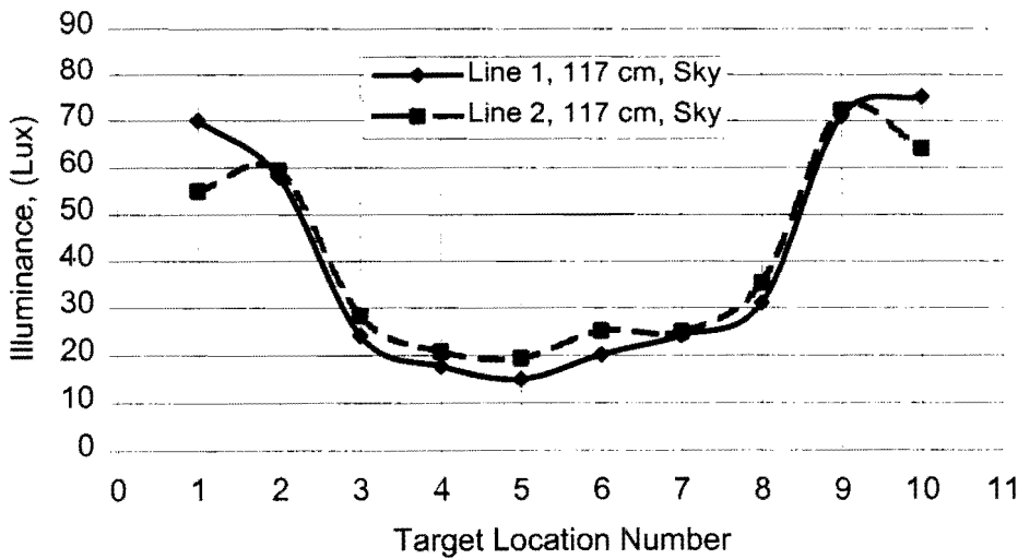
Figure 6.42 Illuminance distribution, in the sky direction, between the installation at 117 cm height above the roadway surface on the lines 1 and 2.
