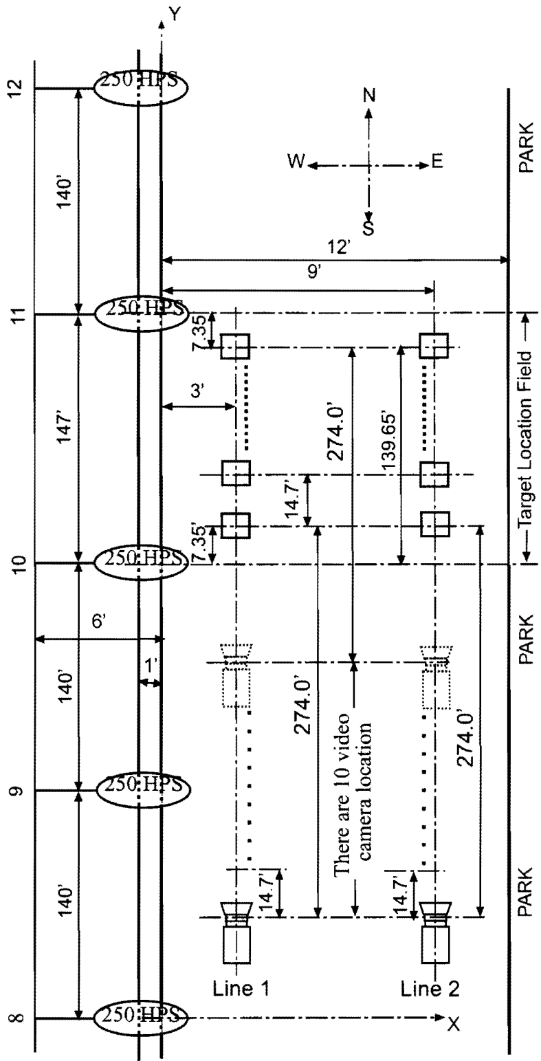
Figure 8.2 Orientation of the video camera and target for static video recording system.
