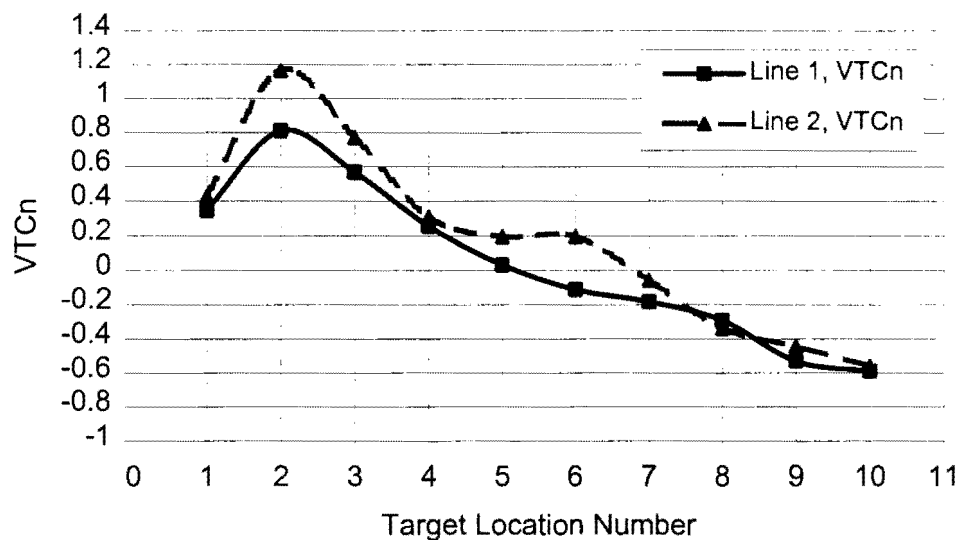
Figure 8.14 VTCn distribution calculated from images for 50% reflective target on the lines 1 and 2.
