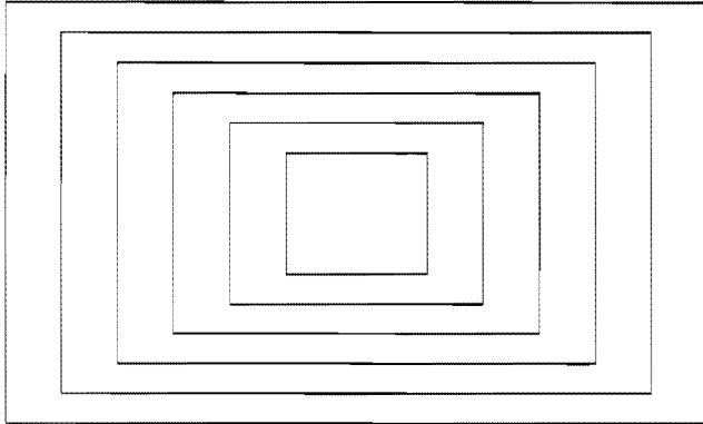
Figure 4.11. Rectangular band division
