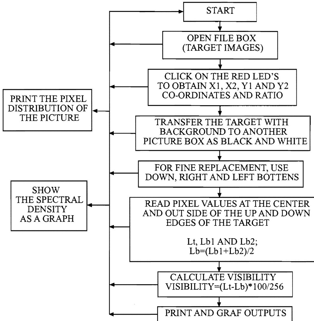
Figure 8.8 Flow chart of the picture analysis program.
