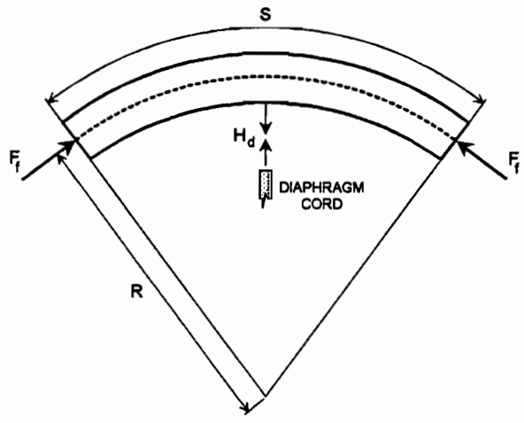
Figure 1-15 Diaphragm equilibrium
