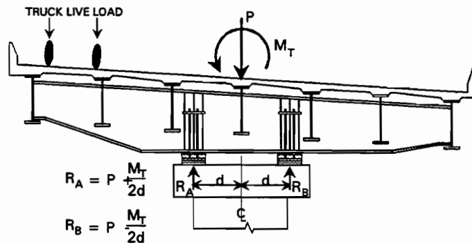
Figure 1-5 Statics of cap girder centered on pier
