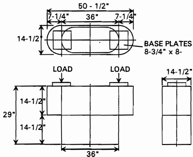
Figure 11- 5 Geometry of the test specimens
