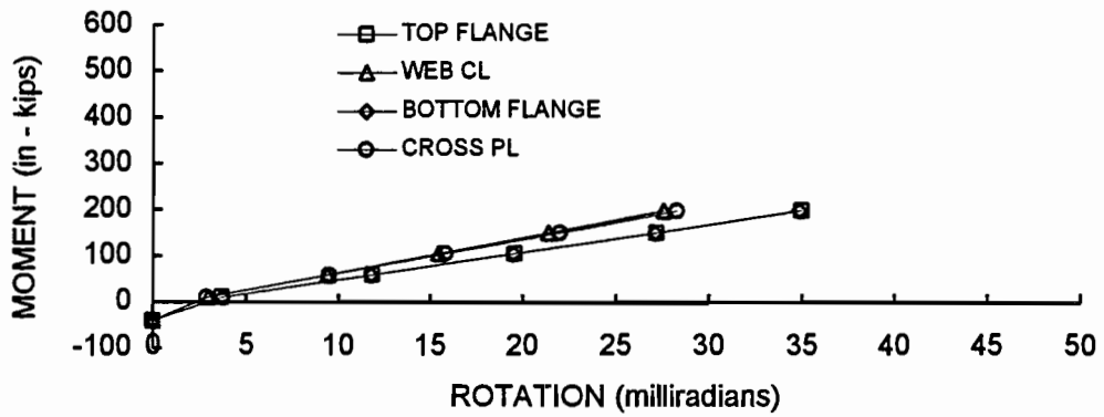
Figure 8-13 Moment vs. rotation (0) anchor bolts, CoR = 0"
