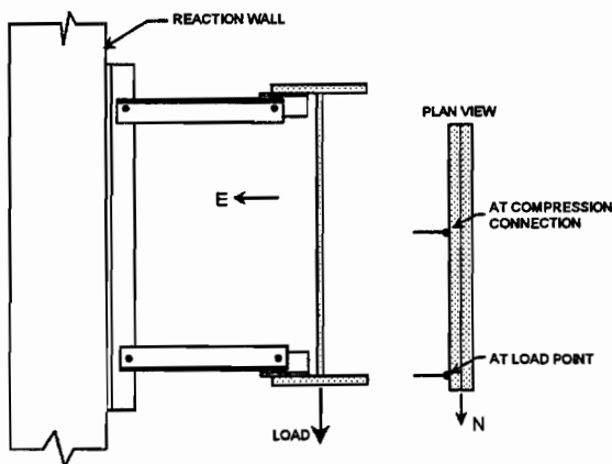
Figure 8-9 Bracing scheme
