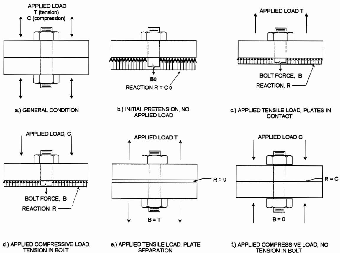
Figure 1- 6 Behavior of pretensioned connection
