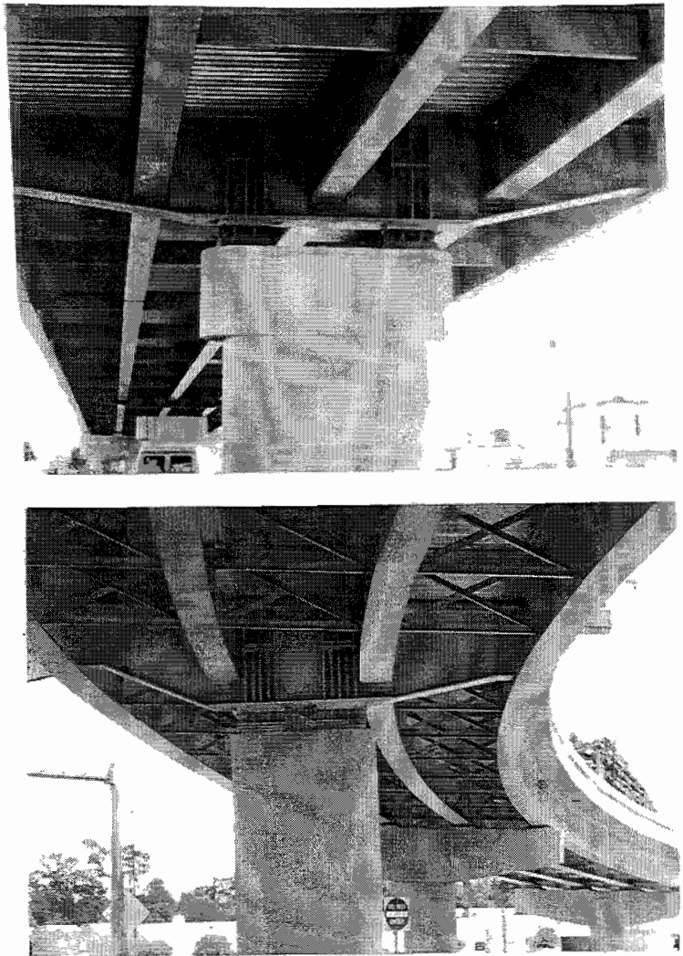
Figure 1- 1 Connection between integral steel cap girder and concrete pier
