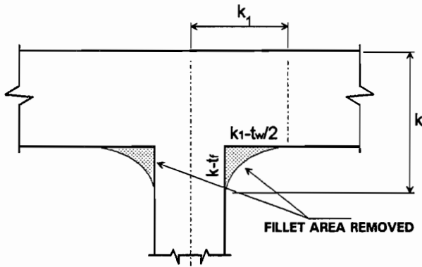
Figure 7-12 Notched specimen detail
