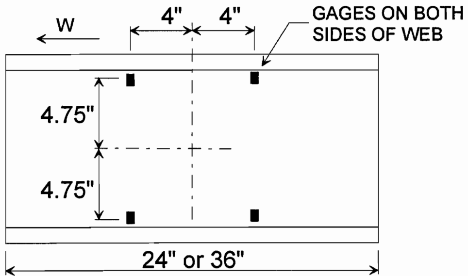
Figure 6-6 Location of strain gages on test specimen
