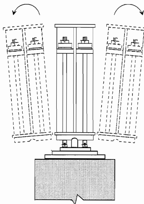
Figure 8-38 Vertical adjustment of cap girder
