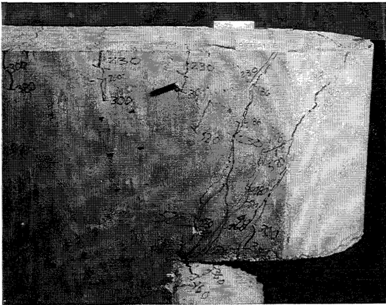
Figure 11- 16 Crack distribution of Pier A1-1 after failure.
