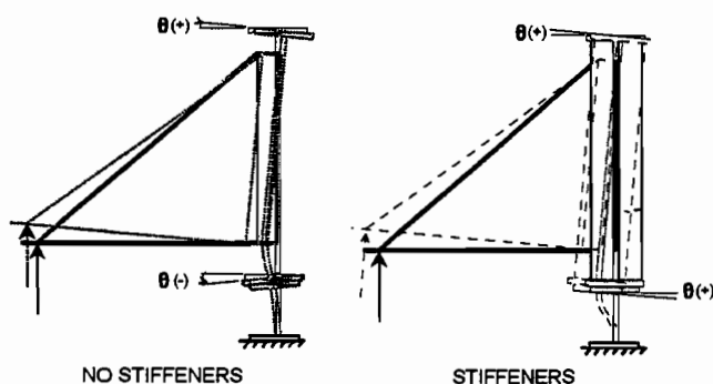
Figure 8- 19 Illustration of negative rotation
