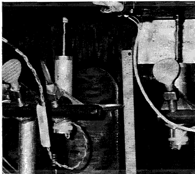
Figure 3- 7 Separation at the uplift bearing
