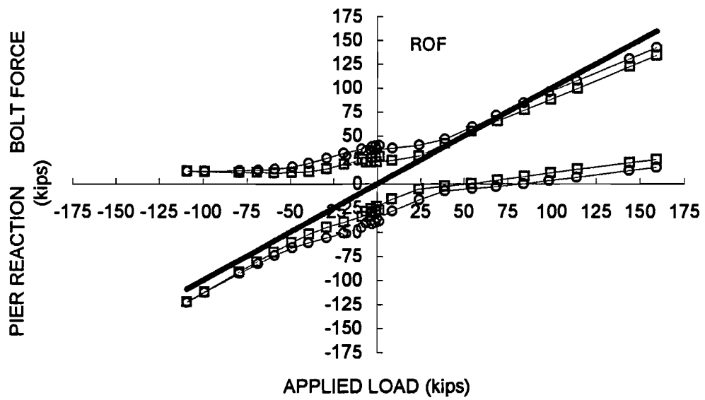
Figure 3- 11 Bolt group force, pier reaction vs. reaction force, ROF pads
