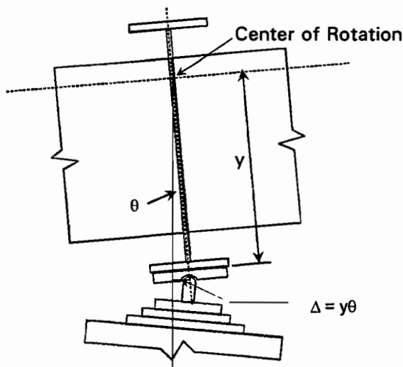
Figure 1-9 Horizontal displacement of bearing
