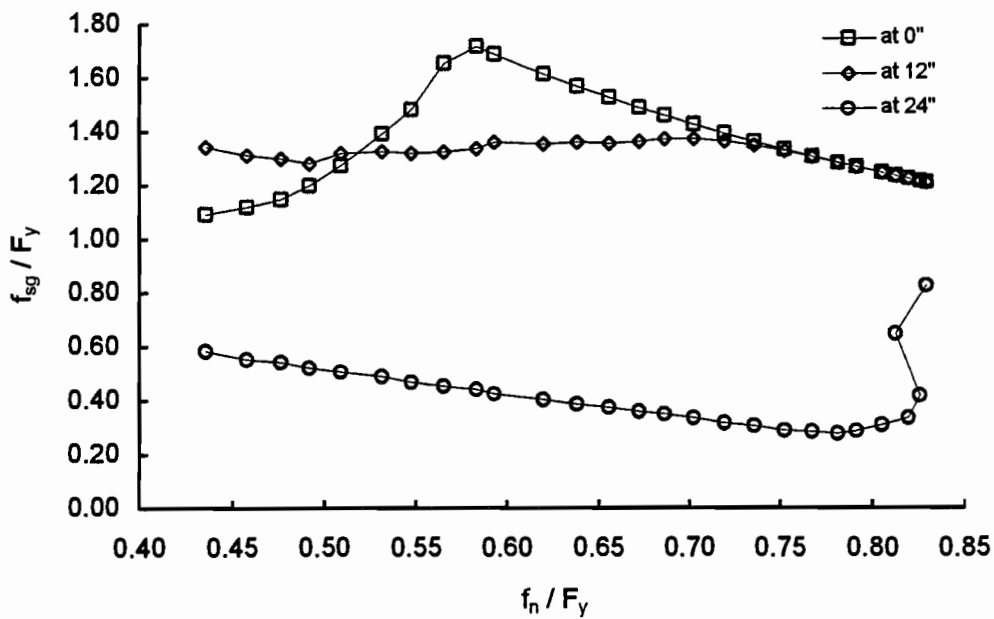
Figure 8-30 Normalized stress at top gages vs. nominal web stress, W12X87. Compression bearing with pretensioned anchor bolts
