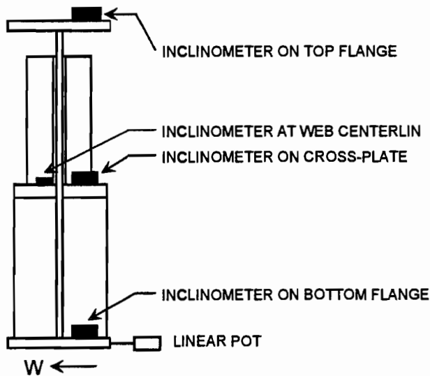
Figure 8-8 Location of inclinometers
