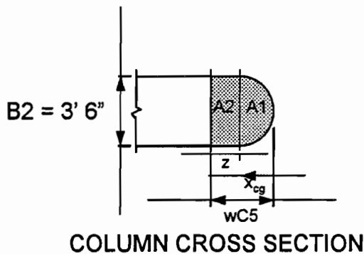
Figure 11-30 Cross section of Strut C5
