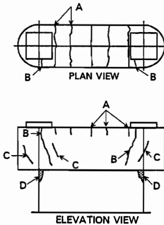
Figure 11-14 Patterns of concrete distress
