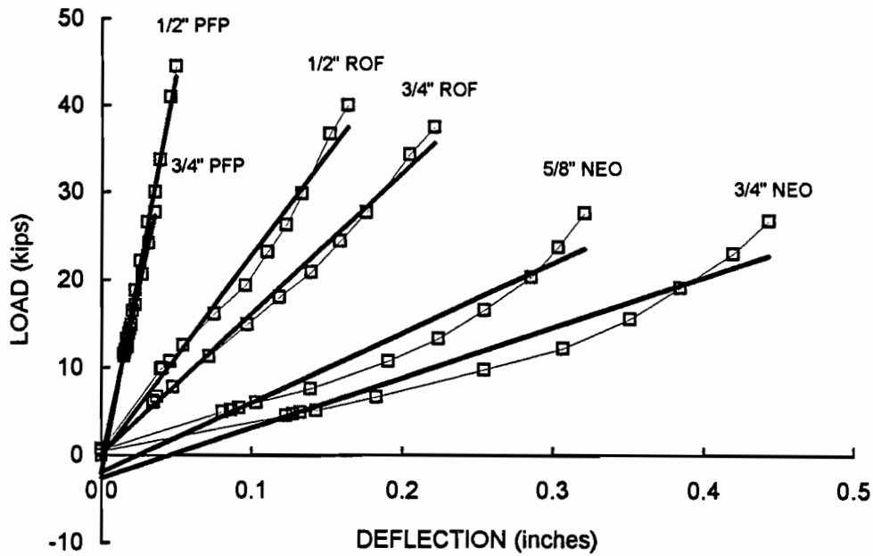
Figure 4-2 Load vs. Deflection curves for bearing pads
