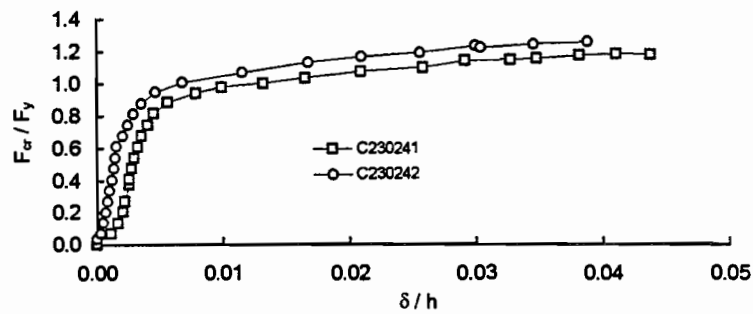
Figure 6- 12 Non-dimensional axial stress vs. lateral deflection, W12 X 230
