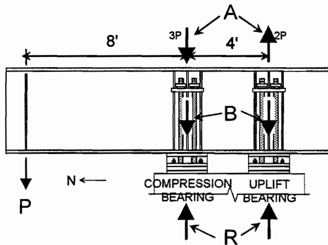
Figure 8- 27 Connection statics
