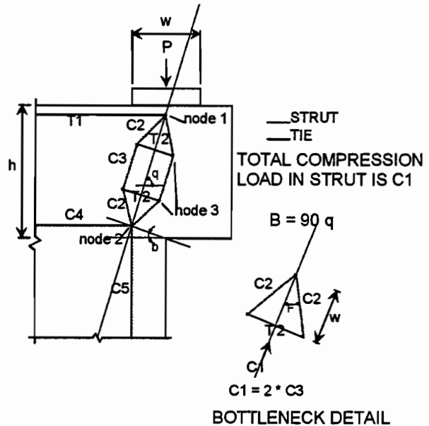
Figure 11-29 Strut-and-tie model for Example Problem
