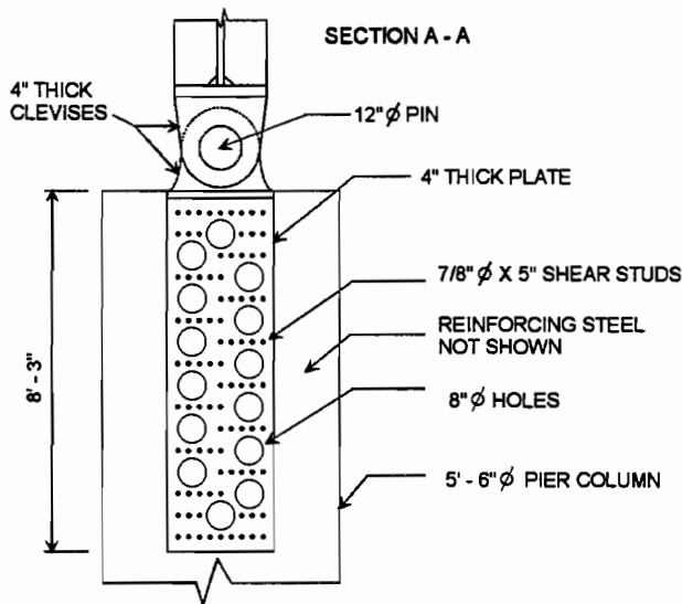
Figure 1- 11 Single column with pinned bearing connection
