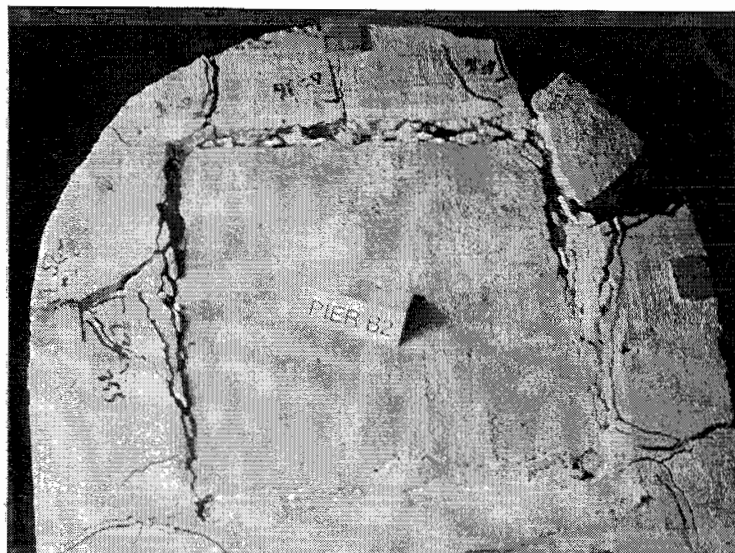
Figure 11- 22 Punching of the base plate into Pier B2-2
