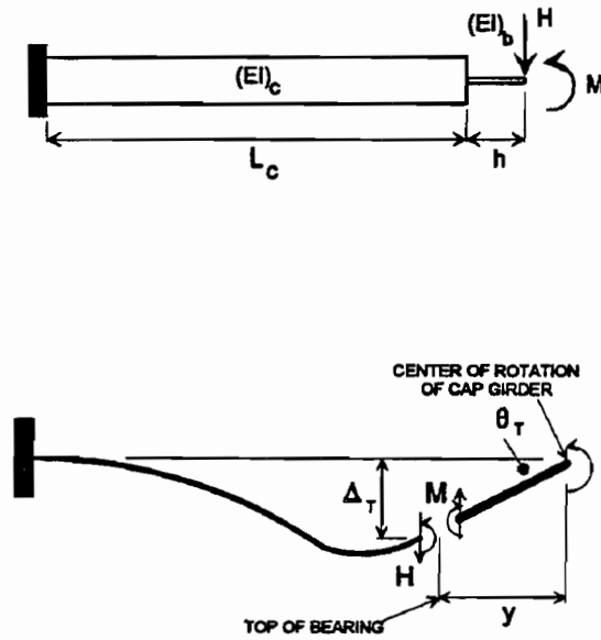
Figure 8-37 Pier column and bearing
