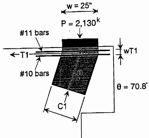
Figure 11-34 Geometry of the CCT Node (Node 1) in the strut-and-tie model
