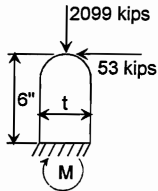
Figure A.3 Forces on Rocker Pin
