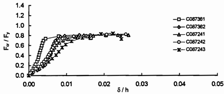
Figure 6- 10 Non-dimensional axial stress vs. lateral deflection, W12 X 87
