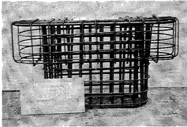
Figure 11- 10 Steel reinforcing cage for Specimen A2
