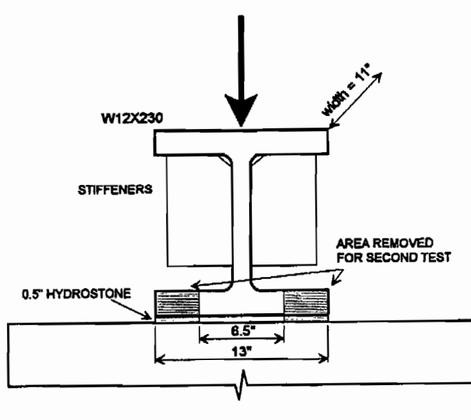
Figure 6- 25 Bearing strength test specimen
