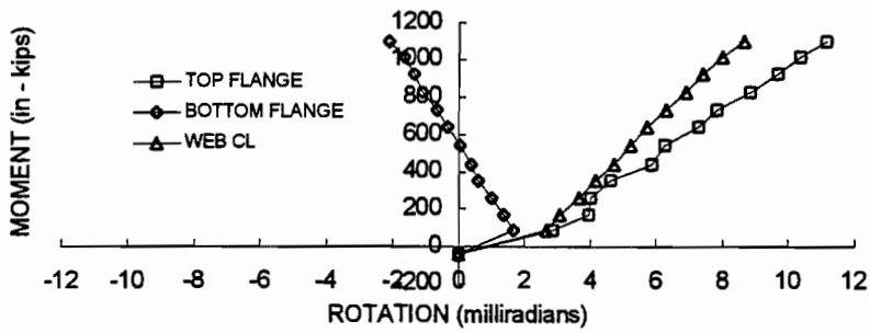
Figure 8- 16 Moment vs. rotation, (0) anchor bolts, CoR = 34"
