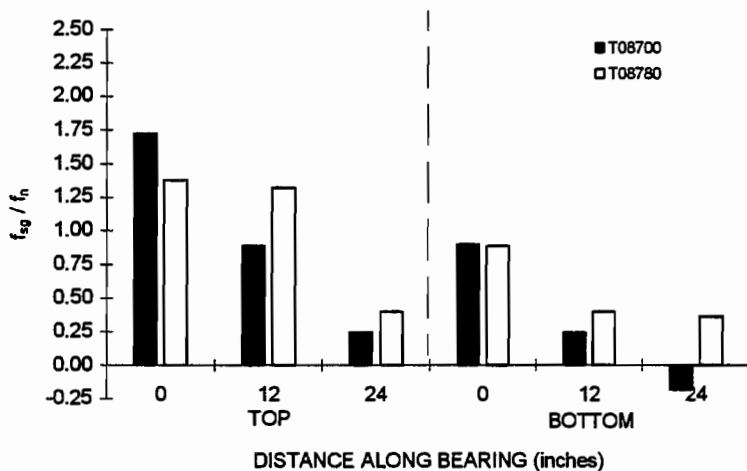
Figure 8-34 Average ratio of gage stress to nominal stress ( f_{sg} / f_n ), W12 x 87
