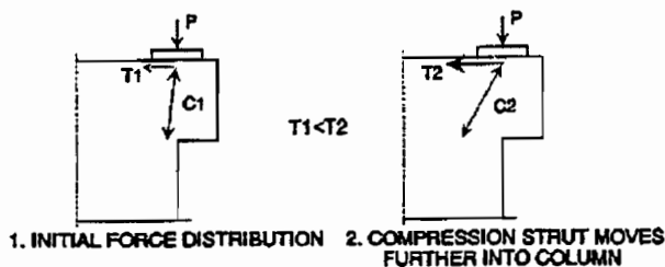
Figure 11- 19 Redirection of internal forces in the pier cap
