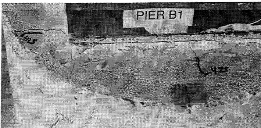
Figure 11- 21 Splitting cracks due to bond distress in Specimen B
