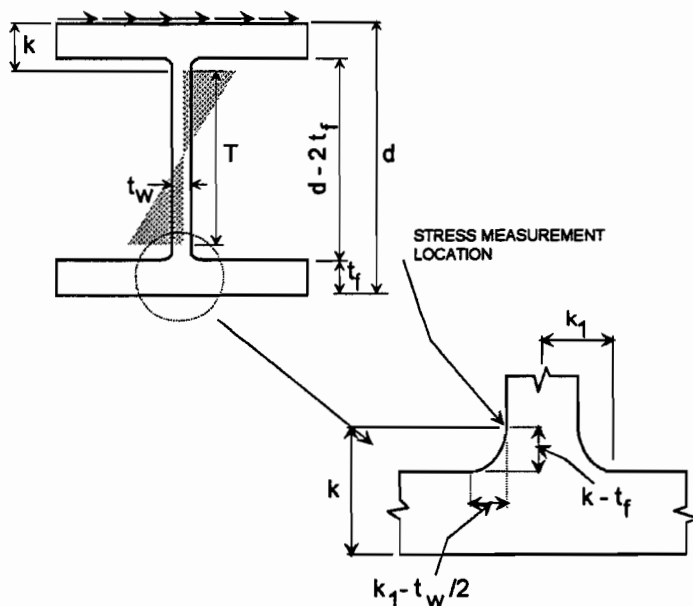
Figure 7-1 Location of maximum stress
