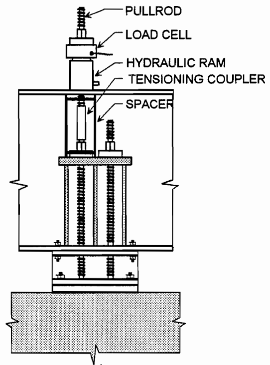
Figure 8-10 Tensioning assembly
