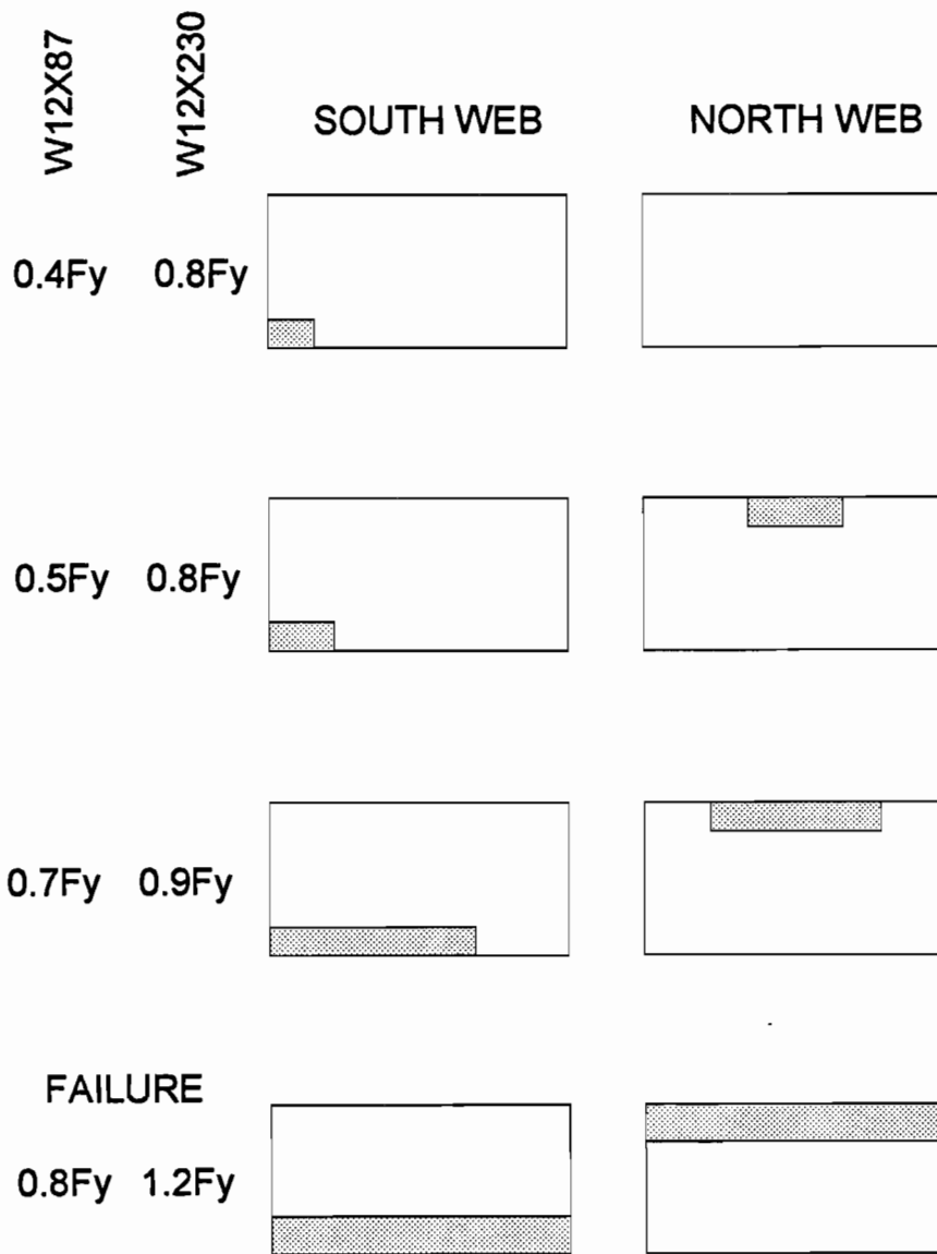
Figure 6-13 Progression of yield
