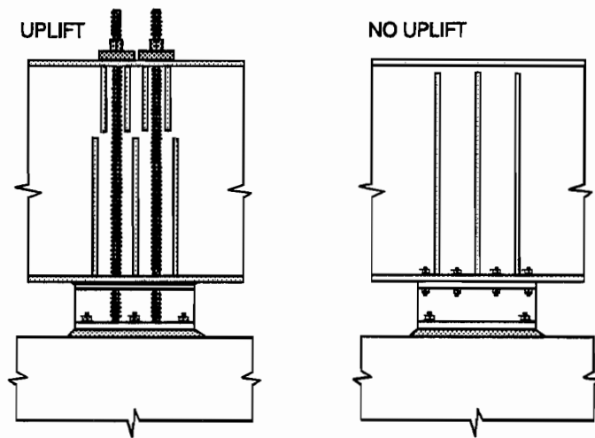
Figure 8-40 Recommended connection details
