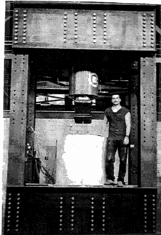
Figure 6-2 Test frame
