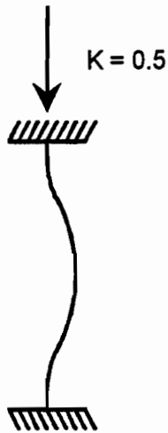
Figure 6- 4 Failure modes
