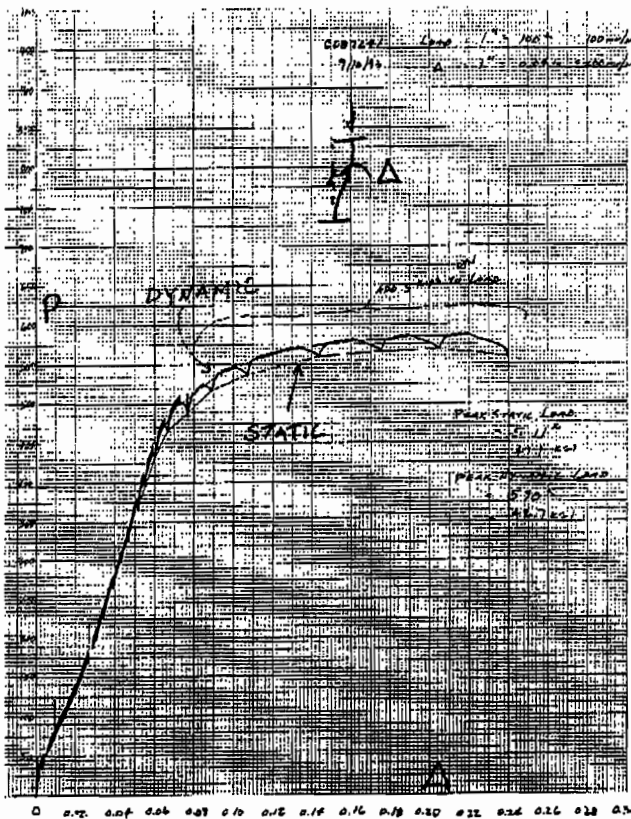
Figure 6-9 Typical load vs. lateral deflection curve
