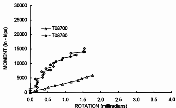
Figure 8- 25 Moment vs. rotation, transverse direction, W12 X 87
