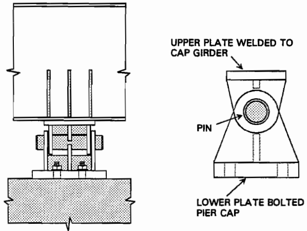
Figure 1-2 Steel bolster shoe
