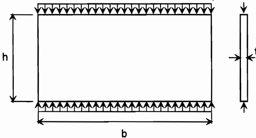
Figure 6-19 Plate under uniform edge compression
