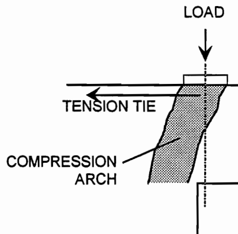
Figure 11-2 Arch action when the span/depth ratio < 1
