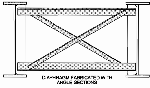
Figure 1-14 Typical diaphragm detail
