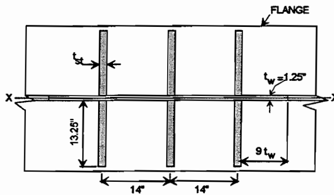
Figure A.4 Bearing Stiffener Properties
