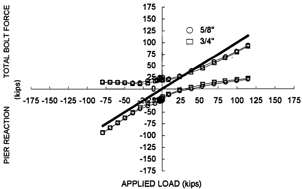
Figure 3- 12 Bolt group force, pier reaction vs. reaction force, neoprene pads
