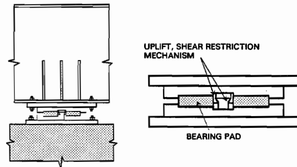
Figure 1-3 Pot bearing
