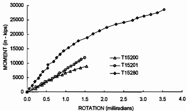
Figure 8- 26 Moment vs. rotation, transverse direction, W12 X 152
