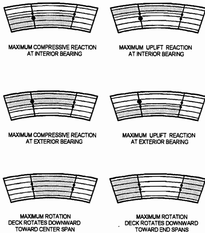
Figure 1-17 Influences surfaces for maximum bearing reactions
