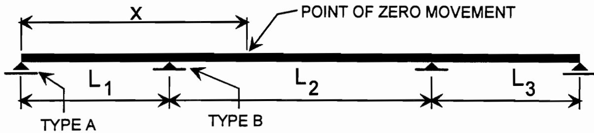
Figure 1- 10 Distribution of horizontal forces in continuous beam
