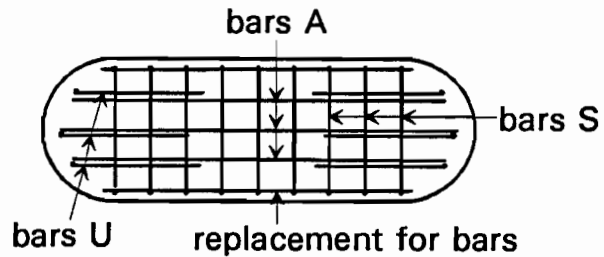
Figure 11-8 Top layer pier cap reinforcing in Specimen B
