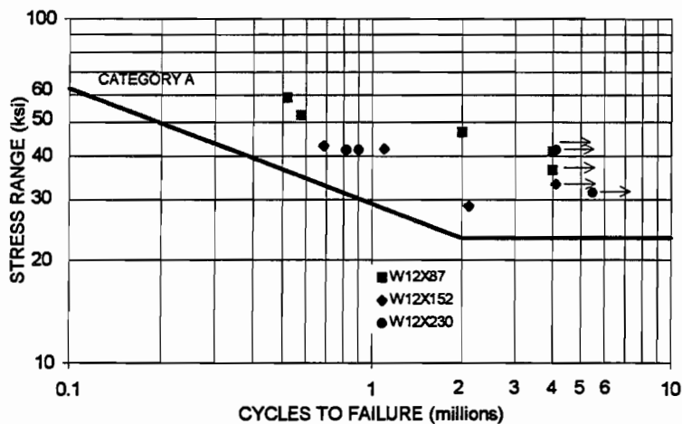
Figure 7-9 Stress range vs. number of cycles to failure
