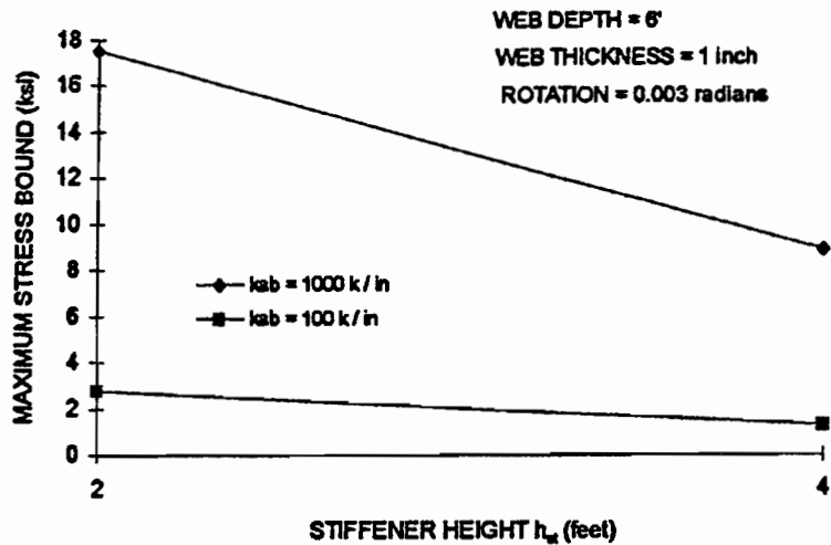
Figure 4- 12 Maximum stress bound vs. stiffener height
