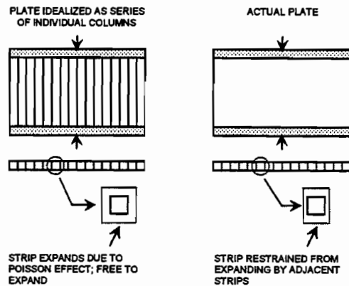
Figure 6-20 Poisson effect in plates
