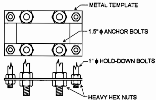
Figure 1- 20 Bolt anchorage
