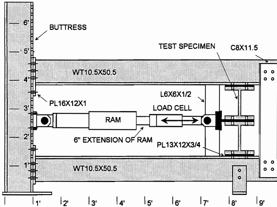
Figure 7-2 Schematic of test setup for symmetric specimens
