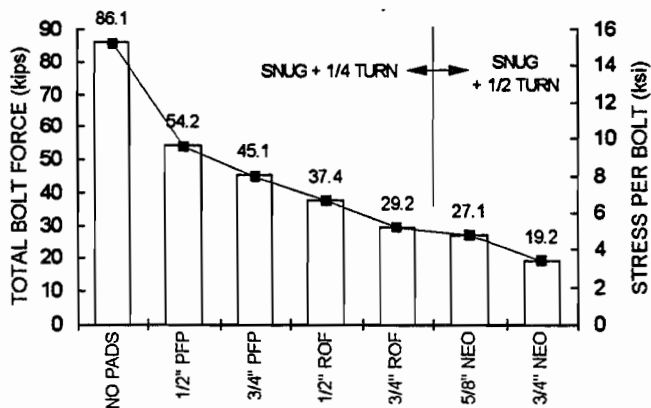
Figure 3- 1 Total pretension force as function of bearing pad
