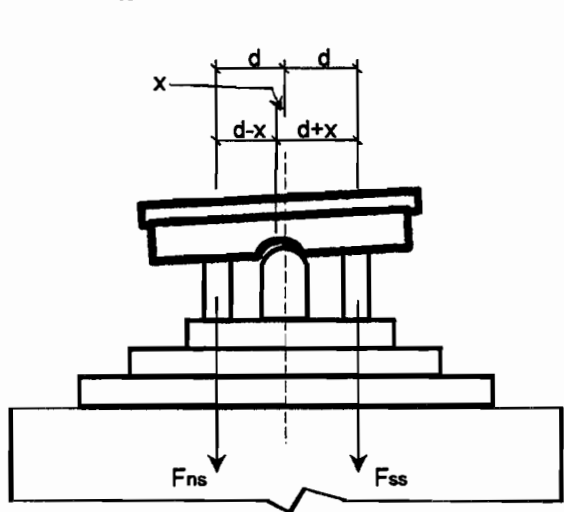
Figure 3- 17 Eccentricity of rotation
