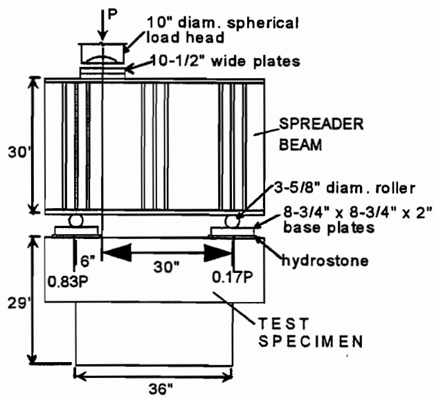
Figure 11- 11 Test set-up geometry.
