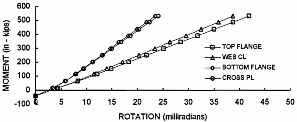
Figure 8-14 Moment vs. rotation, (1) anchor bolts, CoR = 0"
