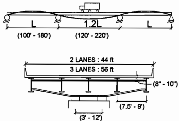
Figure 2-1 Design parameters
