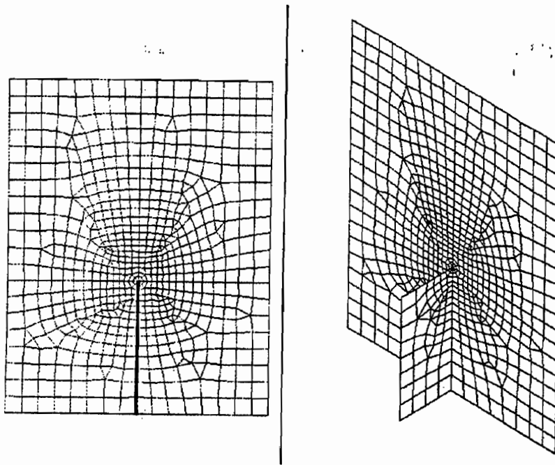
Figure 4-14 Refined finite element mesh
