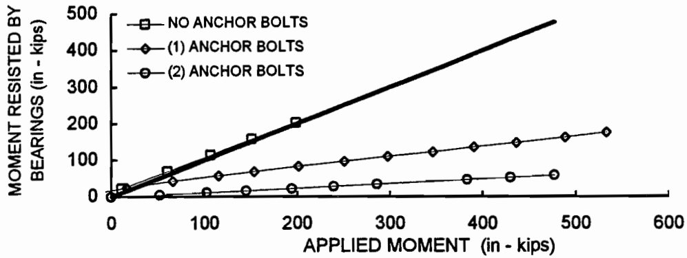
Figure 8-21 Moment in bearings vs. applied moment, CoR = 0"
