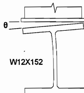
Figure 6-8 Flange out-of-straightness
