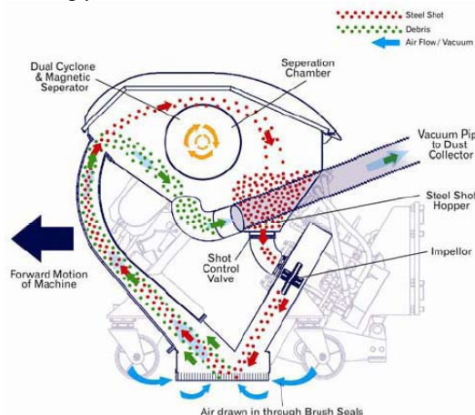
Typical Shotblasting Apparatus Process (TRB 09-0409 pg. 4)
