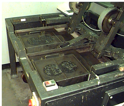
Figure 1. Hamburg Wheel Tracking Device
