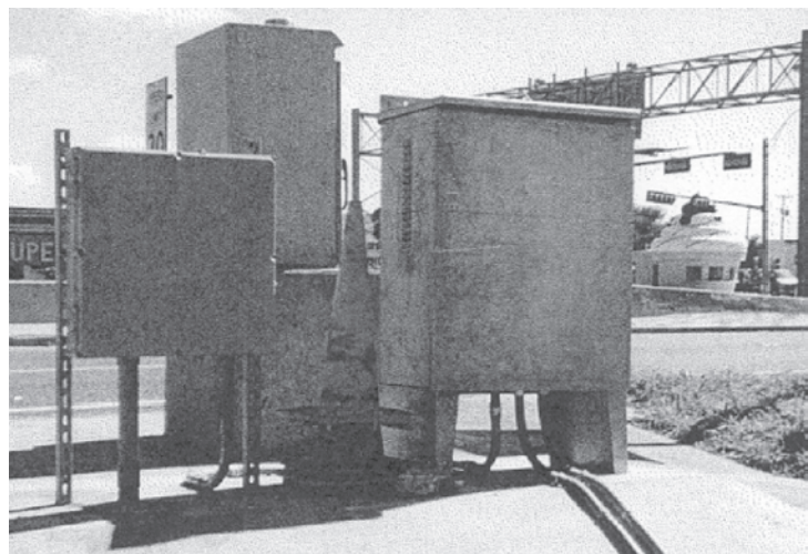
Figure 2 Remote monitoring unit (left) and rectifier (right) installations on Port Isabel shore for cathodic protection systems for the 19th through 23rd bents on QIC.
