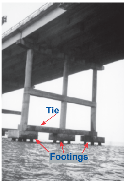
Figure 1 Typical bent showing footing and tie beams protected by CPS in this research.
