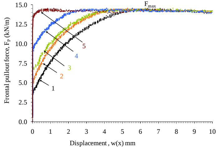
Figure 5.11: Frontal pullout force vs. displacement curve for each LVDT
