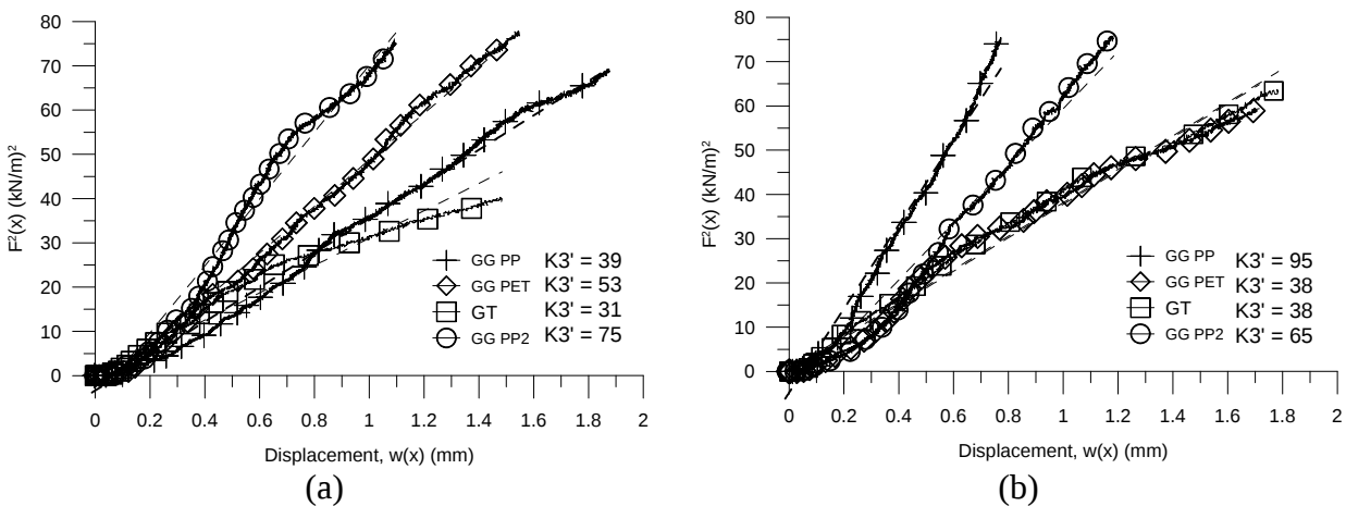
Figure 5.44: Comparison among the geosynthetic in gravel and confinement of 3 psi. Specimen orientation: (a) machine direction and (b) cross machine direction.
