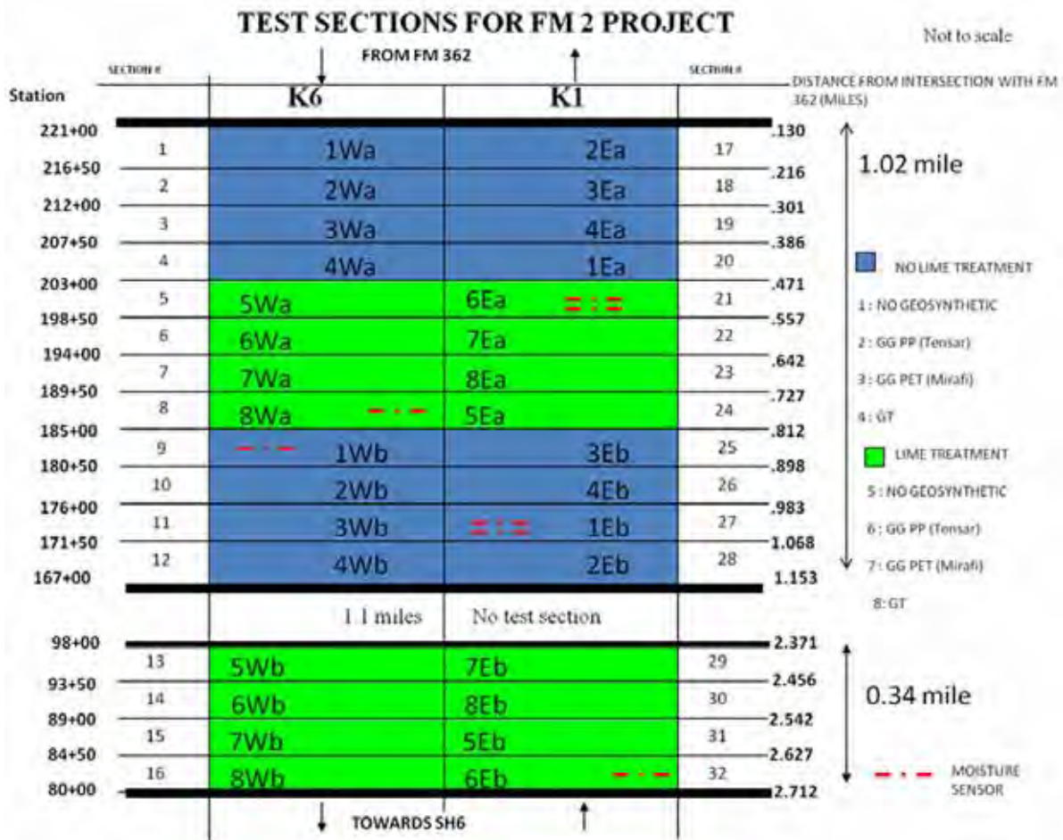
Note: GG PP = Polypropylene (PP) Geogrid (GG). GG PET = Polyester (PET) Geogrid (GG). GT = Geotextile. Figure 6.2: Experimental test sections at FM2 Road. (a) Section Profiles. (b) Location of sections.
