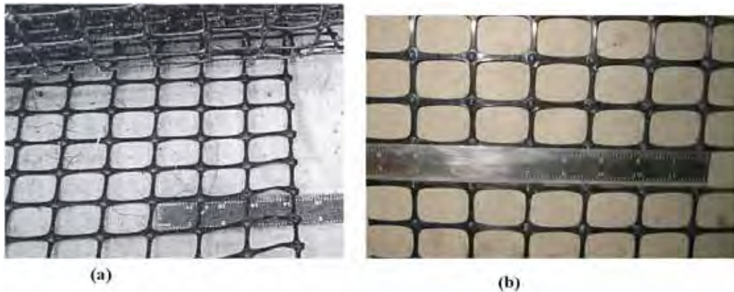
Figure 5.8: Geogrids: (a) Tensar BX-1100 (G1); (b) Tensar BX 1200 (G4) (adapted from Finnefrock, 2008)
