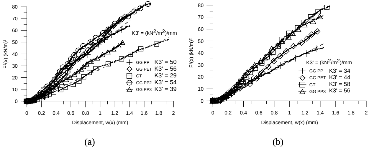
Figure 5.43: Comparison of the geosynthetic confined in sand and 3 psi. Specimen orientation: (a) machine direction and (b) cross machine direction.
