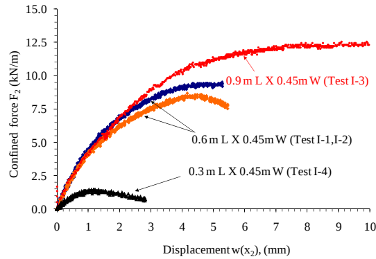
Figure 5.22: Confined force vs. displacement for Tests I-1, I-2, I-3 and I-4 at point x_2
