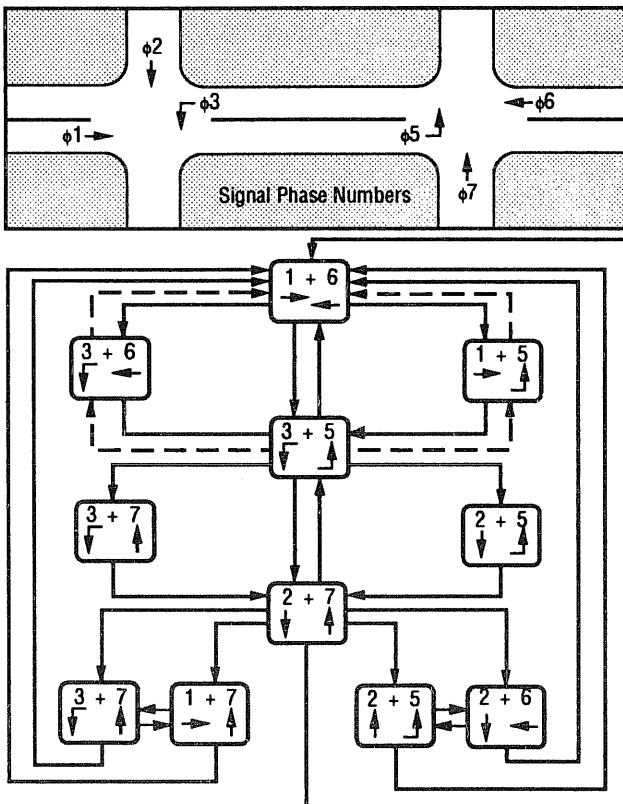
Fig 2-3. Operation of the "Figure 3" signal controller pattern.
