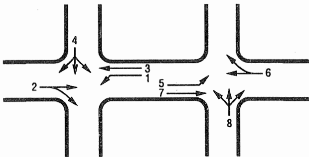
Fig 2-7. Type "170" diamond controller phase arrangement.
