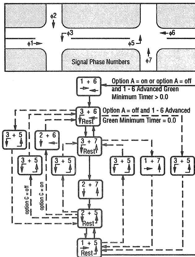
Fig 2-5. Operation of the "Figure 7" signal controller pattern.
