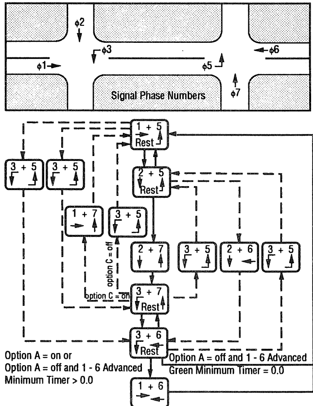
Fig 2-4. Operation of the "Figure 6" signal controller pattern.
