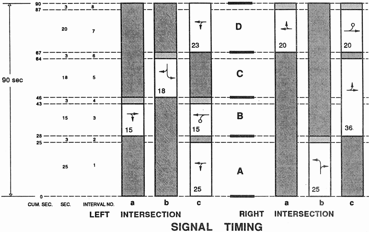
Figure C-3. Compact Diamond, 4-Phase Pretimed Signal Control. (Example 5).
