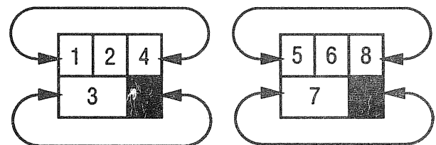
Dual/Dual-Ring Arrangement of "Type 170" Controller Phases
