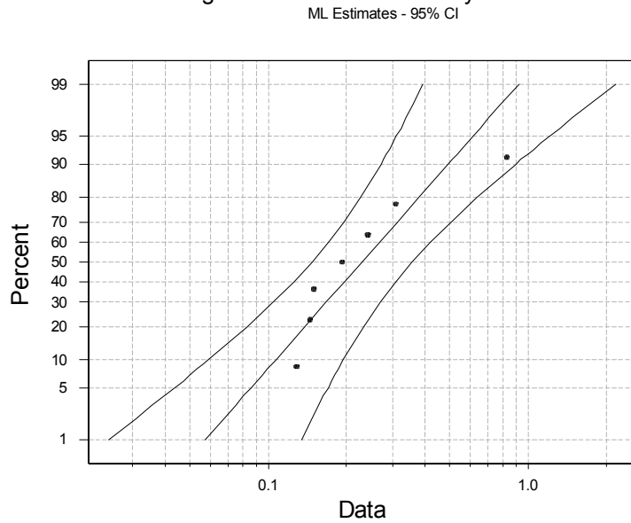
Lognormal base e Probability Plot for TP
