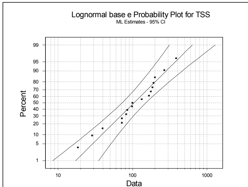
Figure 3-1: Probability Plot for Total Suspended Solids (mg/L)
