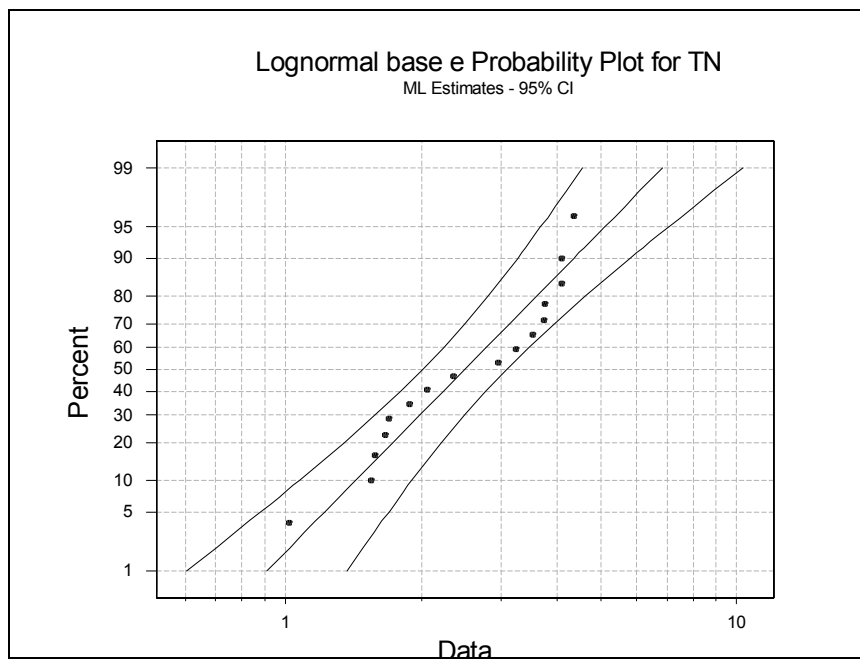
Figure 3-8: Probability Plot for Total Nitrogen (mg/L)
