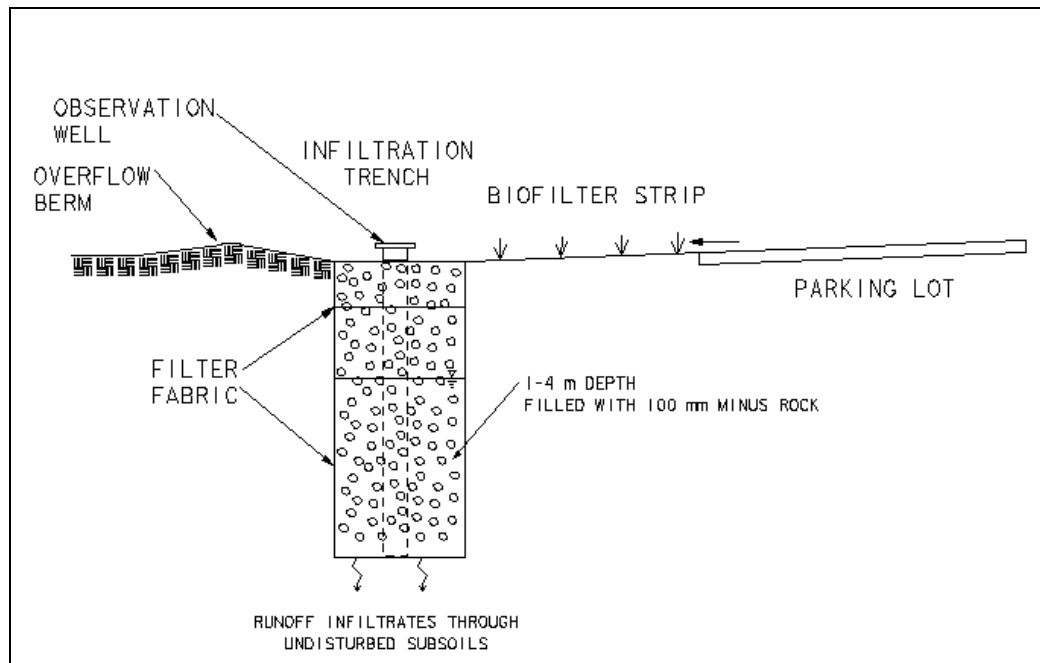
Figure 4-8: Schematic of an Infiltration Trench (Caltrans, 2003a)
