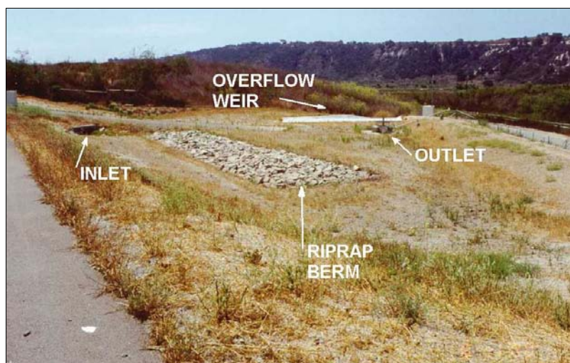
Figure 4-3: Unlined Extended Detention Basin (Caltrans, 2003a)
