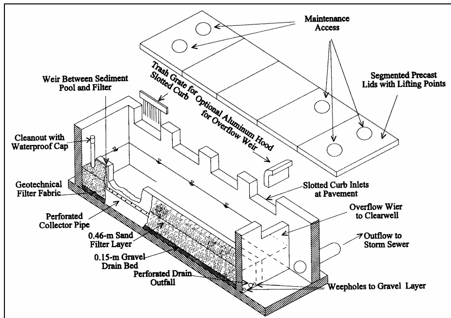
Figure 4-2: Schematic of a Delaware Sand Filter (Caltrans, 2003a)
