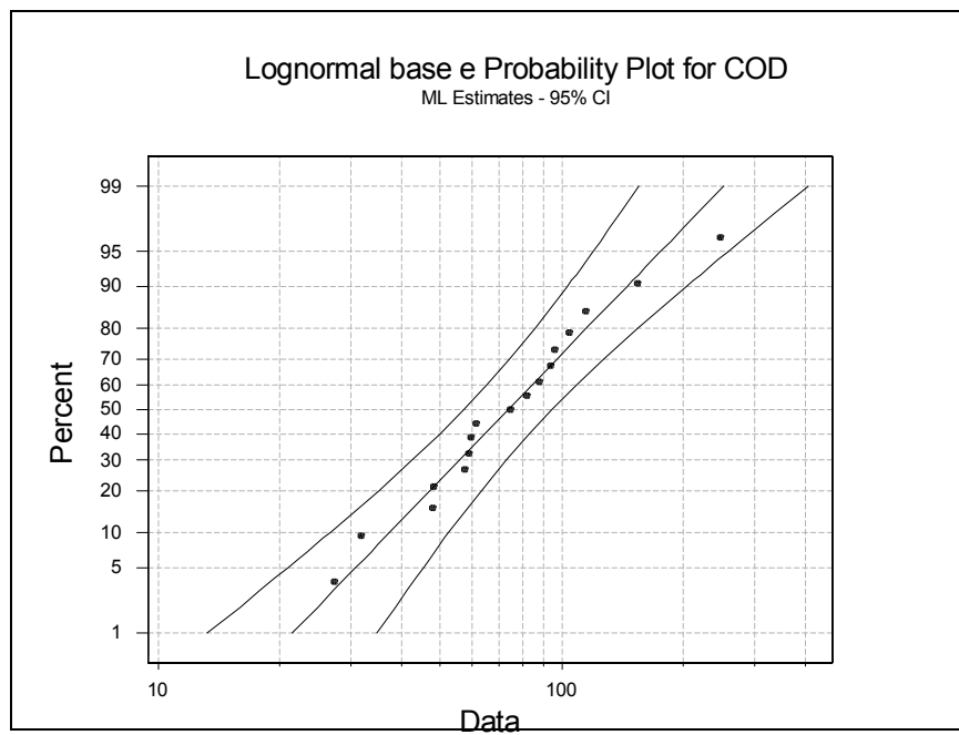
Figure 3-4: Probability Plot for Chemical Oxygen Demand (mg/L)
