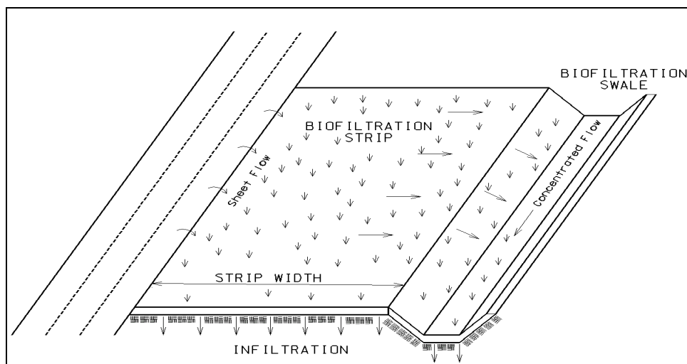
Figure 4-11: Schematic of a Vegetated Buffer Strip (Caltrans, 2003a)
