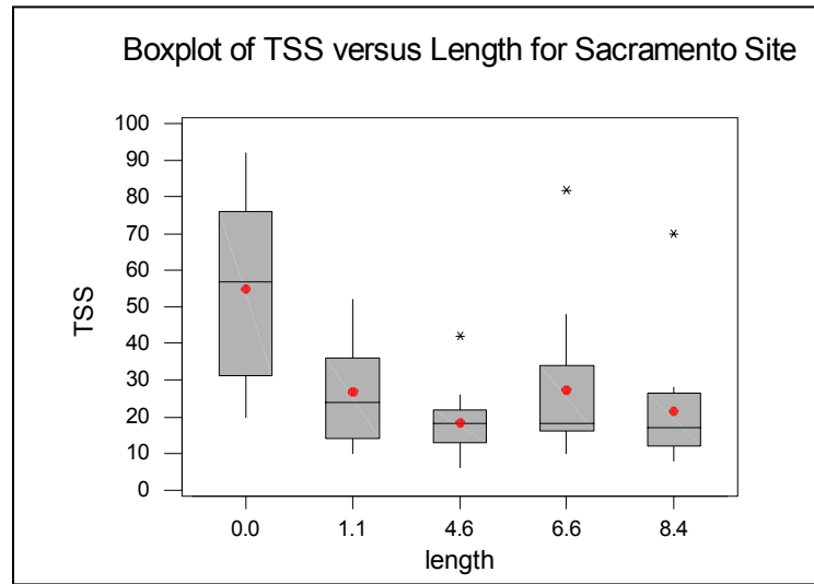
Figure 5-5: Boxplot showing the Effectiveness of the Biofiltration Strip in the California Study
