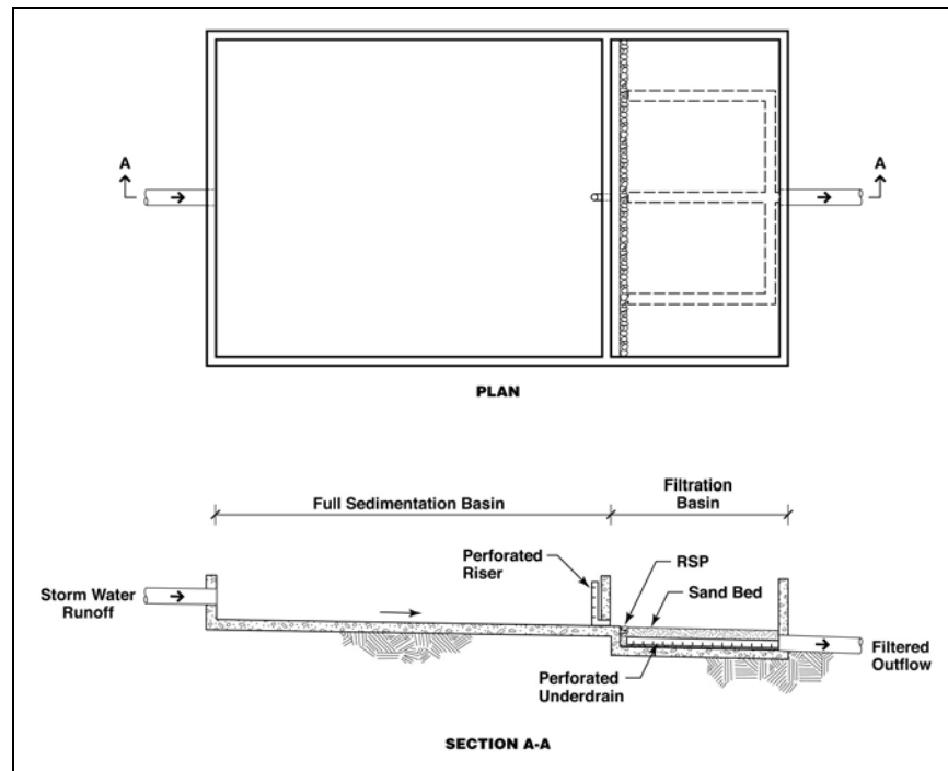
Figure 4-1: Schematic of an Austin Sand Filter (Caltrans, 2003a)
