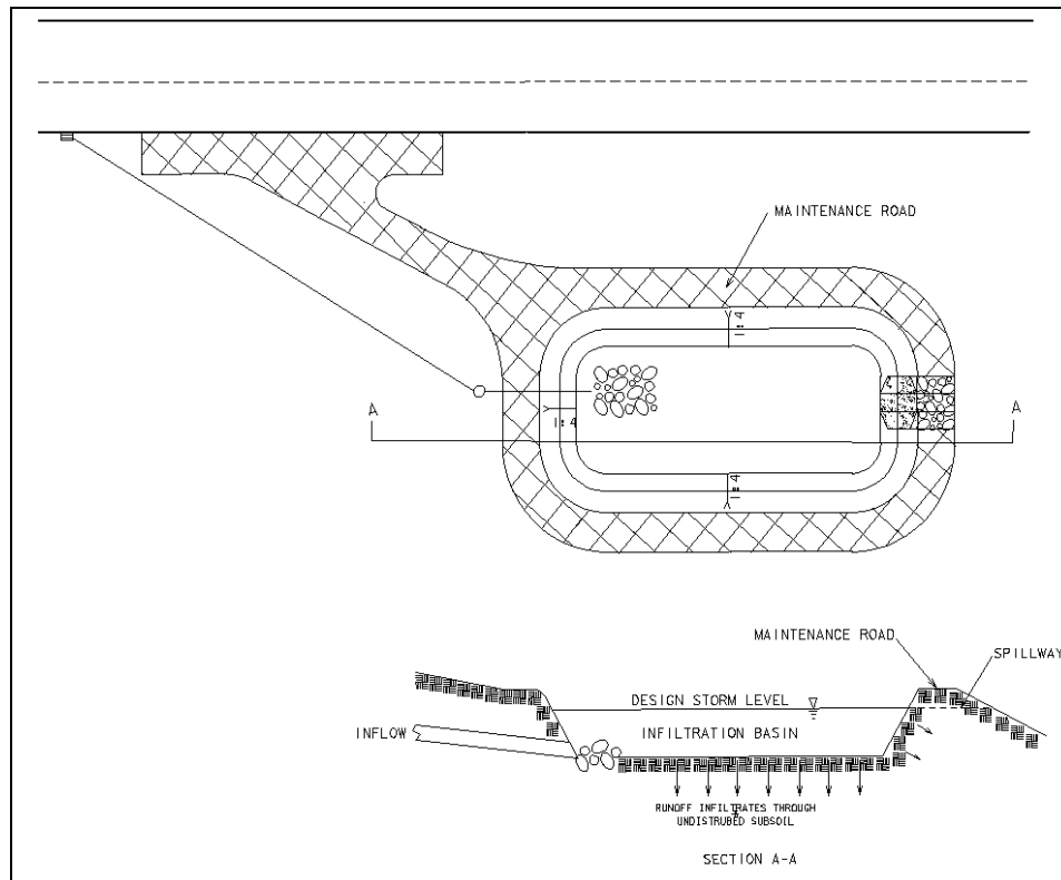
Figure 4-6: Schematic of an Infiltration Basin (Caltrans, 2003a)
