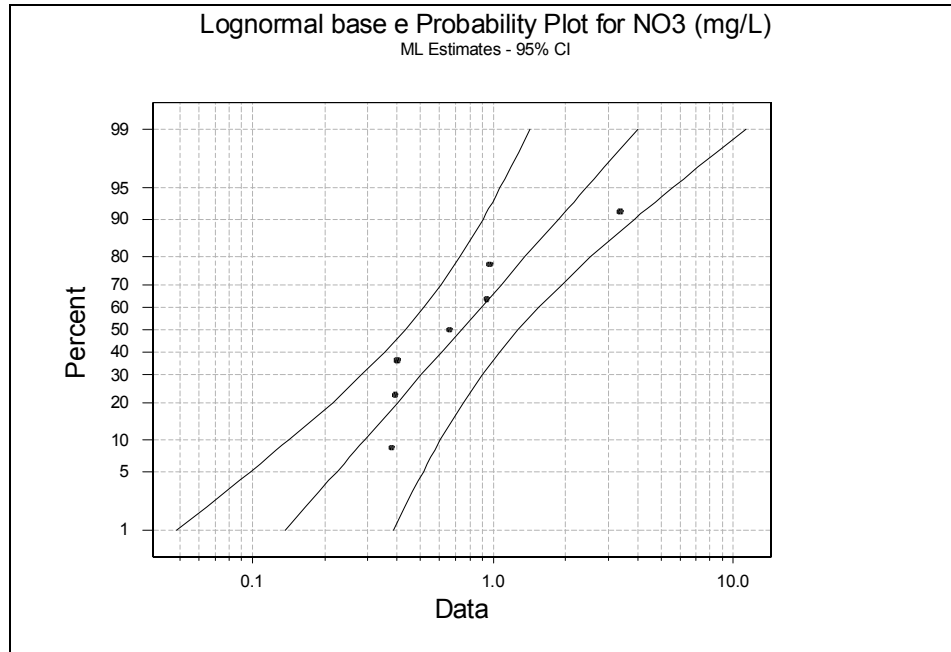
Figure 5-2: Probability Plot of Vegetated Area Effluent Water Quality for Nitrate (mg/L)
