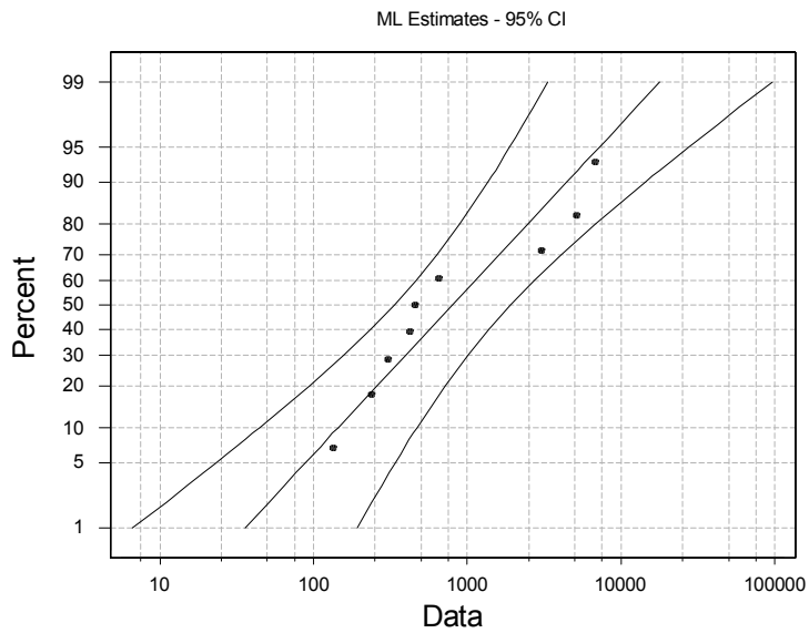
Lognormal base e Probability Plot for Fecal Coliform (CFU/100mL)
