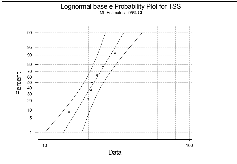
Figure 5-4: Probability Plot of Vegetated Area Effluent Water Quality for Total Suspended Solids (mg/L)
