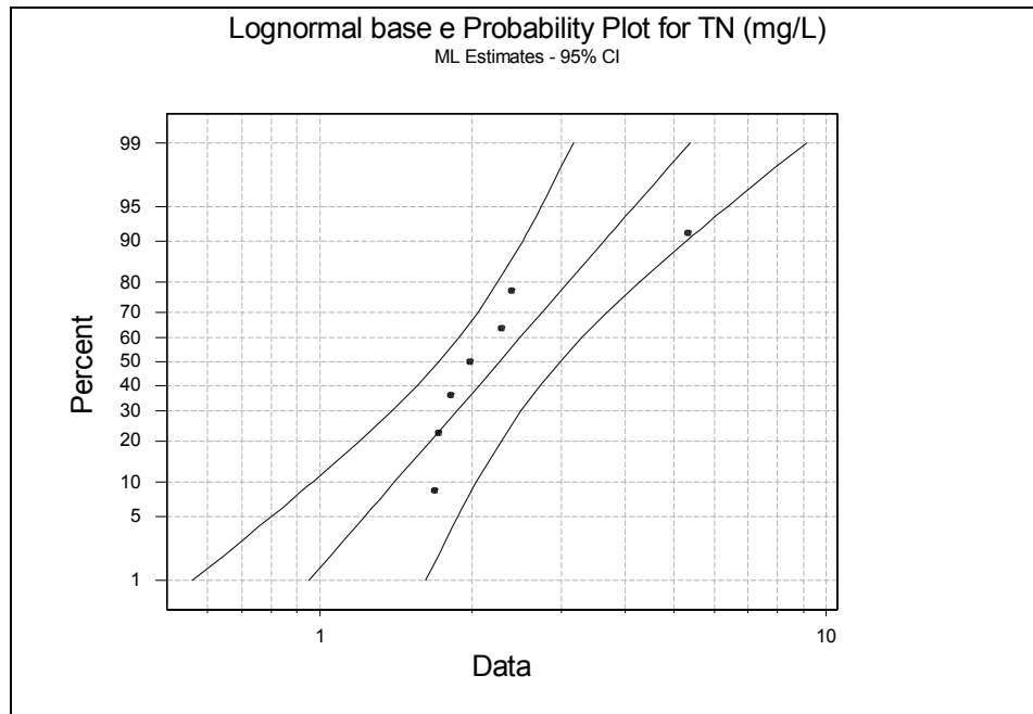
Figure 5-3: Probability Plot of Vegetated Area Effluent Water Quality for Total Nitrogen (mg/L)
