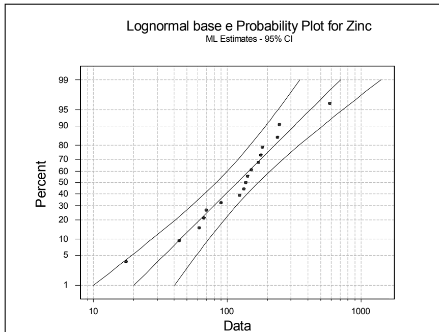
Figure 3-9 Probability Plot for Zinc ( \mu\text{g/L} )
