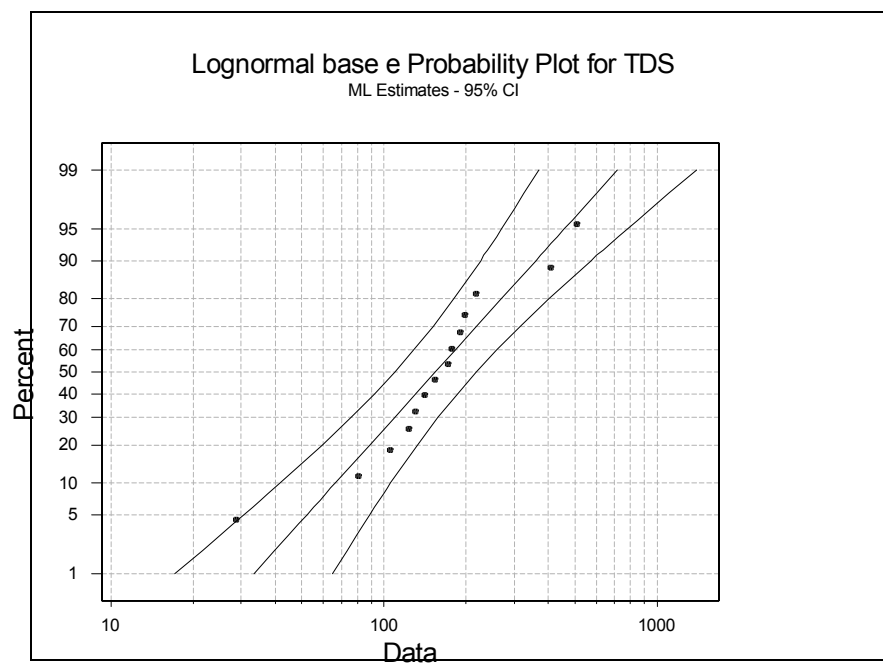
Figure 3-2: Probability Plot for Total Dissolved Solids (mg/L)
