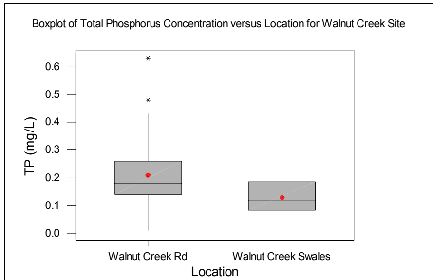
Figure 5-8: Comparison of Total Phosphorus Concentration for Edge of Pavement and Grassed Swale Effluent for Walnut Creek Site in Texas
