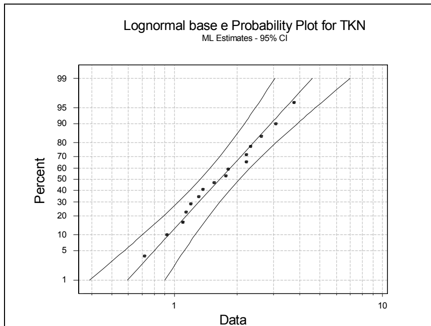
Figure 3-7: Probability Plot for Total Kjeldahl Nitrogen (mg/L)
