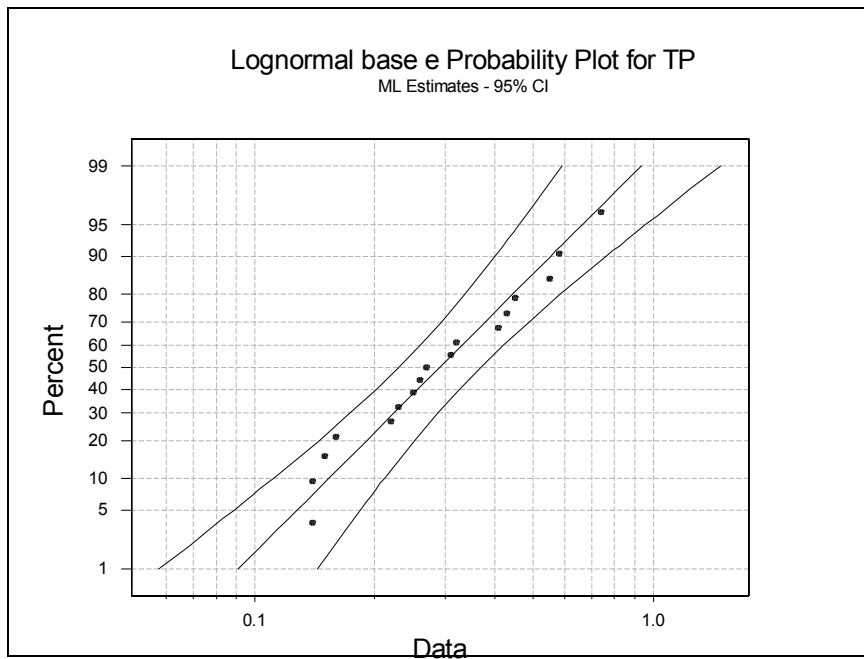
Figure 3-6: Probability Plot for Total Phosphorus (mg/L)
