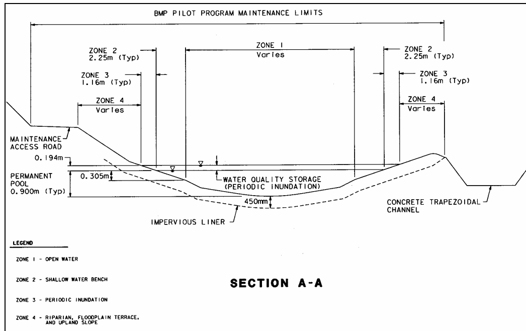
Figure 4-5: Schematic of the Cross-Section of a Wet Basin (Caltrans, 2003a)
