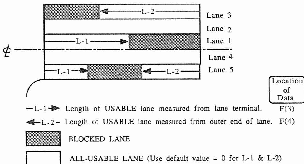
Figure 4. Partially-blocked lane configurations
