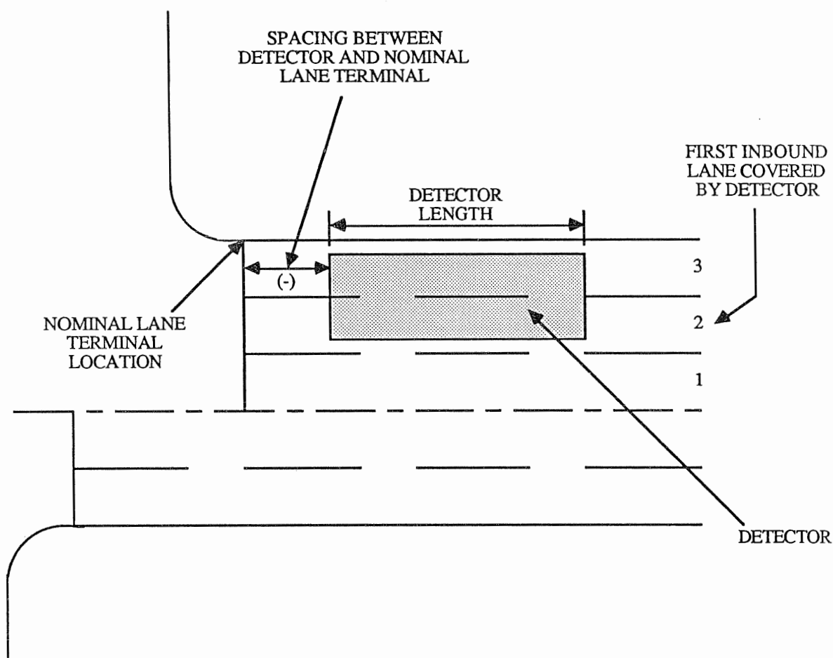
Figure 11. Nomenclature for detector placement.
