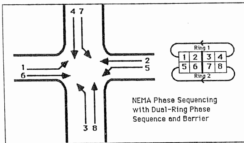
Figure 10. Traffic (NEMA) phases.
