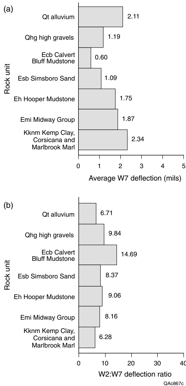
Figure 28. (a) Average W7 deflection and (b) W2:W7 deflection ratio by rock type along Texas 71, Bastrop County.
