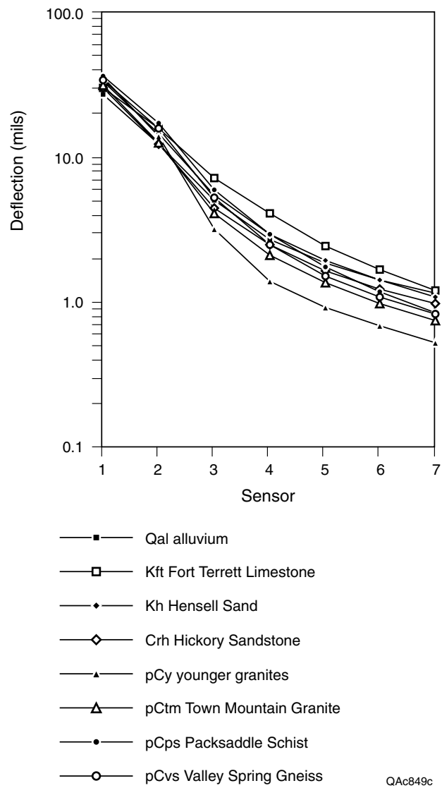
Figure 15. Average deflections for all rock units mapped along Texas 16 in Llano and Gillespie Counties.
