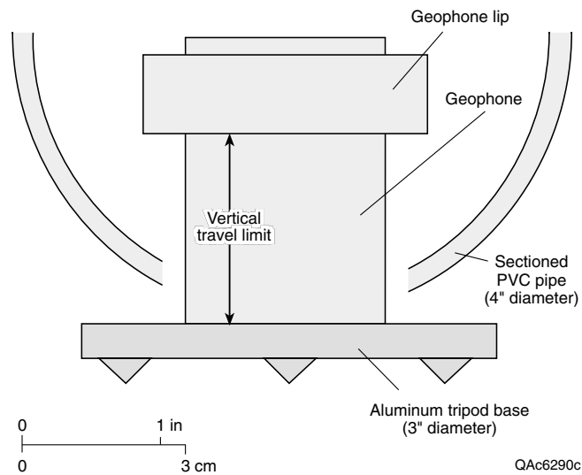
Figure 57. Cross section of recording array showing one geophone installed through PVC pipe rail and resting on aluminum tripod base. Surface irregularities can be accommodated by free vertical movement of the geophone between the tripod base and geophone lip.
