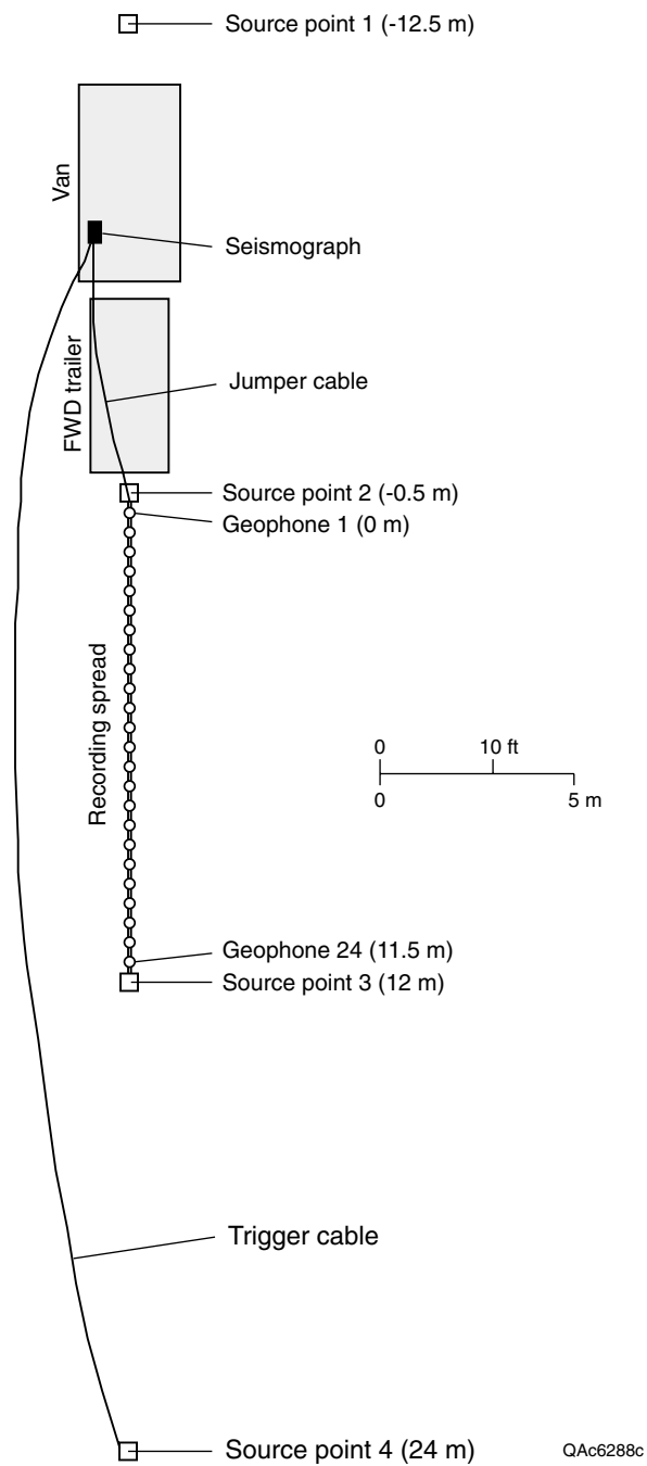
Figure 53. Schematic layout of the Seismic Refraction Bedrock Analyzer as deployed on pavement behind a Falling-Weight Deflectometer trailer.
