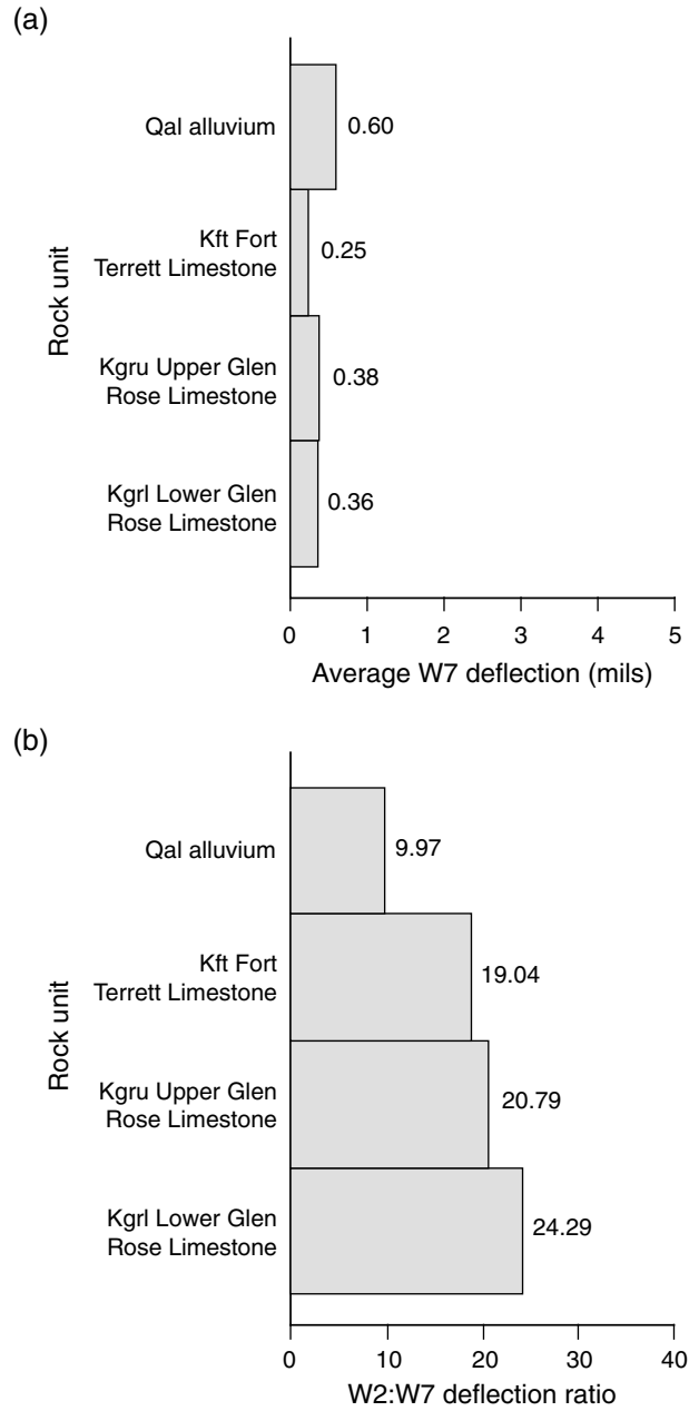
Figure 24. (a) Average W 7 deflection and (b) W 2: W 7 deflection ratio by rock type along U.S. 290, Blanco and Hays Counties.
