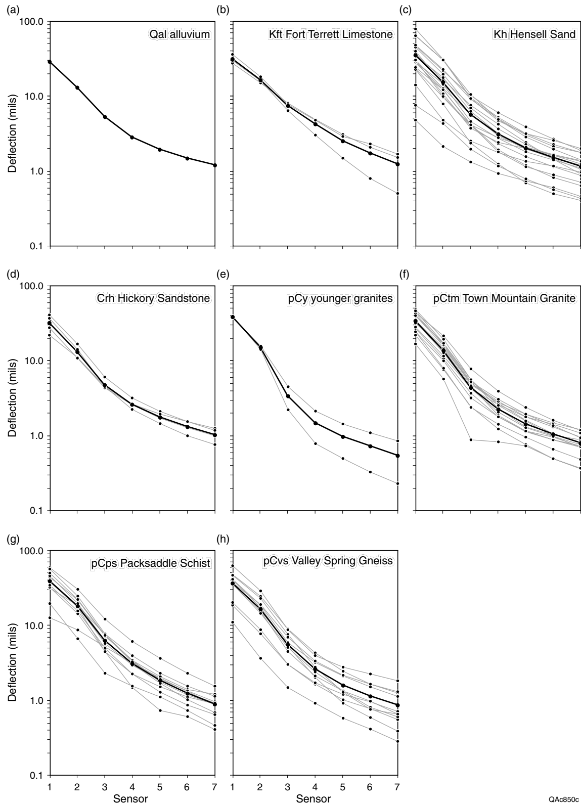
Figure 14. Average and individual deflections for rock types mapped along Texas 16 in Llano and Gillespie Counties.
