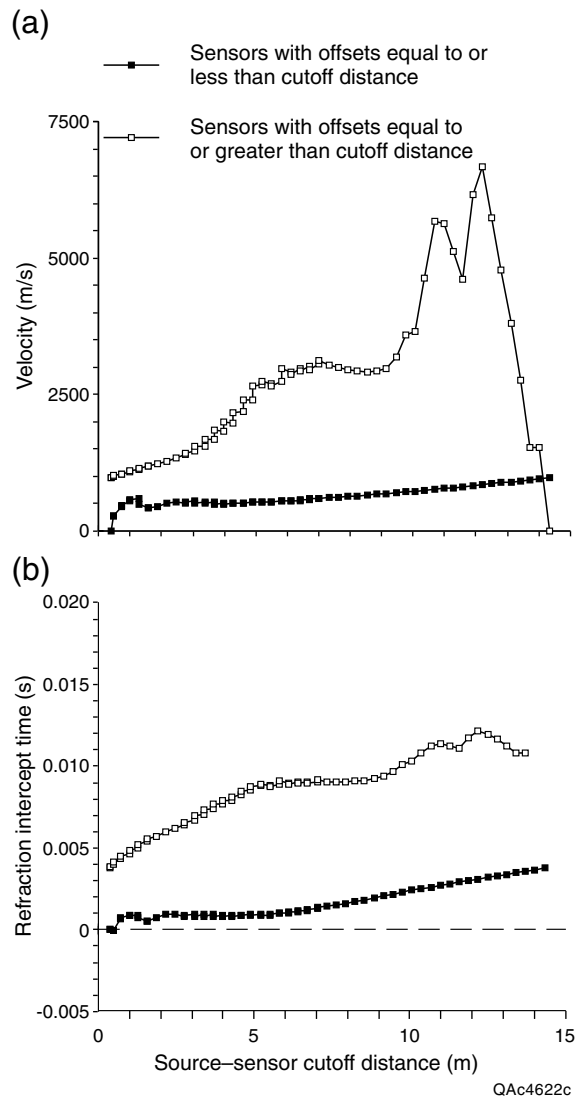
Figure 38. (a) Apparent velocity and (b) zero-offset time for reverse data from refraction test PRC SPH1. Velocities and intercepts calculated by assigning arrivals from various offset ranges to the direct or refracted arrival.
