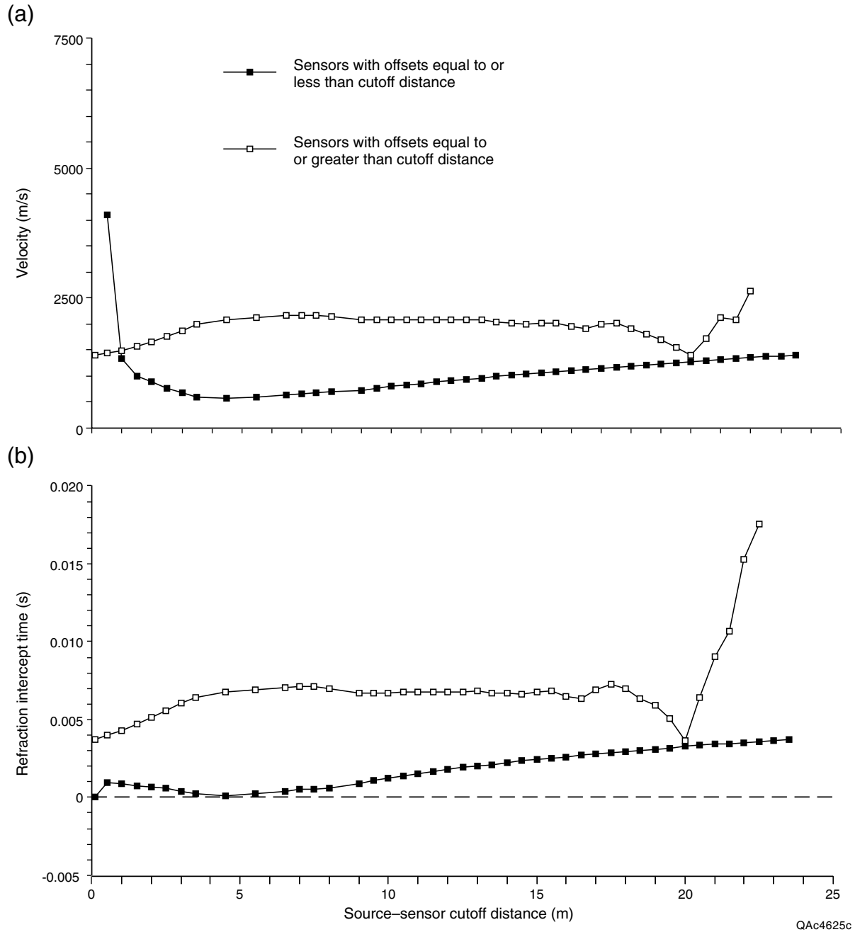
Figure 47. (a) Velocity and (b) intercept plots for forward data from refraction test Jacksboro SPH1. Velocities and intercepts calculated by assigning arrivals from various offset ranges to the direct or refracted arrival.
