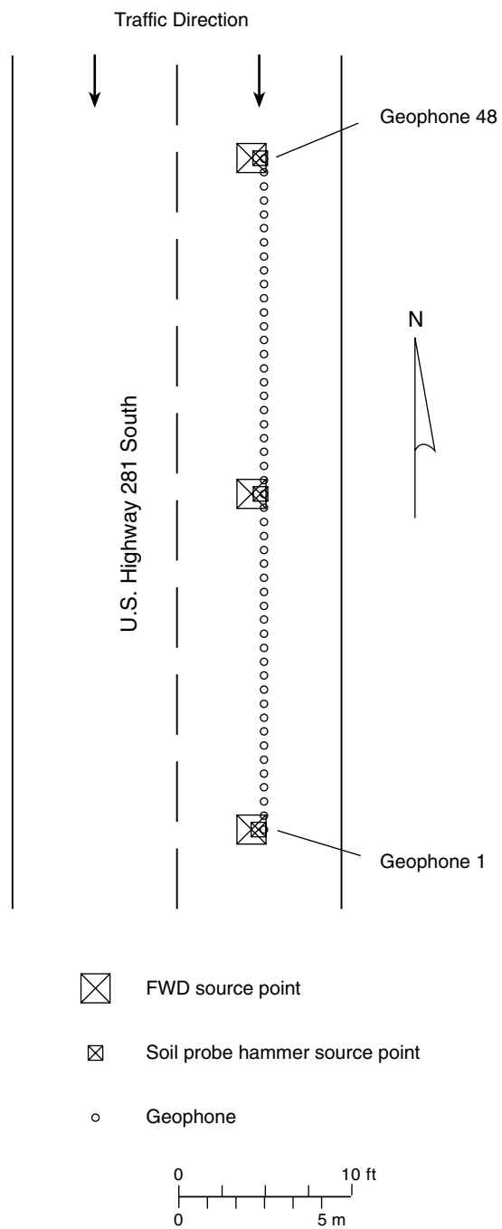
Figure 8. Map of the seismic-refraction test site on southbound U.S. Highway 281 at the Texas Department of Transportation's Mobile Load Simulator site south of Jacksboro, Texas.
