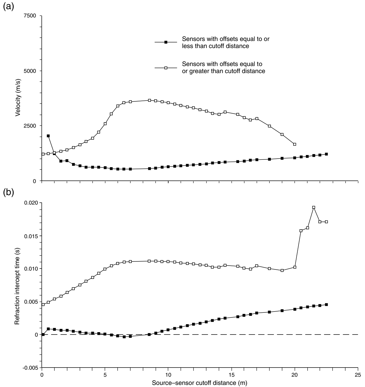
Figure 48. (a) Velocity and (b) intercept plots for reverse data from refraction test Jacksboro SPH1. Velocities and intercepts calculated by assigning arrivals from various offset ranges to the direct or refracted arrival.
