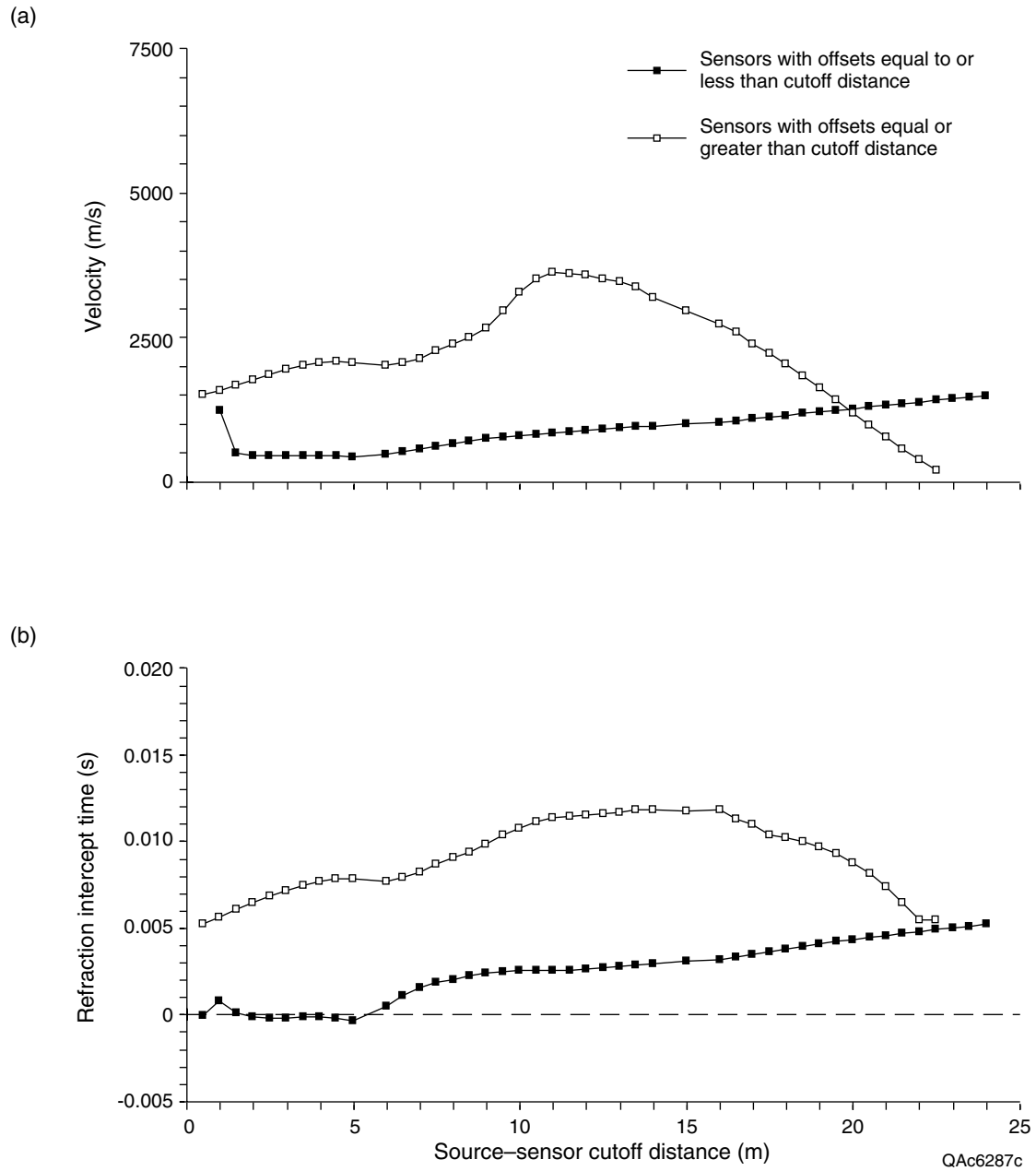
Figure 52. (a) Velocity and (b) intercept plots for reverse data from the Granite Shoals refraction test. Velocities and intercepts calculated by assigning arrivals from various offset ranges to the direct or refracted arrival.
