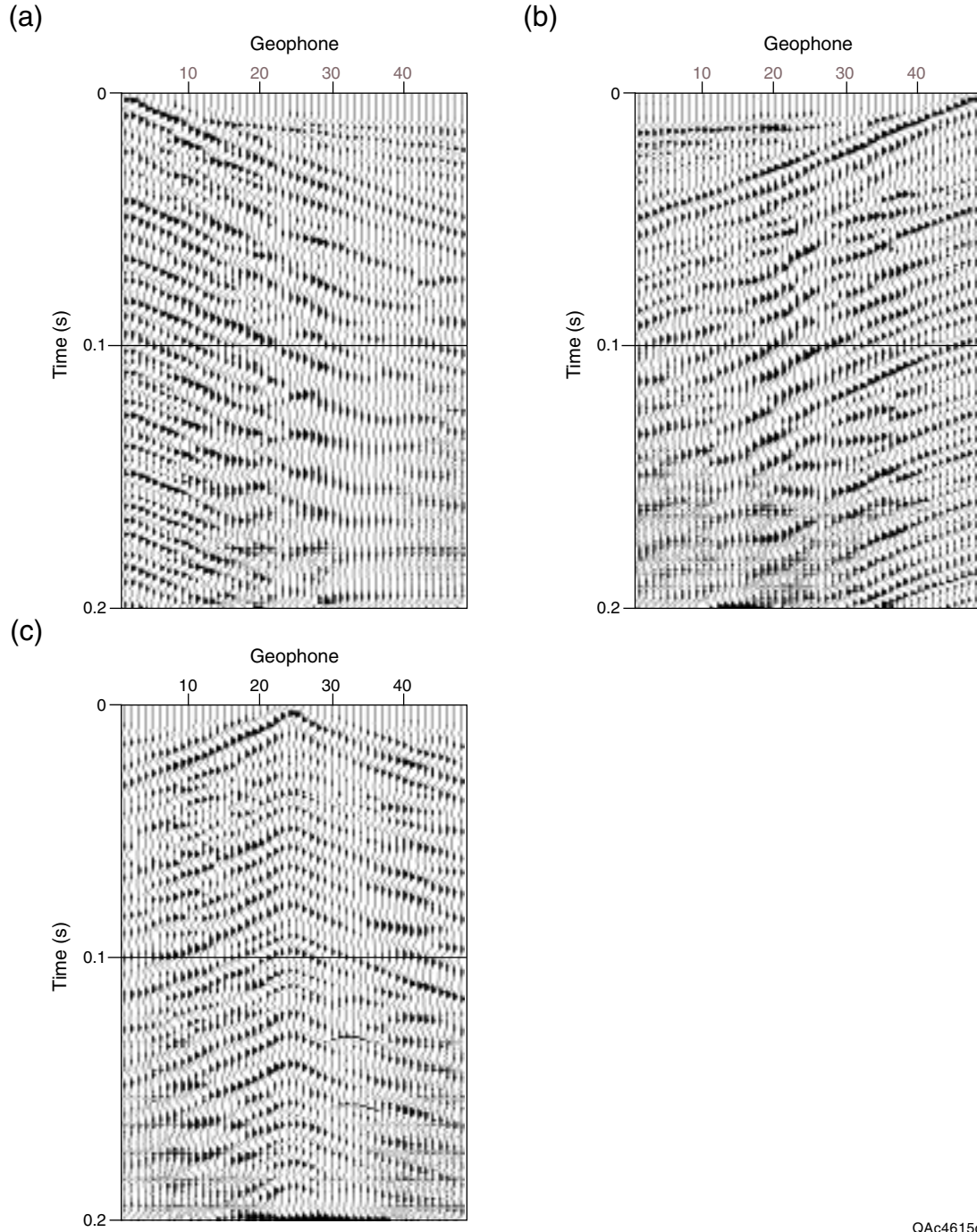
Figure 40. Field records from refraction test PRC SPH2 (site R1, fig. 2) using a soil-probe hammer as a seismic source. Source was located on the pavement of Road D at the (a) west end, (b) east end, and (c) center of the recording spread. Records displayed with a 125-Hz low-cut filter and time-varying gain (20-ms window) applied. Geophone spacing is 0.3 m.
