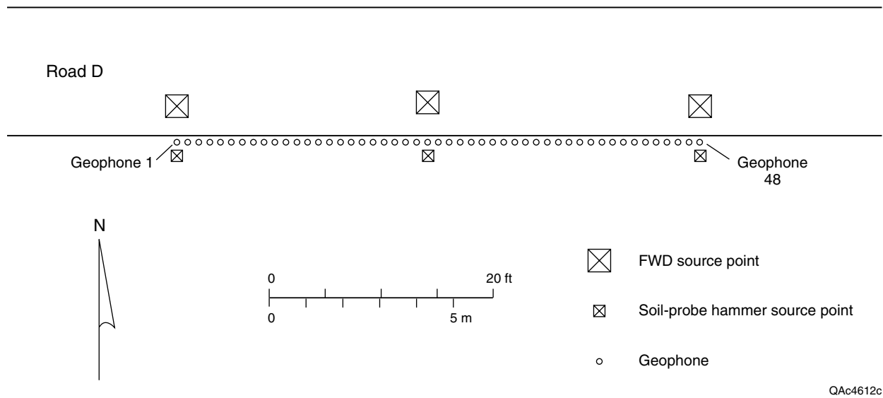
Figure 6. Map of the seismic-refraction test site along Road D at the J. J. Pickle Research Campus, The University of Texas at Austin.
