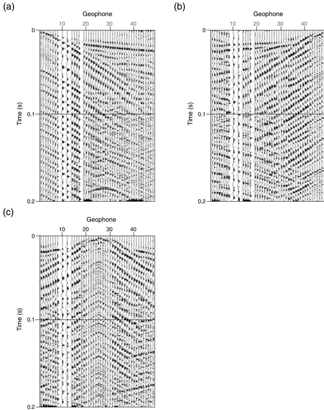
Figure 45. Field records from refraction test Jacksboro SPH1 using a soil-probe hammer as a seismic source. Source and geophones were located on the pavement of U.S. Highway 281. Source was at the (a) south end, (b) north end, and (c) center of the recording spread. Records displayed with a 125-Hz low-cut filter and time-varying gain (20-ms window) applied. Geophone spacing is 0.5 m.
