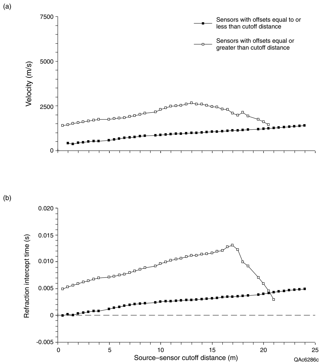
Figure 51. (a) Velocity and (b) intercept plots for forward data from the Granite Shoals refraction test. Velocities and intercepts calculated by assigning arrivals from various offset ranges to the direct or refracted arrival.
