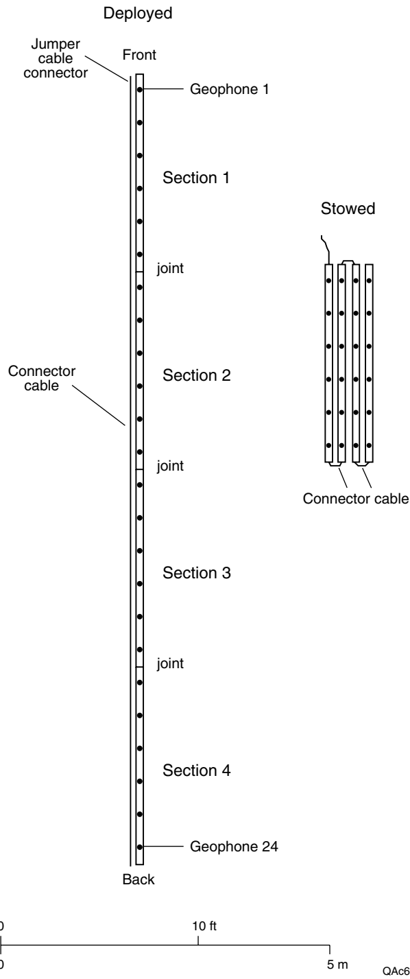
Figure 55. Schematic of recording array (left) as deployed and (right) folded for transport.
