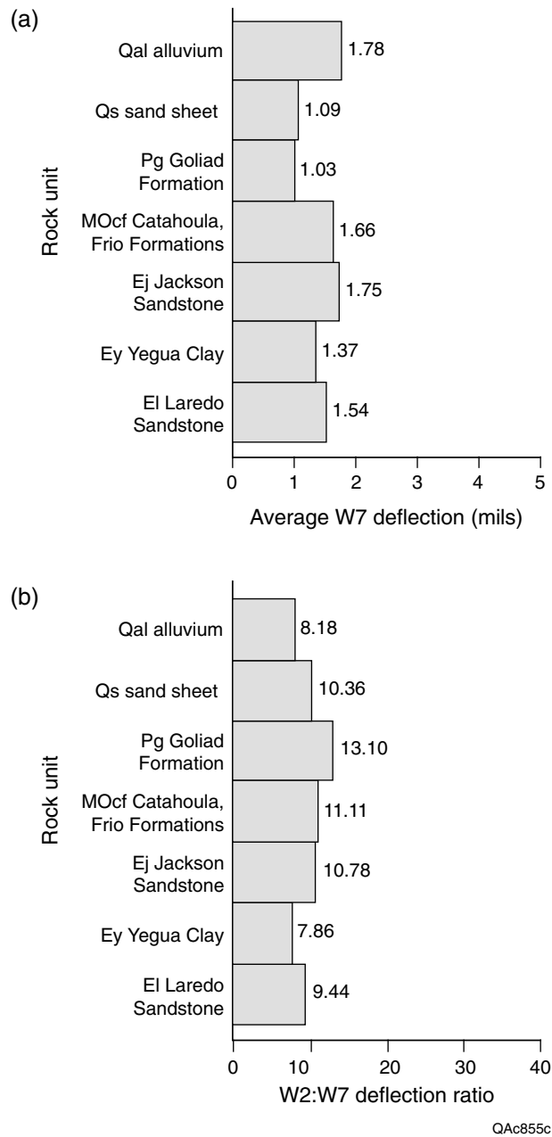
Figure 32. (a) Average W7 deflection and (b) W2:W7 deflection ratio by rock type along Texas 16, Llano and Gillespie Counties.
