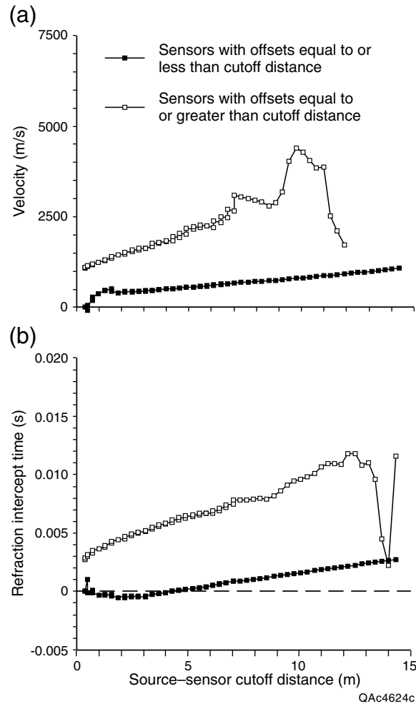
Figure 43. (a) Apparent velocity and (b) zero-offset time for reverse data from refraction test PRC SPH2. Velocities and intercepts calculated by assigning arrivals from various offset ranges to the direct or refracted arrival.
