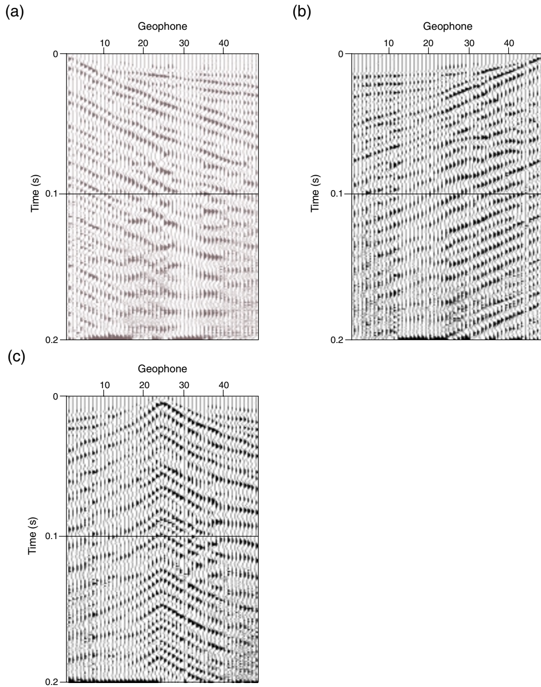
Figure 35. Field records from refraction test PRC SPH1 (site R1, fig. 2) using a soil-probe hammer as a seismic source. Source was located on the shoulder of Road D at the (a) west end, (b) east end, and (c) center of the recording spread. Records displayed with a 125-Hz low-cut filter and time-varying gain (20-ms window) applied. Geophone spacing is 0.3 m.
