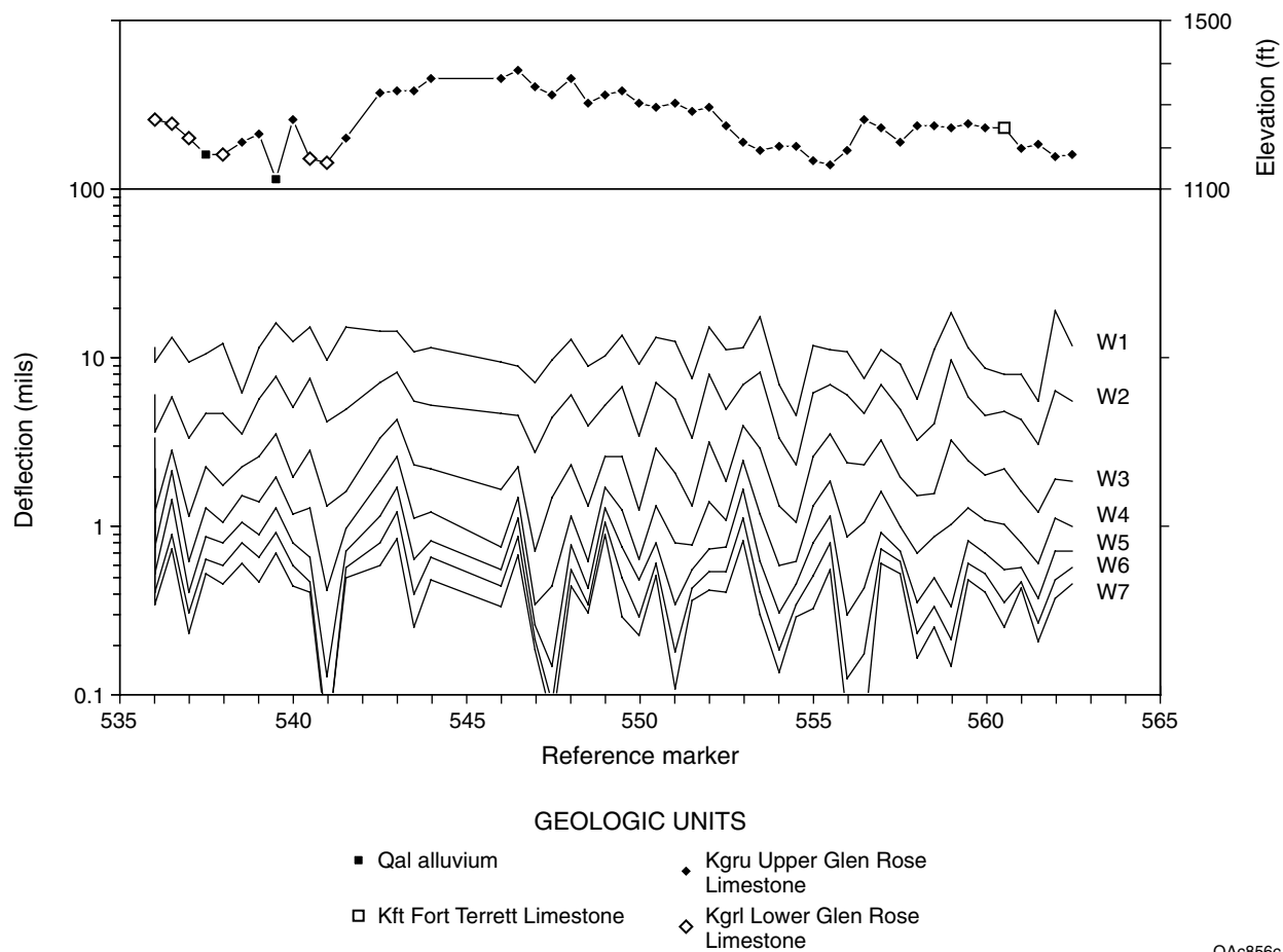
Figure 21. Geologic units, elevation, and W1 through W7 deflections along U.S. 290 between reference markers 536 and 563, Blanco and Hays Counties, Central Texas.
