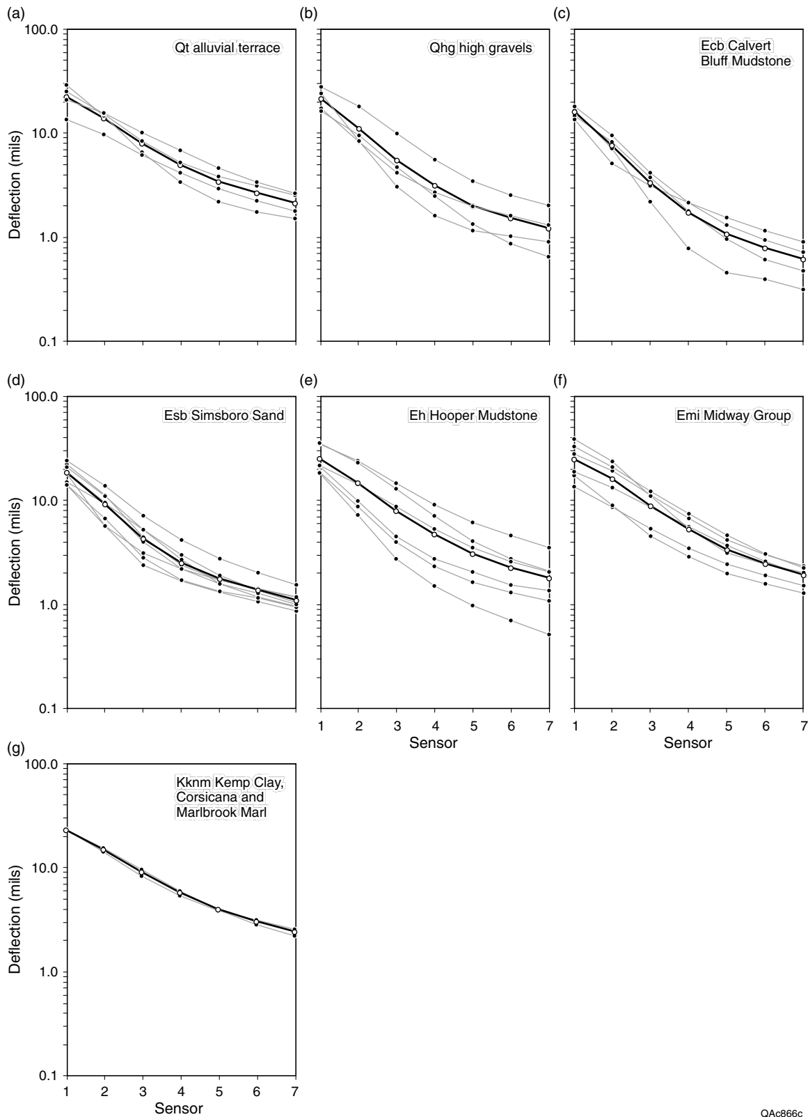
Figure 26. Average and individual deflections for rock types mapped along Texas 71 in Bastrop County.
