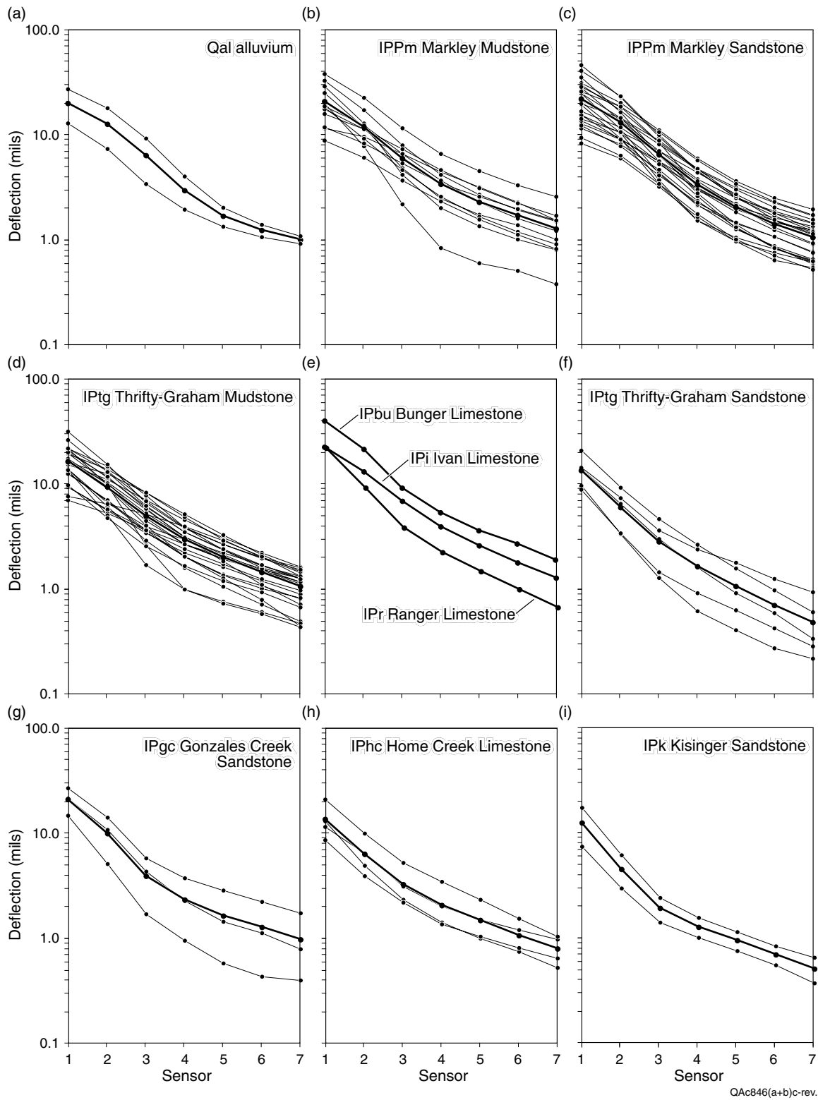
Figure 10. Average and individual deflections for rock types mapped along Texas 16 in Archer and Young Counties.
