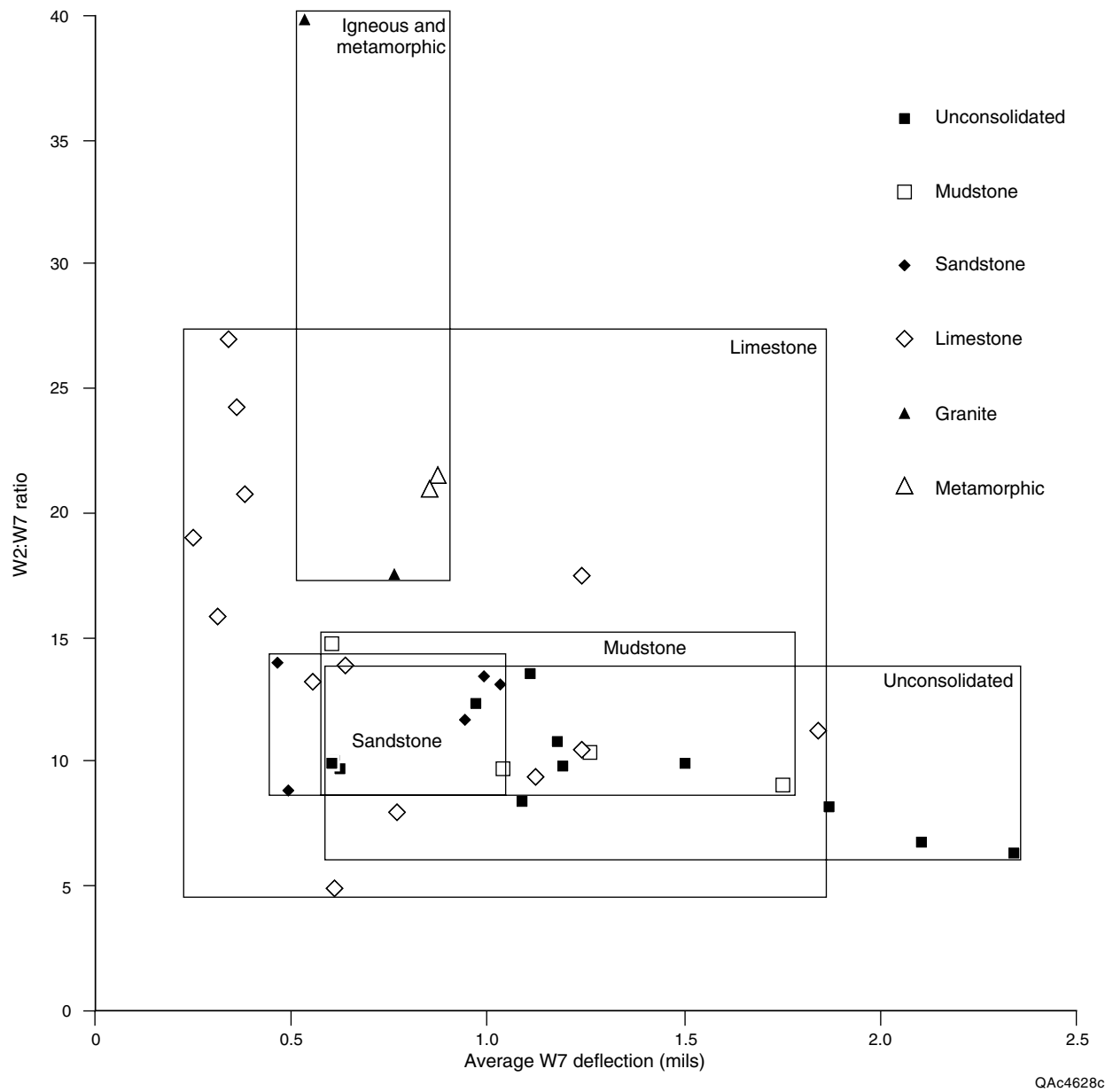
Figure 33. Average W 7 deflection and W 2: W 7 deflection ratio for individual rock types mapped along the Texas 16, U.S. 290, and Texas 71 test sites.
