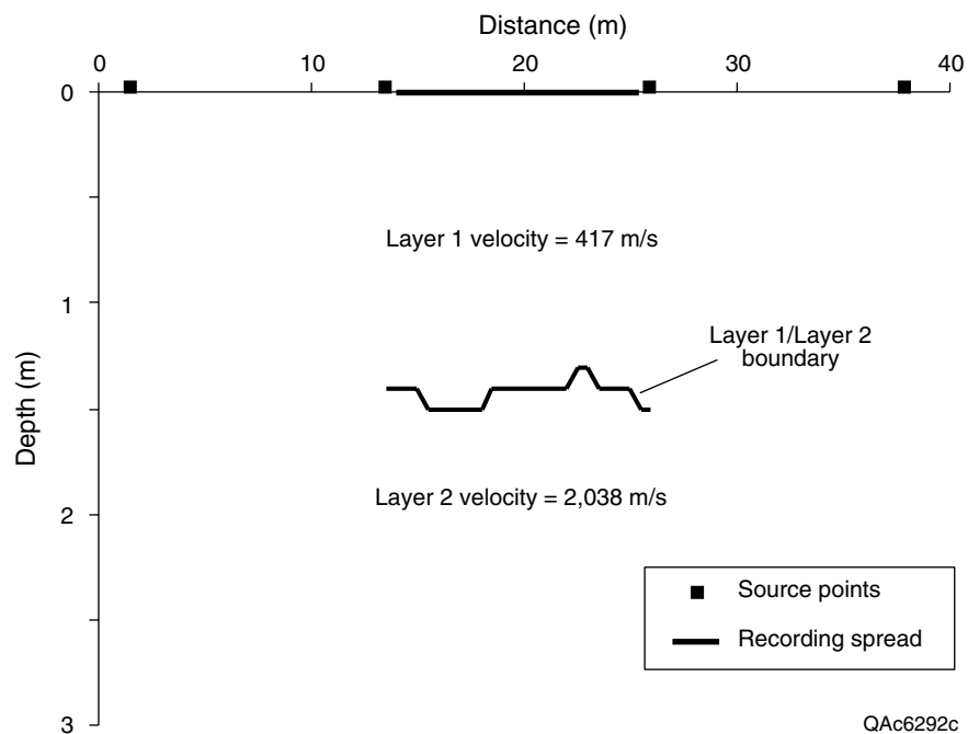
Figure 59. Cross section beneath Road D at the J. J. Pickle Research Campus, The University of Texas at Austin, showing locations of source points and recording array, interpreted depths to bedrock beneath the array, and approximate compressional-wave velocities of layer 1 (soil and road material) and layer 2 (bedrock).
