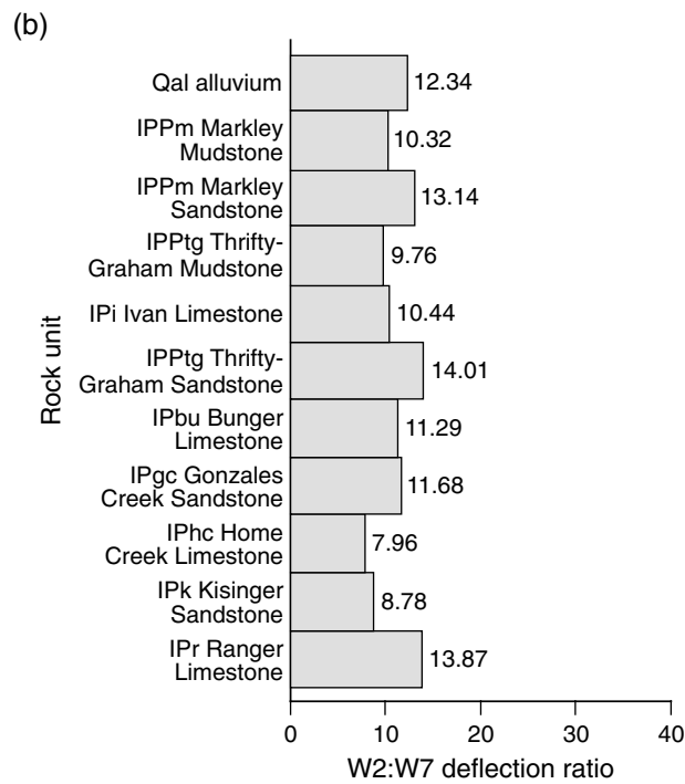
Figure 12. (a) Average W7 deflection and (b) W2:W7 deflection ratio by rock type along Texas 16, Archer and Young Counties.
