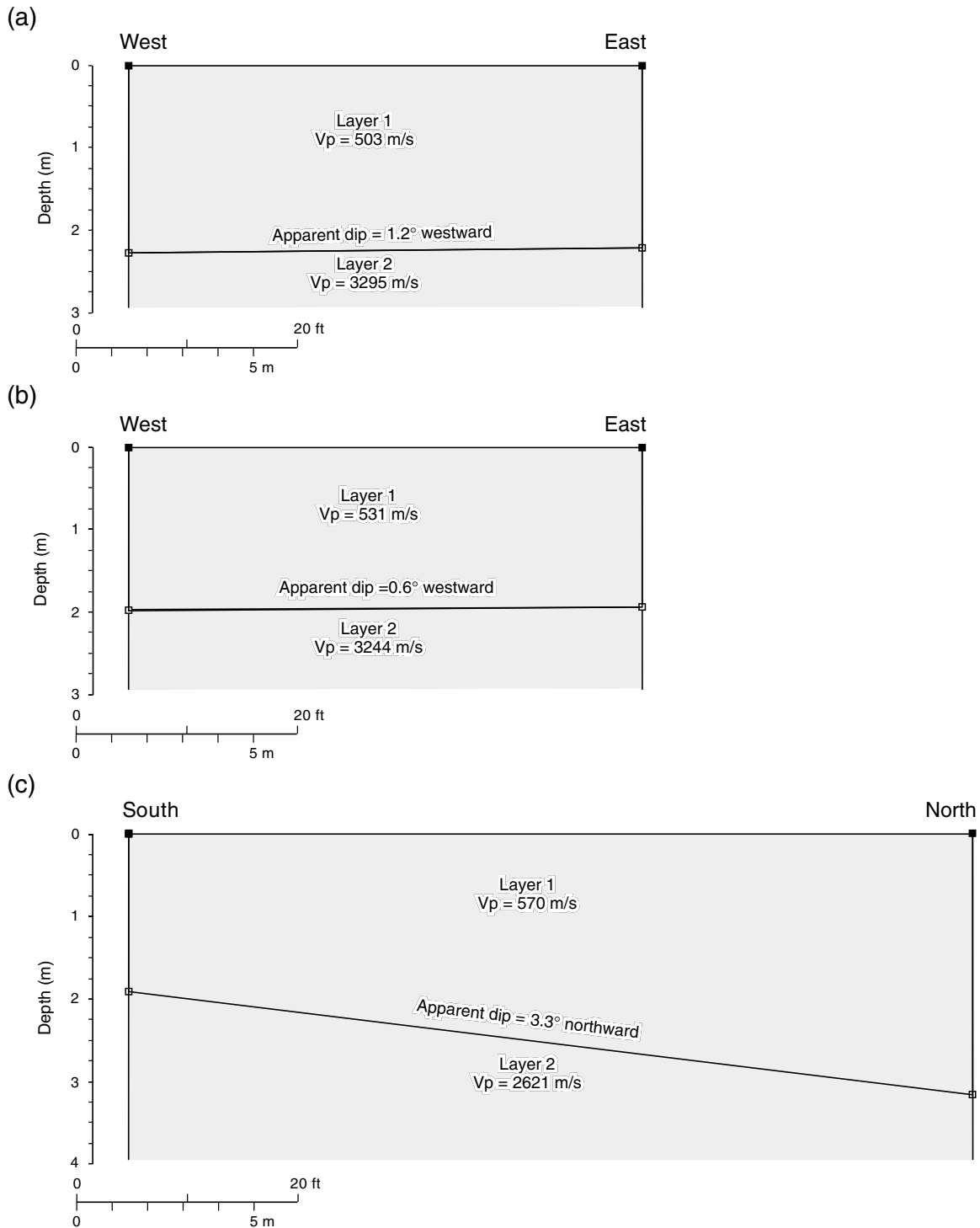
Figure 39. Calculated layer velocities and thicknesses and apparent dips of layer interfaces for refraction tests (a) PRC SPH1, (b) PRC SPH2, and (c) Jacksboro SPH1.
