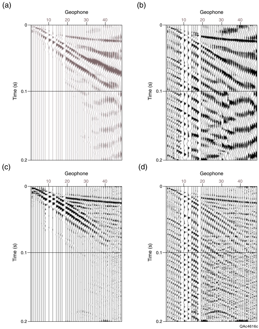
Figure 44. Effect of digital filtering and amplification on a field record from the Jacksboro MLS site (site R2, fig. 2) using a soil-probe hammer as a seismic source. Record displayed with (a) neither digital filtering nor time-varying gain; (b) time-varying gain (20-ms window) but no digital filtering; (c) 125-Hz low-cut filter without time-varying gain; and (d) 125-Hz low-cut filter and time-varying gain (20-ms window) applied. Geophone spacing is 0.5 m.
