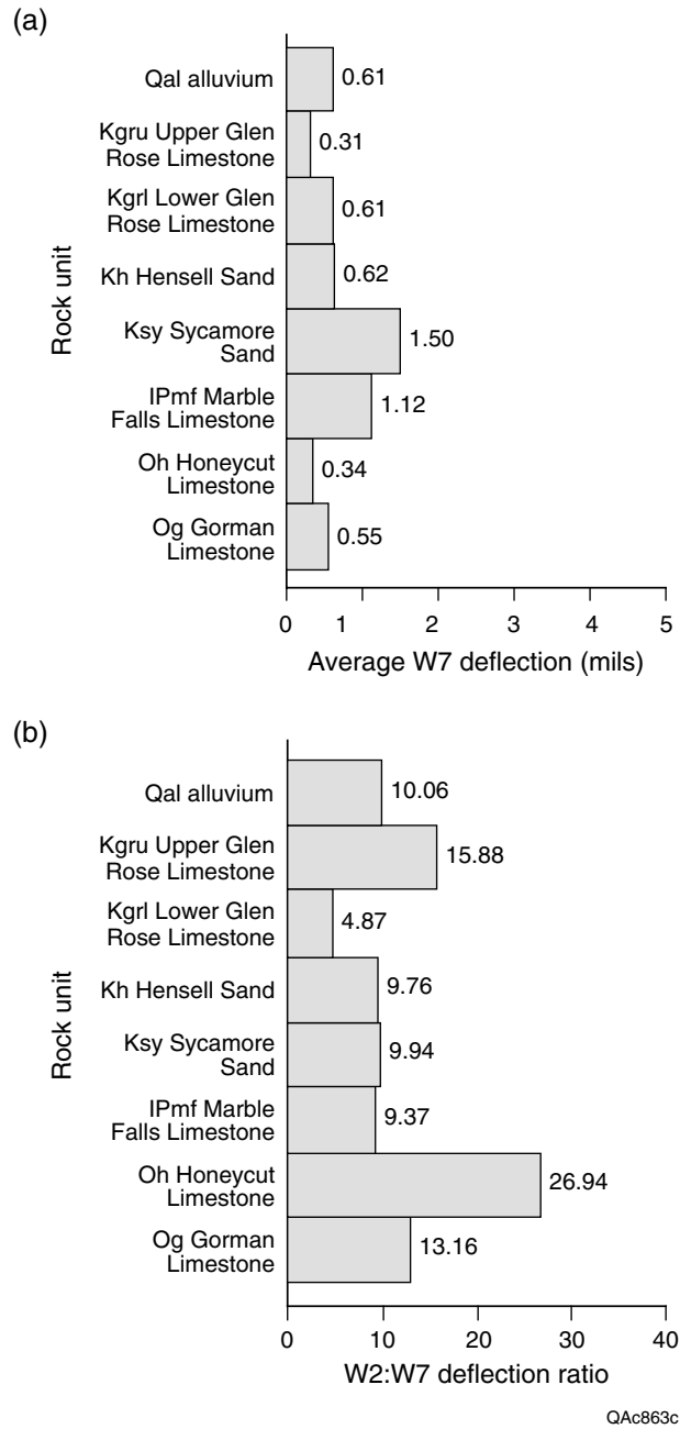
Figure 20. (a) Average W7 deflection and (b) W2:W7 deflection ratio by rock type along Texas 71, Burnet County.
