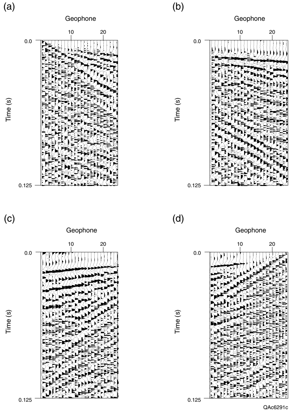
Figure 58. Field records acquired using Seismic Refraction Bedrock Analyzer at the J. J. Pickle Research Campus, The University of Texas at Austin (site R1, fig. 2). Source and recording array were located on the pavement of Road D. Source was (a) at the east end of the recording spread, (b) 12.5 m east of the east end of the recording spread, (c) 12.5 m west of the west end of the recording spread, and (d) at the west end of the recording spread. Records displayed with a 125-Hz low-cut filter and time-varying gain (20-ms window) applied. Geophone spacing is 0.5 m.
