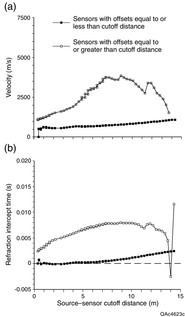
Figure 42. (a) Apparent velocity and (b) zero-offset time for forward data from refraction test PRC SPH2. Velocities and intercepts calculated by assigning arrivals from various offset ranges to the direct or refracted arrival.
