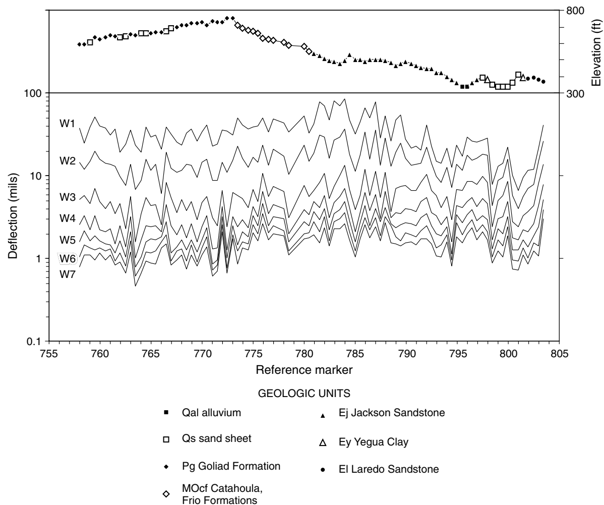
Figure 29. Geologic units, elevation, and W1 through W7 deflections along Texas 16 between reference markers 758 and 804, Jim Hogg and Zapata Counties, South Texas.
