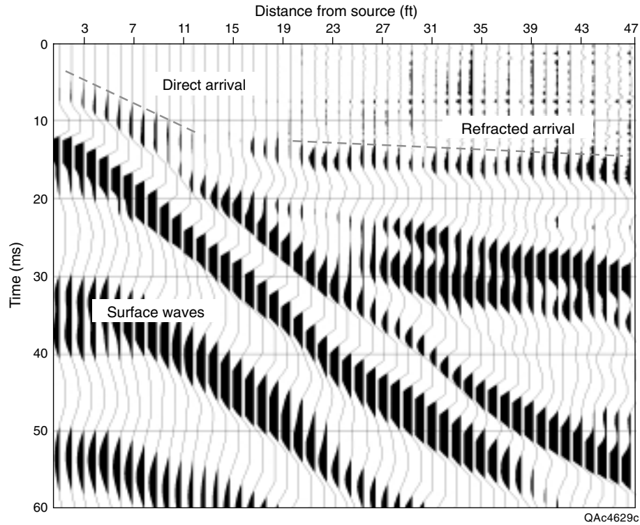
Figure 34. Seismic response recorded with a 48-geophone spread using the FWD as a seismic source. Visible phases include the direct arrival, a critically refracted arrival from the underlying rigid layer, long-wavelength, low-frequency surface waves, and reflected compressional waves. Data recorded on a flexible-pavement road on the J. J. Pickle Research Campus, The University of Texas at Austin.
