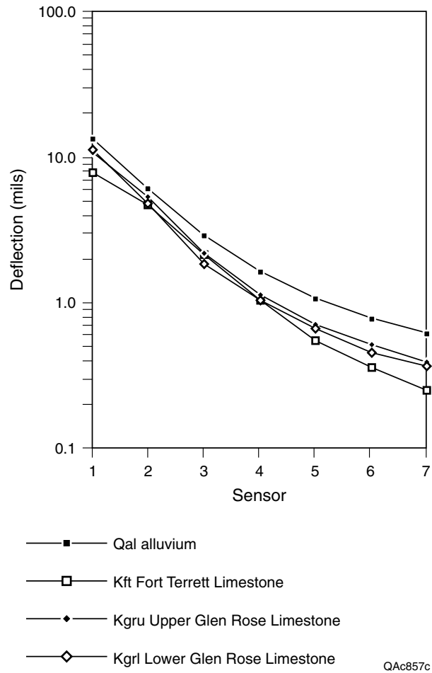
Figure 23. Average deflections for all rock units mapped along U.S. 290 in Blanco and Hays Counties.
