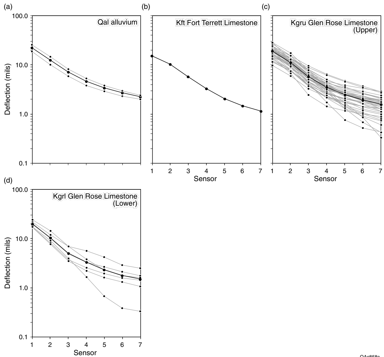
Figure 22. Average and individual deflections for rock types mapped along U.S. 290 in Blanco and Hays Counties.
