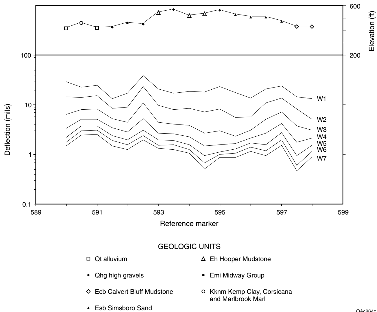
Figure 25. Geologic units, elevation, and W1 through W7 deflections along Texas 71 between reference markers 590 and 598, Bastrop County, southeast Texas.
