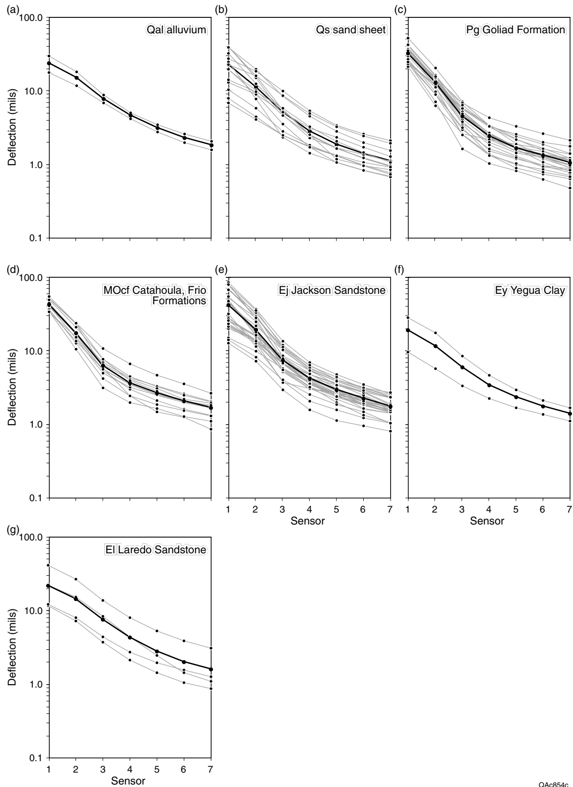
Figure 30. Average and individual deflections for rock types mapped along Texas 16 in Jim Hogg and Zapata Counties.
