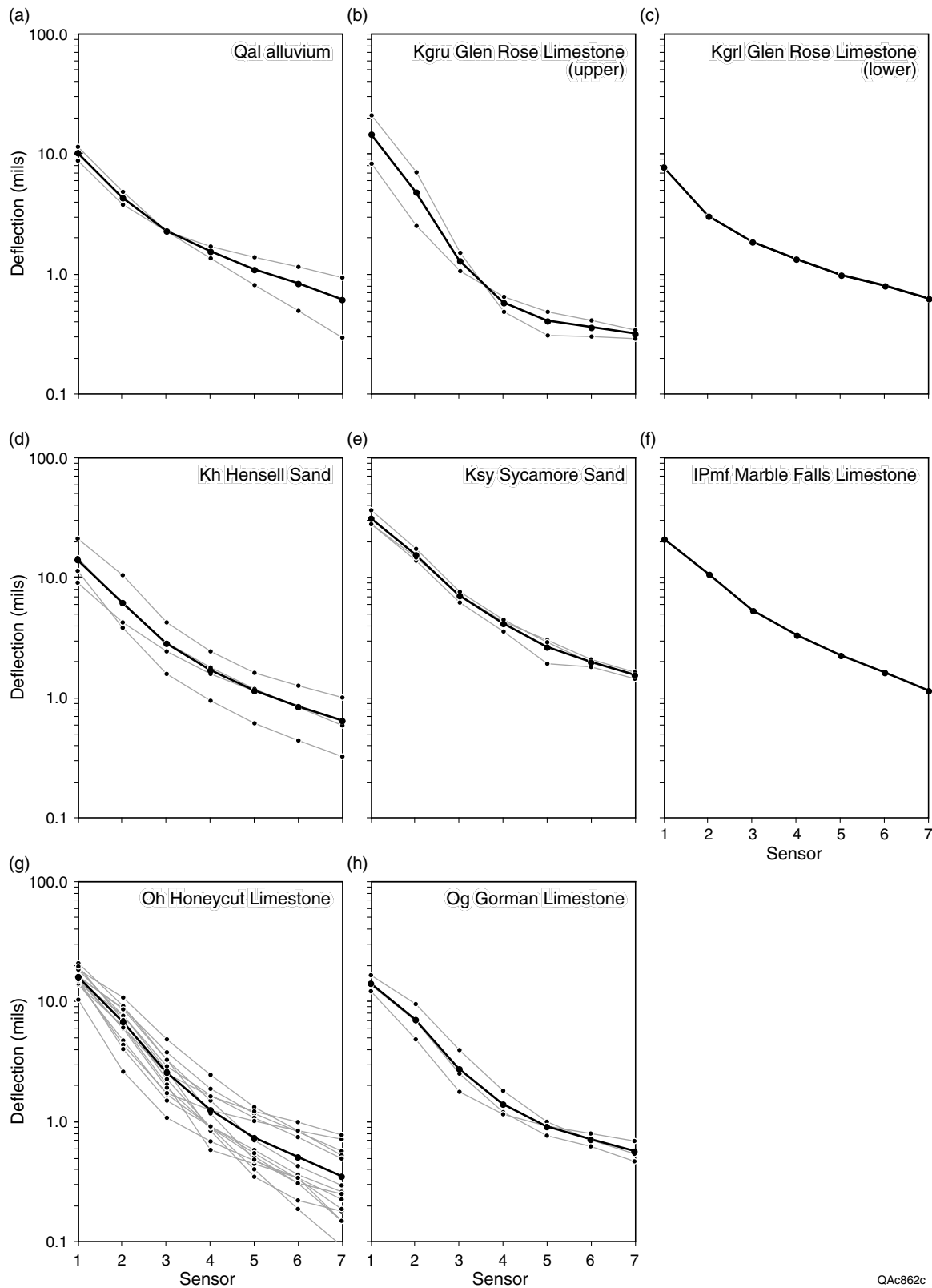
Figure 18. Average and individual deflections for rock types mapped along Texas 71 in Burnet County.
