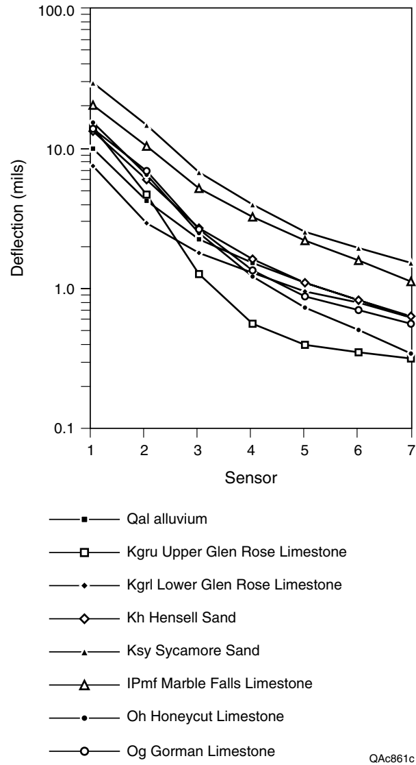
Figure 19. Average deflections for all rock units mapped along Texas 71 in Burnet County.
