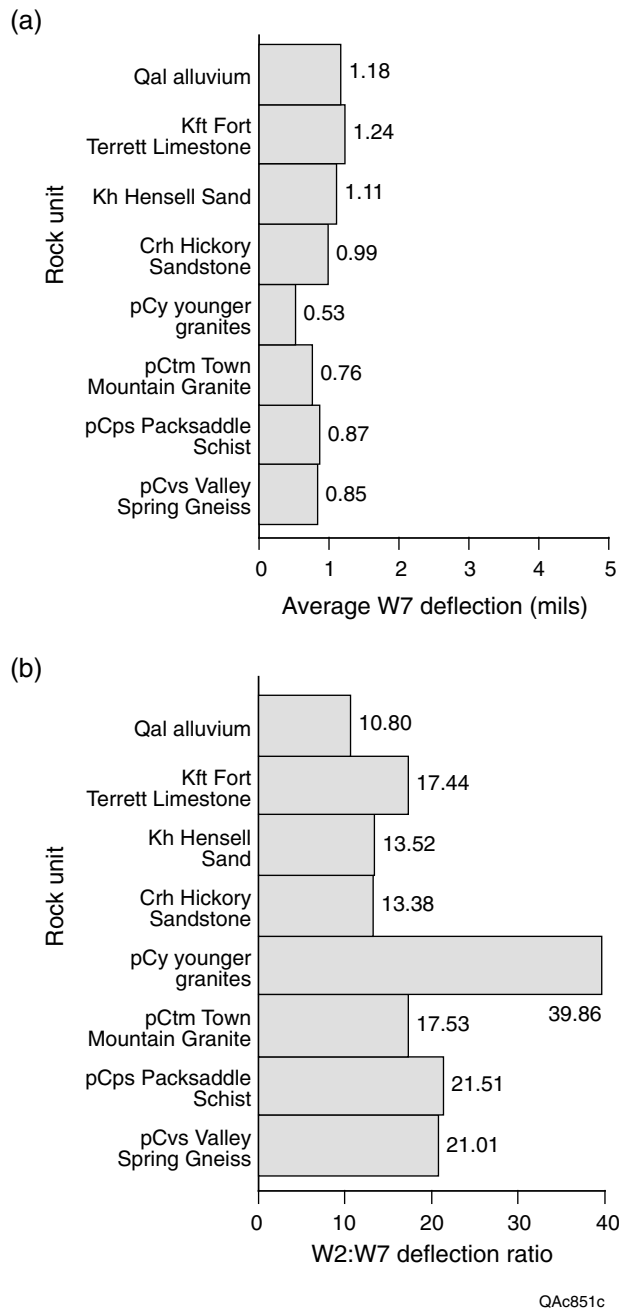
Figure 16. (a) Average W7 deflection and (b) W2:W7 deflection ratio by rock type along Texas 16, Llano and Gillespie Counties.
