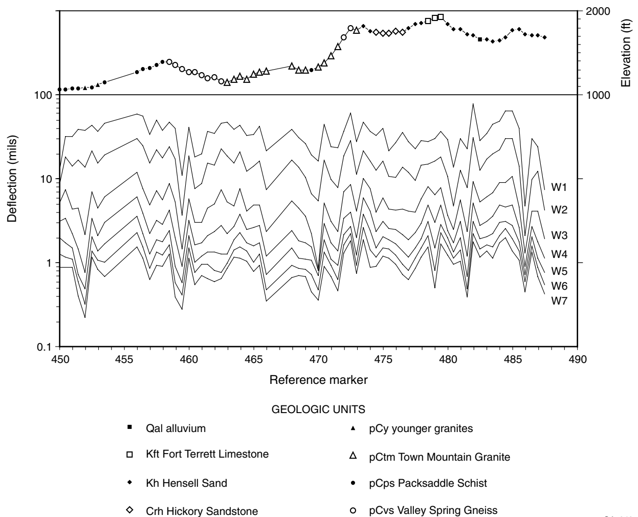
Figure 13. Geologic units, elevation, and W1 through W7 deflections along Texas 16 between reference markers 450 and 490, Llano and Gillespie Counties, Central Texas.
