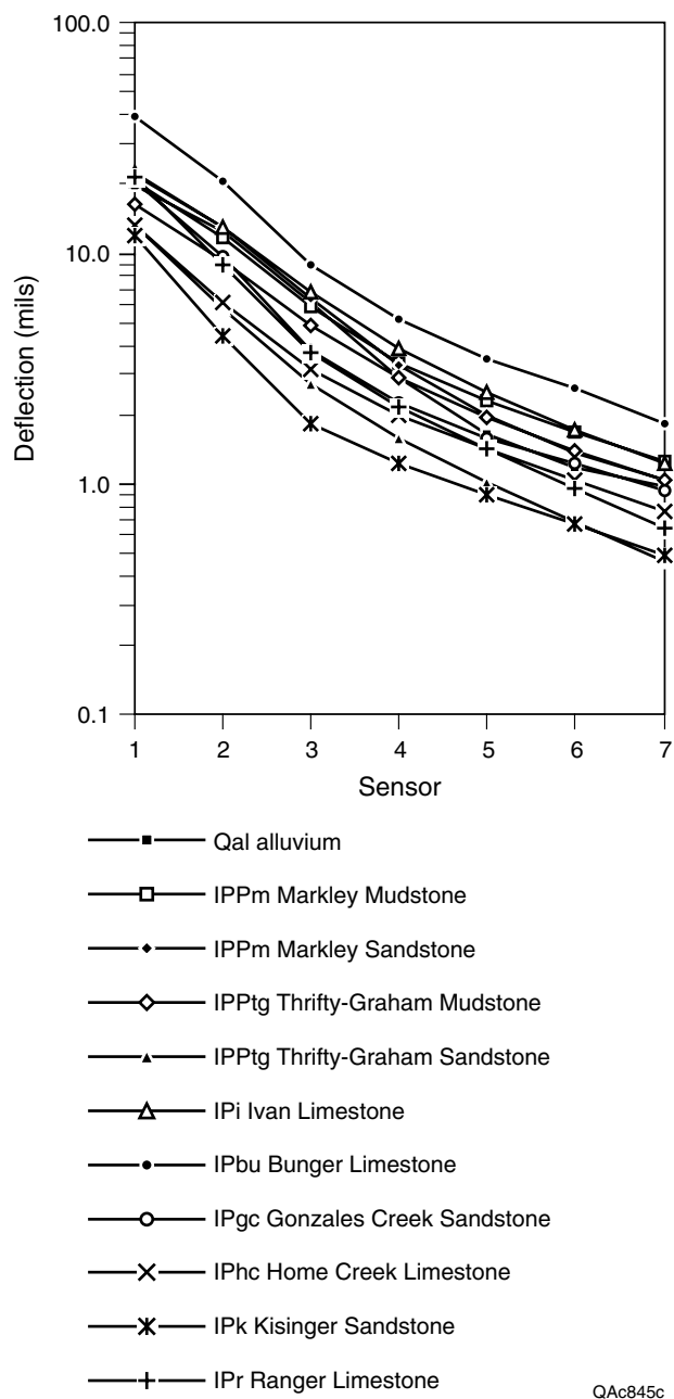
Figure 11. Average deflections for all rock units mapped along Texas 16 in Archer and Young Counties.
