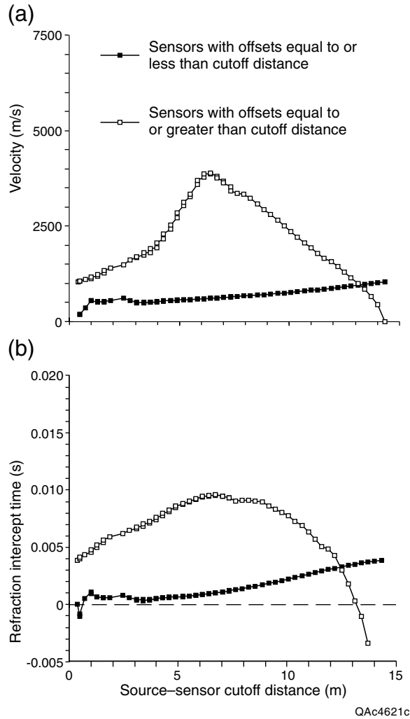
Figure 37. (a) Apparent velocity and (b) zero-offset time for forward data from refraction test PRC SPH1. Velocities and intercepts calculated by assigning arrivals from various offset ranges to the direct or refracted arrival. Velocities and intercepts (black boxes) calculated from arrivals at geophones located between the source and progressively increasing source-receiver distances are used to pick the optimal velocity and offset range for arrivals assigned to the direct wave. Velocities and intercepts (open boxes) calculated from arrivals at geophones located between the maximum source-receiver distance and progressively decreasing source-receiver distances are used to pick the optimal velocity, intercept time, and offset range for arrivals assigned to the critically refracted wave.
