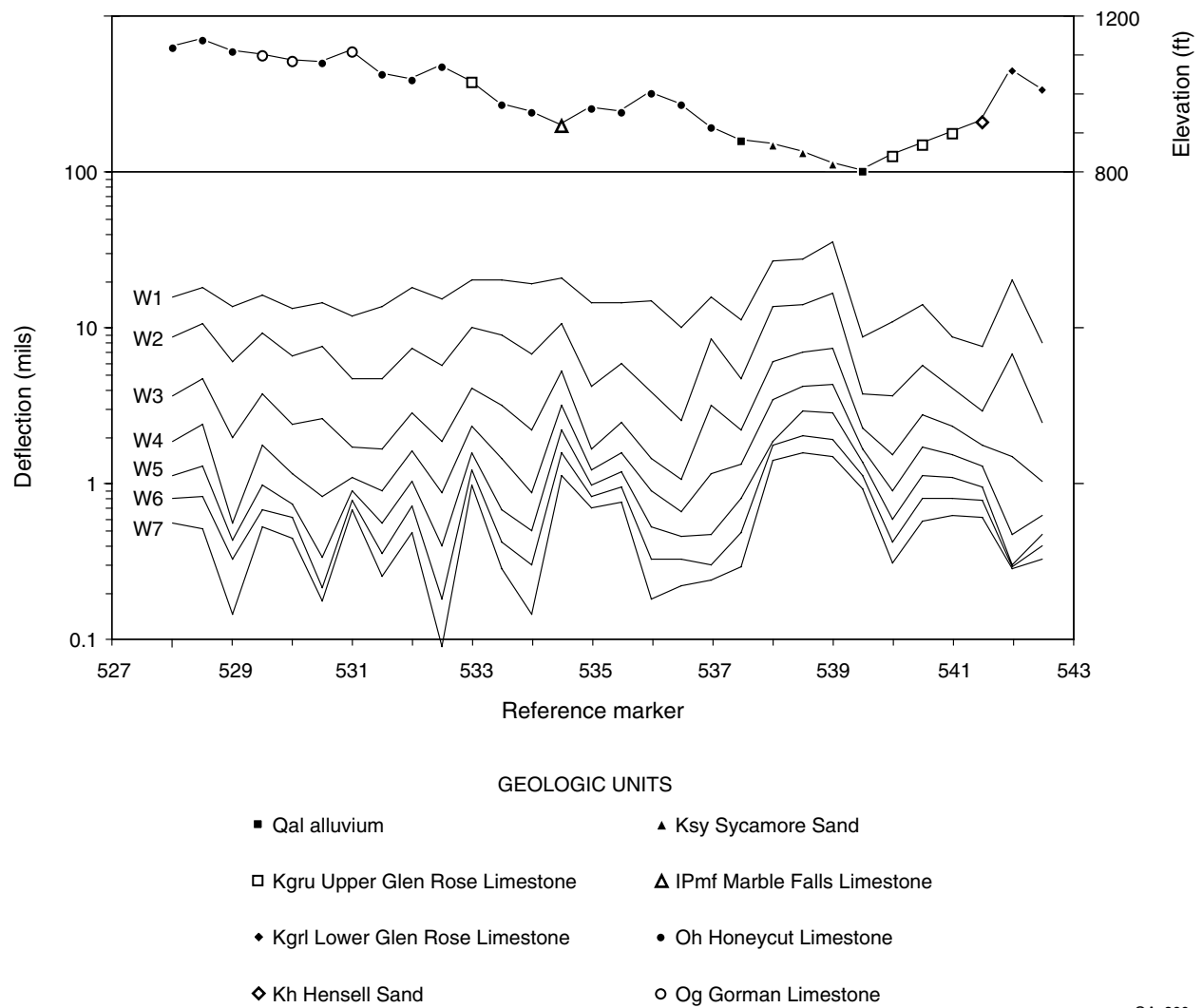
Figure 17. Geologic units, elevation, and W1 through W7 deflections along Texas 71 between reference markers 528 and 542, Burnet County, Central Texas.
