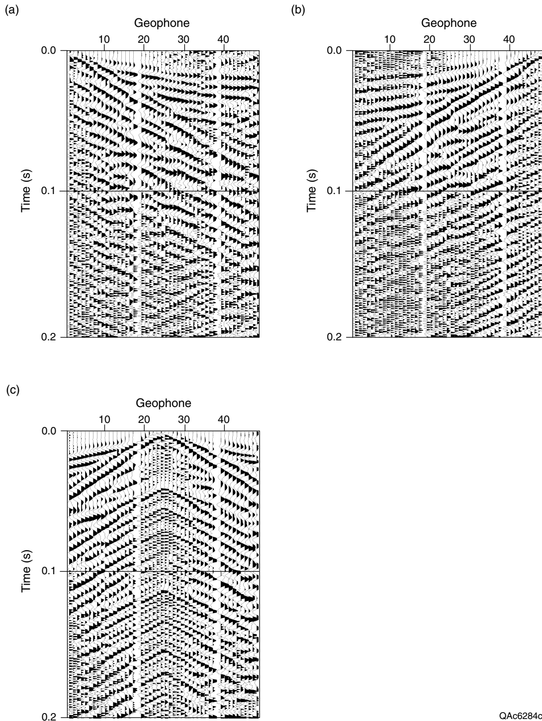
Figure 49. Field records from a refraction test near Granite Shoals (site R3, fig. 2) using a soil-probe hammer as a seismic source. Source and geophones were located on the pavement of FM 1431. Source was located at the (a) east end, (b) west end, and (c) center of the recording spread. Records displayed with a 125-Hz low-cut filter and time-varying gain (20-ms window) applied. Geophone spacing is 0.5 m.
