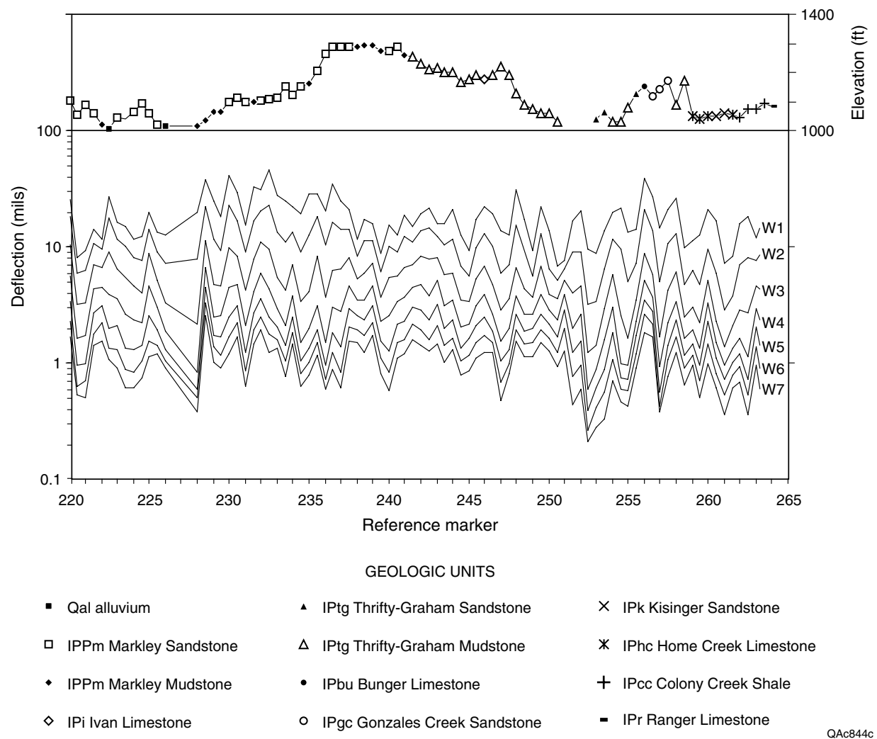
Figure 9. Geologic units, elevation, and W1 through W7 deflections along Texas 16 between reference markers 220 and 265, Archer and Young Counties, North Texas.
