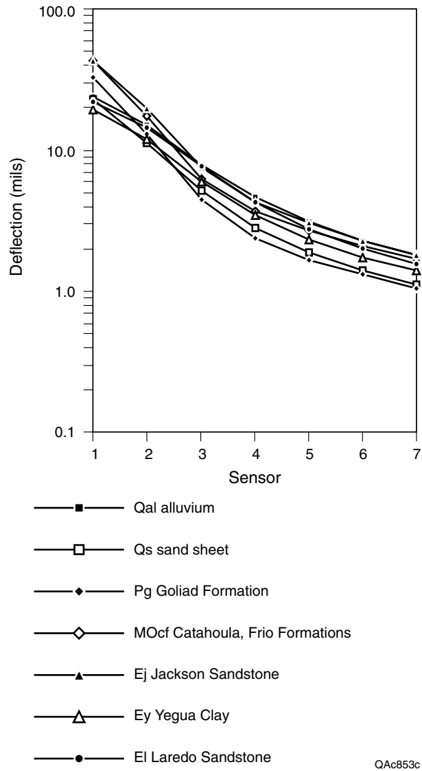
Figure 31. Average deflections for all rock units mapped along Texas 16 in Jim Hogg and Zapata Counties.
