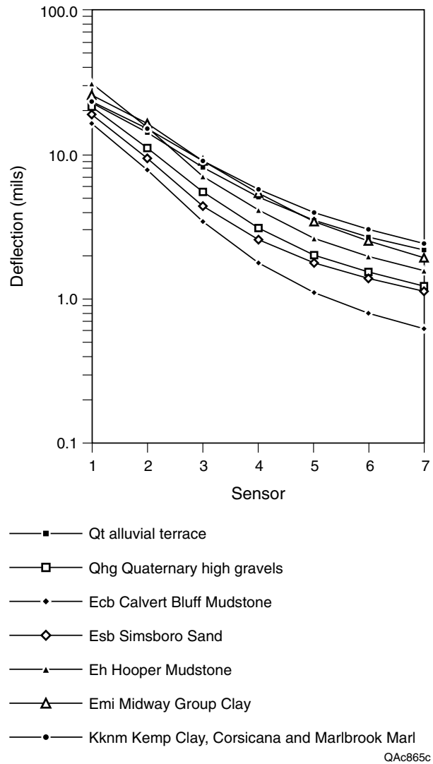
Figure 27. Average deflections for all rock units mapped along Texas 71 in Bastrop County.
