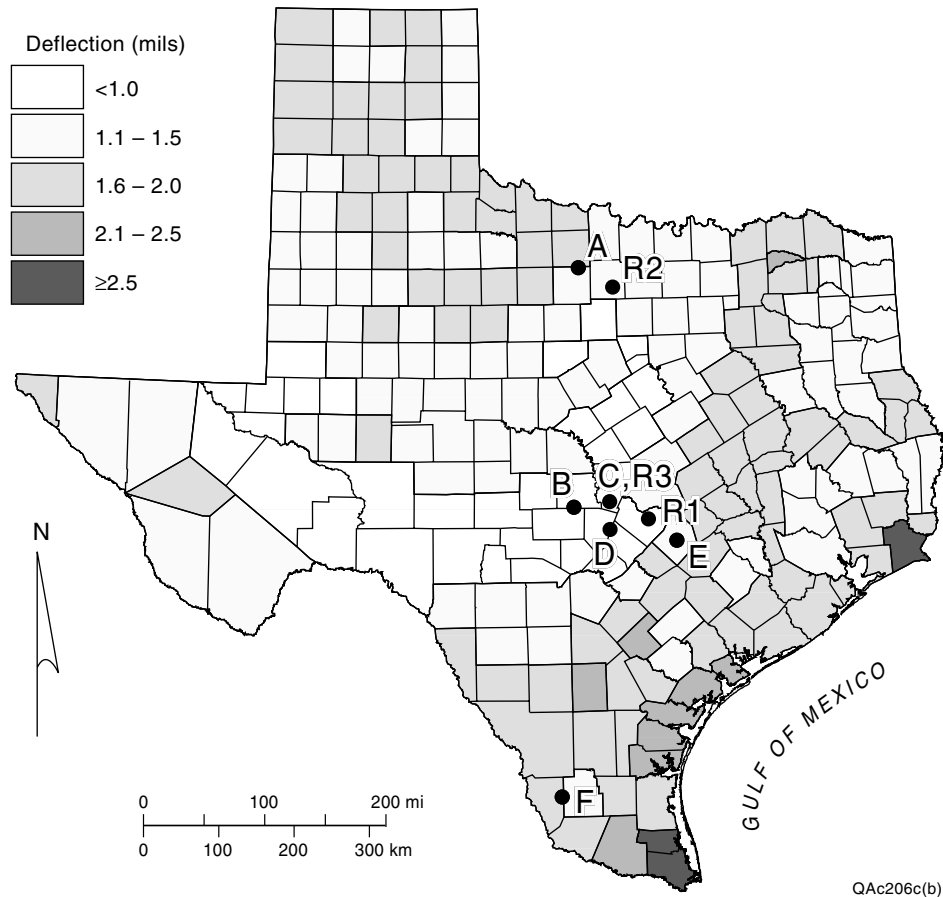
Figure 2. Average roadway deflection by county measured at Falling-Weight Deflectometer detector W7. Also shown are locations of study areas A through F and refraction test sites R1 (Road D, J. J. Pickle Research Campus), R2 (U.S. Highway 281 near Jacksboro), and R3 (FM 1431 near Granite Shoals).
