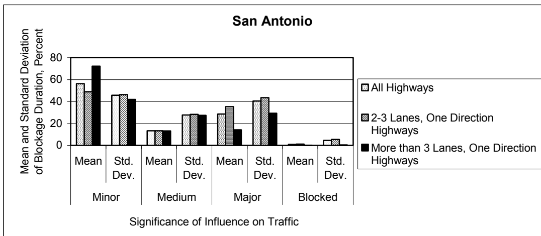
Figure 3.10b Percentage of Total Observed Traffic Influence Time by Cross Section Location (San Antonio)
