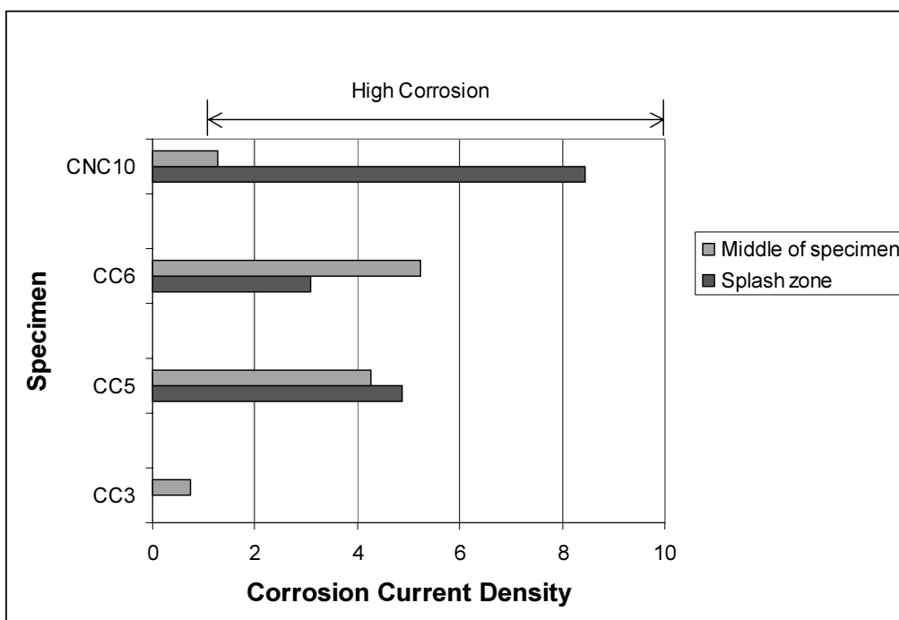
Figure 6.9 Corrosion current density ( \mu\text{A}/\text{cm}^2 ) values for Group B
