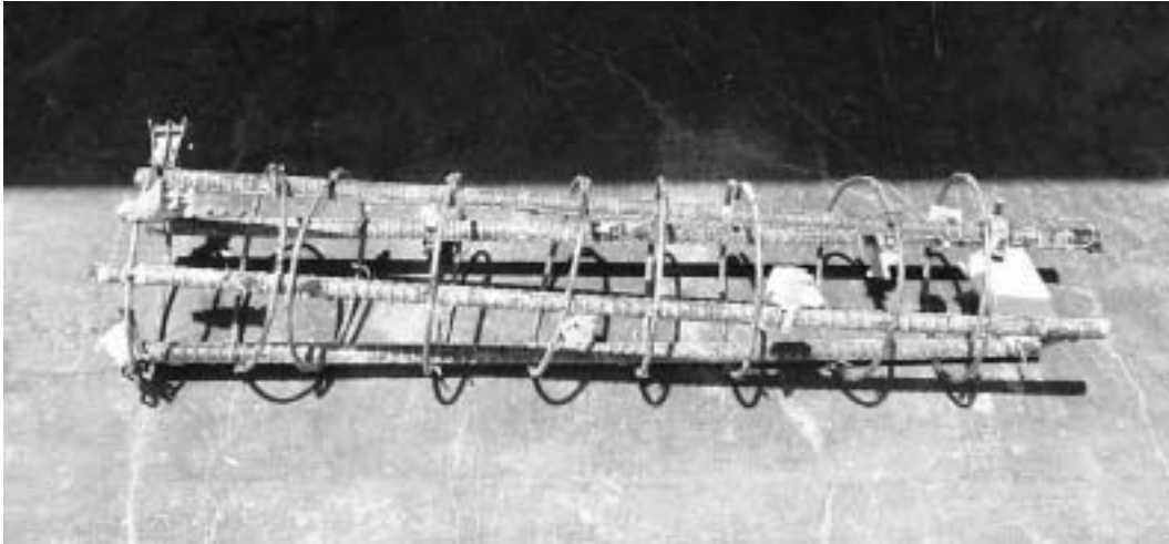
Figure C.1 Specimen CC7
