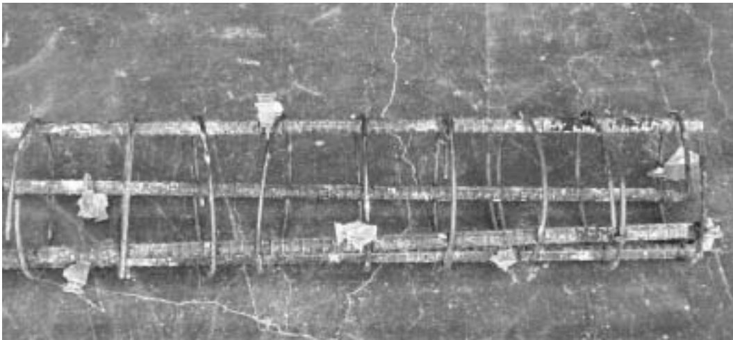
Figure C.4 Specimen CNC13
