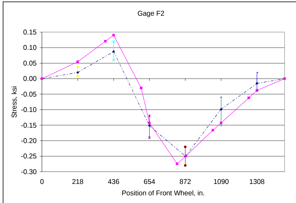
Fig. D.83: Field Test No. 2 - Vertical member L2U2
