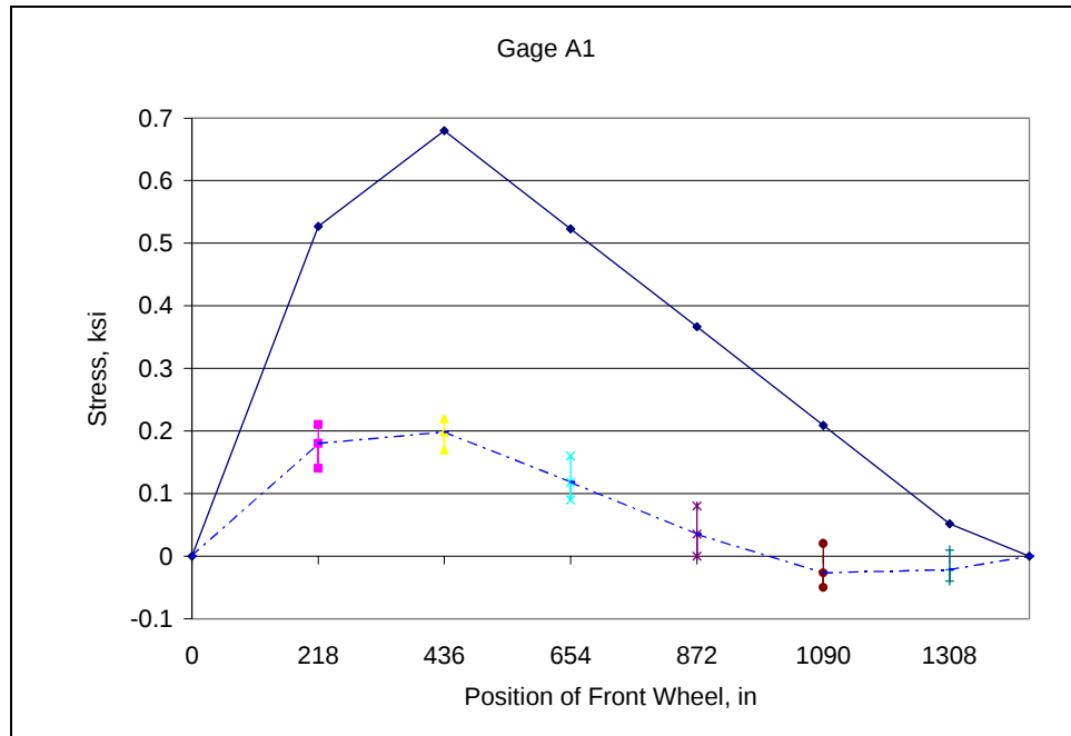
Fig. D.1: Field Test No. 1 - Member L0L1 (Outside) of upstream truss
