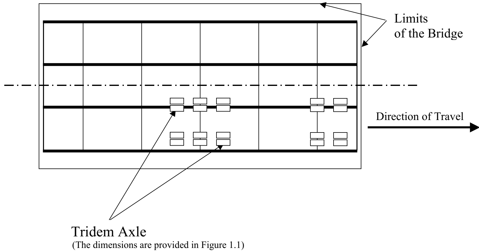
Figure 4.2. Input Loads for Truck with Tridem and Tandem Axles
