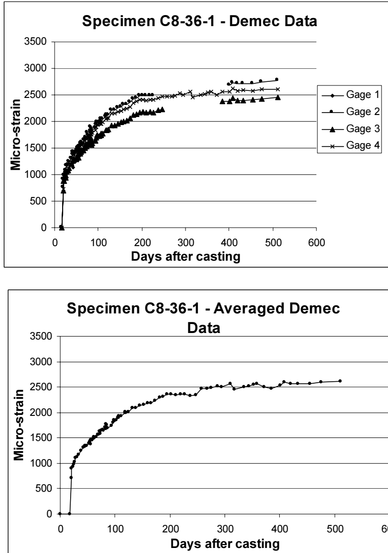
Figure 4.2 Mechanical Strain Gage Data for Specimen C8-36-1
