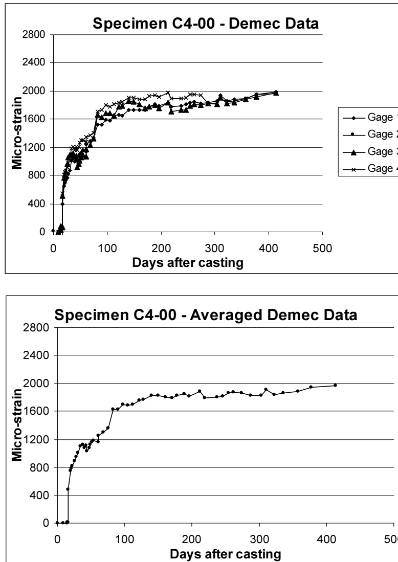
Figure 4.11 Mechanical Strain Gage Data for Specimen C4-00
