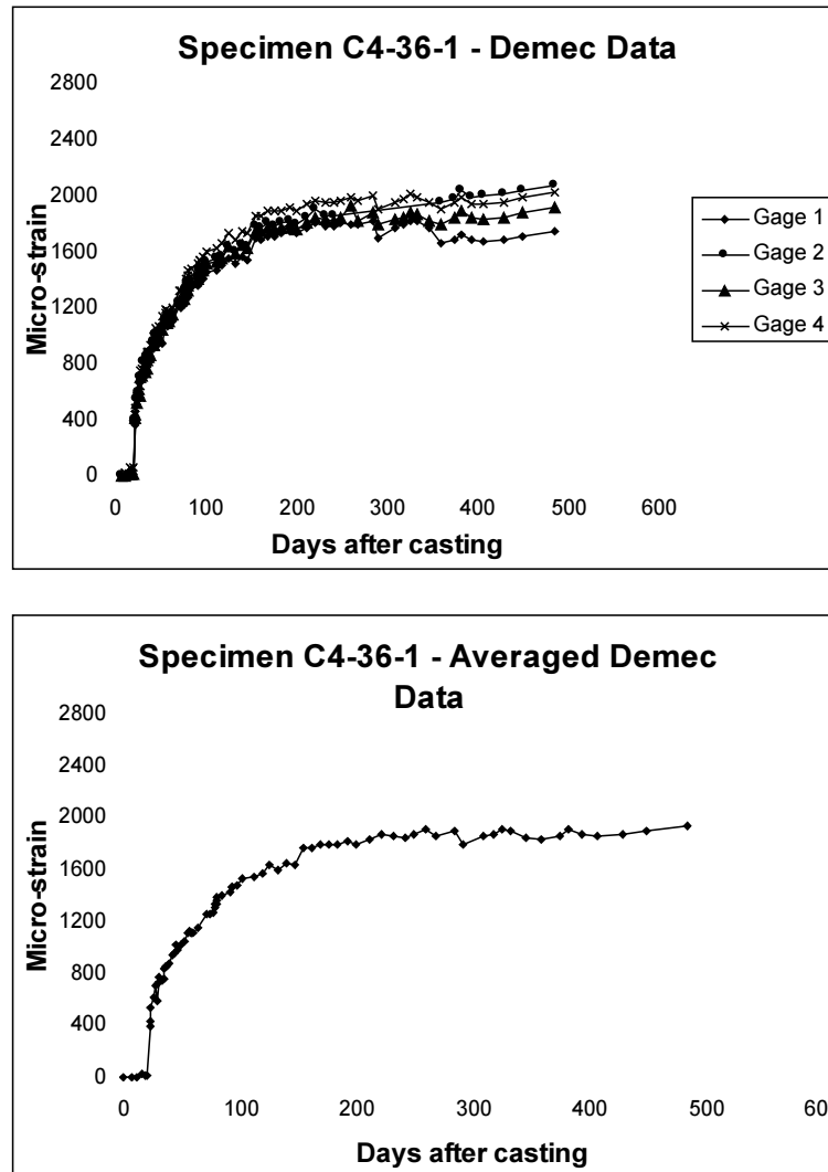
Figure 4.12 Mechanical Strain Gage Data for Specimen C4-36-1
