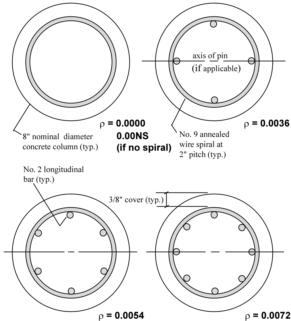
Figure 3.2 Column Specimen Cross Sections
