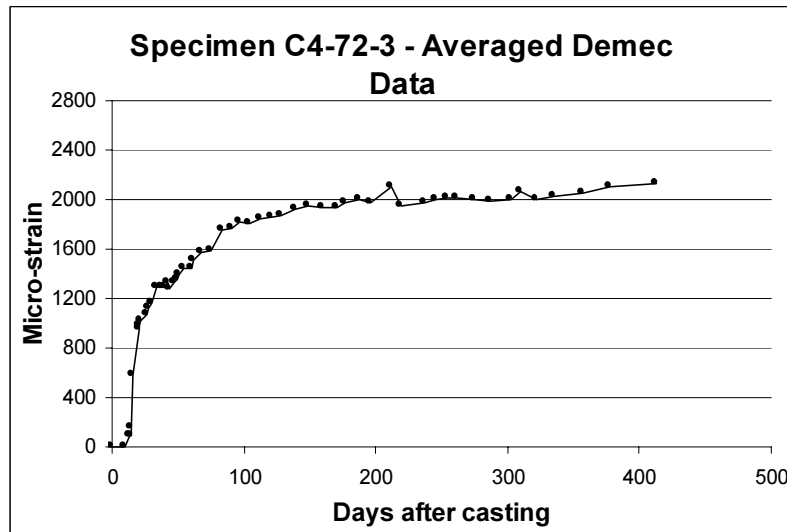
Figure 4.20 Mechanical Strain Gage Data for Specimen C4-72-3
