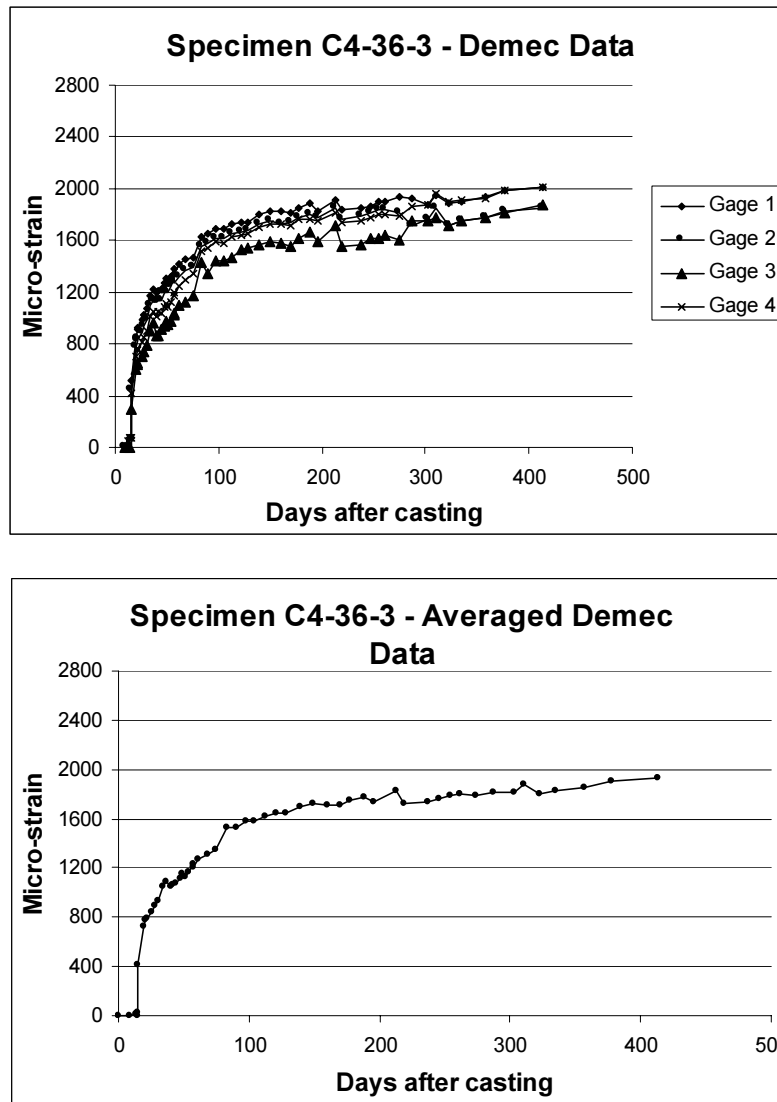
Figure 4.14 Mechanical Strain Gage Data for Specimen C4-36-3
