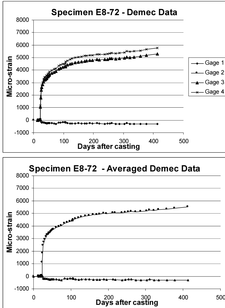
Figure 4.22 Mechanical Strain Gage Data for Specimen E8-72
