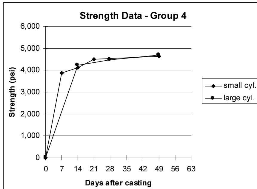
Figure 4.50 Strength and Modulus Data for Group 4
