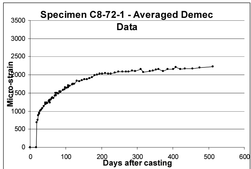
Figure 4.8 Mechanical Strain Gage Data for Specimen C8-72-1
