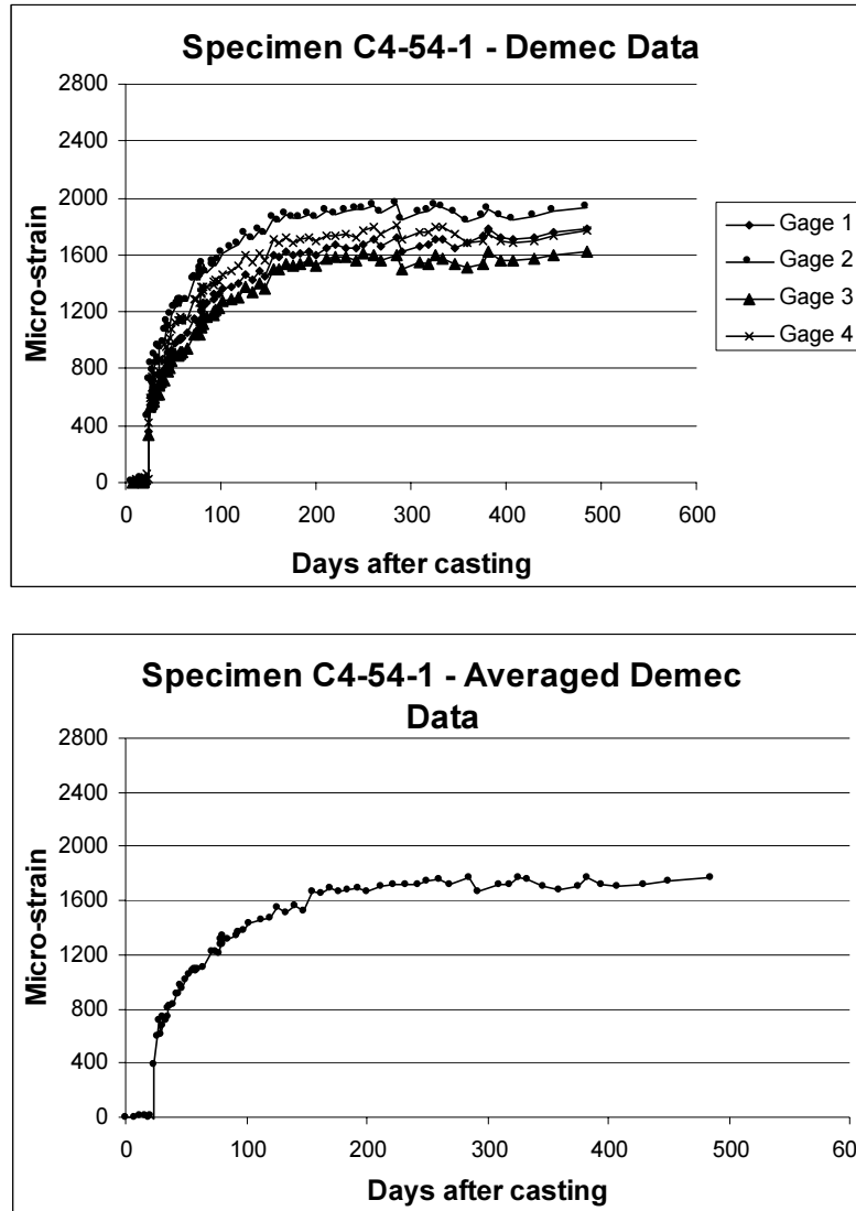
Figure 4.15 Mechanical Strain Gage Data for Specimen C4-54-1
