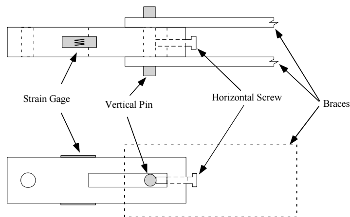
Figure 3.18 Coupler-Brace Connection
