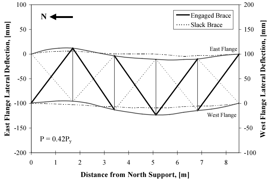
Figure 4.11 Typical Buckled Shape for 5 Brace Panels
