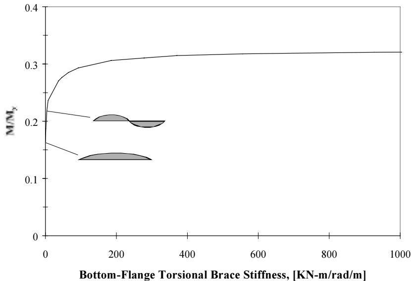
Figure 2.7 Effect of Increasing Bottom-Flange Torsional Brace Stiffness
