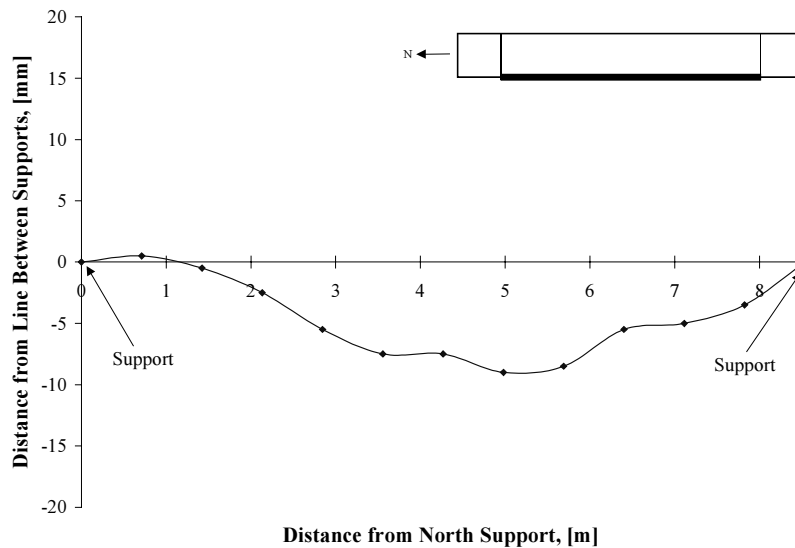
Figure 4.6 Initial Imperfections of West Flange of Rectangular Girder
