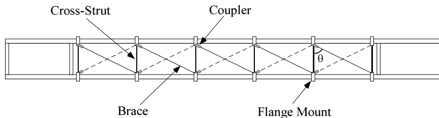
Figure 3.14 X- Brace System
