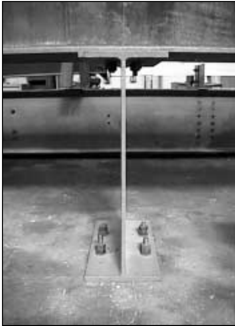
Figure 3.5 Support Beam
