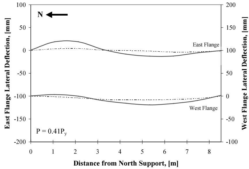
Figure 4.9 Typical Buckled Shape for Unbraced Girder
