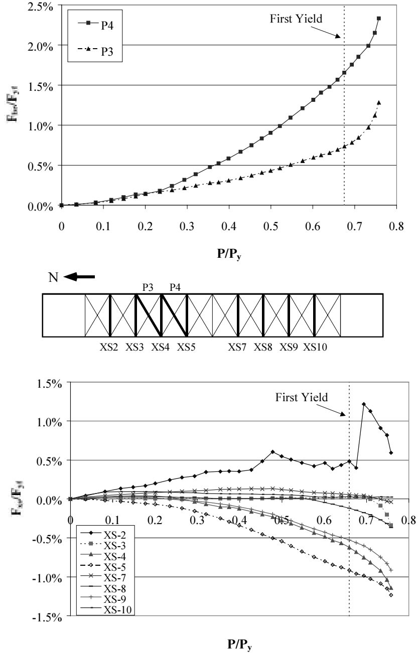
Figure 4.25 Brace Force Distribution for R10-W
