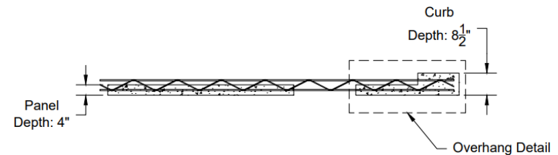
Figure 4-3 9'-6" Panel Pair Details
