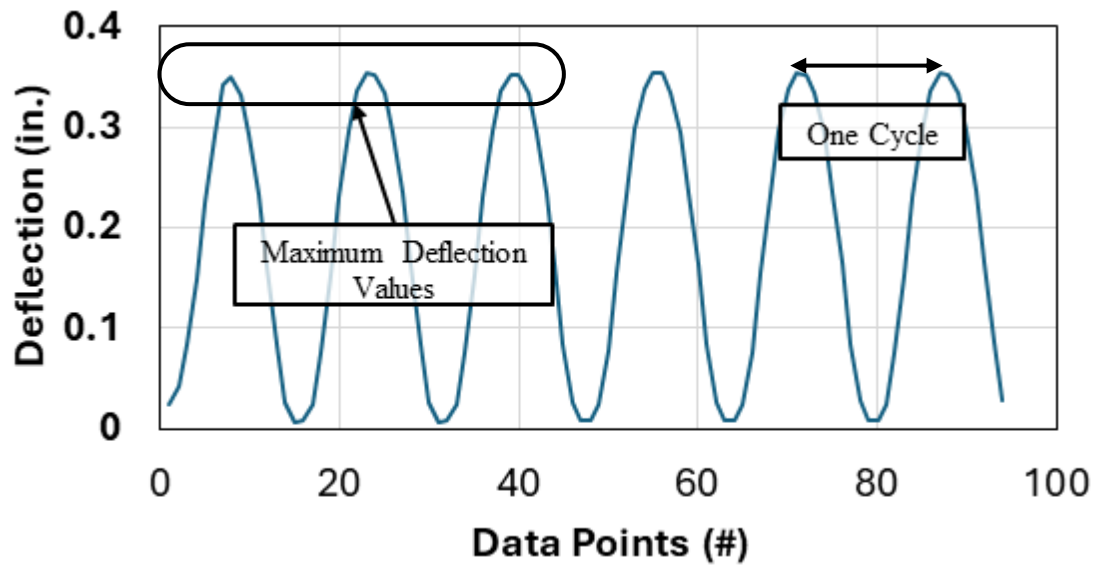
Figure 5-19: Test 1 - Stress Example Deflection Data
