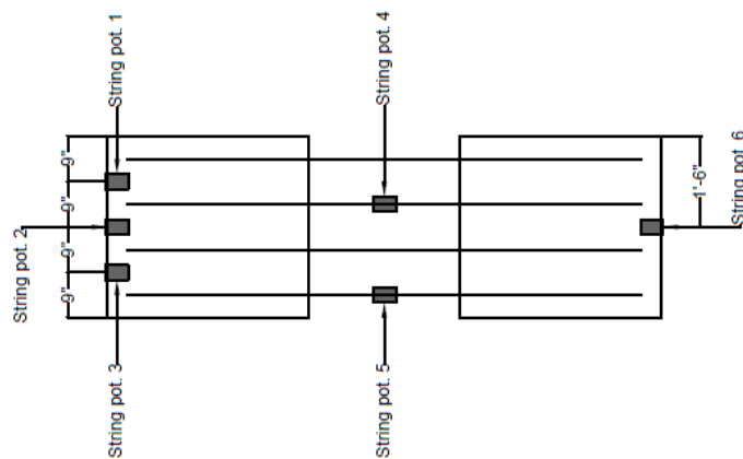
Figure 3-16 String potentiometer locations
