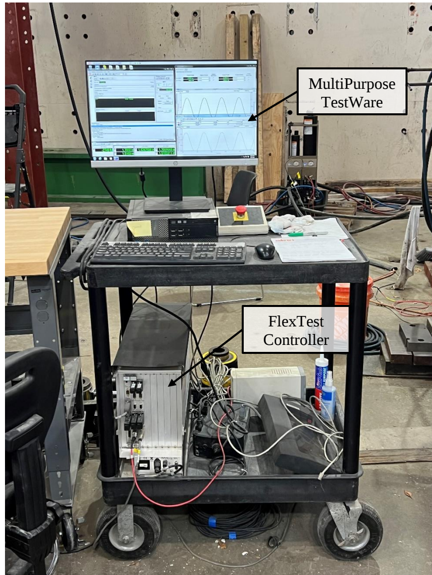
Figure 5-16: FlexTest Controller and Software Overview
