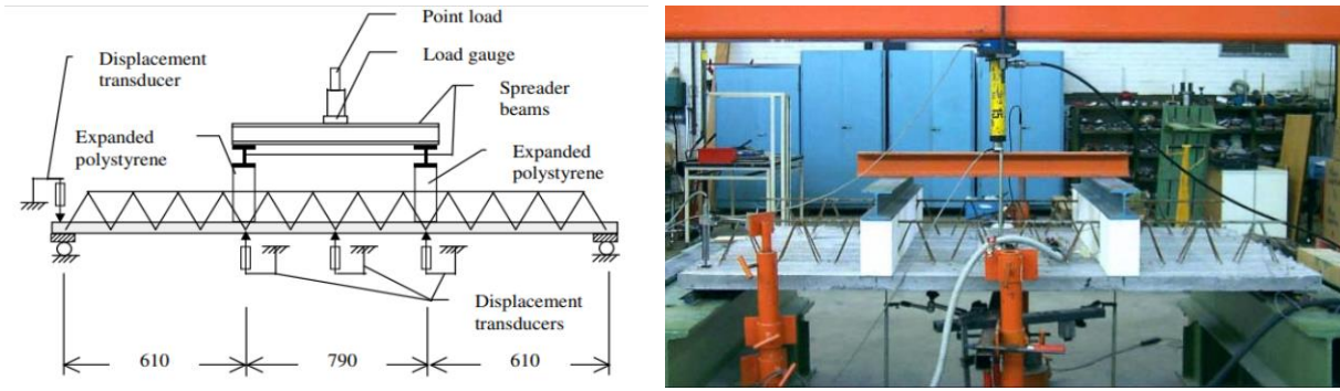
Figure 2-11 Loading test setup for four-point bending (Löfgren et al., 2001)
