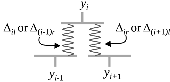
Figure 3-43 relative displacement in springs
