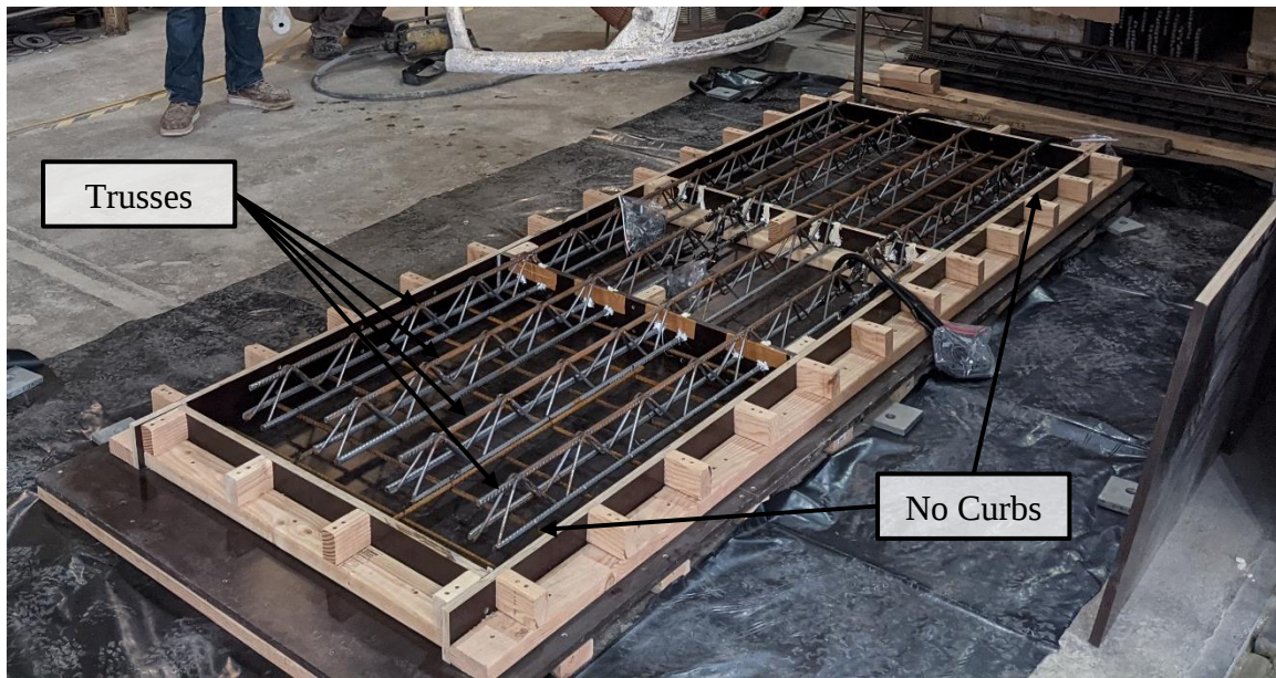
Figure 5-4: Construction of Formwork for Testing Specimen
