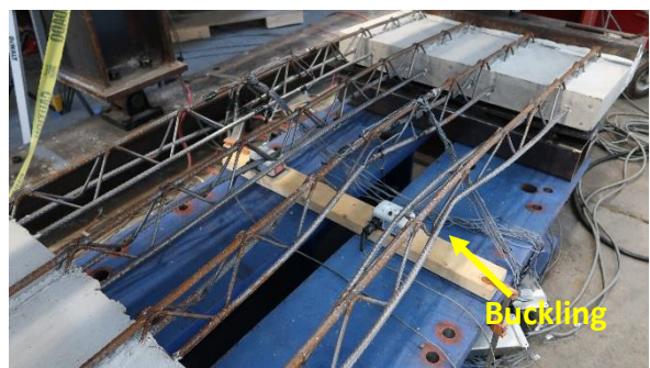
Specimen I-E-U49
