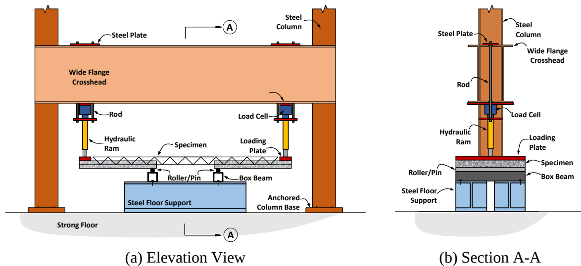
Figure 3-12 Test Frame
