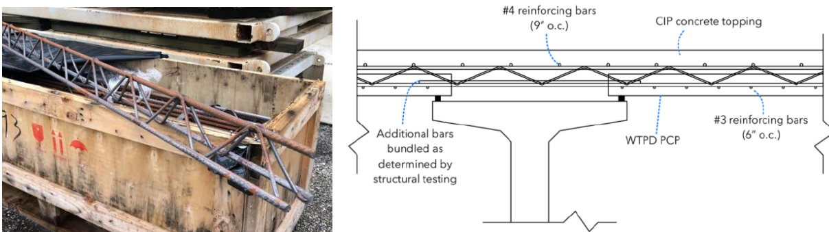
Figure 3-1 Wire trusses and typical design of NextGen decks with wire trusses
