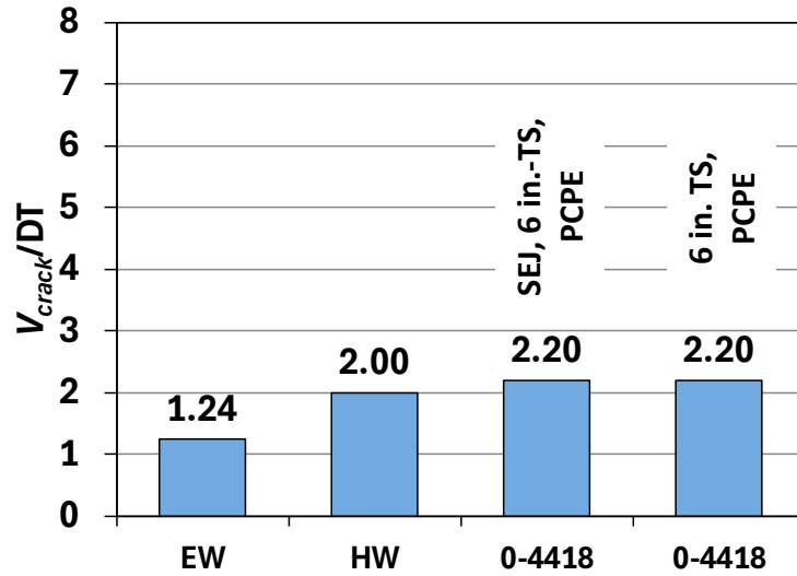
Figure 4-64 Comparison of Cracking loads in Long Span under Positive Moment
