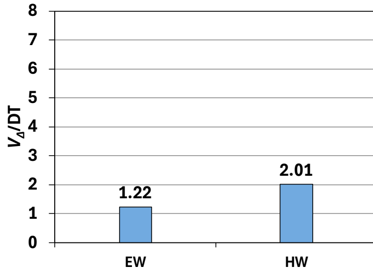
Figure 4-65 Comparison of loads causing deflection limit in Long Span under Positive Moment
