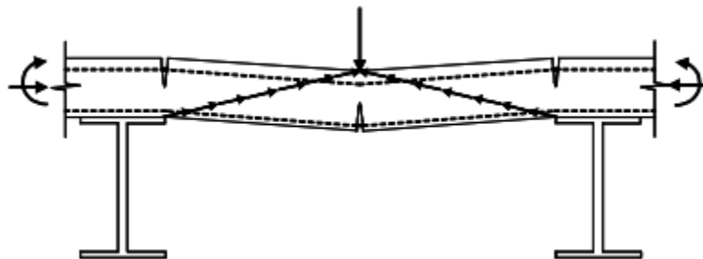
Figure 2-1 Arching action
