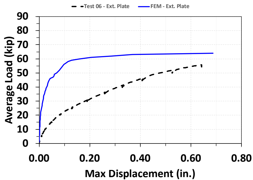
Figure 4-82: Test 6 Load Deflection Comparison
