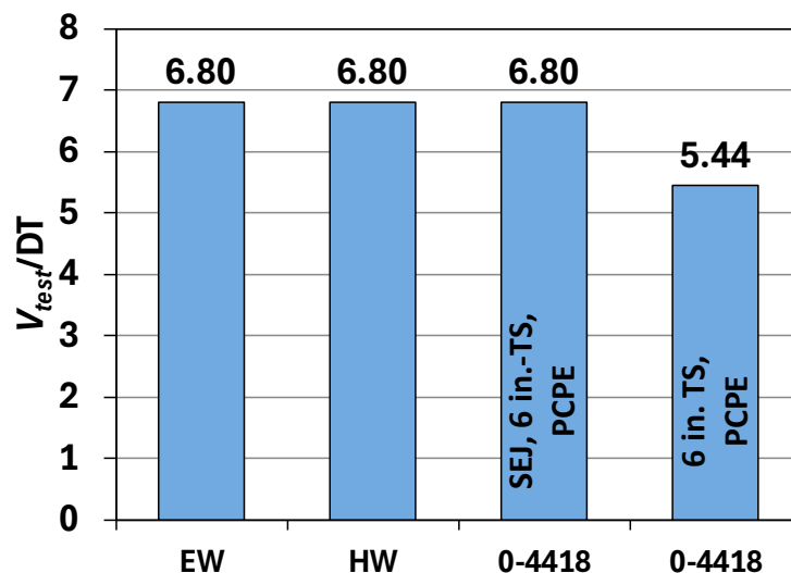
Figure 4-63 Comparison of Ultimate Load Carrying Capacity in Long Span under Positive Moment
