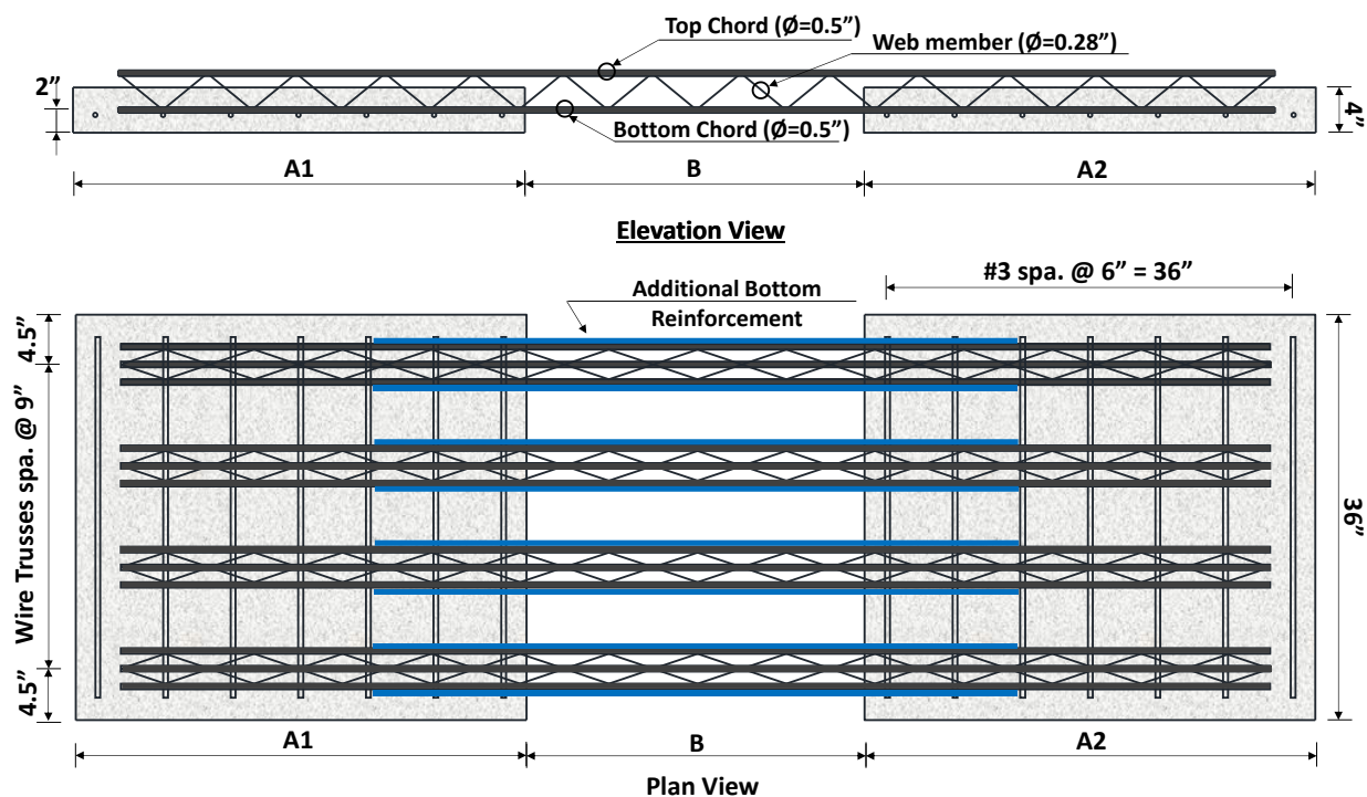
Figure 3-2 Specimen design
