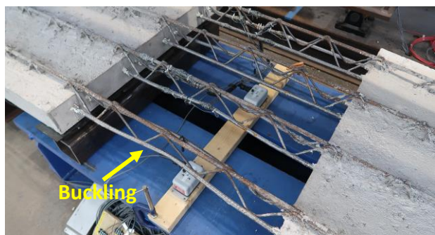
Specimen I-E-U30
