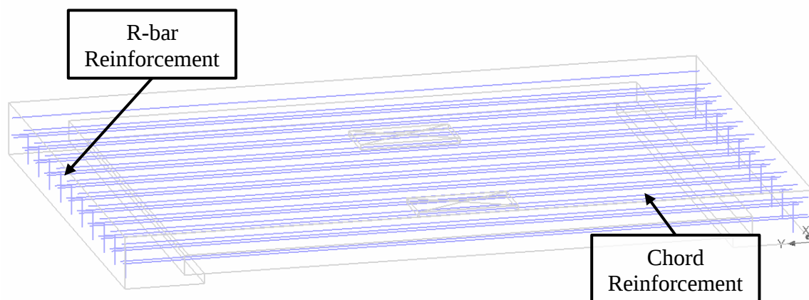
Figure 4-74: Reinforcement Layout
