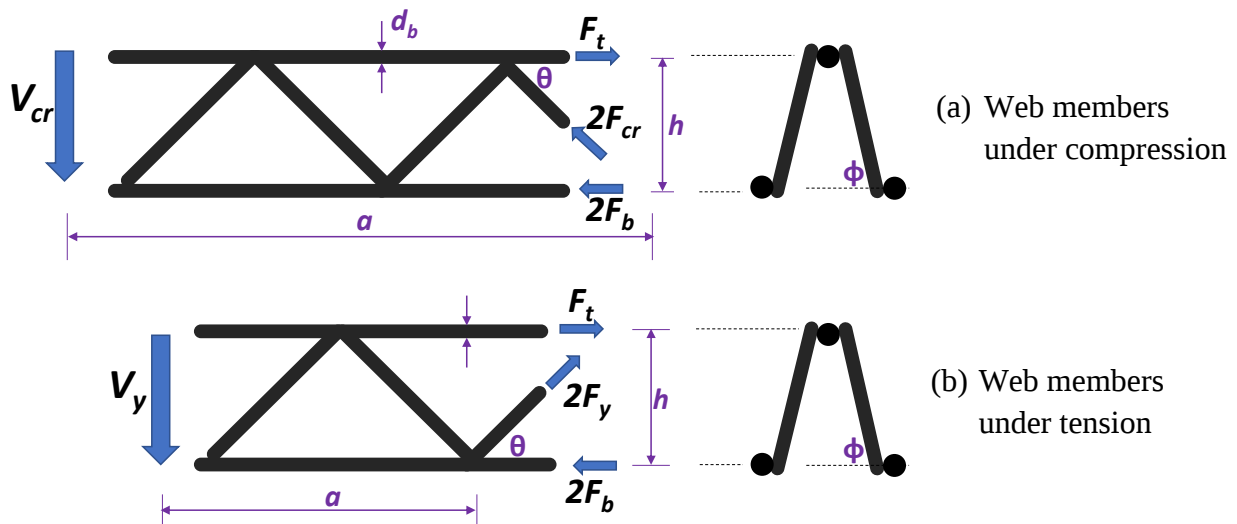
Figure 3-39 Wire trusses under shear force
