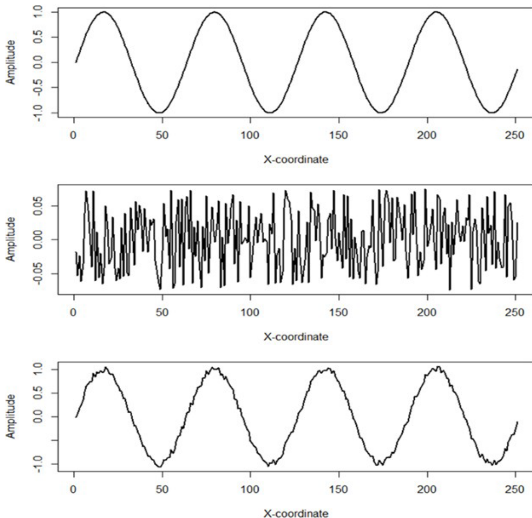
Figure 2.7 Example of how white noise can be mistaken for microtexture: sine wave (top), white noise (middle), signal and noise (bottom)
