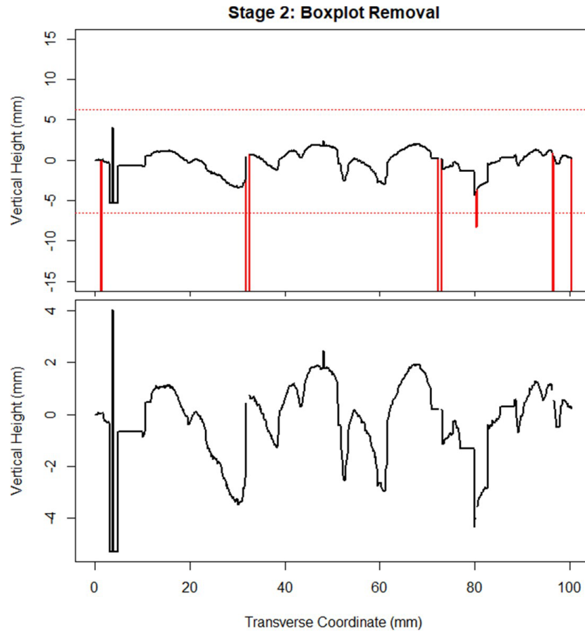
Figure 2.12 Boxplot filter with threshold shown as red horizontal dashed lines and removed data points highlighted in red (top) and profile after boxplot filter has been applied (bottom).
