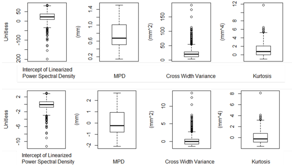
Figure 2.45 Boxplot of four unnormalized statistics (top), boxplot of the same statistics after being converted to standard normal variables (bottom).
