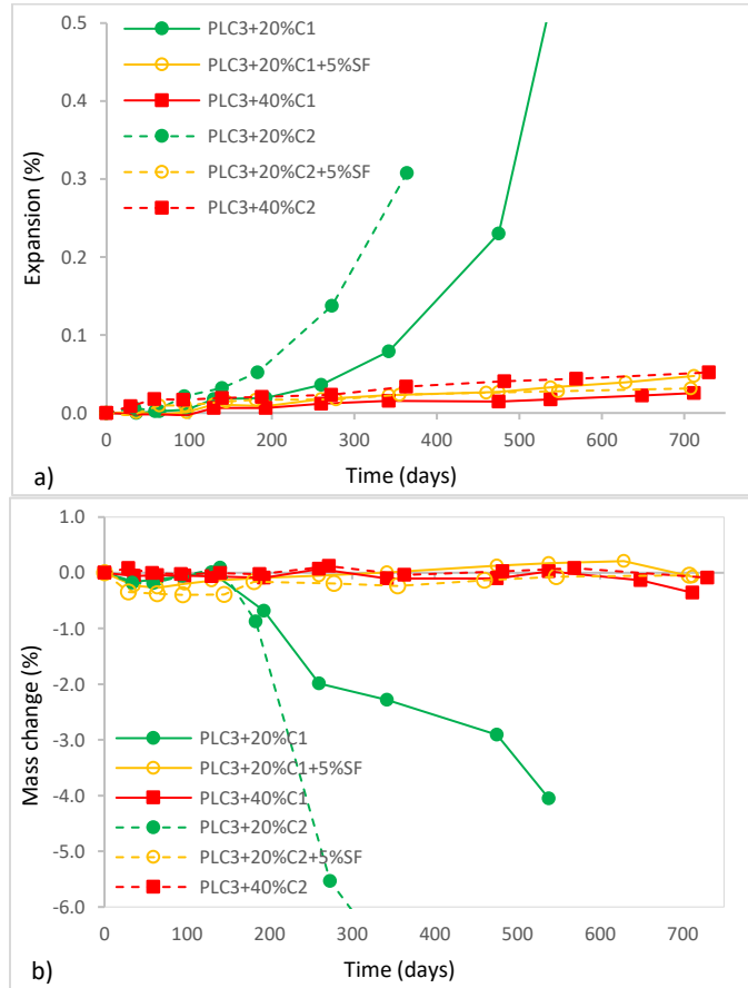
Figure 10.22: Expansion and Mass Data. a) Expansion and, b) mass change data of concrete systems with Class C fly ash fully submerged in the outdoor sodium sulfate trough.
