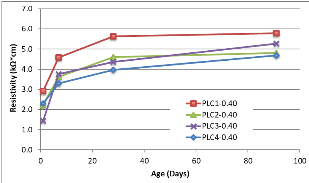
Figure 5.25: Electrical Resistivity vs. Age for PLC1-PLC4 at w/cm = 0.40
