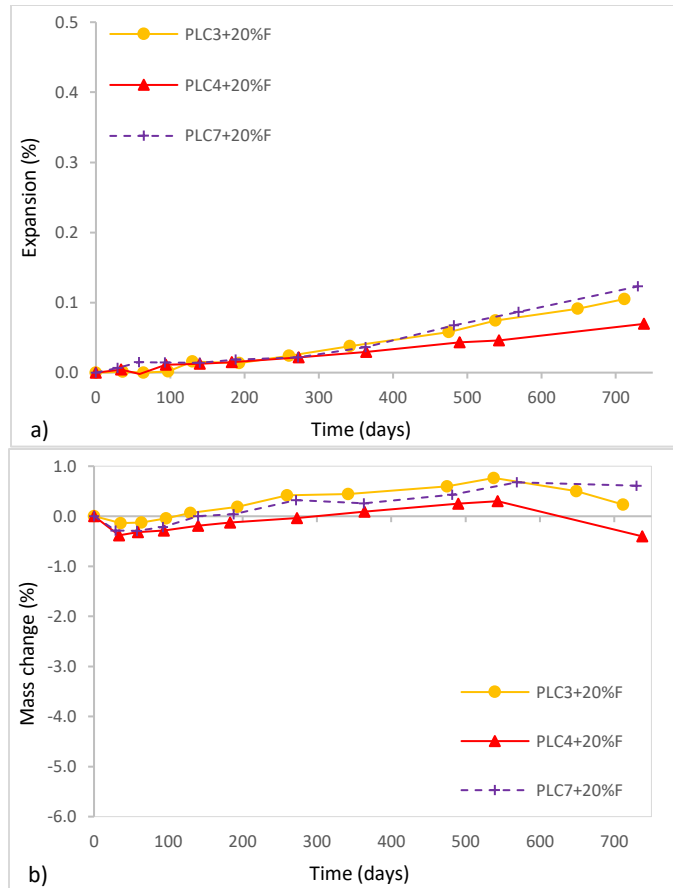
Figure 10.15 Mass Change Plots. a) Expansion and b) mass change data of concrete systems with 20% Class F fly ash fully submerged in the outdoor sodium sulfate trough.
