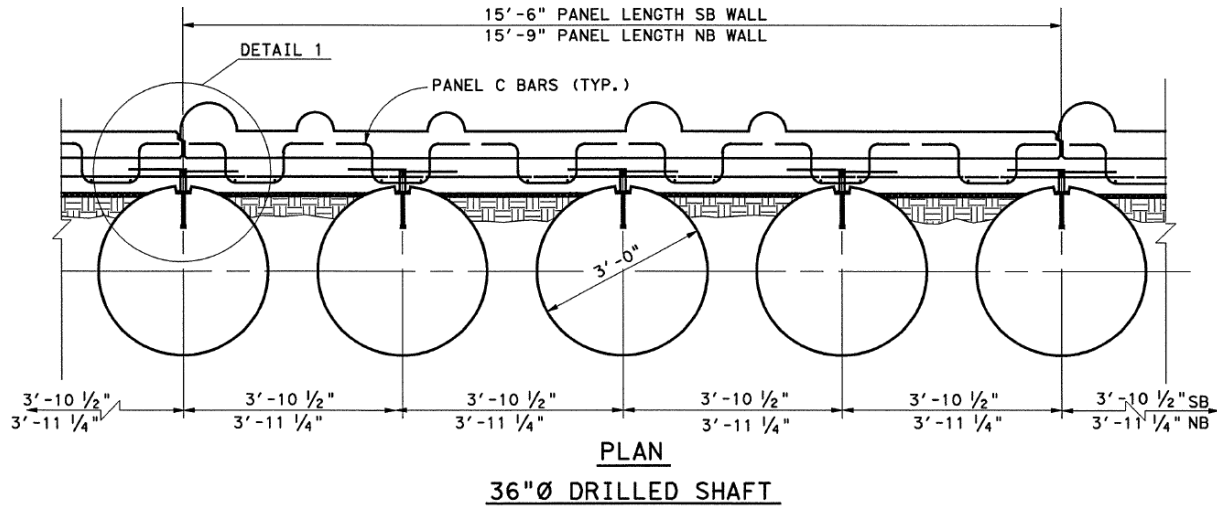
Figure 3.16: Shaft spacing.
