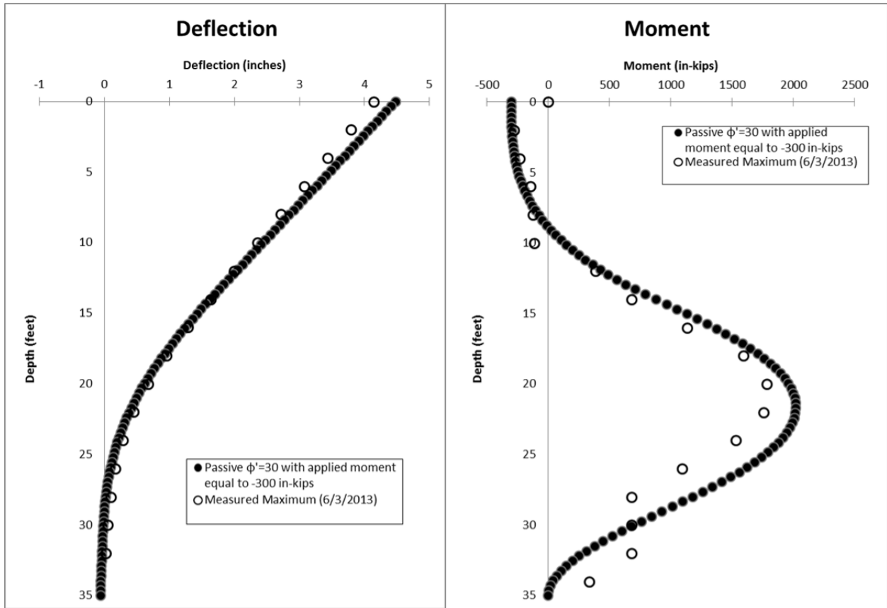
Figure 6.24: Calculated wall response from LPILE with apparent moment applied to account for thermal effects for long-term loading condition.
