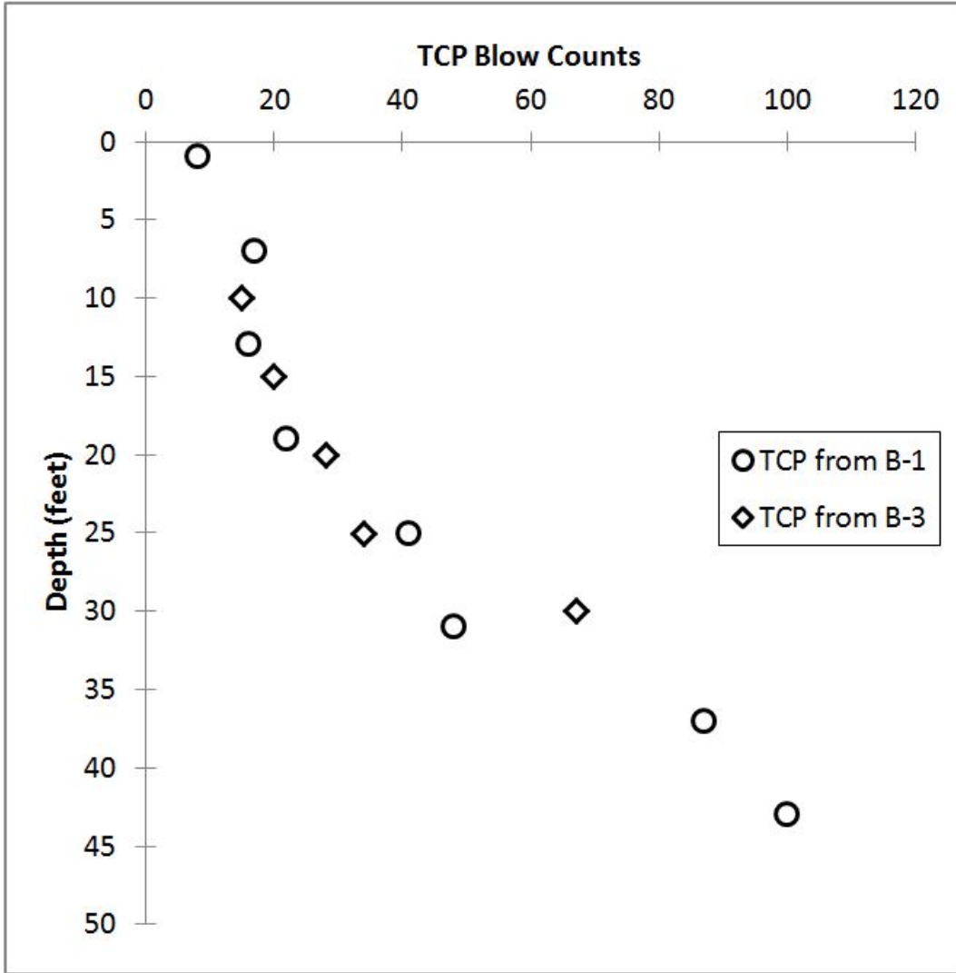
Figure 4.4: TCP blow counts versus depth.
