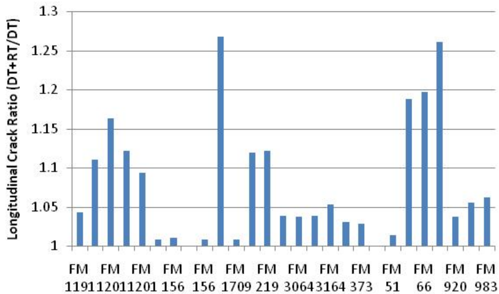
Figure A2.49: Ratio of Longitudinal Cracks on FM Sections due to Rig Traffic (for 365 Natural Gas Site Installations over a 20-Year Analysis Period)
