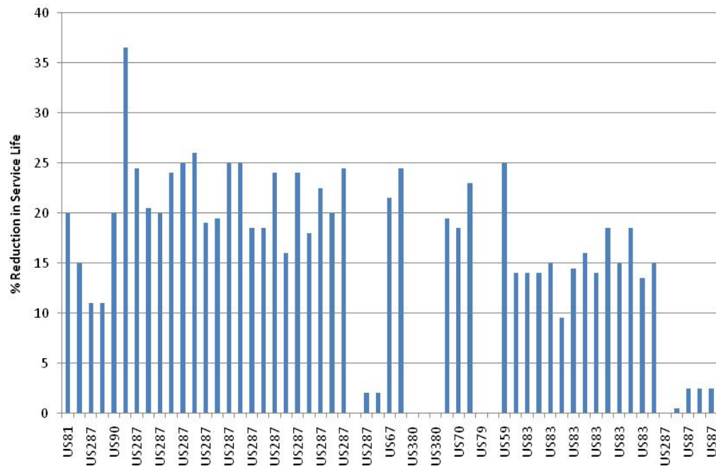
Figure A3.2: Reduction in Service Life of US Highway Sections due to Wind Turbine Truck Traffic
