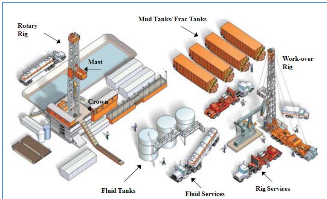
Figure 2.16: Rig Site
