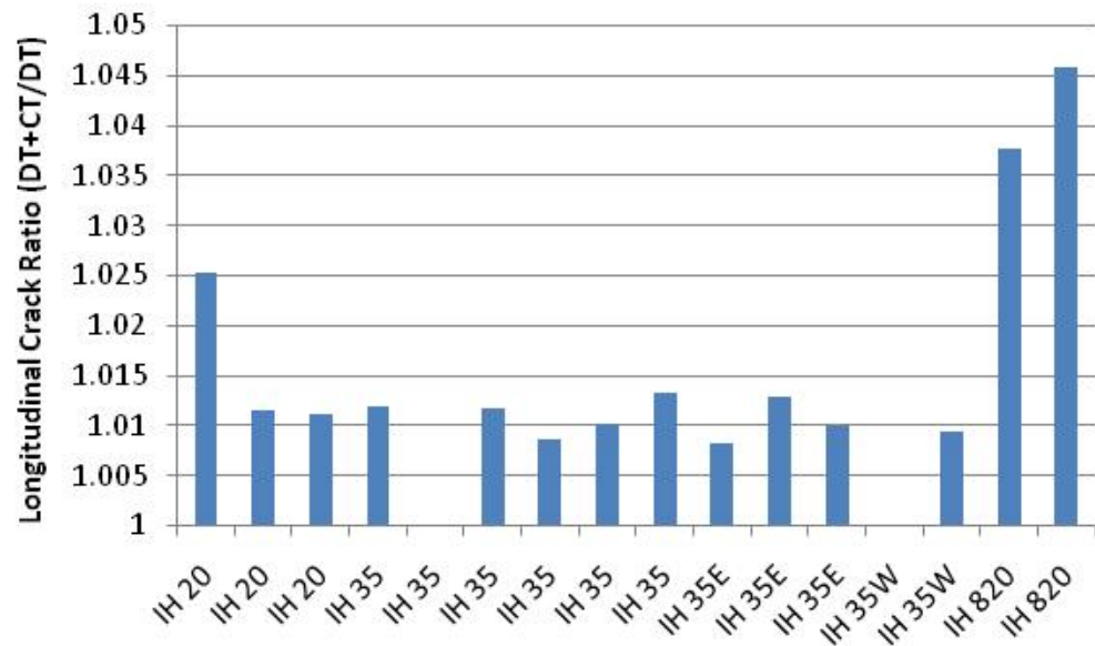
Figure A2.21: Ratio of Longitudinal Cracks on IH Sections due to Construction Traffic (for 10 Natural Gas Wellheads over a 20-Year Analysis Period)
