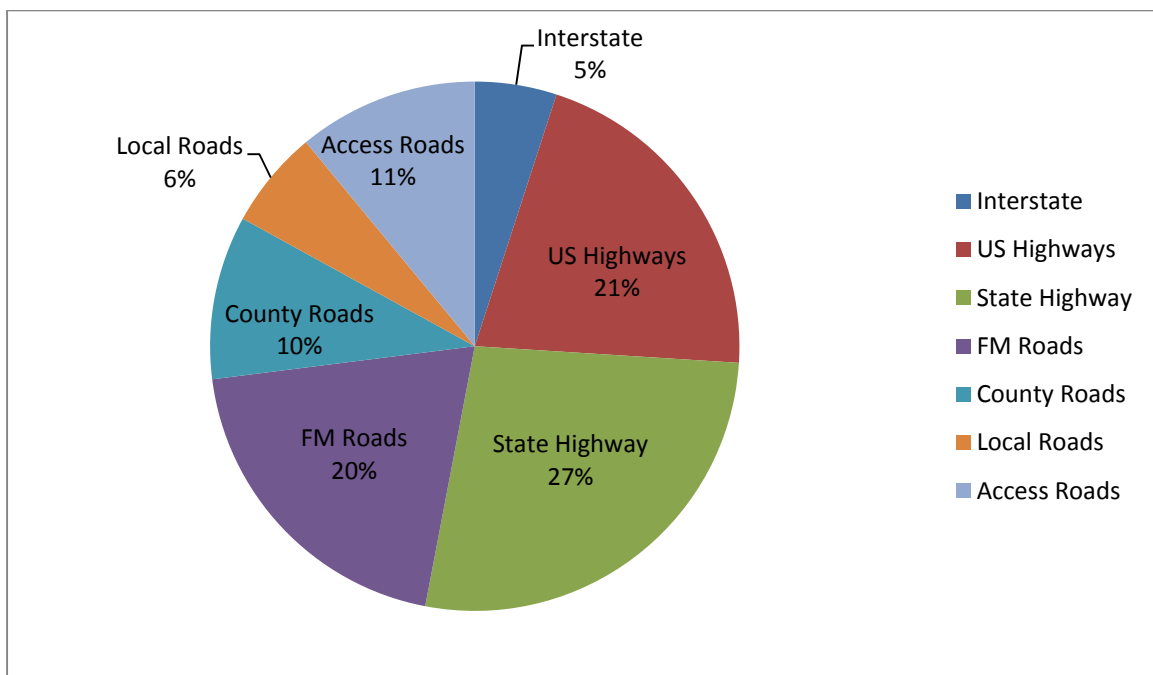
Figure 2.27: Facility Usage by Oil Production Traffic in the Permian Basin
