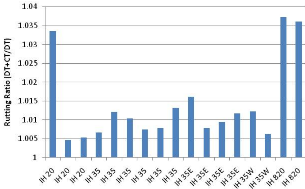
Figure A2.23: Ratio of Rut Depths on IH Sections due to Construction Traffic (for 10 Natural Gas Wellheads over a 20-Year Analysis Period)
