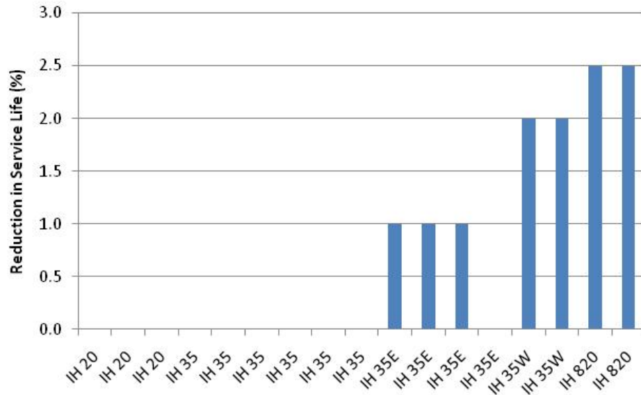
Figure A3.4: Reduction in Service Life of IH Sections in the Barnett Shale Region due to Rig Traffic (for 365 Natural Gas Site Installations over a 20-Year Analysis Period)
