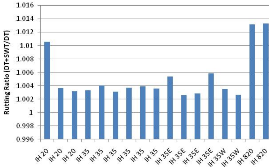
Figure 3.11: Ratio of the Permanent Deformation of IH Sections due to Saltwater Traffic (for 10 Natural Gas Wellheads over a 20-year Analysis Period)
