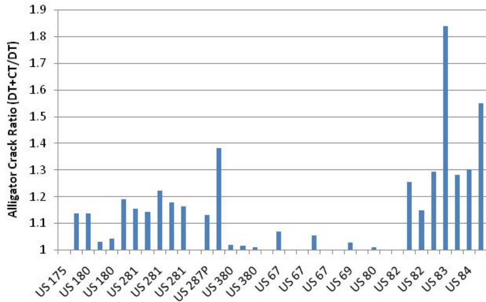
Figure A2.34: Ratio of Alligator Cracks on US Highway Sections due to Construction Traffic (for 10 Natural Gas Wellheads over a 20-Year Analysis Period)
