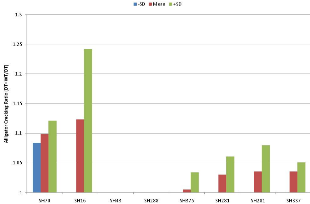
Figure A2.10: Ratio of Alligator Cracks on State Highway Sections at the End of a 20-Year Analysis Period
