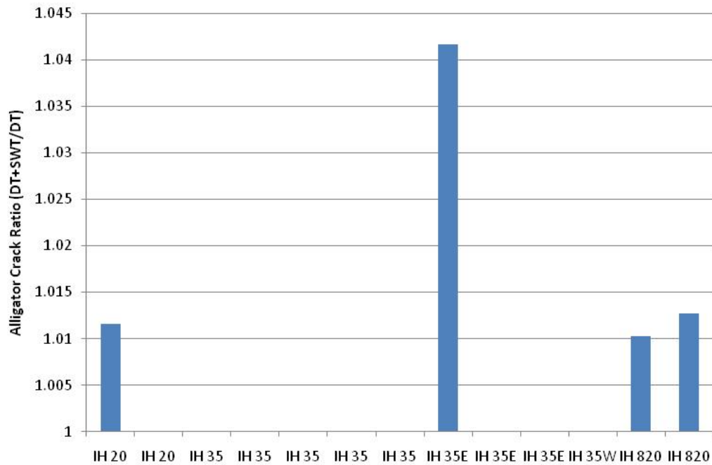
Figure A2.18: Ratio of Alligator Cracks on IH Sections due to Saltwater Traffic (for 10 Natural Gas Wellheads over a 20-Year Analysis Period)
