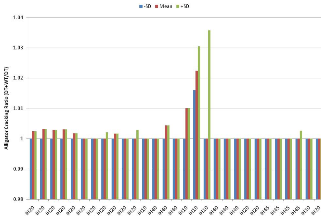
Figure 3.6: Damage Parameter for Alligator Cracking—IH Sections at the End of 20 Years
