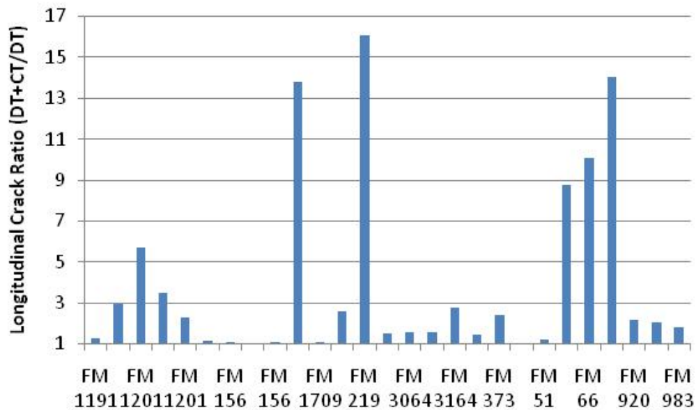
Figure A2.57: Ratio of Longitudinal Cracks on FM Sections due to Construction Traffic (for 10 Natural Gas Wellheads over a 20-Year Analysis Period)
