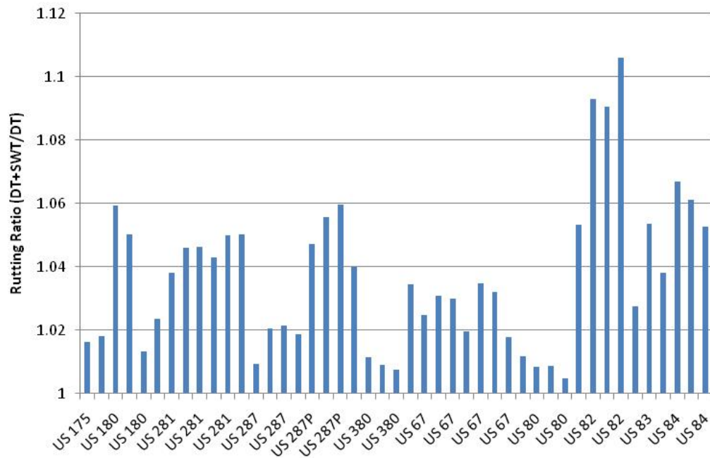
Figure A2.31: Ratio of Rut Depths on US Highway Sections due to Saltwater Traffic (for 10 Natural Gas Wellheads over a 20-Year Analysis Period)
