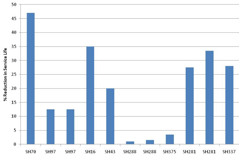
Figure A3.3: Reduction in Service Life of State Highway Sections due to Wind Turbine Truck Traffic
