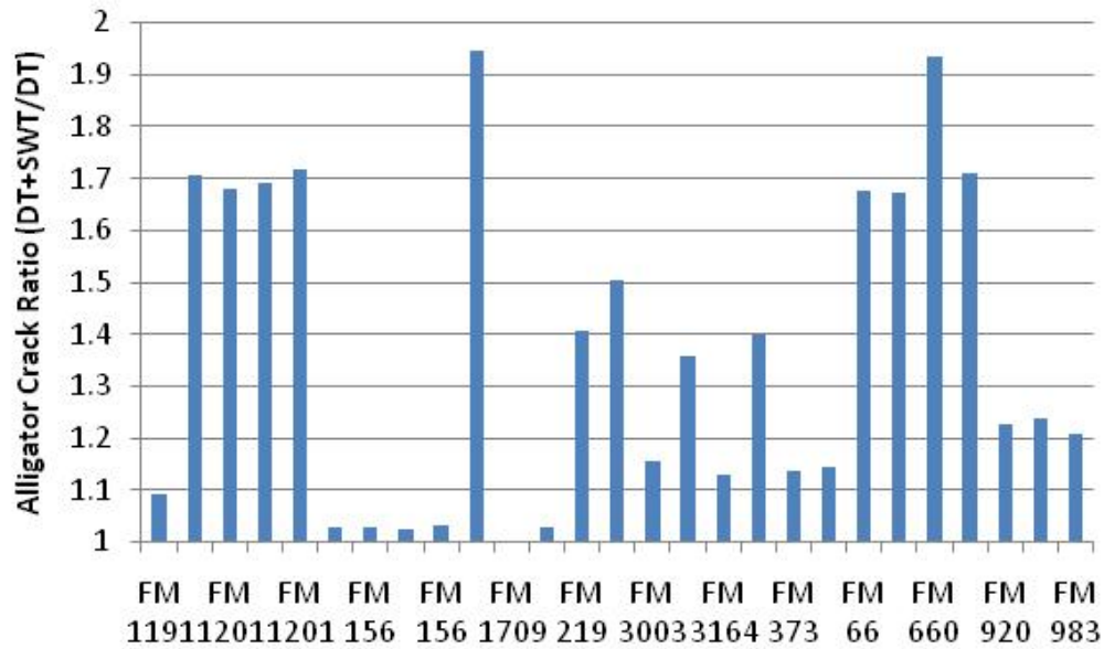
Figure A2.54: Ratio of Alligator Cracks on FM Sections due to Saltwater Traffic (for 10 Natural Gas Wellheads over a 20-Year Analysis Period)
