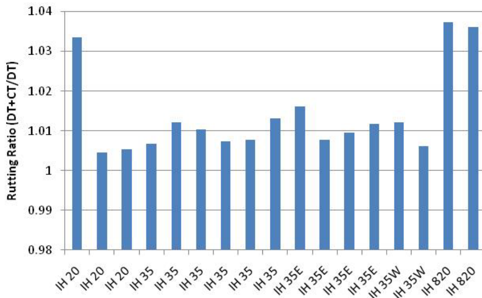
Figure 3.10: Ratio of the Permanent Deformation of IH Sections due to Construction Traffic (for 10 Natural Gas Wellheads over a 20-year Analysis Period)
