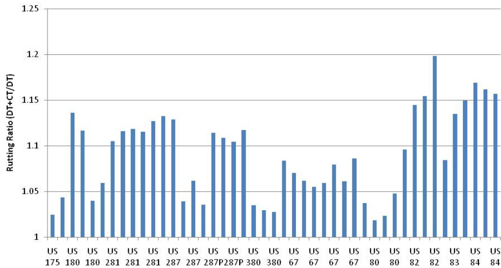
Figure A2.35: Ratio of Rut Depths on US Highway Sections due to Construction Traffic (for 10 Natural Gas Wellheads over a 20-Year Analysis Period)
