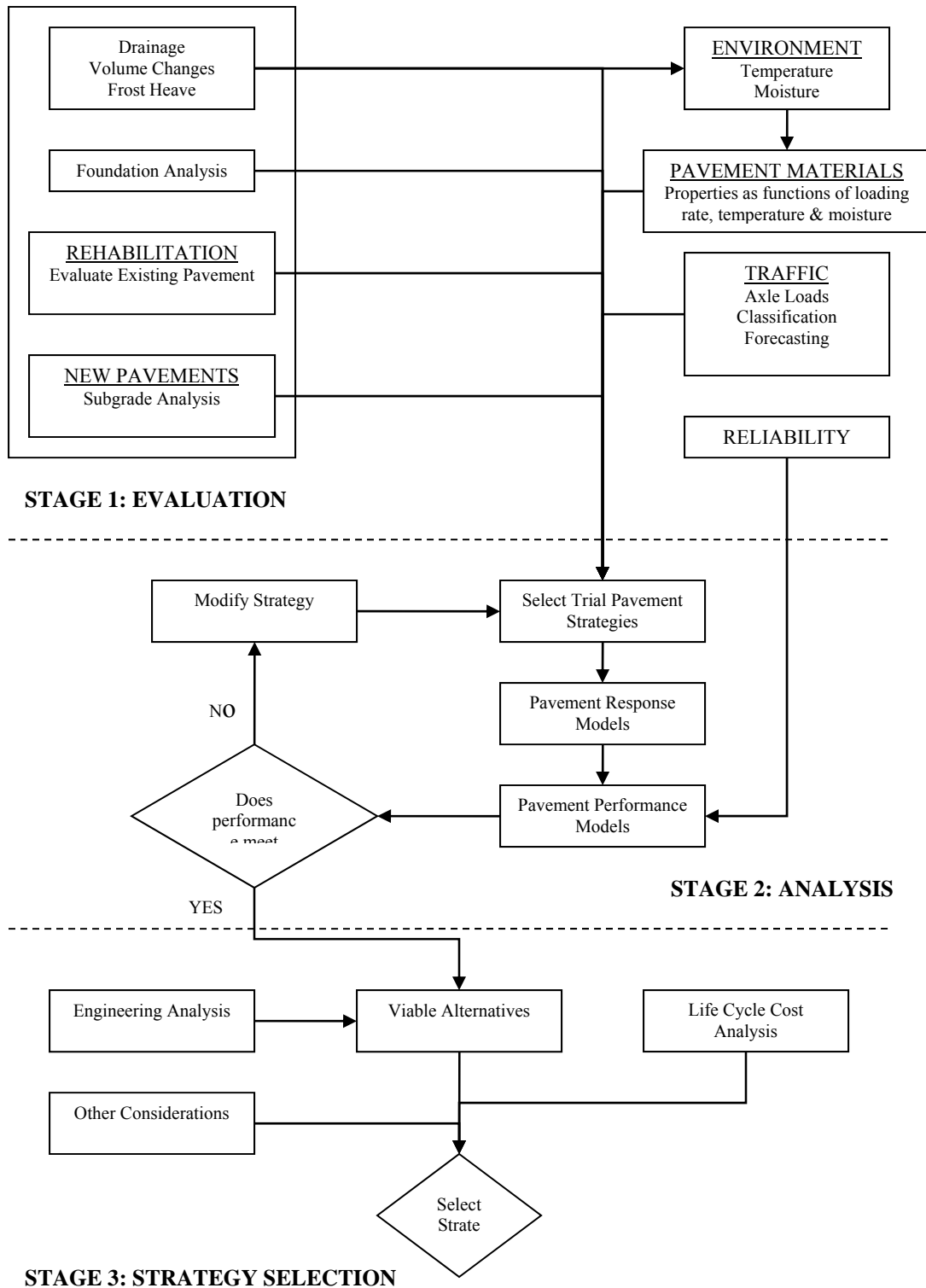
Figure A4.1: MEPDG Design Procedure (ARA, 2004)
