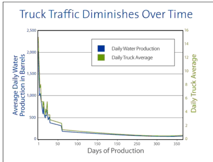
Figure 2.7: Truck Traffic Generated by Saltwater Production
