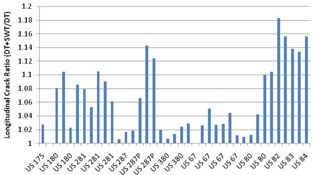
Figure A2.29: Ratio of Longitudinal Cracks on US Highway Sections due to Saltwater Traffic (for 10 Natural Gas Wellheads over a 20-Year Analysis Period)
