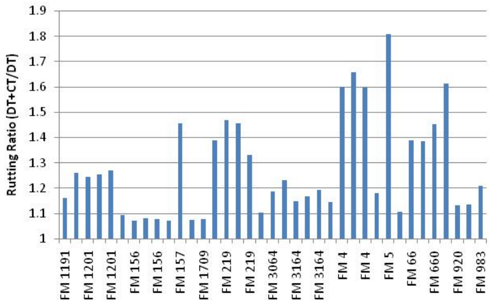
Figure A2.59: Ratio of Rut Depths on FM Sections due to Construction Traffic (for 10 Natural Gas Wellheads over a 20-Year Analysis Period)
