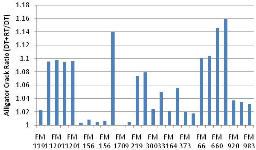
Figure A2.50: Ratio of Alligator Cracks on FM Sections due to Rig Traffic (for 365 Natural Gas Site Installations over a 20-Year Analysis Period)
