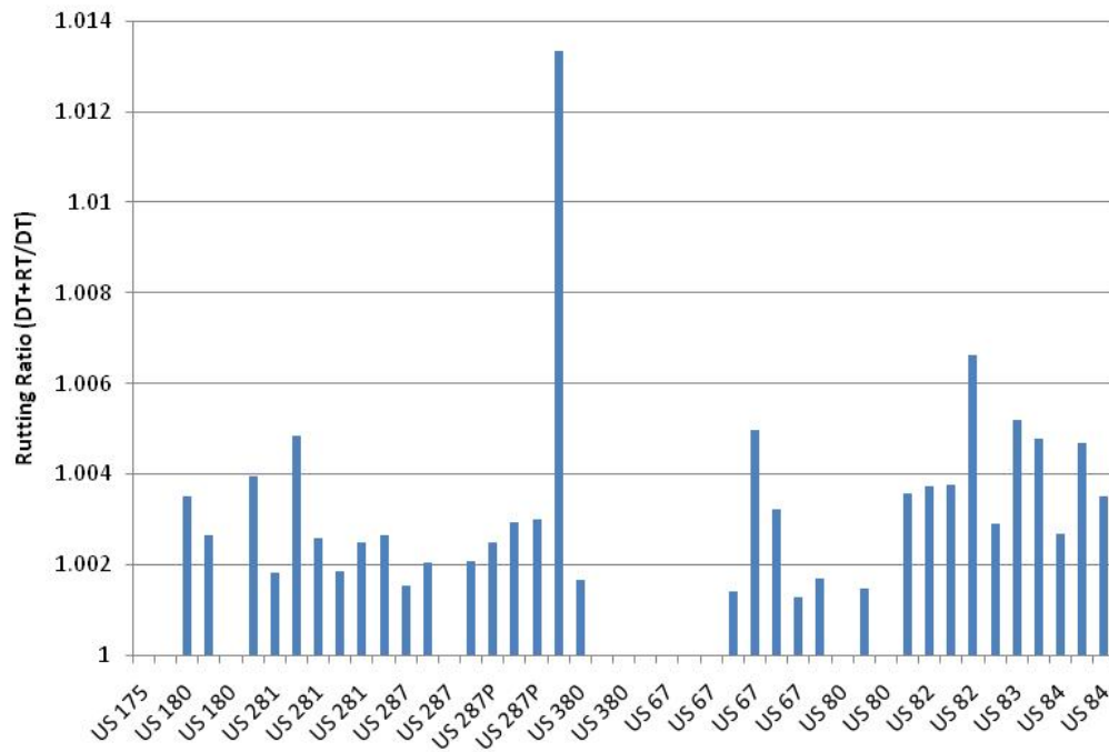
Figure A2.27: Ratio of Rut Depths on US Highway Sections due to Rig Traffic (for 365 Natural Gas Site Installations over a 20-Year Analysis Period)
