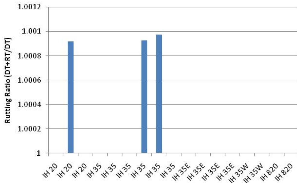
Figure A2.15: Ratio of Rut Depths on IH Sections due to Rig Traffic (for 365 Natural Gas Site Installations over a 20-Year Analysis Period)
