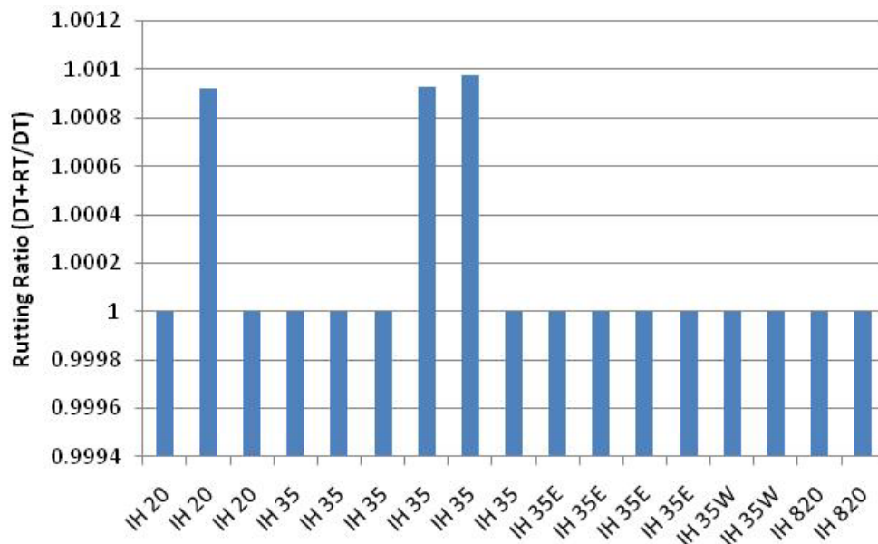
Figure 3.9: Ratio of the Permanent Deformation of IH Sections due to Rig Traffic (for 365 Natural Gas Site Installations over a 20-year Analysis Period)
