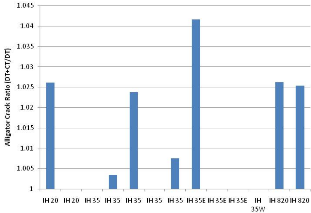
Figure A2.22: Ratio of Alligator Cracks on IH Sections due to Construction Traffic (for 10 Natural Gas Wellheads over a 20-Year Analysis Period)
