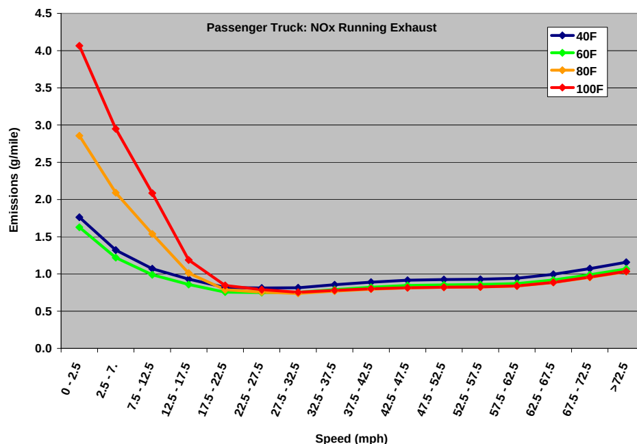
Figure C8: Average running exhaust \text{NO}_x emission rates (g/mile) for ambient temperatures of 40°F, 60°F, 80°F, and 100°F for gasoline passenger trucks (model year 2010, restricted urban roads) binned by vehicle speed
