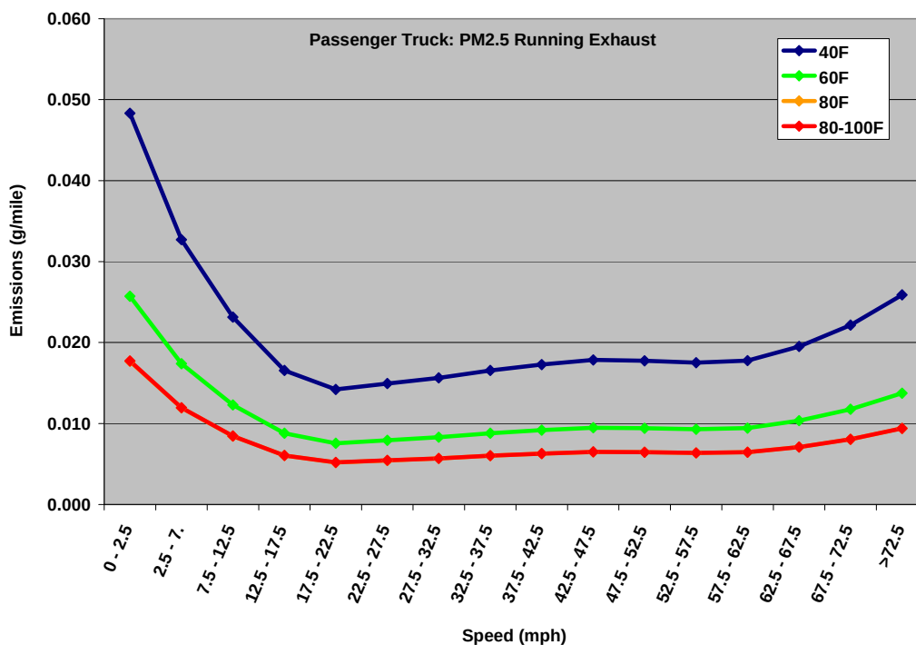
Figure C9: Average running exhaust \text{PM}_{2.5} emission rates (g/mile) for ambient temperatures of 40°F, 60°F, 80°F, and 100°F for gasoline passenger trucks (model year 2010, restricted urban roads) binned by vehicle speed
