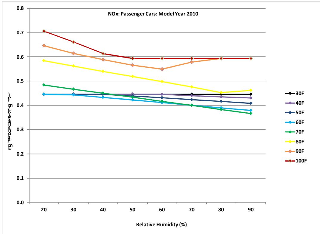
Figure C6: Average \text{NO}_x emission rates (g/mile) versus relative humidity for gasoline passenger cars (model year 2010, unrestricted urban roads) by constant temperature
