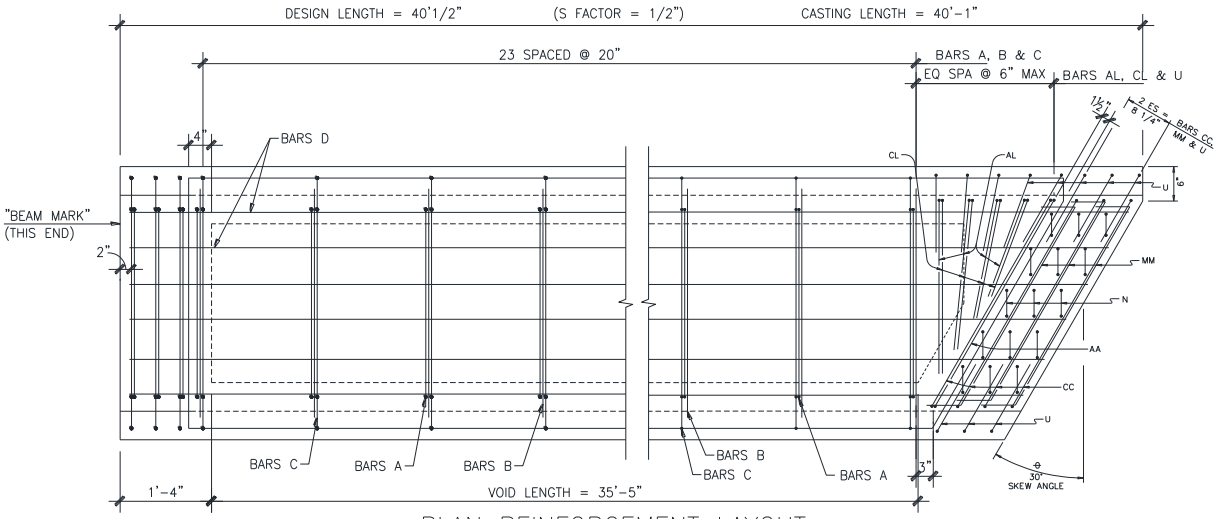
PLAN REINFORCEMENT LAYOUT
