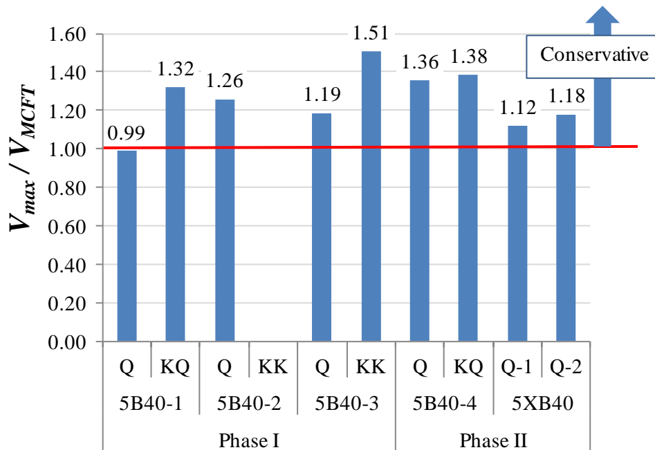
Figure 6-11: Shear Strength Ratios for 5B40 box beam series
