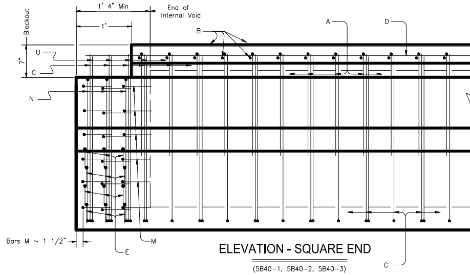
Figure B-9: Cross sections and elevations. Beams 5B40-1, 5B40-2 and 5B40-3
