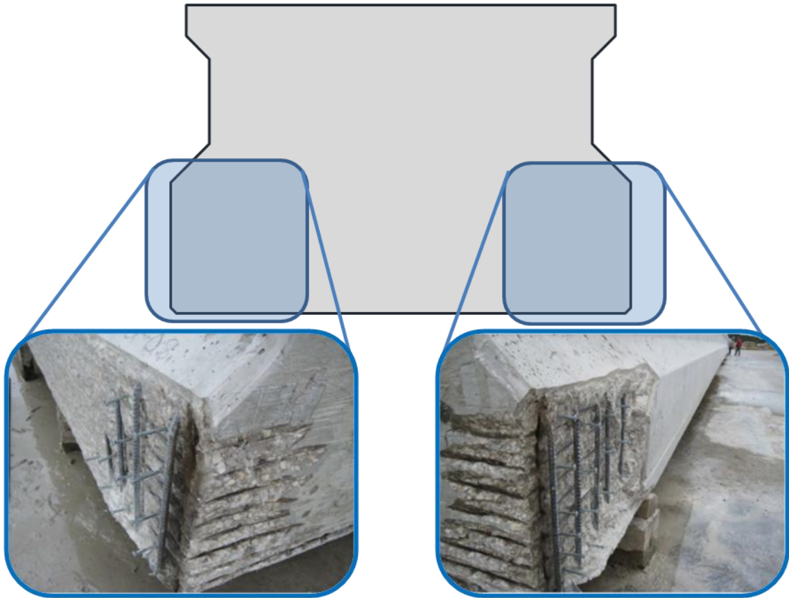
Figure 5-2: Spalling of concrete cover immediately after prestress transfer
