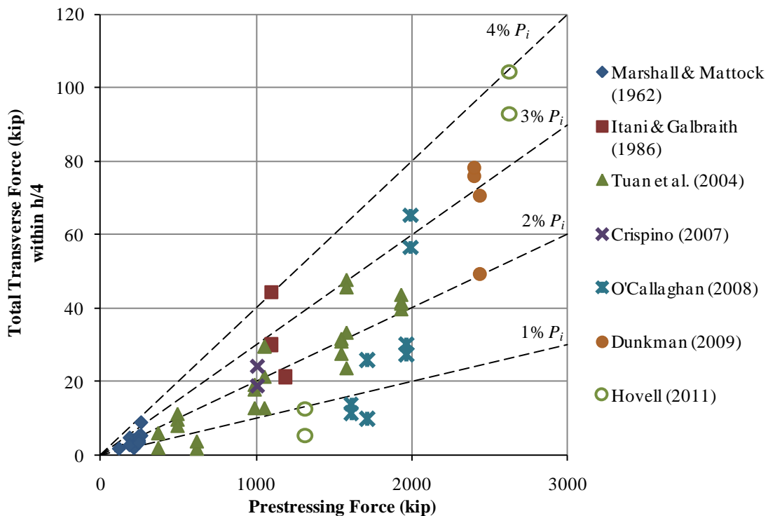
Figure 2-18: Results from experimental studies on Transverse Forces
