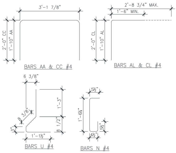
Figure B-1: Reinforcement bars for all 4B28 box beams.
