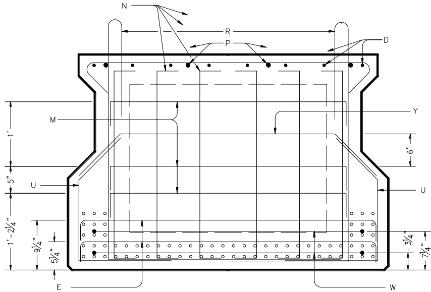
SECTION THRU BLOCKOUT ~ TYPE 5XB40
