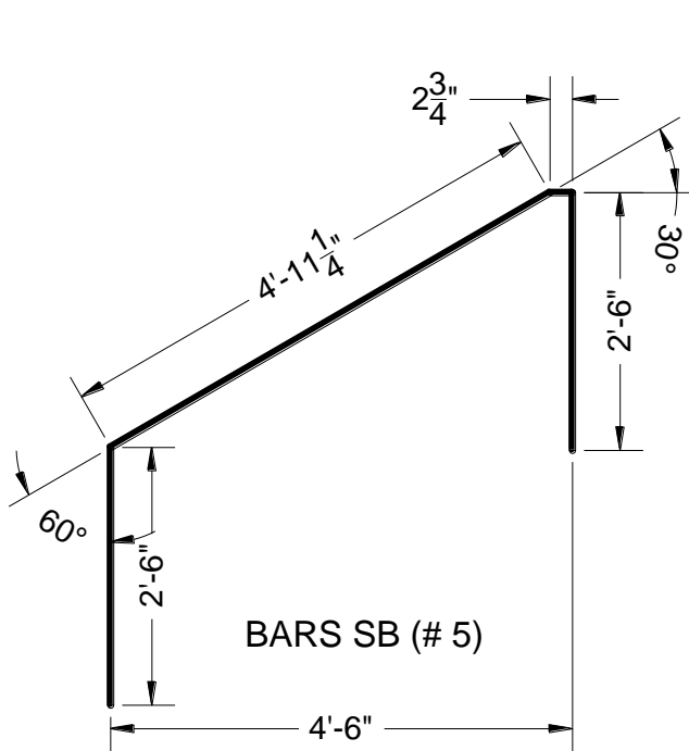
Figure B-13: New Reinforcement Bars Details. Beam 5B40-4
