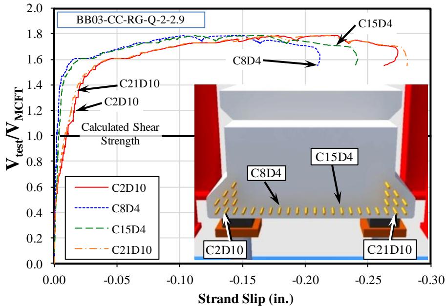
Figure 4-17: Load vs. Strand Slip curves (Instrumentation Configuration C)
