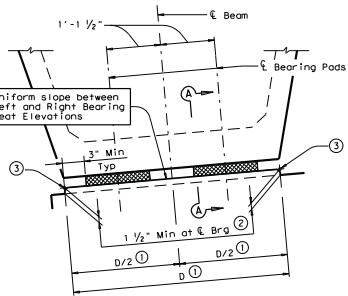
BEARING SEAT DETAIL Looking up-station with two-pad condition.
