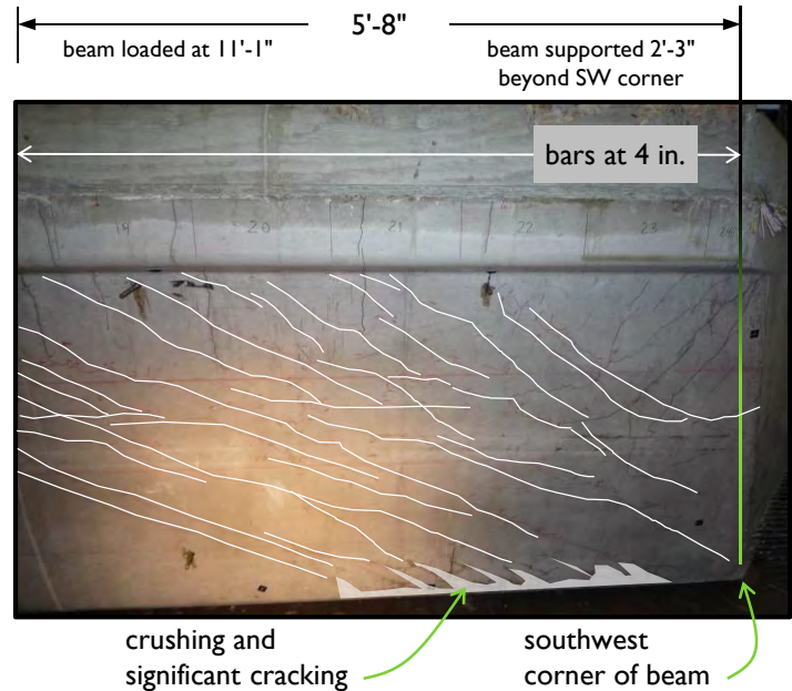
Figure 4-3: Test region B1S after failure of end region.
