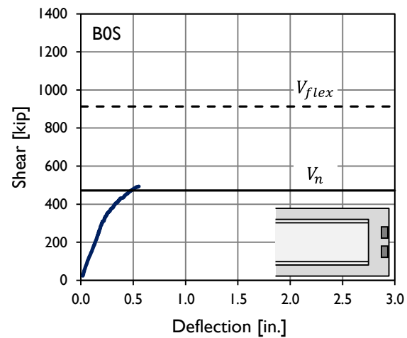
Figure B-44: Shear-deflection plot for specimen BOS.
