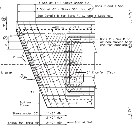
PLAN - SKEWED ENDBLOCK
