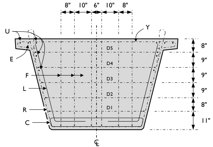
Figure A-28: Beam 5 end-region plan views and cross-sections.
