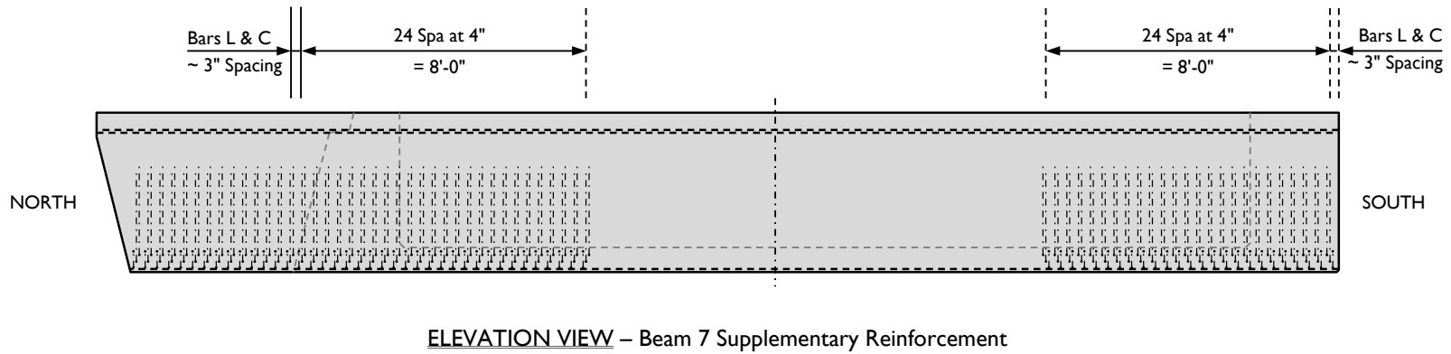
Figure A-35: Beam 7 plan view, elevation view, and sections showing supplementary reinforcement.
