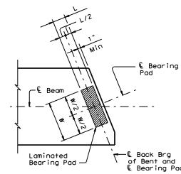
ONE-PAD DETAIL Type U1-"N" Bearing
