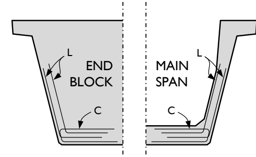
CROSS-SECTIONS – Beam 6
