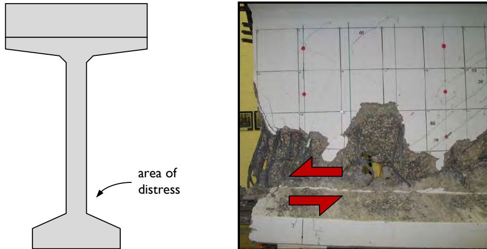
Figure 2-13: Horizontal sliding failure mode seen in several of the BT-63 specimens tested by Nagle and Kuchma (2007).
