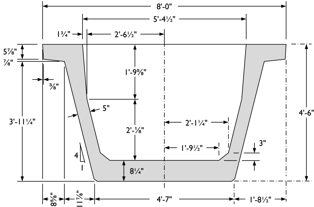
Figure 3-2: Geometry of the Texas U54 beam.
