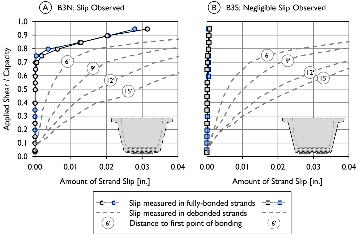
Figure 6-22: Strand slip data gathered during shear tests B3N and B3S.
