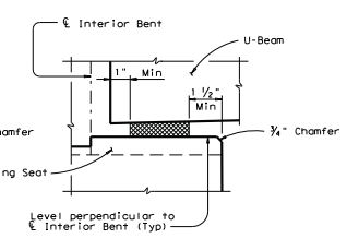
AT CONVENTIONAL BENT
