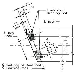
TWO-PAD DETAIL Type U2-"N" Bearing
