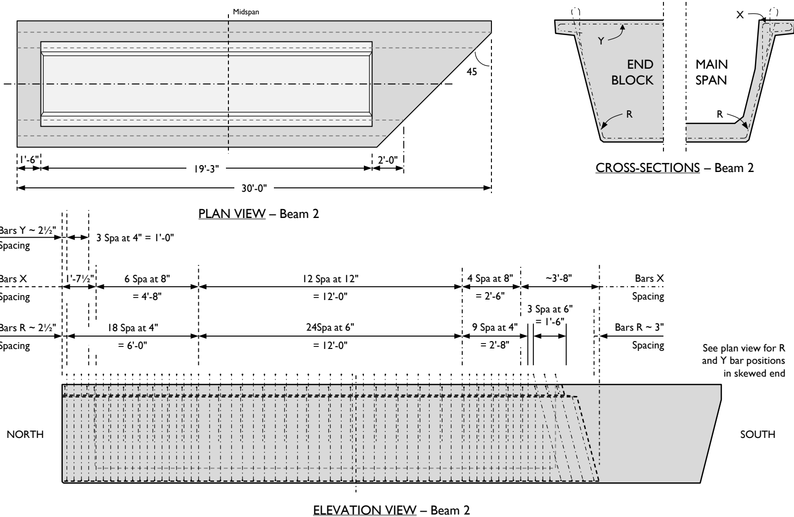
Figure A-12: Beam 2 plan view, elevation view, and standard sections.
