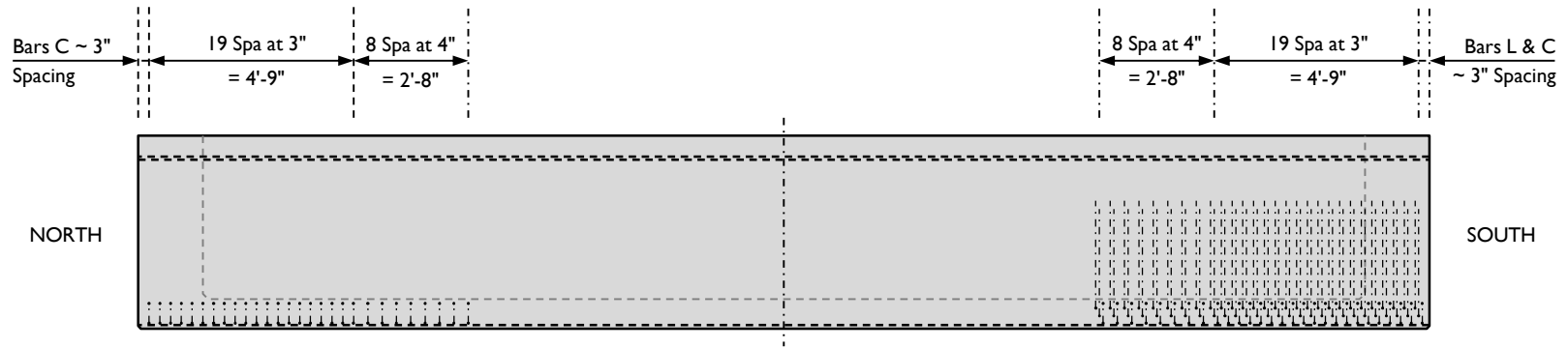
ELEVATION VIEW – Beam 4 Supplementary Reinforcement
