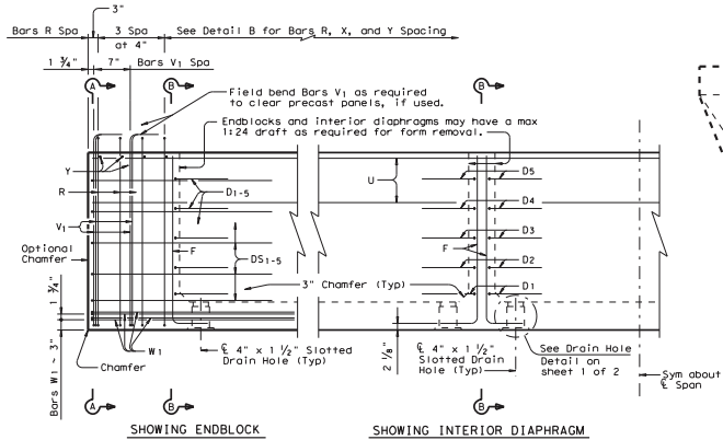
SHOWING ENDBLOCK SHOWING INTERIOR DIAPHRAGM
