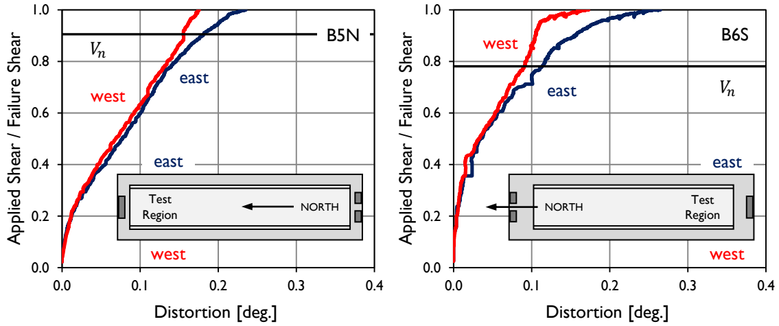
Figure B-7: Distortion measured in the webs during loading of test specimens B5N and B6S.
