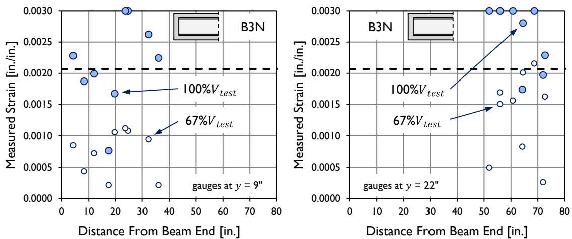
Figure B-40: Strain measured in reinforcing bars during load-testing of specimen B3N.
