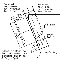
BEAM END DETAIL (At Abutment Backwall or Inverted Tee Stem)
