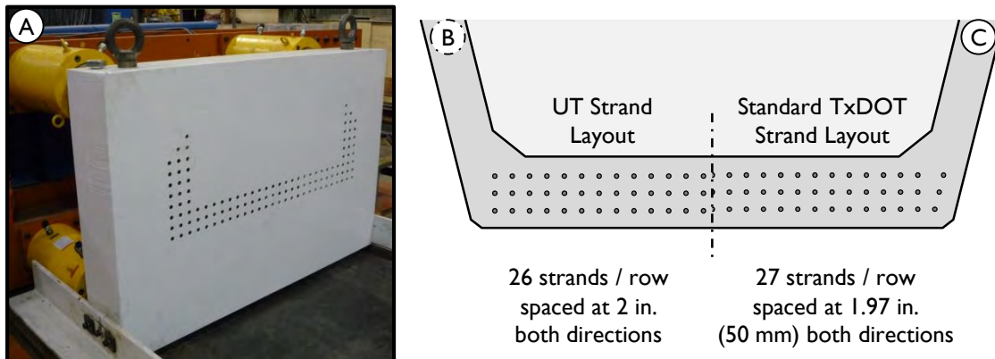
Figure 3-5: (A) Reaction plate at the live end of the prestressing bed at FSEL. (B) Strand layout for UT-fabricated U-Beams and (C) TxDOT standard strand layout.
