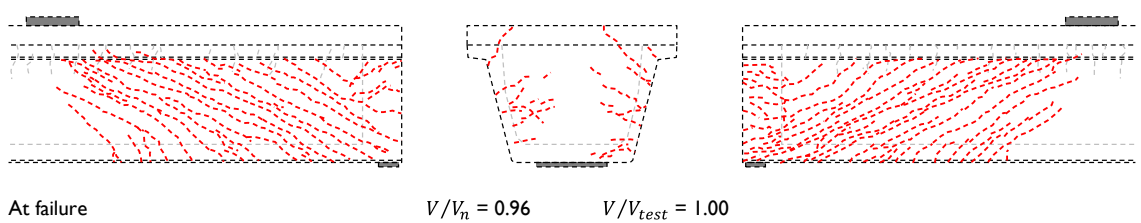
Figure B-20: Cracks observed during testing of specimen B3N.
