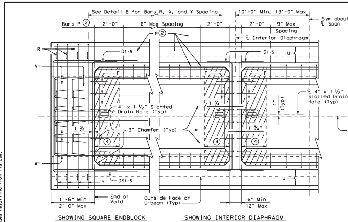
SHOWING SQUARE ENDBLOCK SHOWING INTERIOR DIAPHRAGM
