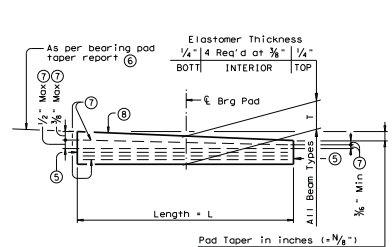
LAMINATED BEARING PAD (50 DURMETER)
