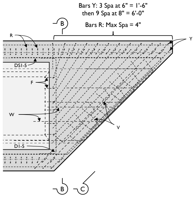
PLAN VIEW - B2S
