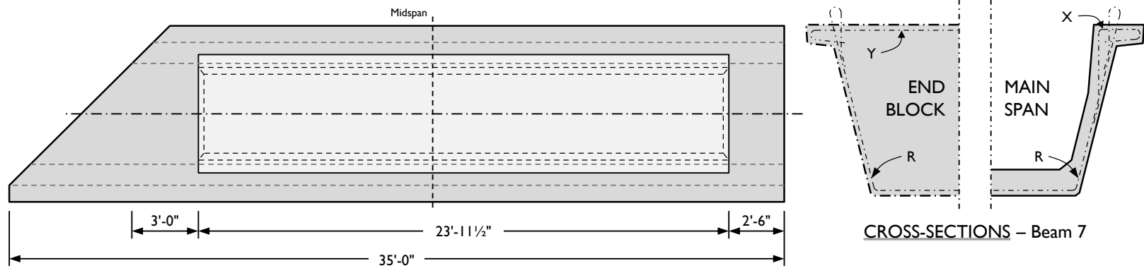
PLAN VIEW – Beam 7
