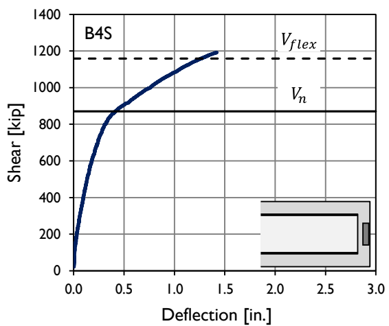
Figure B-48: Shear-deflection plot for specimens B4N and B4S.
