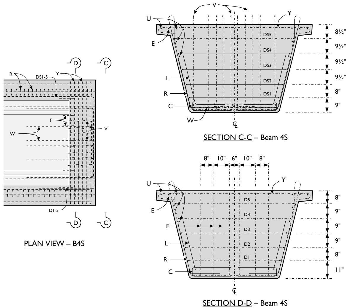
Figure A-23: Beam 4 south end region plan views and cross-sections.
