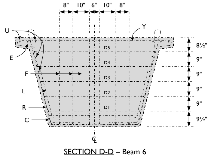
Figure A-32: Beam 6 end-region plan views and cross-sections (2 of 2).
