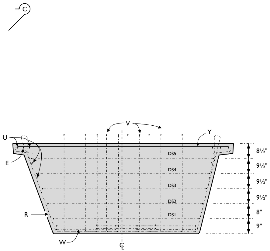
SECTION C-C - Beam 2S
