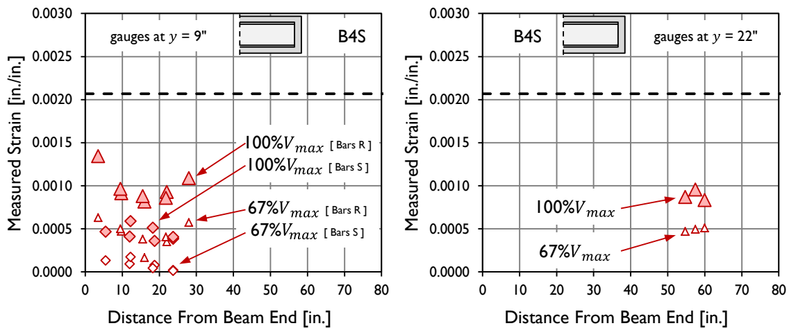
Figure B-43: Strain measured in reinforcing bars during load-testing of specimen B4S.
