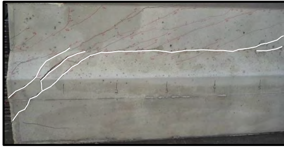
(C) Horizontal shear distress in Texas 5B40 (Avendaño, 2011)
