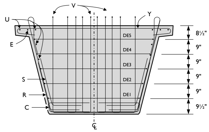
SECTION C-C - Beam 7S
