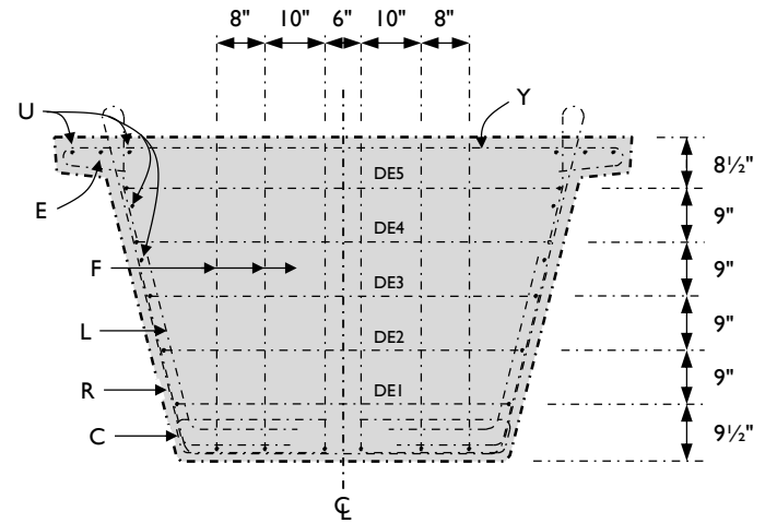
SECTION B-B - Beam 6
