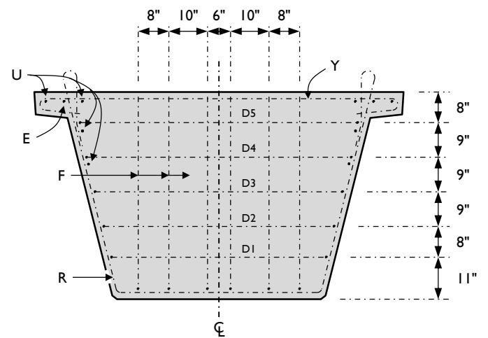
Figure A-18: Beam 3 end-region plan views and cross-sections.
