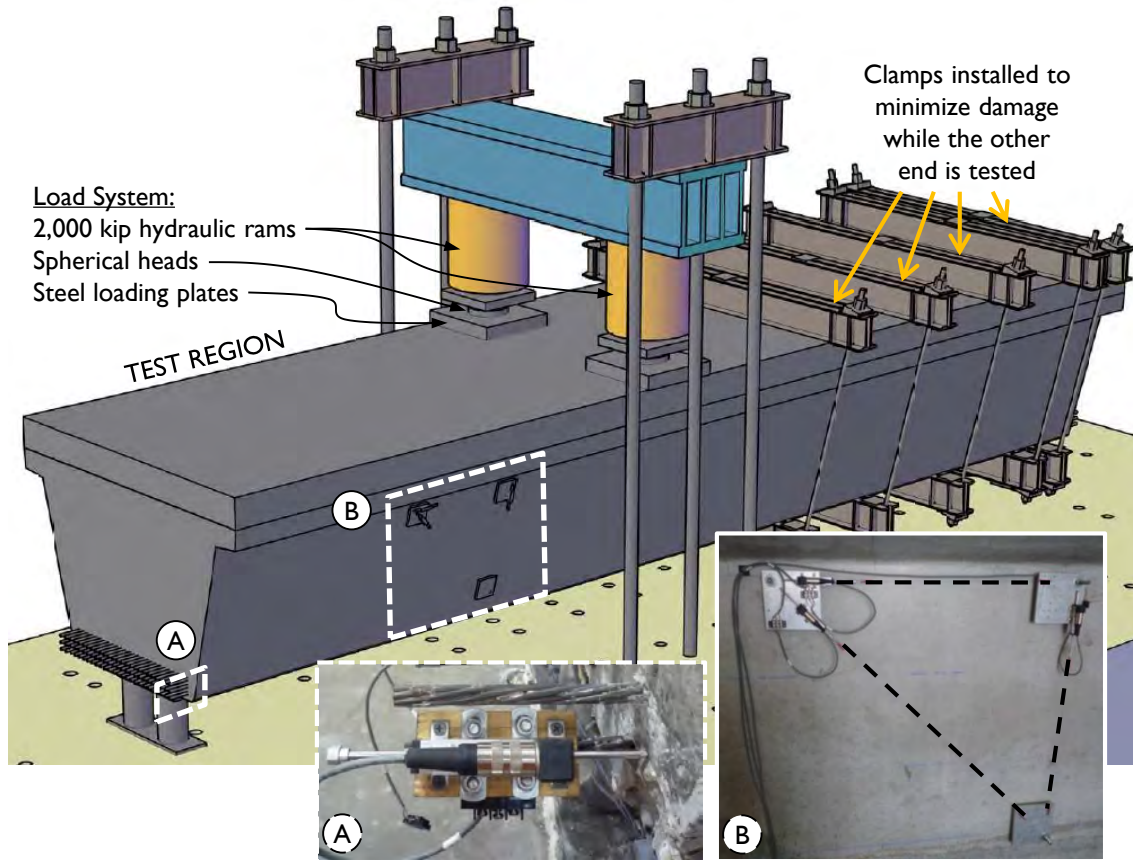
Figure 3-16: Shear testing frame, with pictures of (A) strand slip and (B) shear deformation instrumentation shown.
