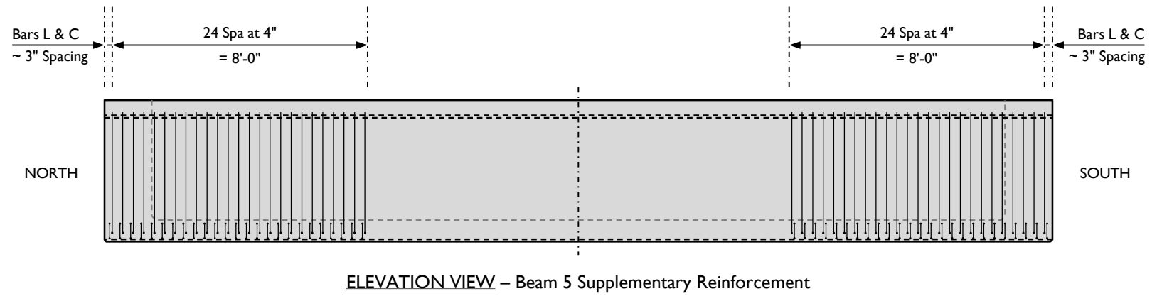
Figure A-27: Beam 5 plan view, elevation view, and sections showing supplementary reinforcement.
