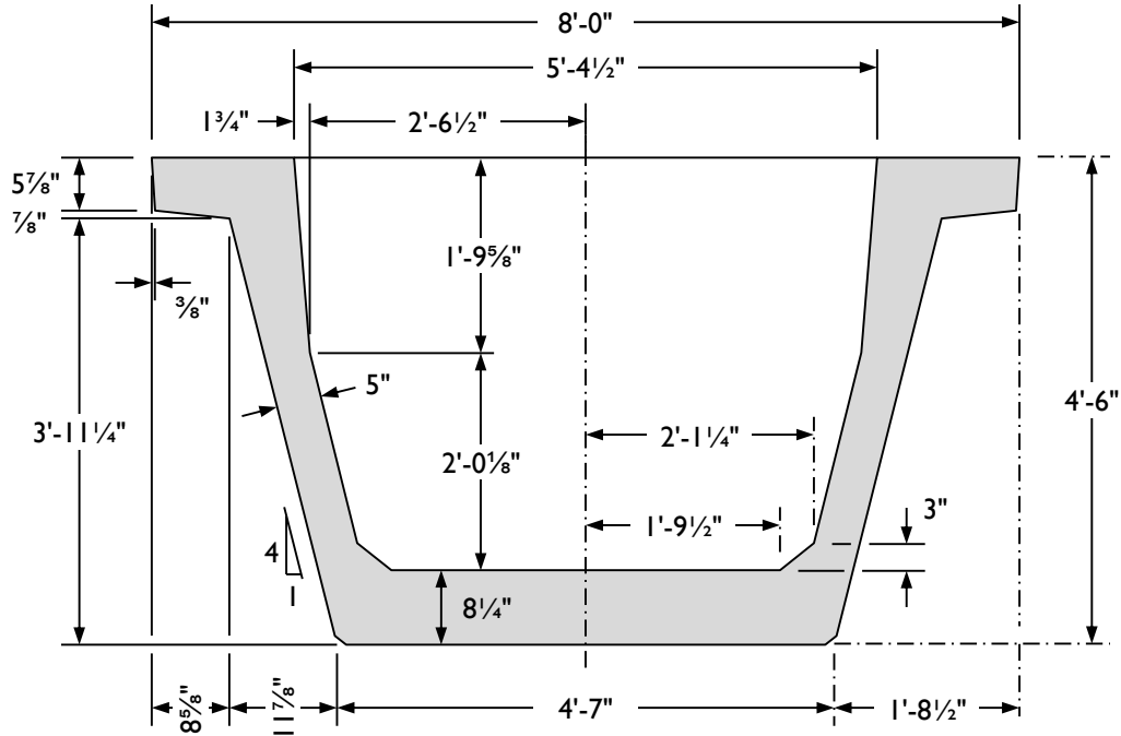
Figure 2-1: Cross-sectional dimensions of the Texas U54 U-Beam.
