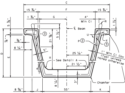
TYPICAL SECTION
