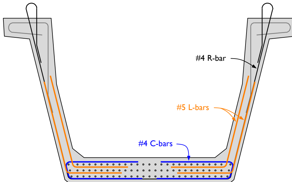
Figure 6-36: Key reinforcing bars in the recommended new Texas U-Beam design.
