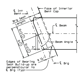
BEAM END DETAIL (At Conventional Bent)
