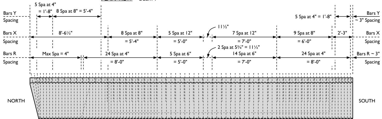
PLAN VIEW – Beam 7
