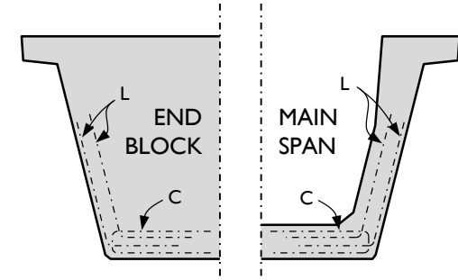
CROSS-SECTIONS – Beam 4
