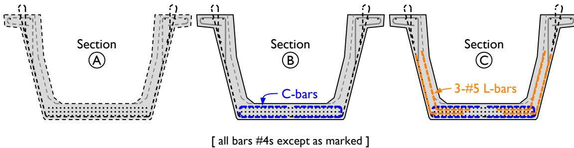
Figure 5-1: (ii) Standard cross sections of Beam 4.
