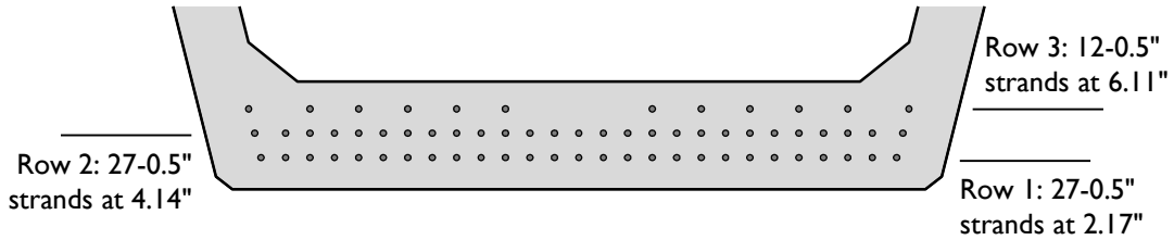
Figure A-25: Prestressing strand positions for Beam 5.
