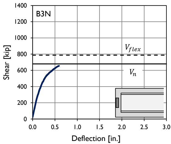
Figure B-47: Shear-deflection plot for specimens B3N and B3S.
