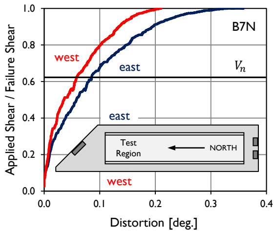
Figure B-8: Distortion measured in the webs during loading of test specimen B7N.
