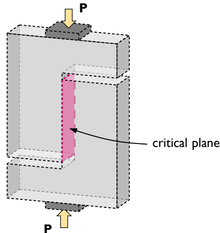
Figure 7-27: Typical push-off specimen as described in literature.
