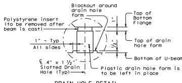
DRAIN HOLE DETAIL
