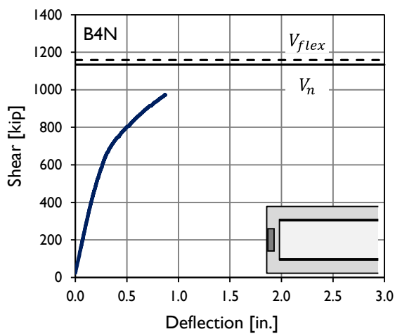
Figure B-48: Shear-deflection plot for specimens B4N and B4S.
