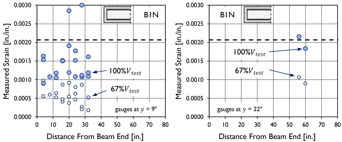
Figure B-38: Strain measured in reinforcing bars during load-testing of specimen B1N.
