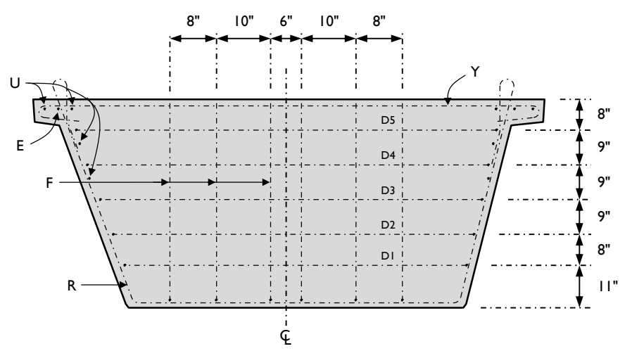
SECTION D-D - Beam 1S
