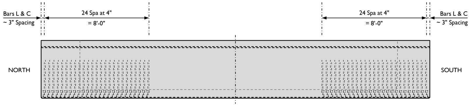
ELEVATION VIEW – Beam 6 Supplementary Reinforcement
