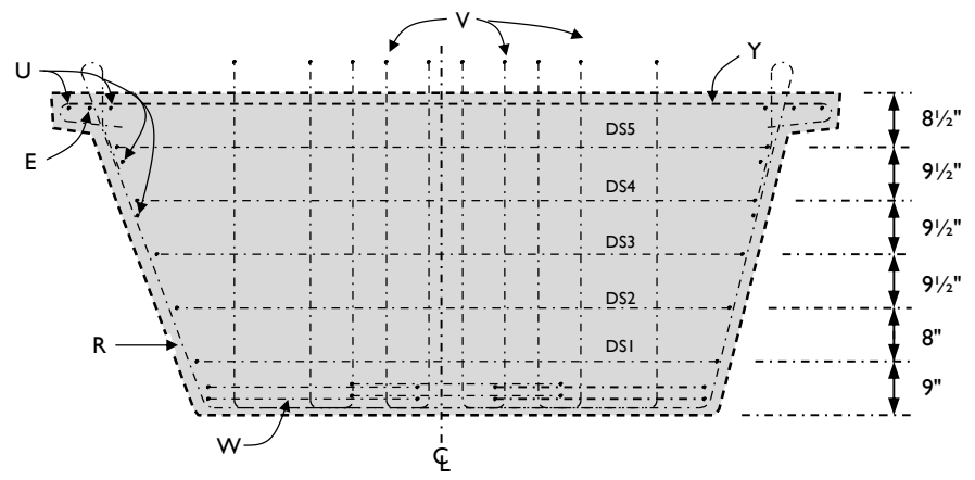
SECTION C-C - Beam 1S
