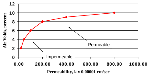
Typical Permeability vs. In-situ Air Voids
