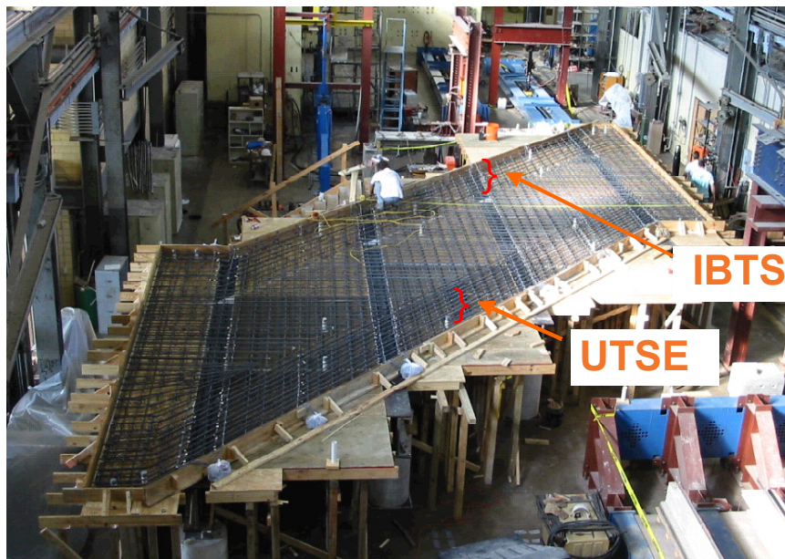
Figure 5: Full-Scale Test Specimen with 45° skew
