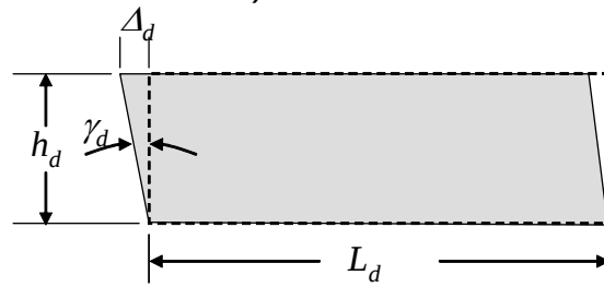
b) Diaphragm Plate Deformations
