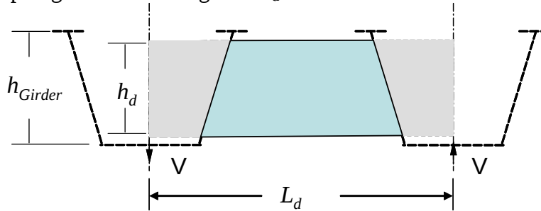
Figure 5.14 Idealized Rectangular Diaphragm Plate
