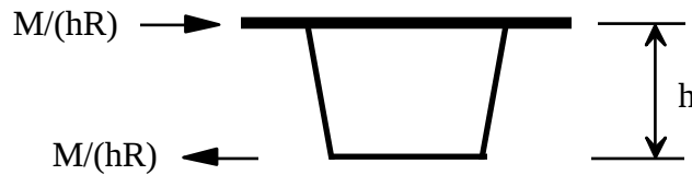
Figure 2.3 Equivalent Torsional Loads on Curved Box Girder
