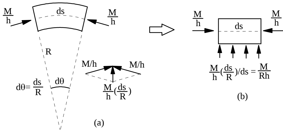
Figure 2.2 Approximation of the Effect of Curvature on Box Girder Flanges
