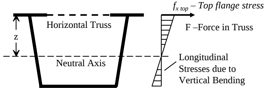
Figure 3.6 Box Girder Vertical Bending Stresses
