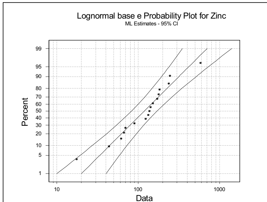
Figure 3-9 Probability Plot for Zinc (µg/L)
