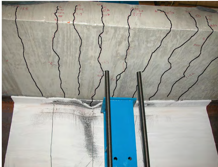
Figure 5.15: Specimen NON-00BS—Cracks in the slab and beam local buckling (11-in. deflection)
