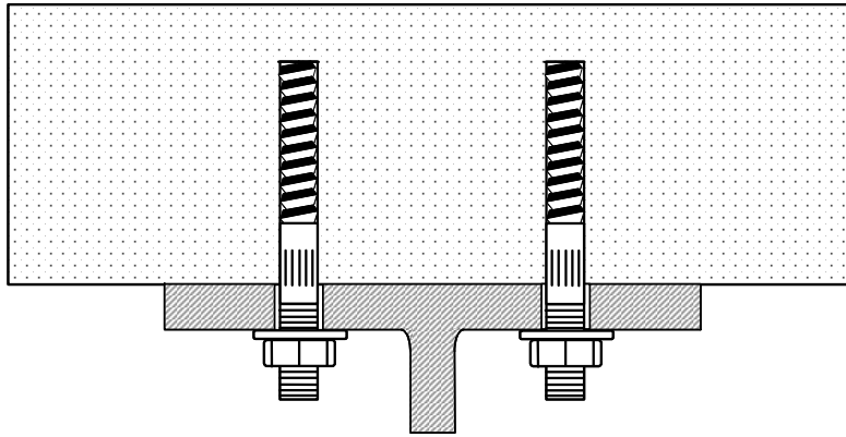
Figure 3.11: HIT-TZ adhesive anchor
