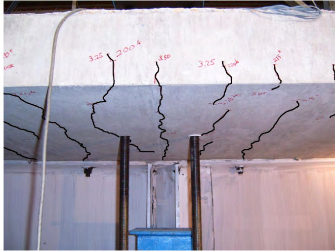
Figure 5.17: Specimen DBLNB-30BS—Cracks on the bottom of the concrete slab (3.25-in deflection)
