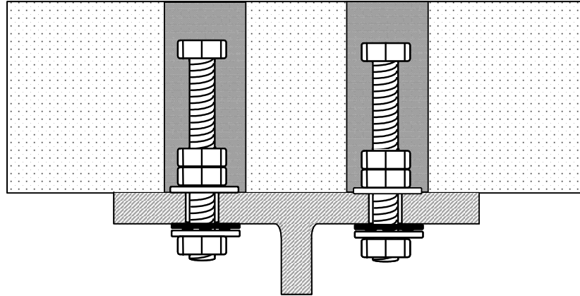
Figure 3.5: Double-nut bolt
