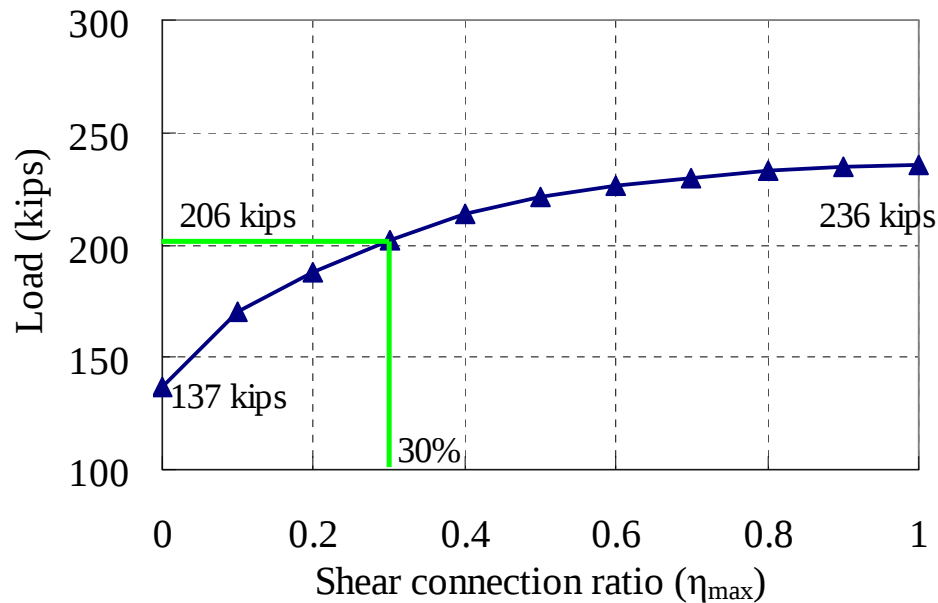
Figure 5.4: Predicted load capacity of test specimens versus shear connection ration (based on minimum specified material properties)
