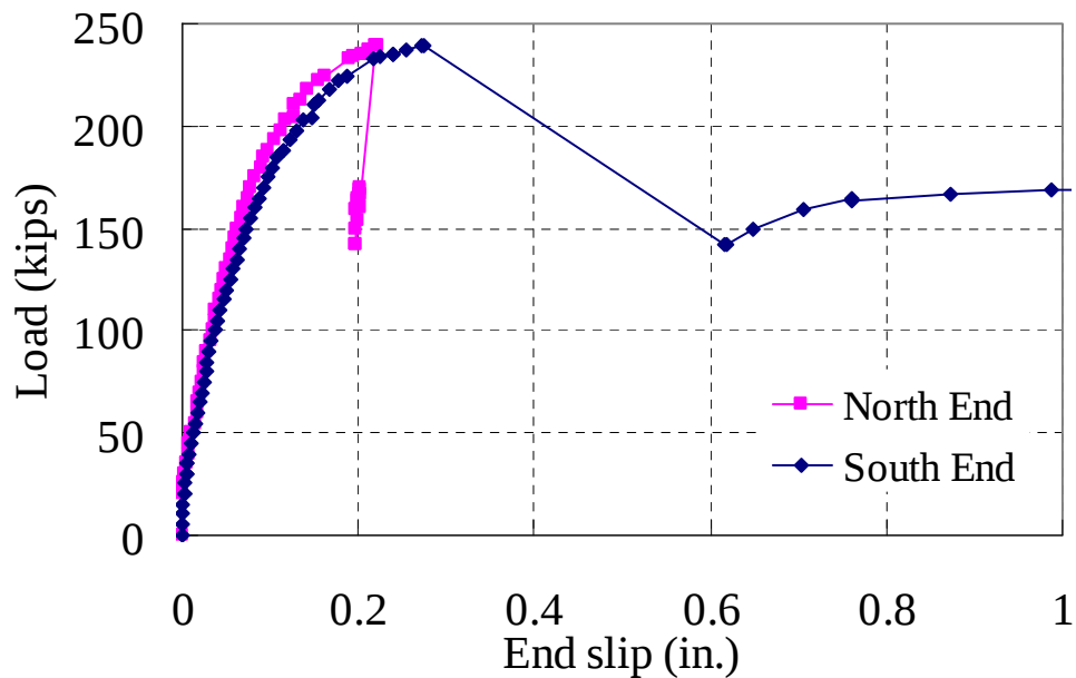
Figure 5.25: Slip at the ends of Specimen HASAA-30BS
