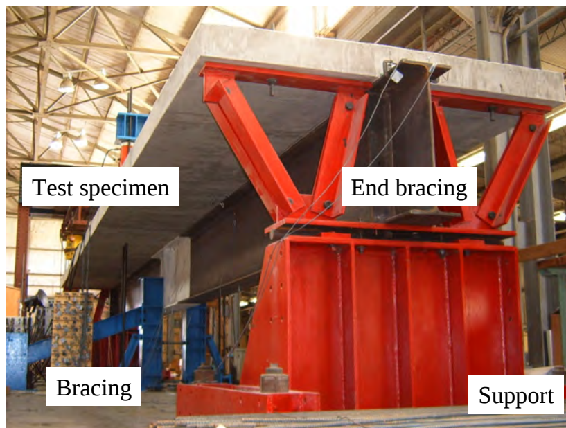
Figure 5.11: Test setup
