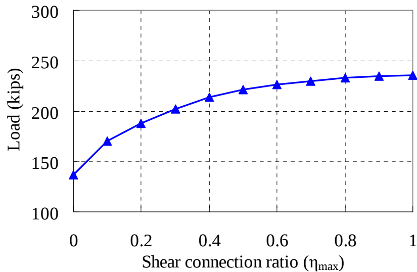
Figure 2.9: Ultimate load carrying capacity of a composite beam
