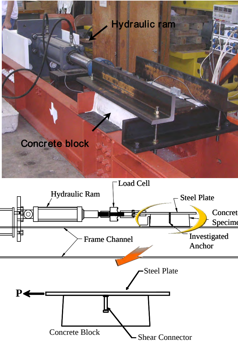
Figure 3.18: Test setup and test specimen for single-shear connector tests
