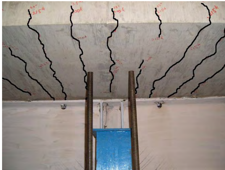
Figure 5.19: Specimen HASAA-30BS—Cracks on the bottom of the concrete slab (4.25-in deflection)
