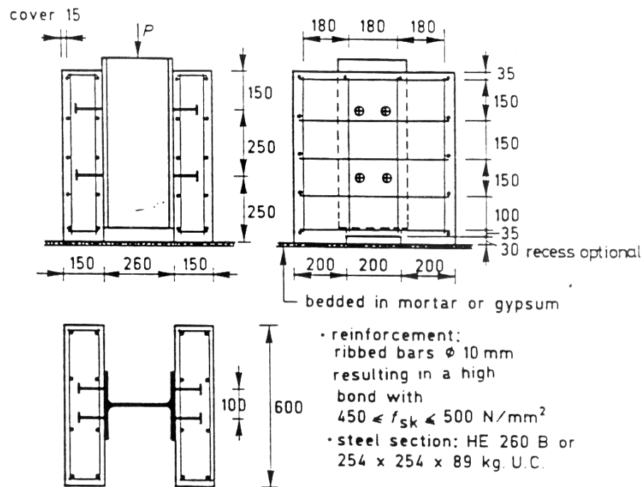
Figure 2.2: Push-out test setup according to the Eurocode (SI units)
