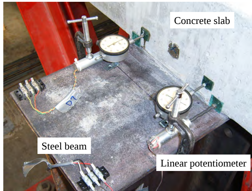
Figure 5.12: Linear potentiometers for measuring slip at the end of the specimen
