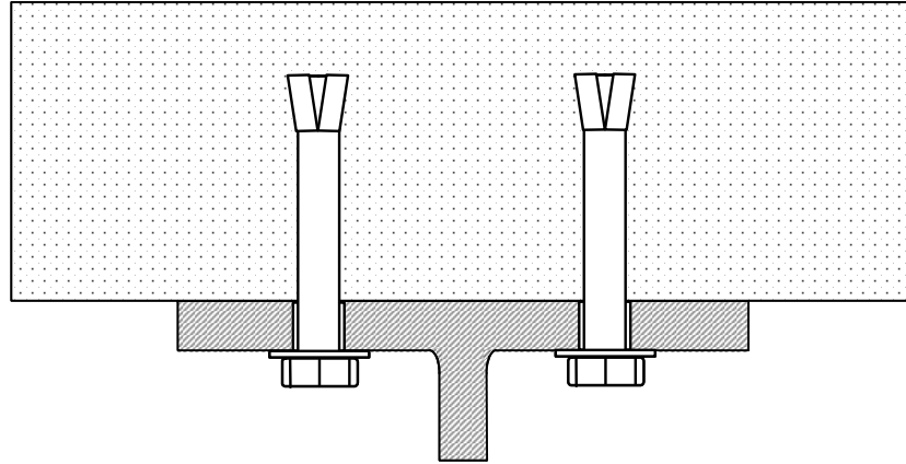
Figure 3.7: Expansion anchor
