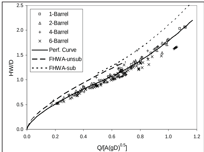
Figure 2: Performance curves for a box culvert without wingwalls, comparing the FHWA equations with results from this experimental program
