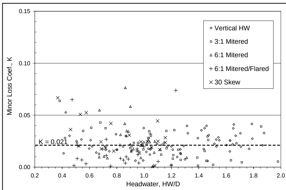
Figure 3: SET minor loss coefficient as a function of headwater for different culvert end configurations
