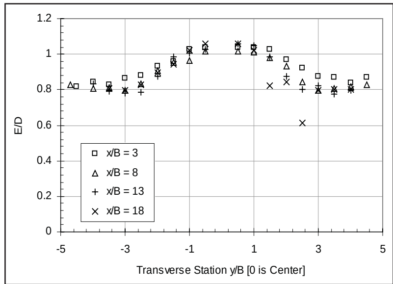
Figure 1: Measured specific energy distribution at different cross section distances ( x/B ) upstream of the model culvert system
