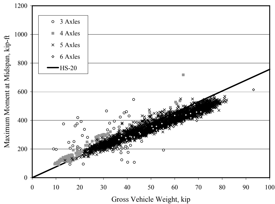
Figure 9.6 Maximum Moments at Midspan for 60-ft Span
