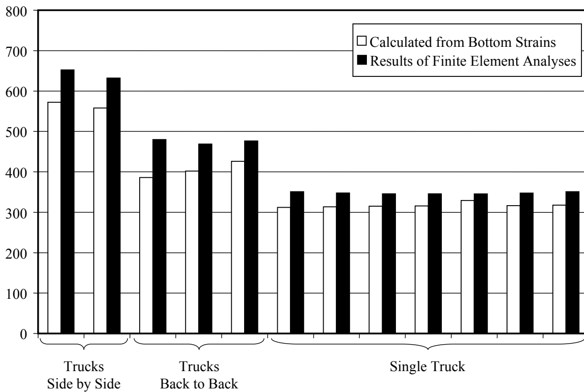
(b) Span 2
