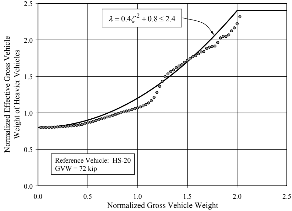
Figure 9.8 Idealized Variation of Gross Effective Weight of Heavier Vehicles
