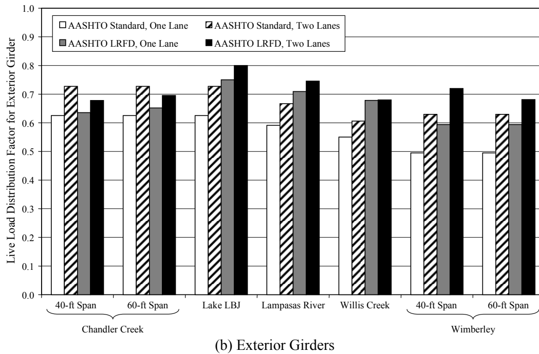
Figure A.3 Comparison of Live Load Distribution Factors Calculated Using AASHTO Standard and LRFD Specifications
