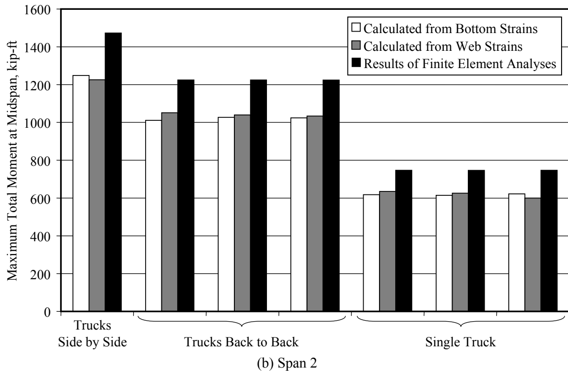
Figure 4.10 Total Live Load Moments at Midspan – Lampasas River Bridge
