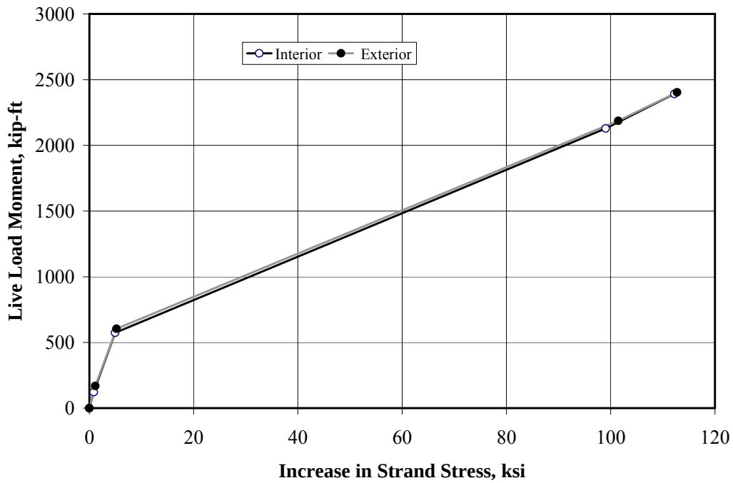
Figure B.4 Calculated Live Load Response of Lampasas River Bridge
