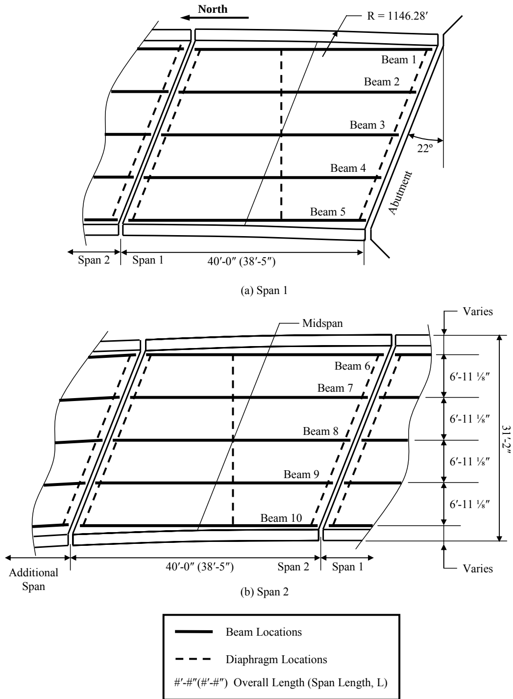
Figure 2.10 Plan of Wimberley Bridge
