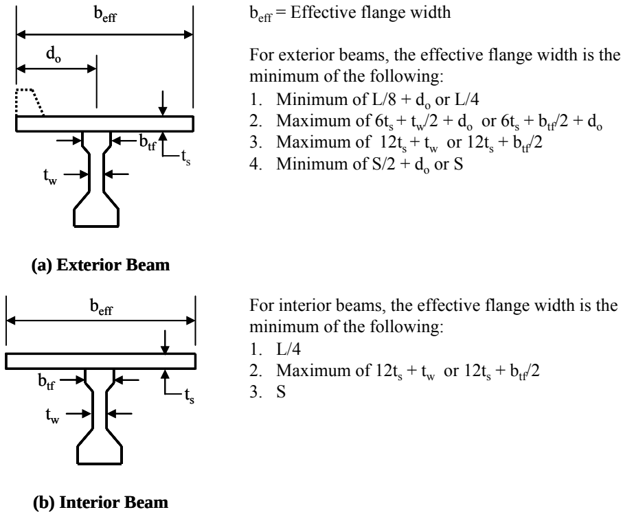
Figure 2.16 Definition of Effective Flange Width (AASHTO LRFD)
