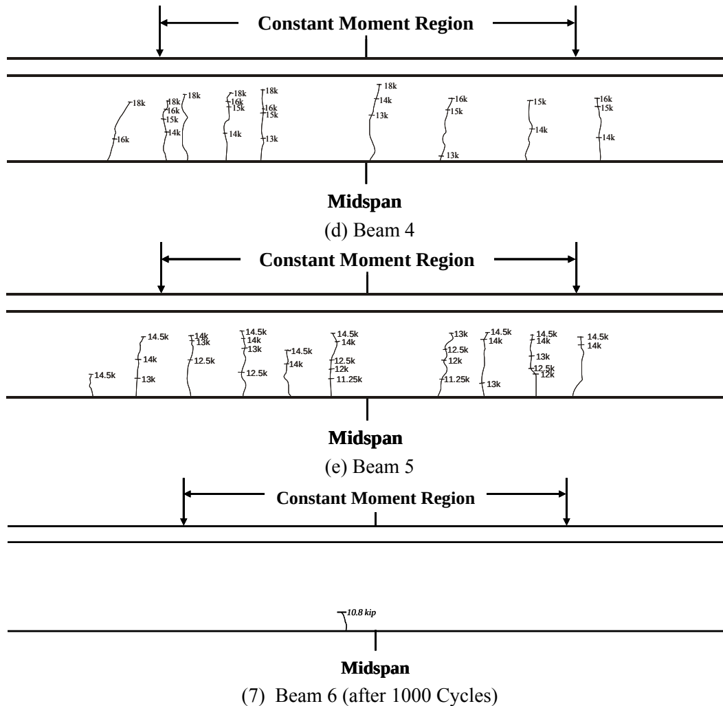
Figure 6.2 (cont.) Observed Crack Patterns Following Initial Static Tests
