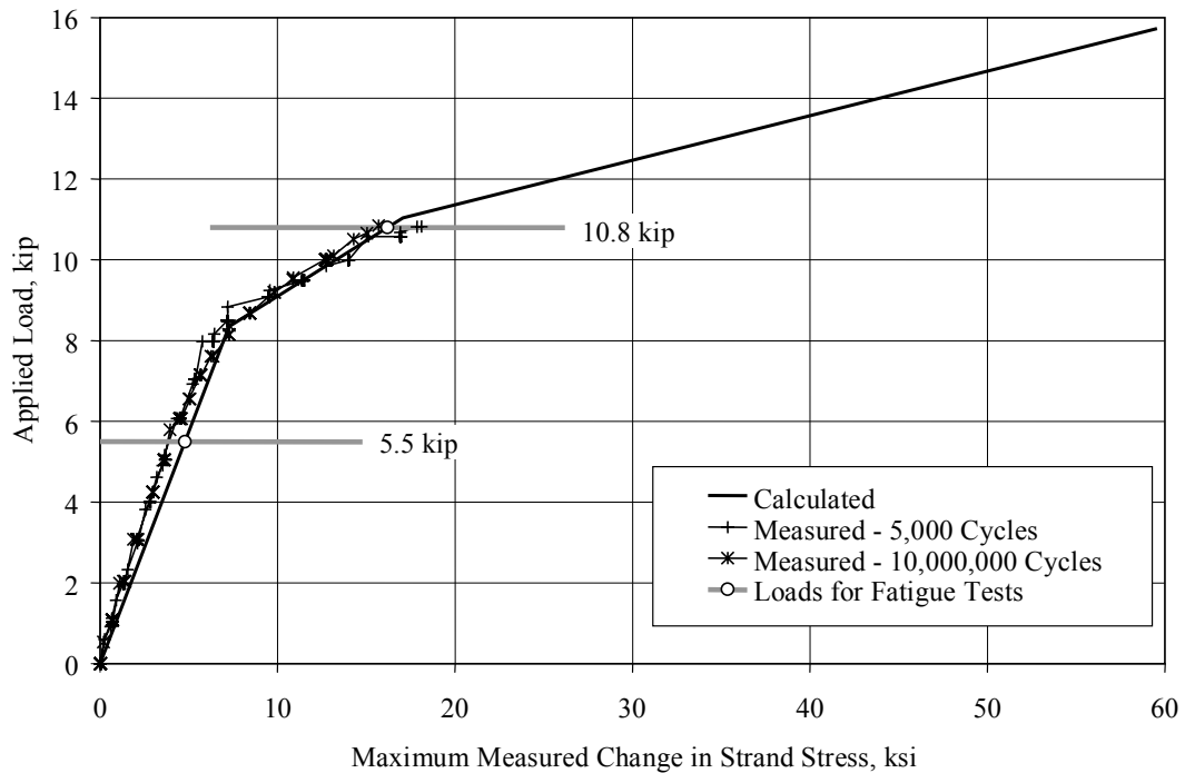
Figure 6.14 Comparison of Calculated and Measured Response of Beam 6
