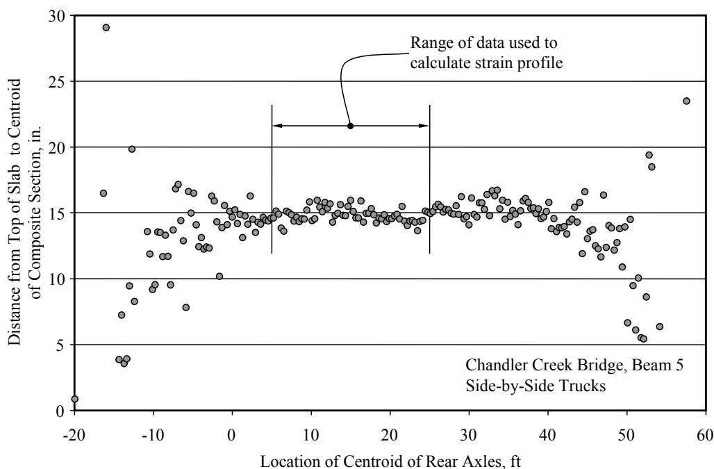
Figure 4.3 Distance from Top of Slab to Centroid of Composite Section Calculated from Measured Strain Data
