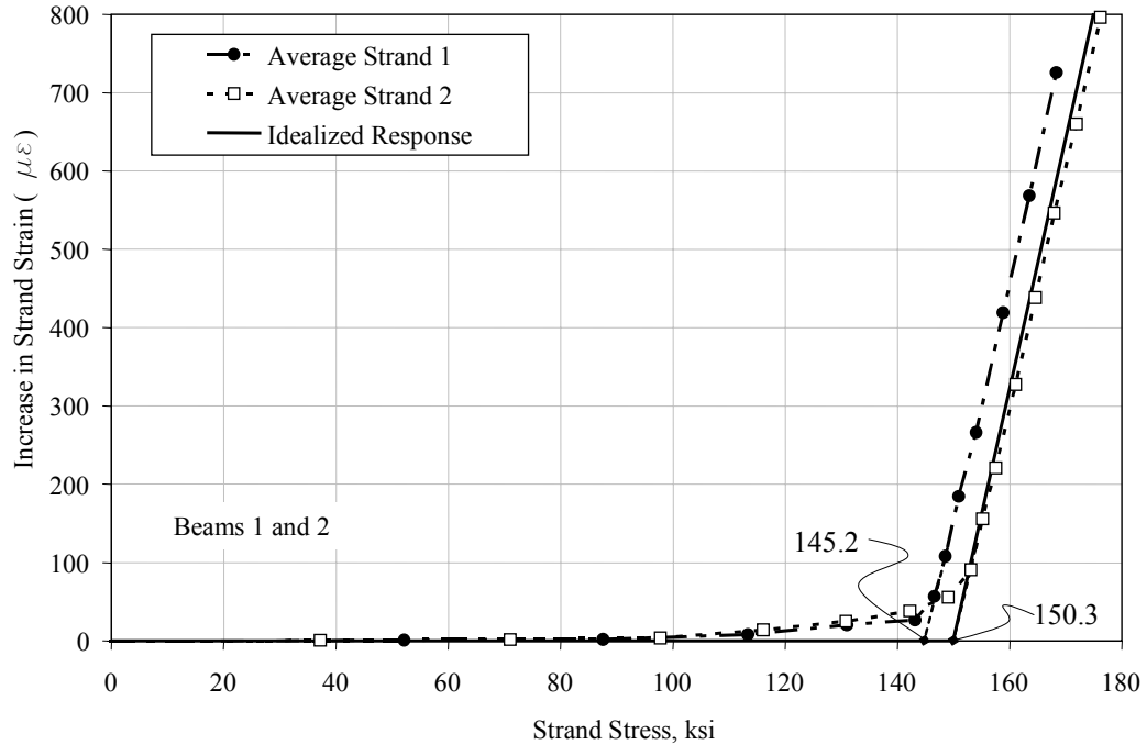
Figure 5.9 Variation of Strand Strain and Stress During Load Test
