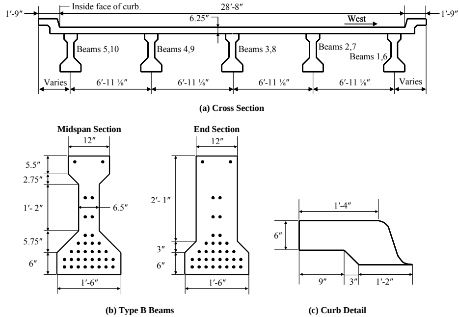
Figure 2.15 Cross Section, Beam and Curb Details for Wimberley Bridge
