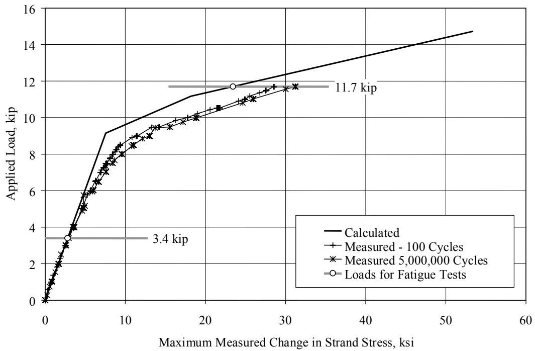
Figure 6.10 Comparison of Calculated and Measured Response of Beam 2
