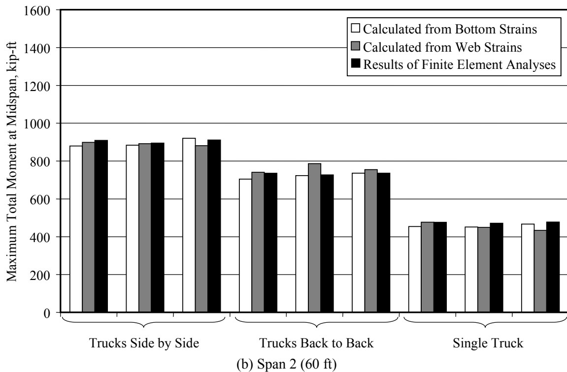
Figure 4.8 Total Live Load Moments at Midspan – Chandler Creek Bridge
