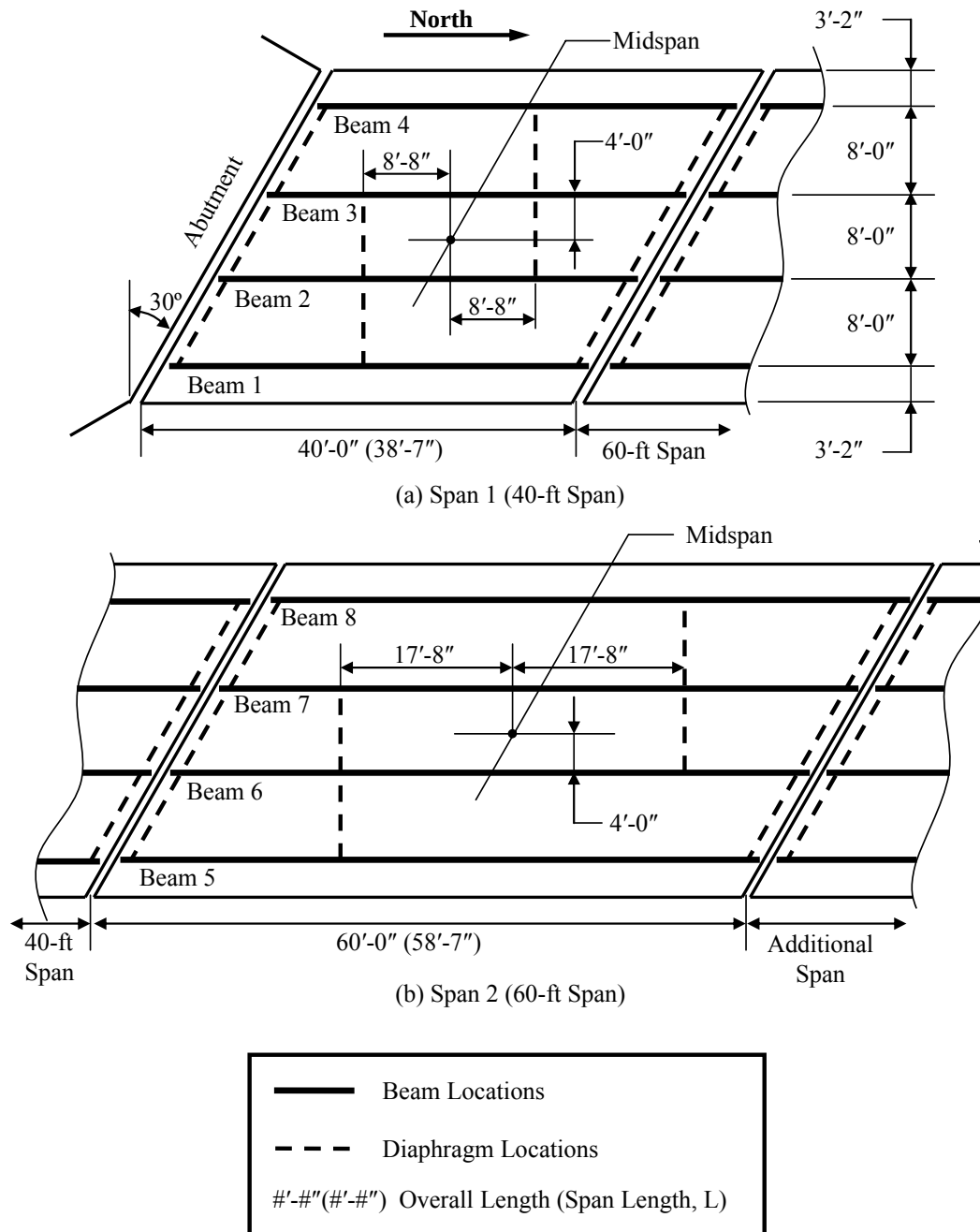
Figure 2.2 Plan of Chandler Creek Bridge
