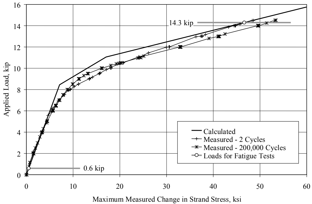
Figure 6.13 Comparison of Calculated and Measured Response of Beam 5
